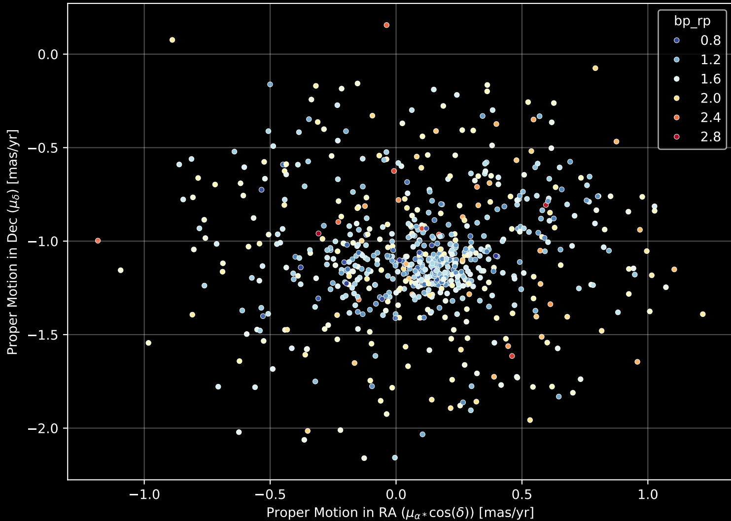
Gaia Cluster: [ASCC_9] Proper Motion Diagram (n= 711)
