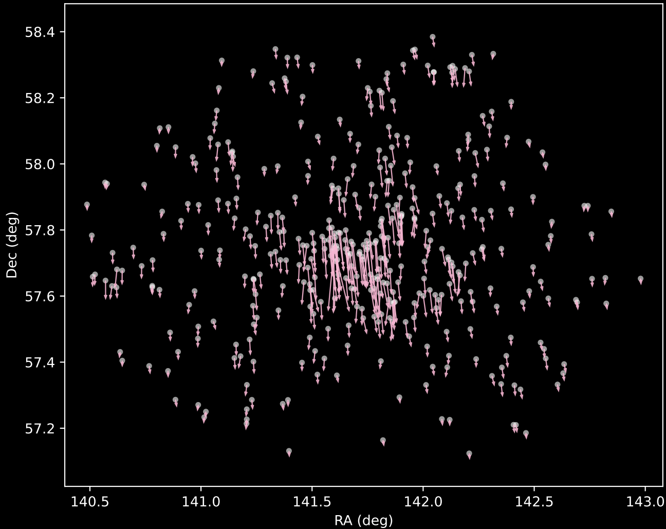
Gaia DR3 Cluster 13 Proper Motion Vectors (n=402)
