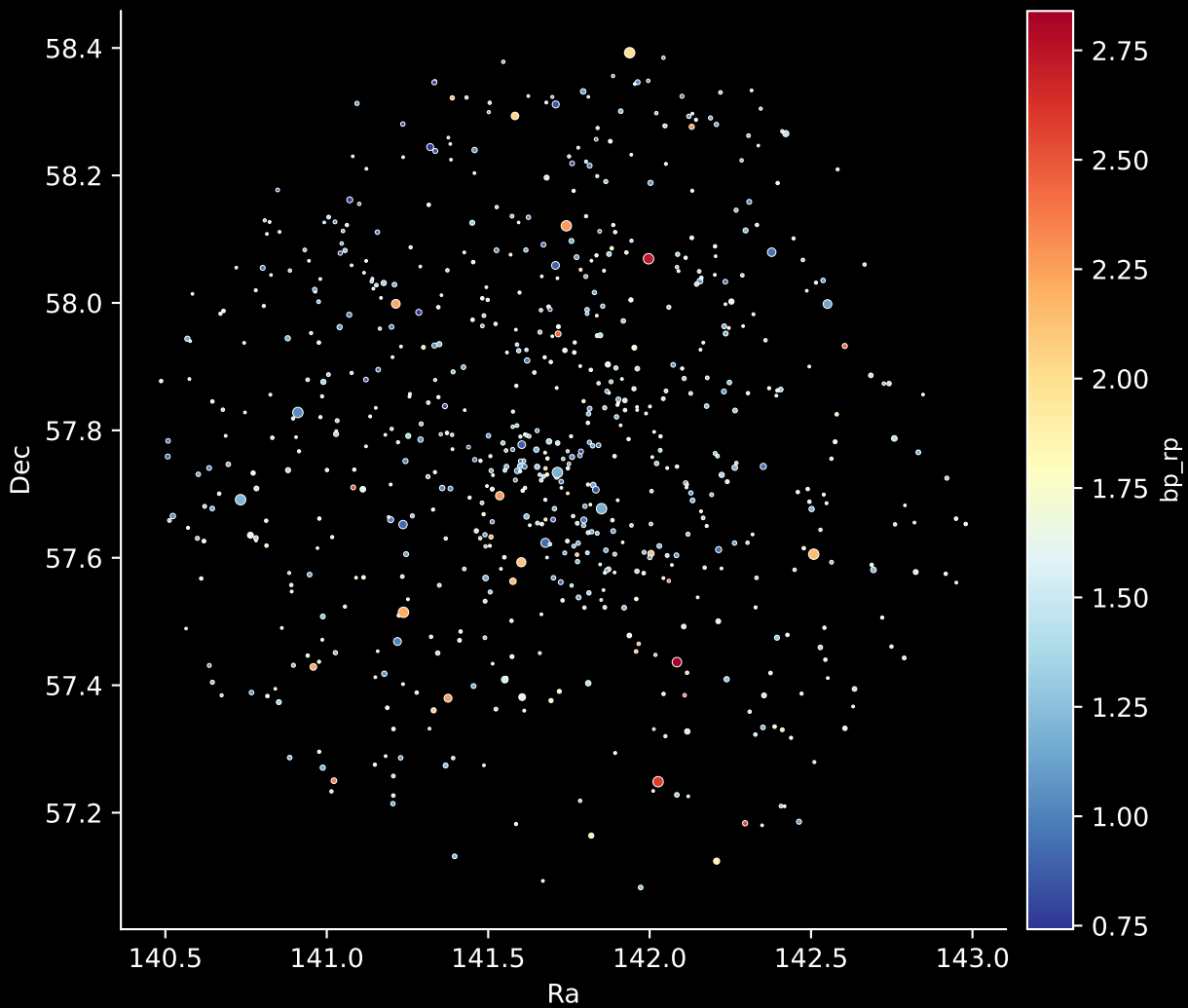
Gaia Cluster: [ASCC_9] Stars: 711
