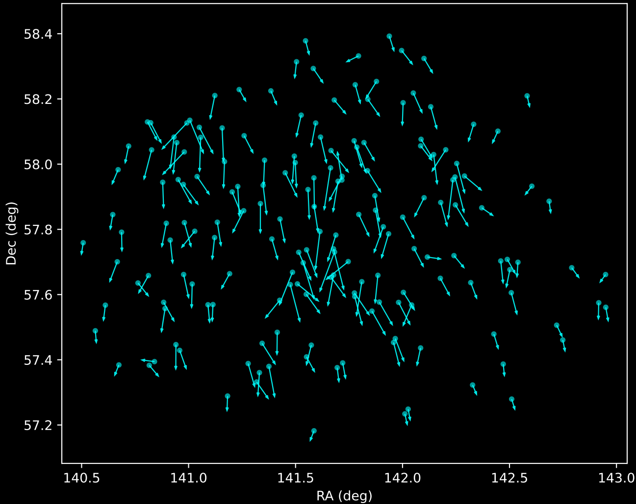
Gaia DR3 Noise Stream Proper Motion Vectors (n=172)
