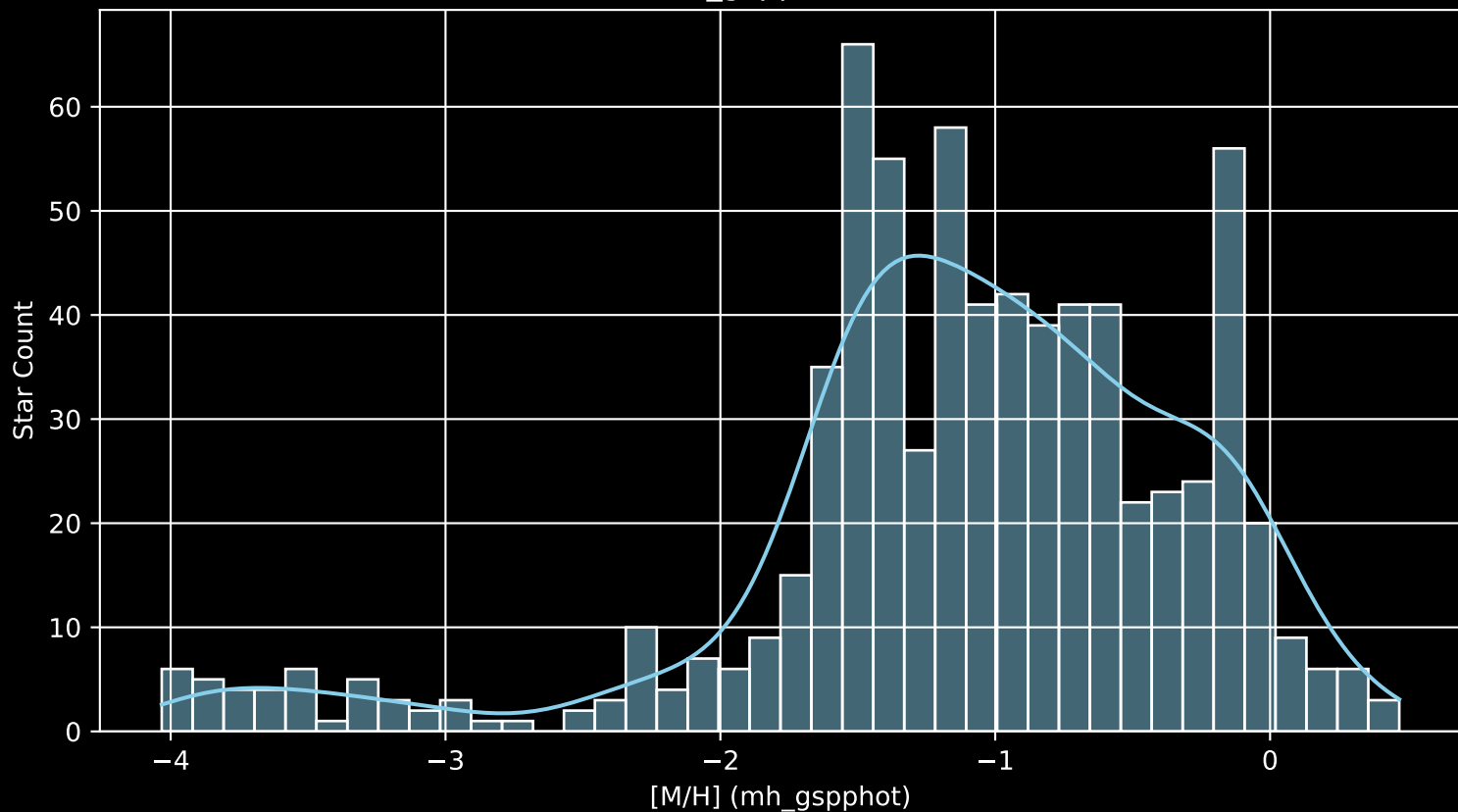
Gaia Cluster: [ASCC_9 [M/H] (mh_gspphot) (n= 711)
