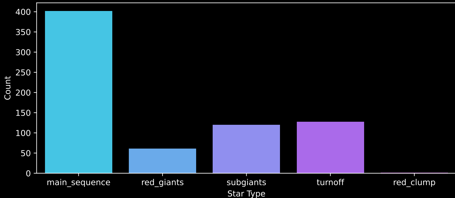
Gaia Cluster: [ASCC_9] Count plot of Star Type
