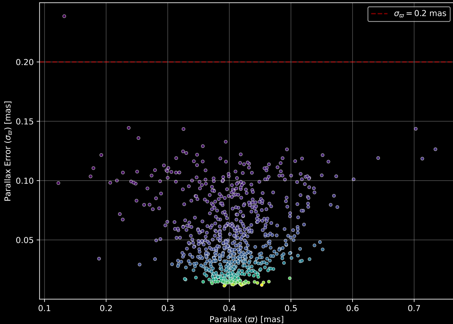
Gaia Cluster: [ASCC_9] Parallax Quality (n= 711)
