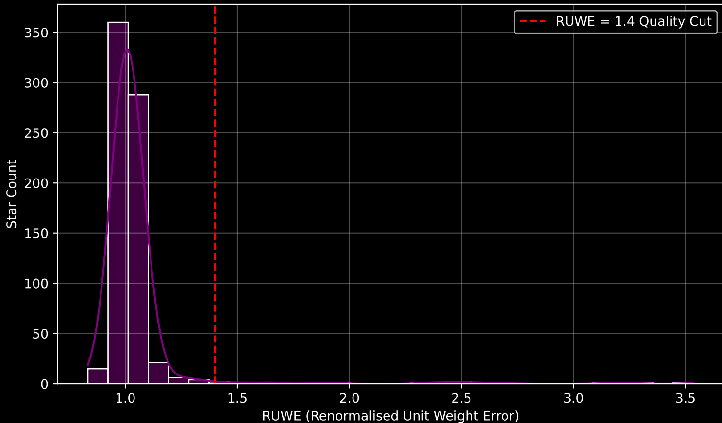
Gaia Cluster: [ASCC_9] RUWE Distribution (n= 710)
