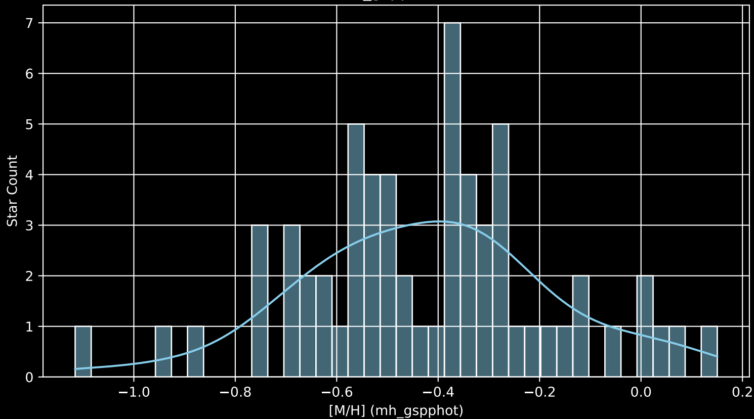
Gaia Cluster: [ASCC_90 [M/H] (mh_gspphot) (n= 62)
