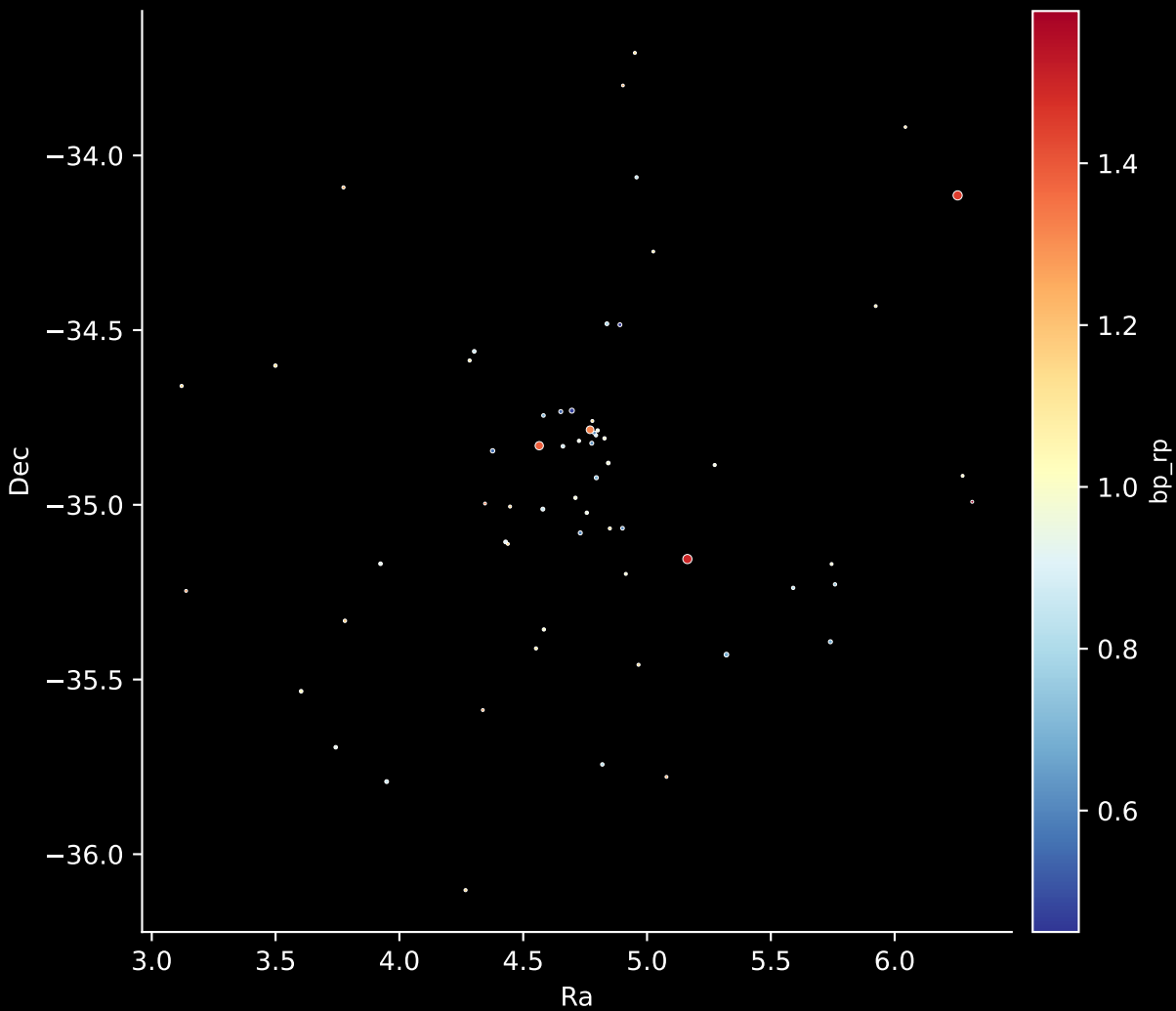
Gaia Cluster: [ASCC_90] Stars: 63
