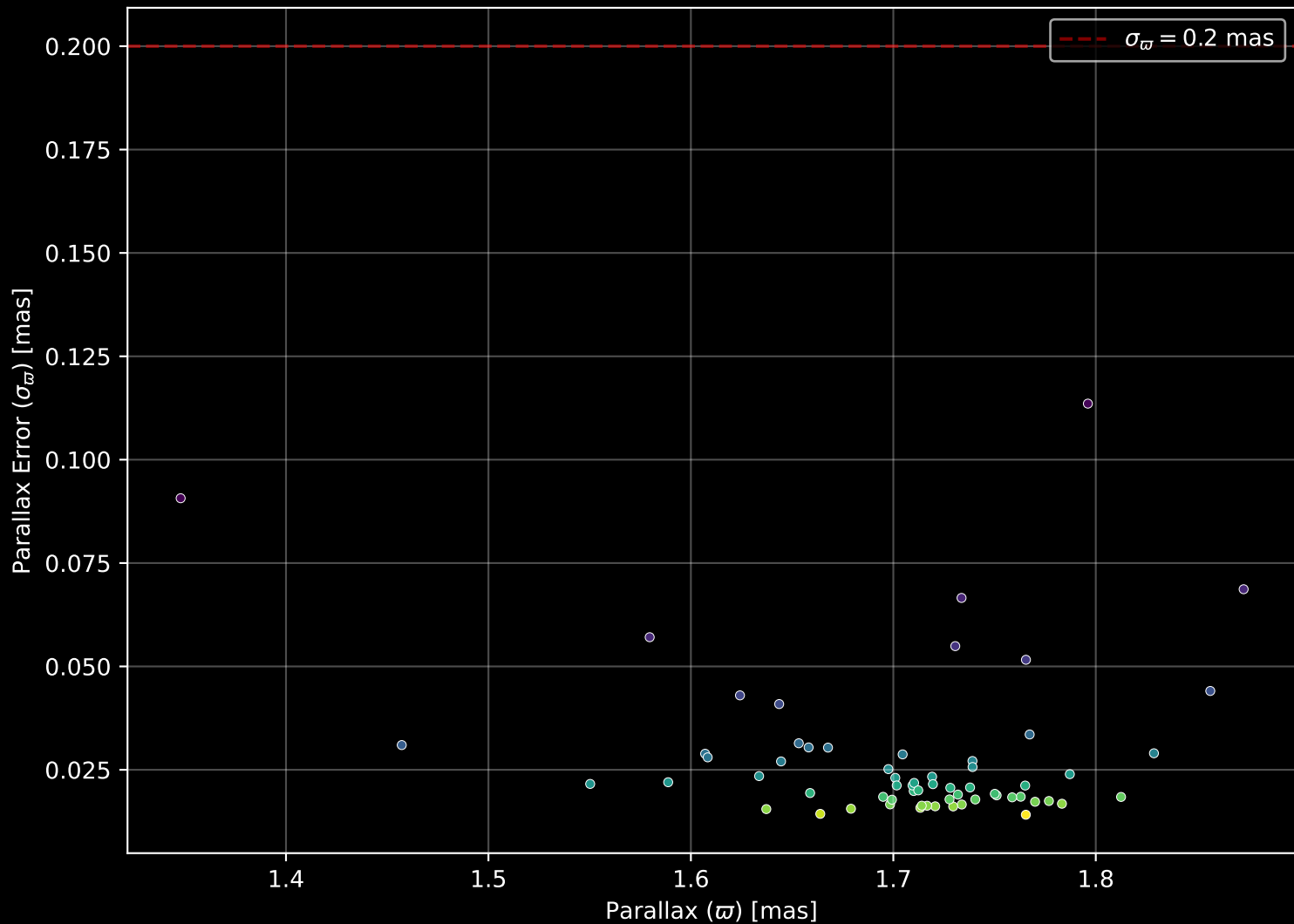
Gaia Cluster: [ASCC 90] Parallax Quality (n= 63)
