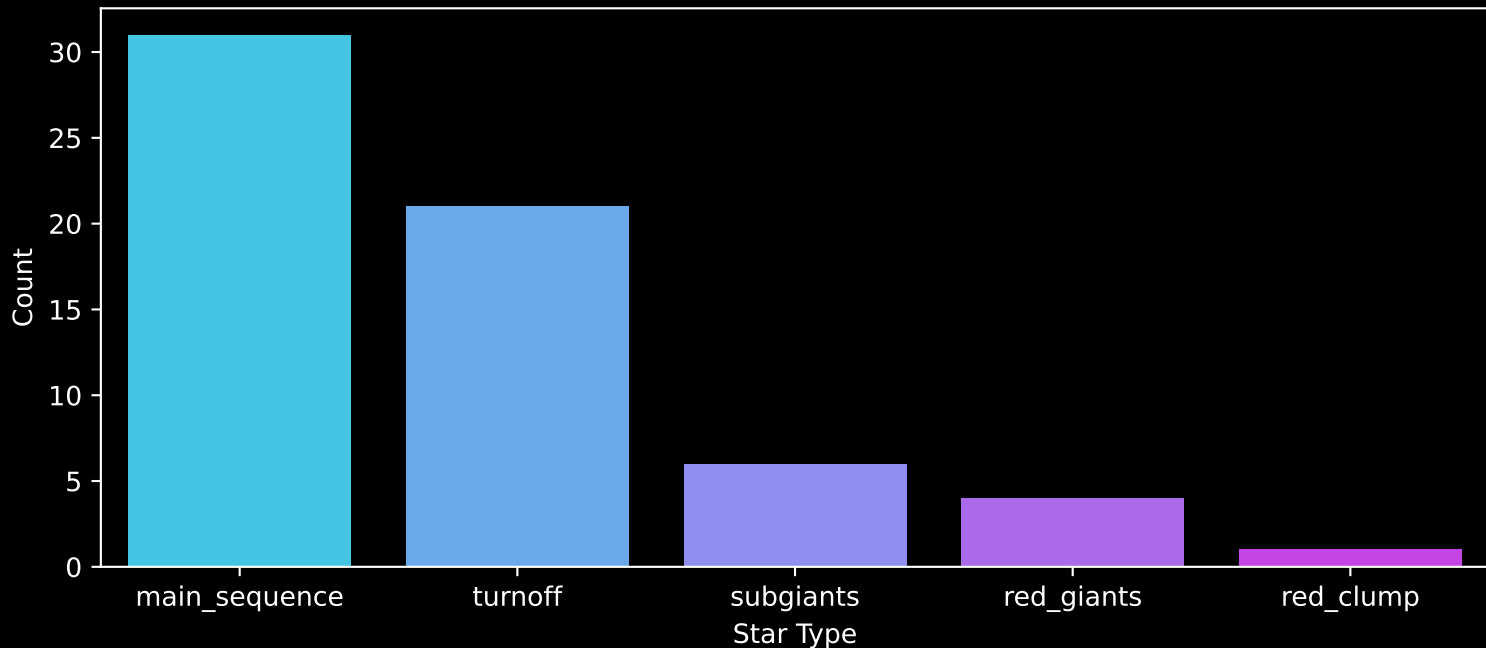
Gaia Cluster: [ASCC_90] Count plot of Star Type
