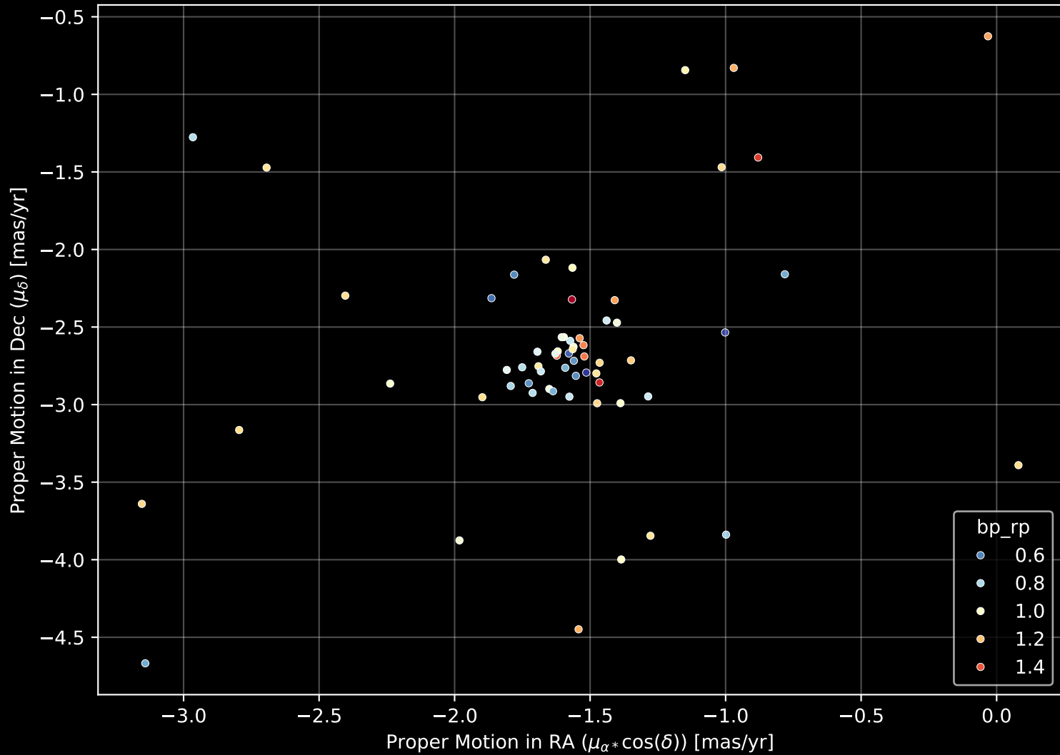
Gaia Cluster: [ASCC_90] Proper Motion Diagram (n= 63)
