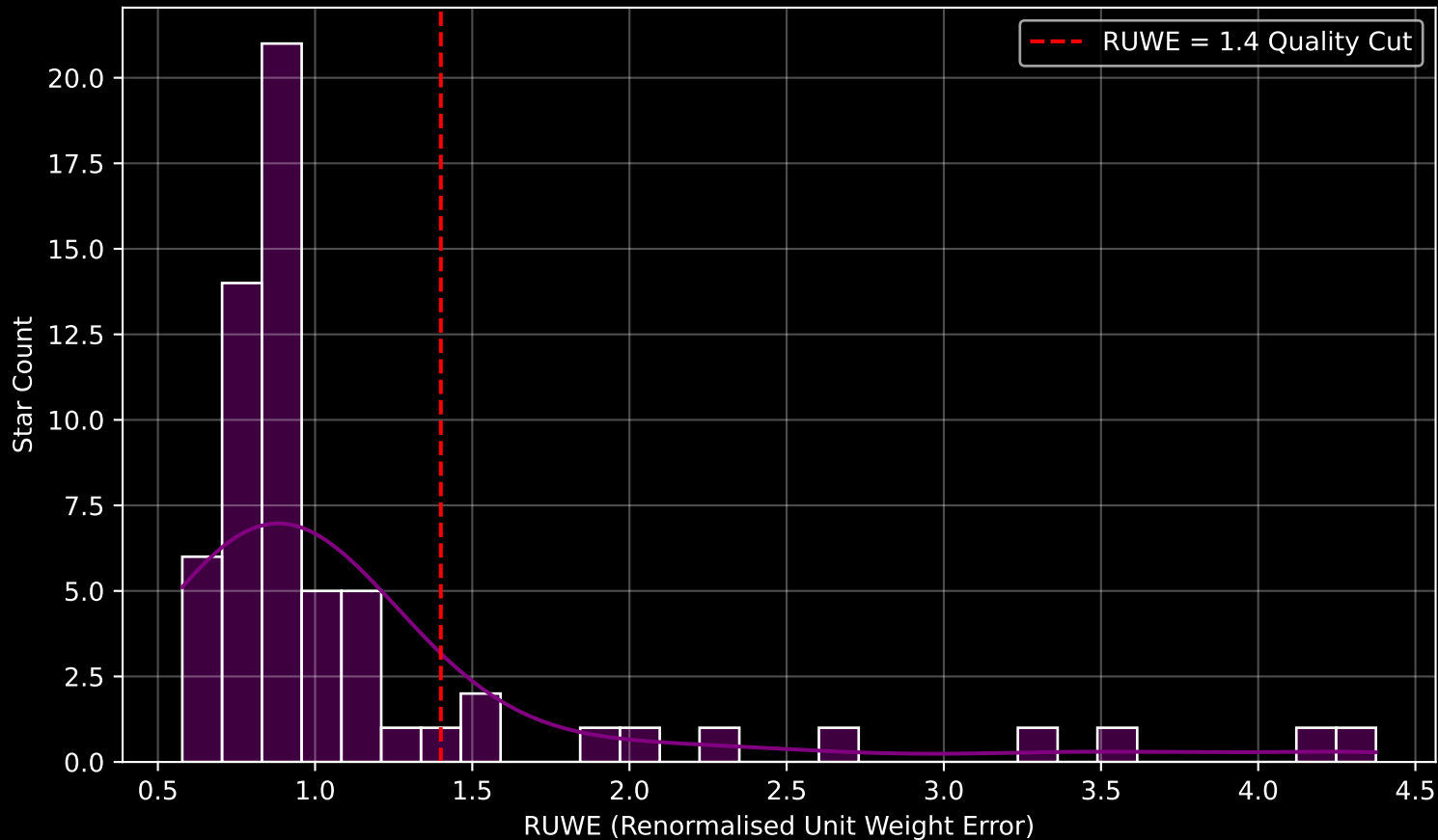
Gaia Cluster: [ASCC_90] RUWE Distribution (n= 63)
