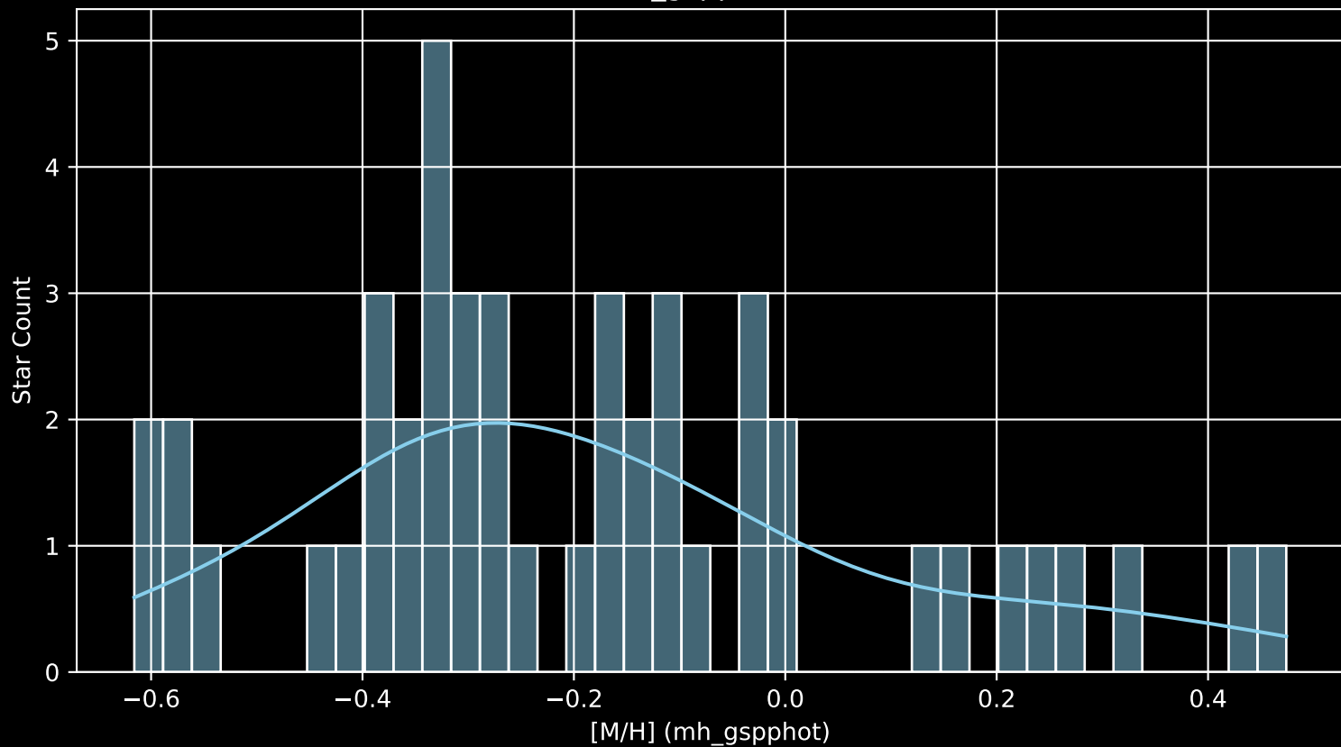
Gaia Cluster: [Alessi_1 [M/H] (mh_gspphot) (n= 47)
