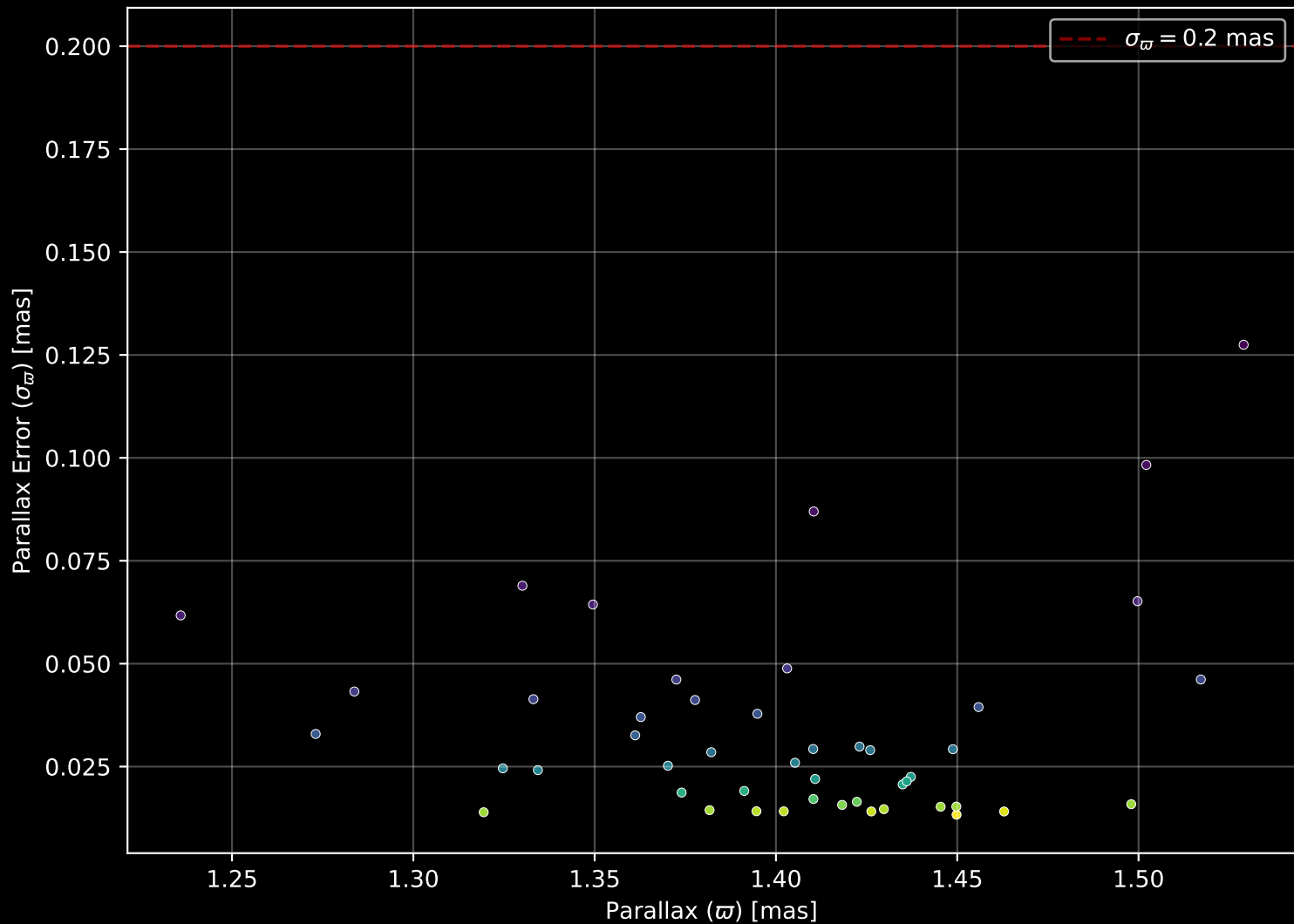
Gaia Cluster: [Alessi_1] Parallax Quality (n= 47)
