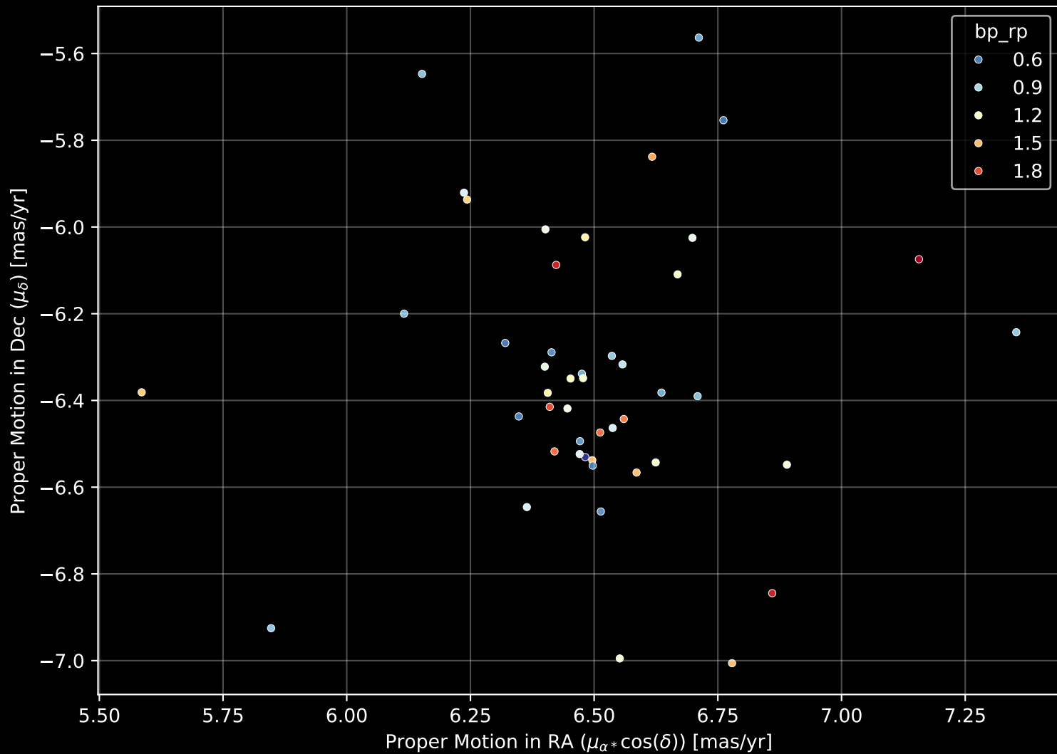
Gaia Cluster: [Alessi_1] Proper Motion Diagram (n= 47)
