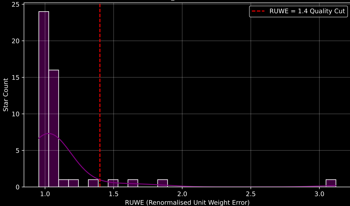
Gaia Cluster: [Alessi_1] RUWE Distribution (n= 47)
