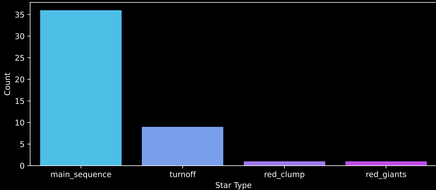
Gaia Cluster: [Alessi_1] Count plot of Star Type
