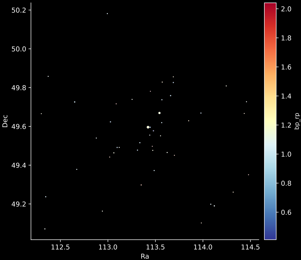
Gaia Cluster: [Alessi_1] Stars: 47
