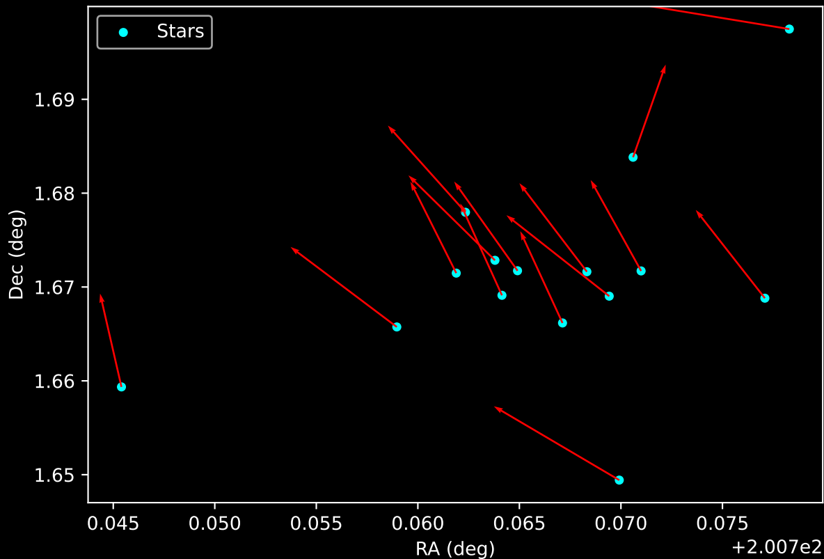
Gaia Cluster: [Alessi_15] Proper Motion Vectors for Gaia Star Field (n= 15)
