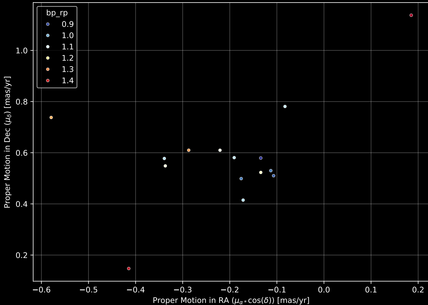
Gaia Cluster: [Alessi_15] Proper Motion Diagram (n= 15)
