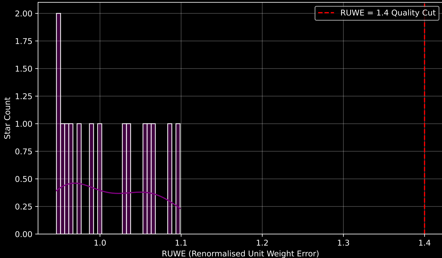
Gaia Cluster: [Alessi_15] RUWE Distribution (n= 15)
