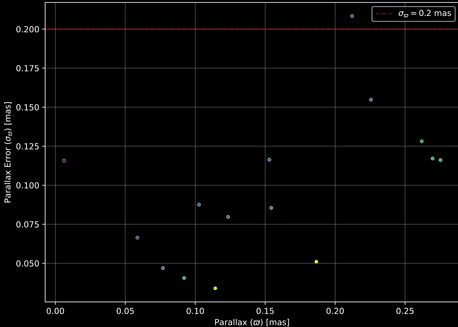
Gaia Cluster: [Alessi_15] Parallax Quality (n= 15)
