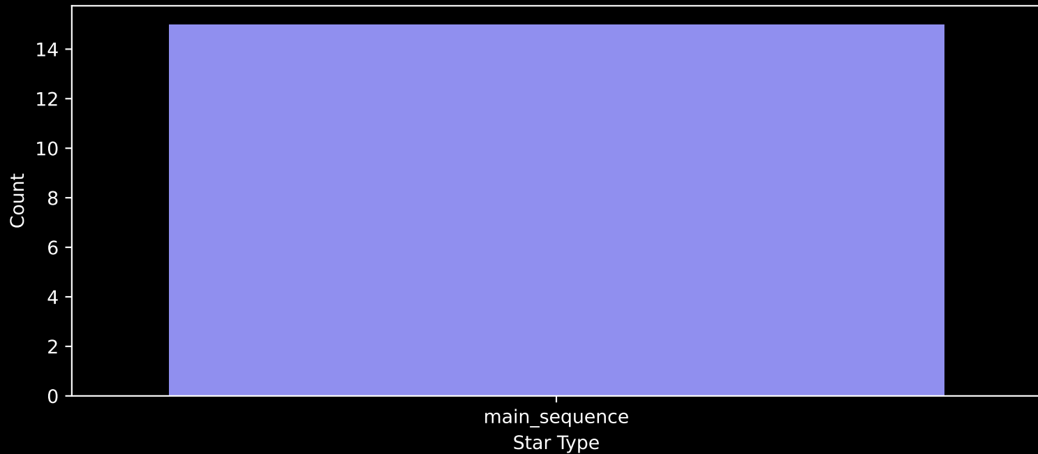
Gaia Cluster: [Alessi_15] Count plot of Star Type
