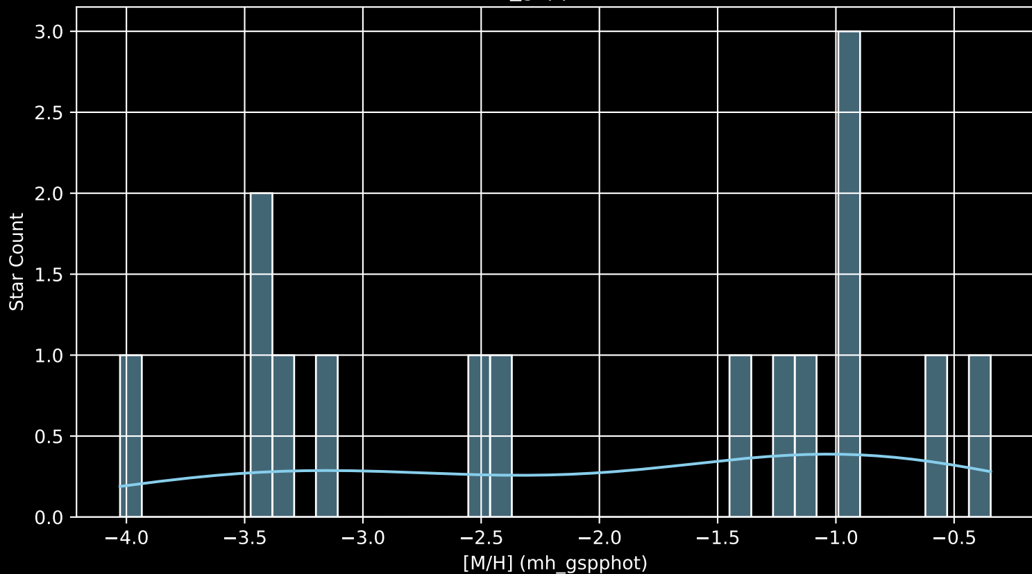
Gaia Cluster: [Alessi_15 [M/H] (mh_gspphot) (n= 15)
