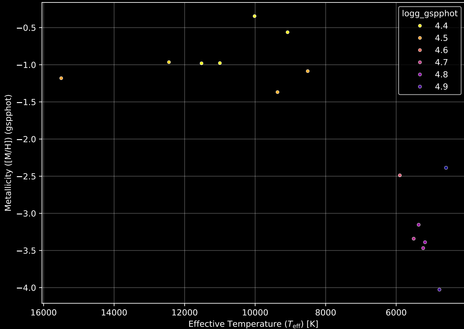
Gaia Cluster: [Alessi_15] Stellar Population Parameters (n= 15)
