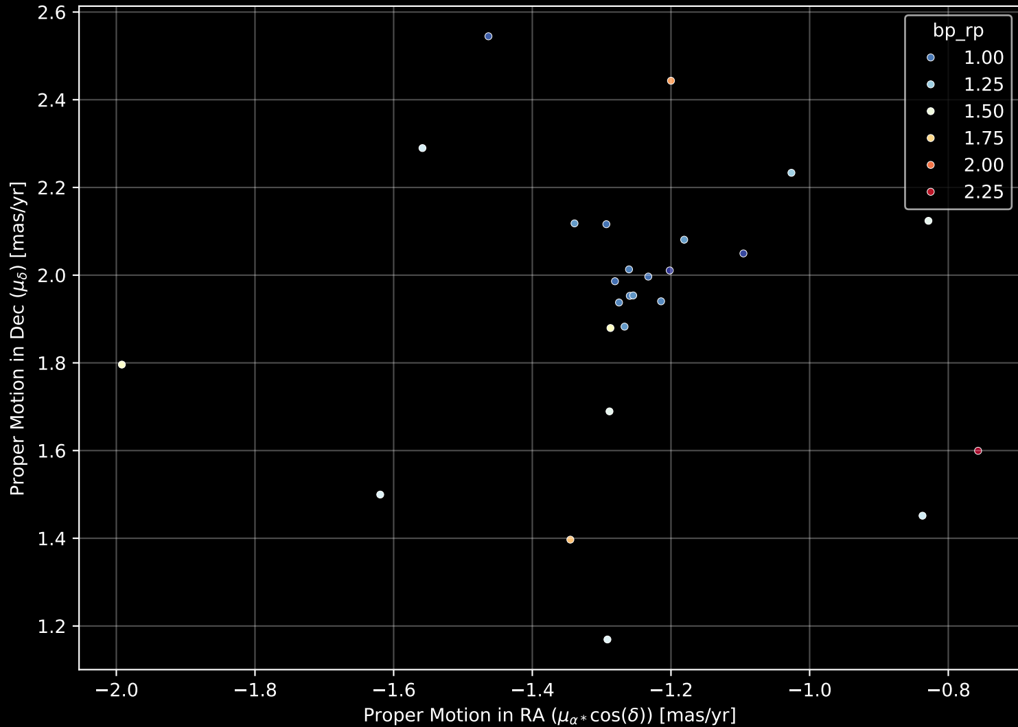
Gaia Cluster: [Alessi_18] Proper Motion Diagram (n= 26)
