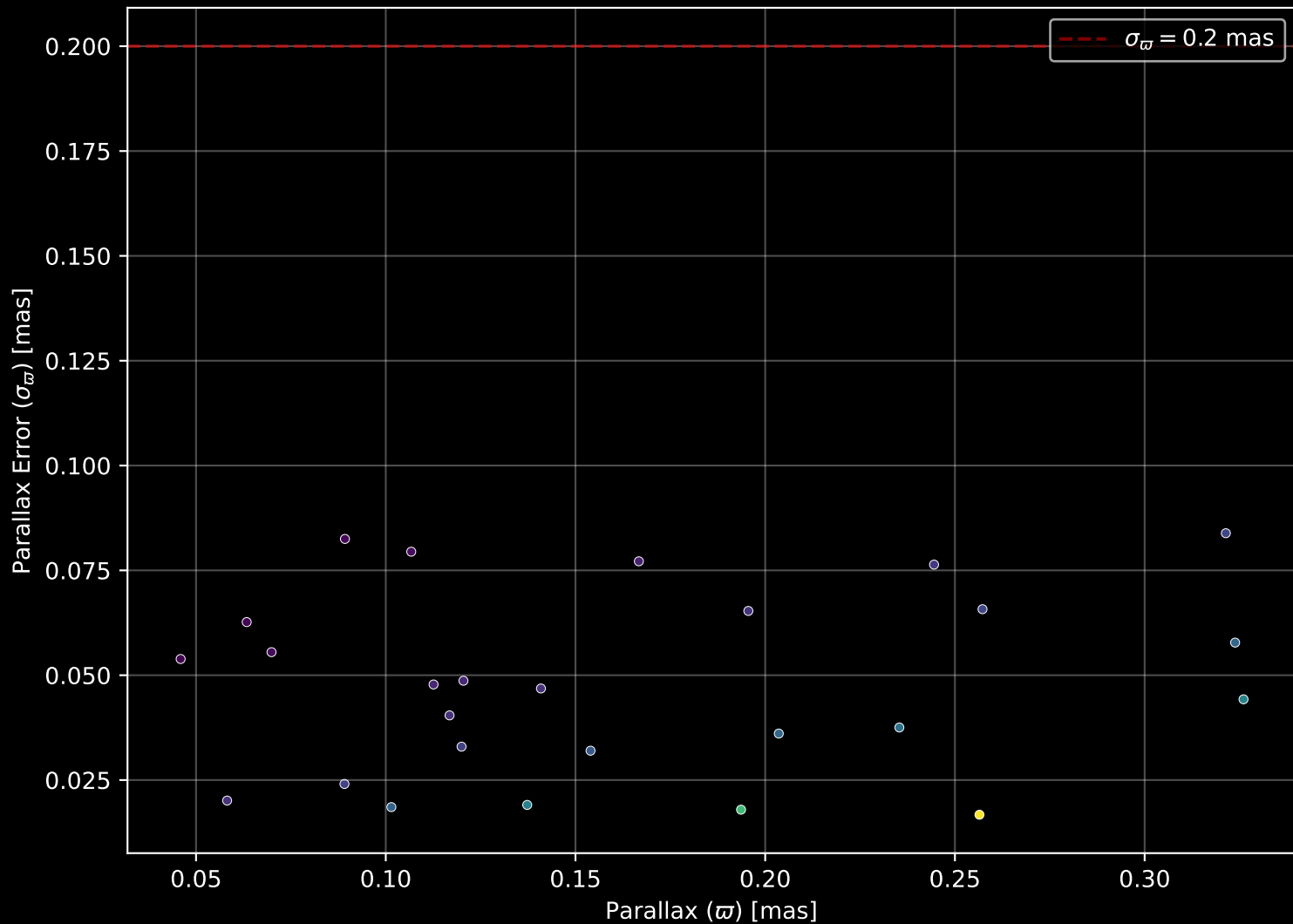
Gaia Cluster: [Alessi_18] Parallax Quality (n= 26)
