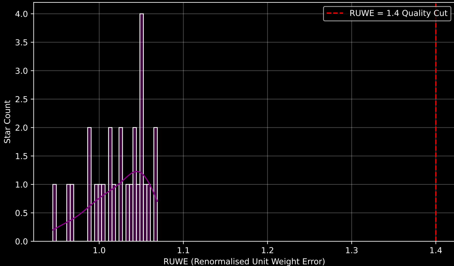
Gaia Cluster: [Alessi_18] RUWE Distribution (n= 26)
