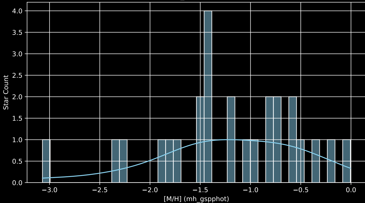
Gaia Cluster: [Alessi_18 [M/H] (mh_gspphot) (n= 26)
