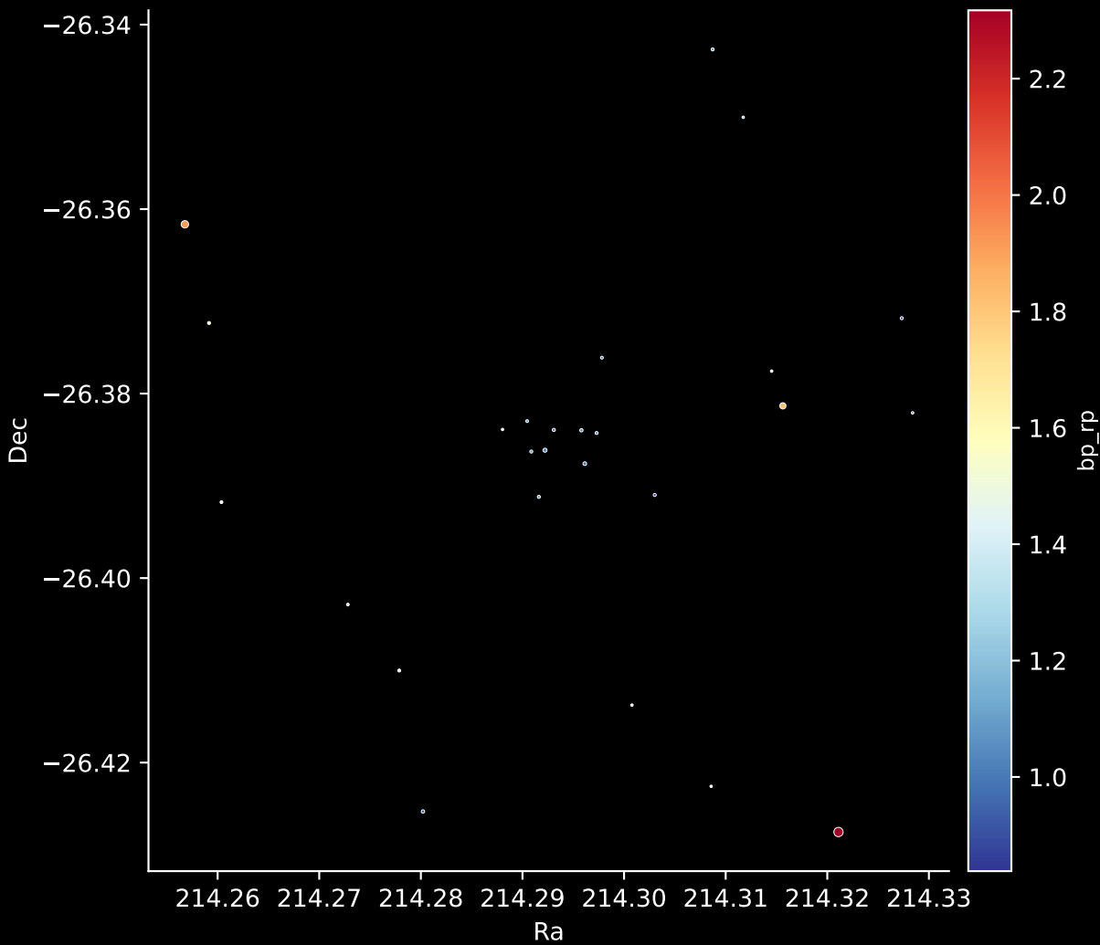
Gaia Cluster: [Alessi_18] Stars: 26
