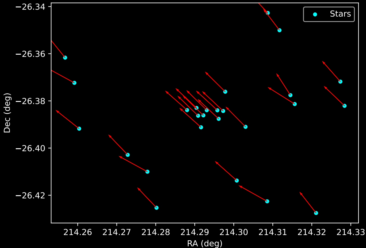
Gaia Cluster: [Alessi_18] Proper Motion Vectors for Gaia Star Field (n= 26)
