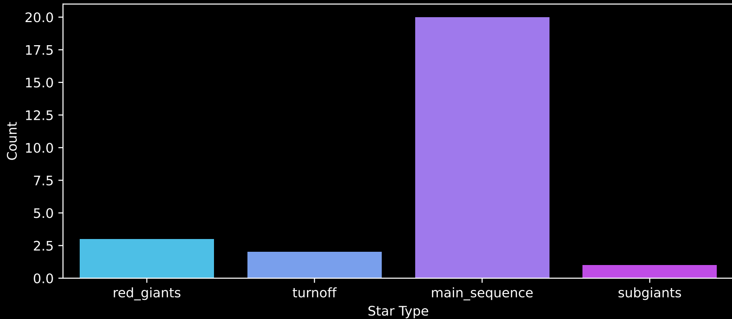
Gaia Cluster: [Alessi_18] Count plot of Star Type
