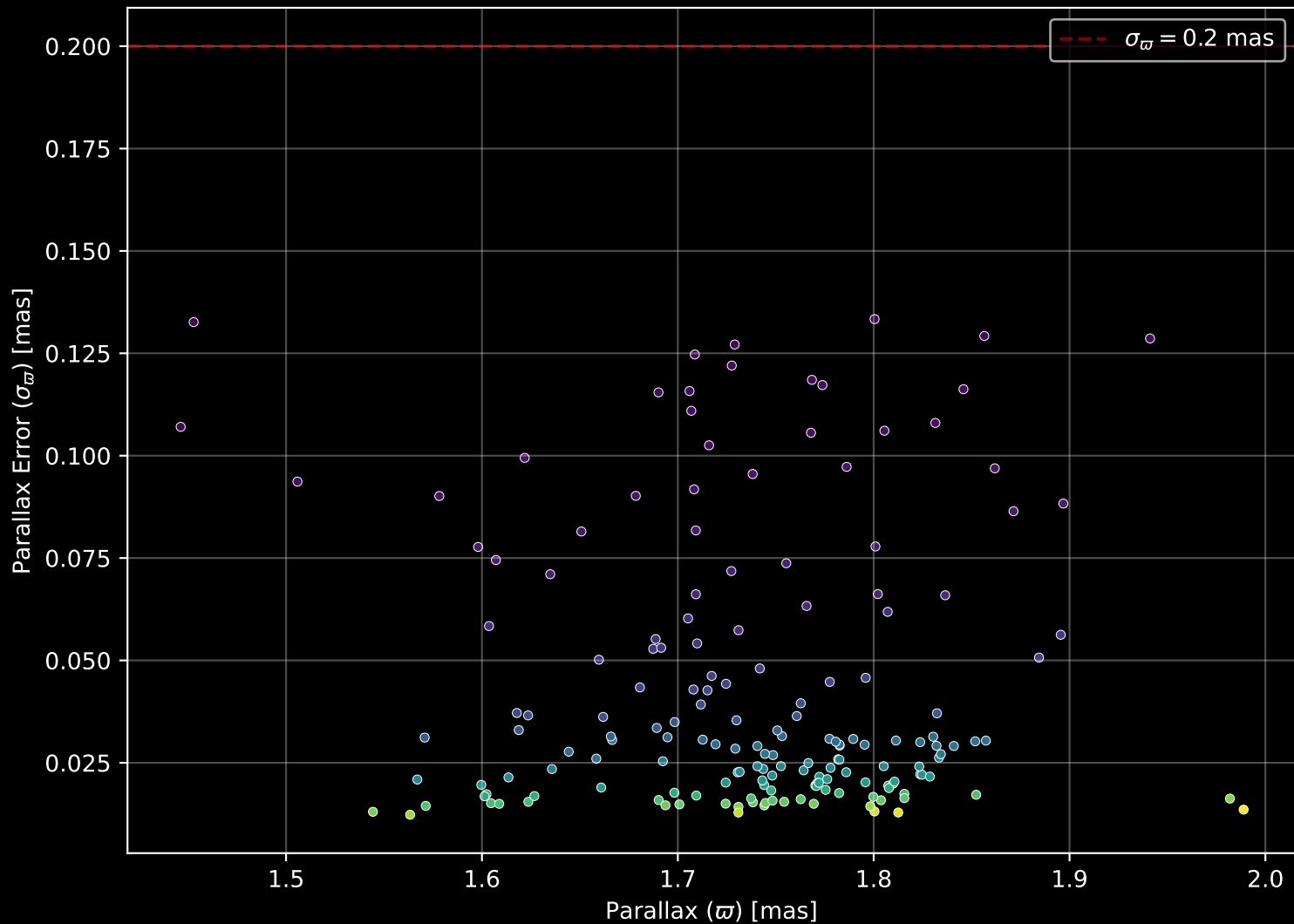
Gaia Cluster: [Alessi_21] Parallax Quality (n= 174)
