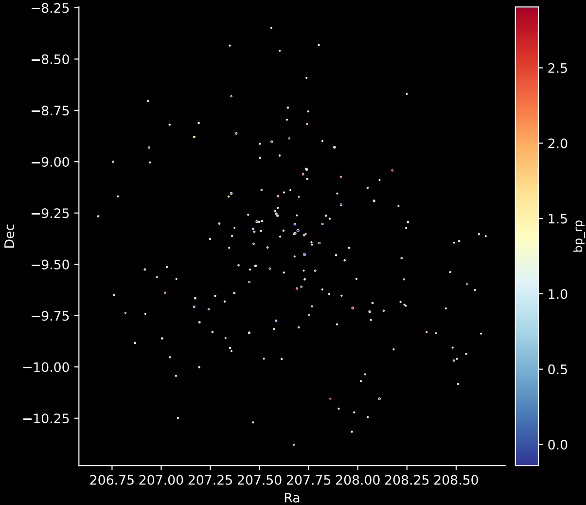
Gaia Cluster: [Alessi_21] Stars: 174
