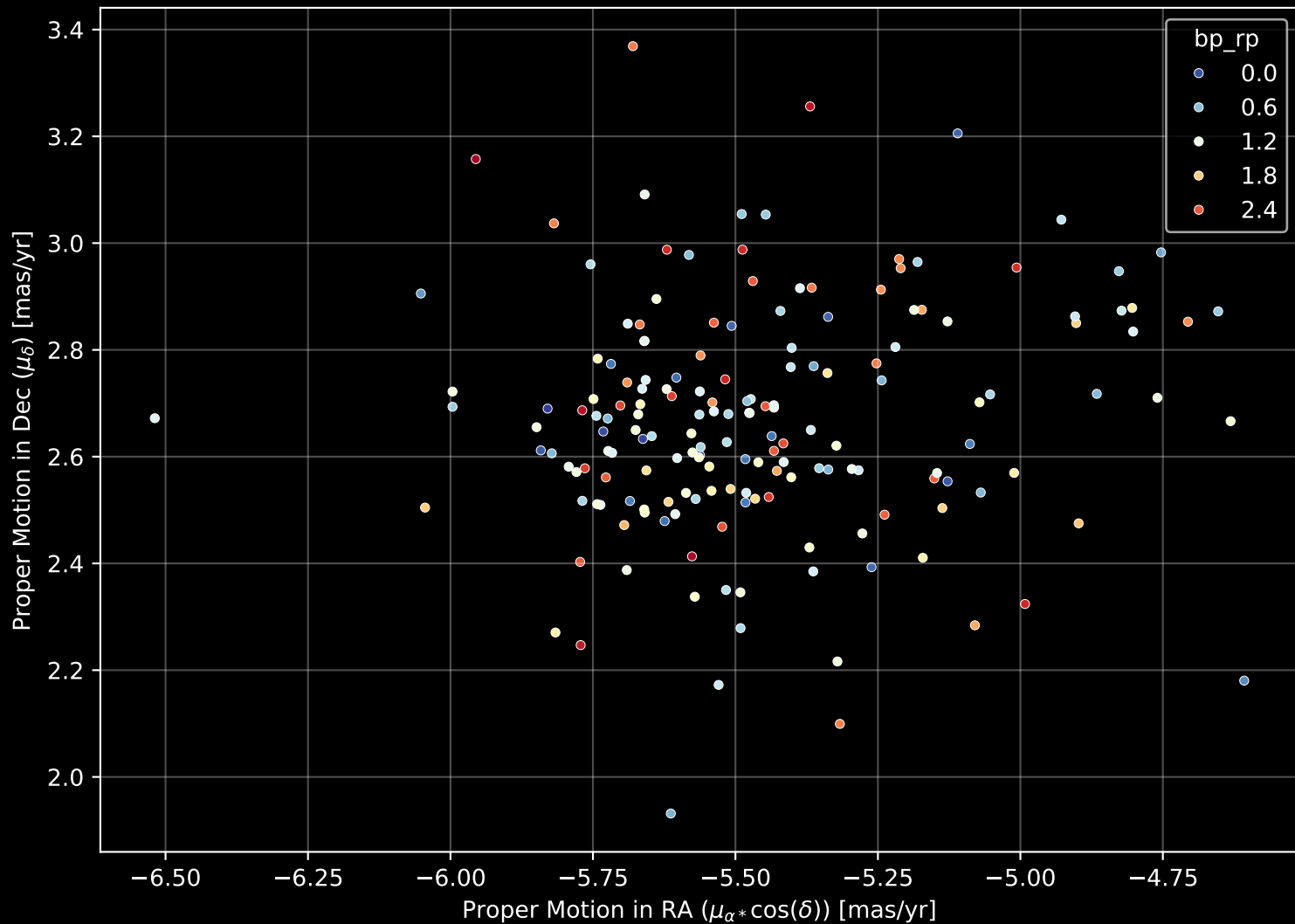
Gaia Cluster: [Alessi_21] Proper Motion Diagram (n= 174)
