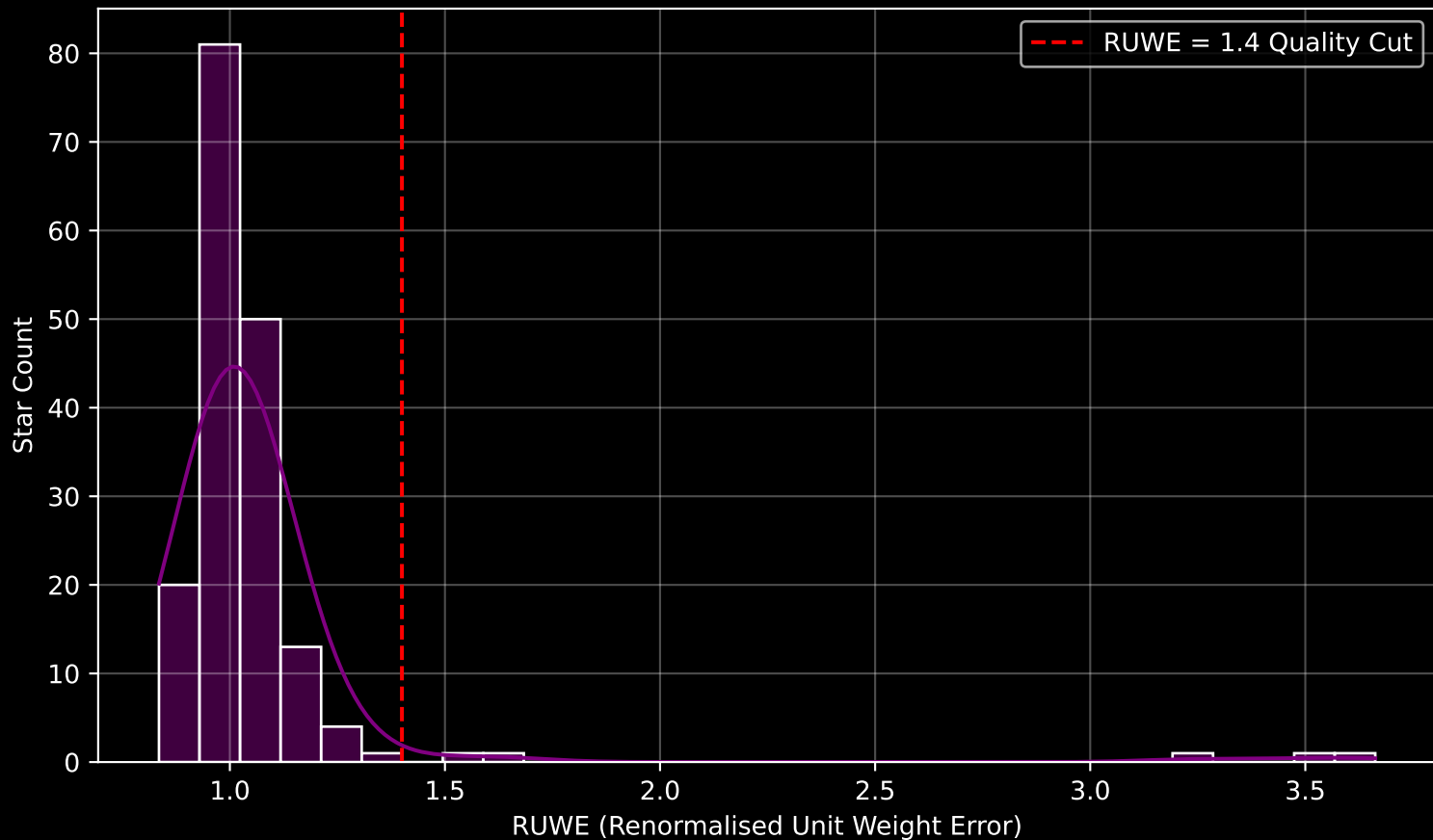
Gaia Cluster: [Alessi_21] RUWE Distribution (n= 174)
