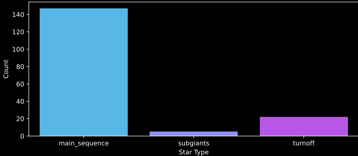
Gaia Cluster: [Alessi_21] Count plot of Star Type
