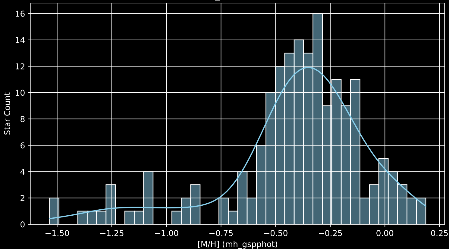
Gaia Cluster: [Alessi_21 [M/H] (mh_gspphot) (n= 174)
