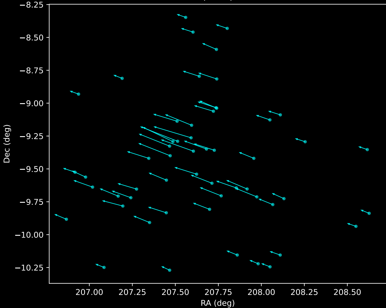
Gaia DR3 Noise Stream Proper Motion Vectors (n=55)
