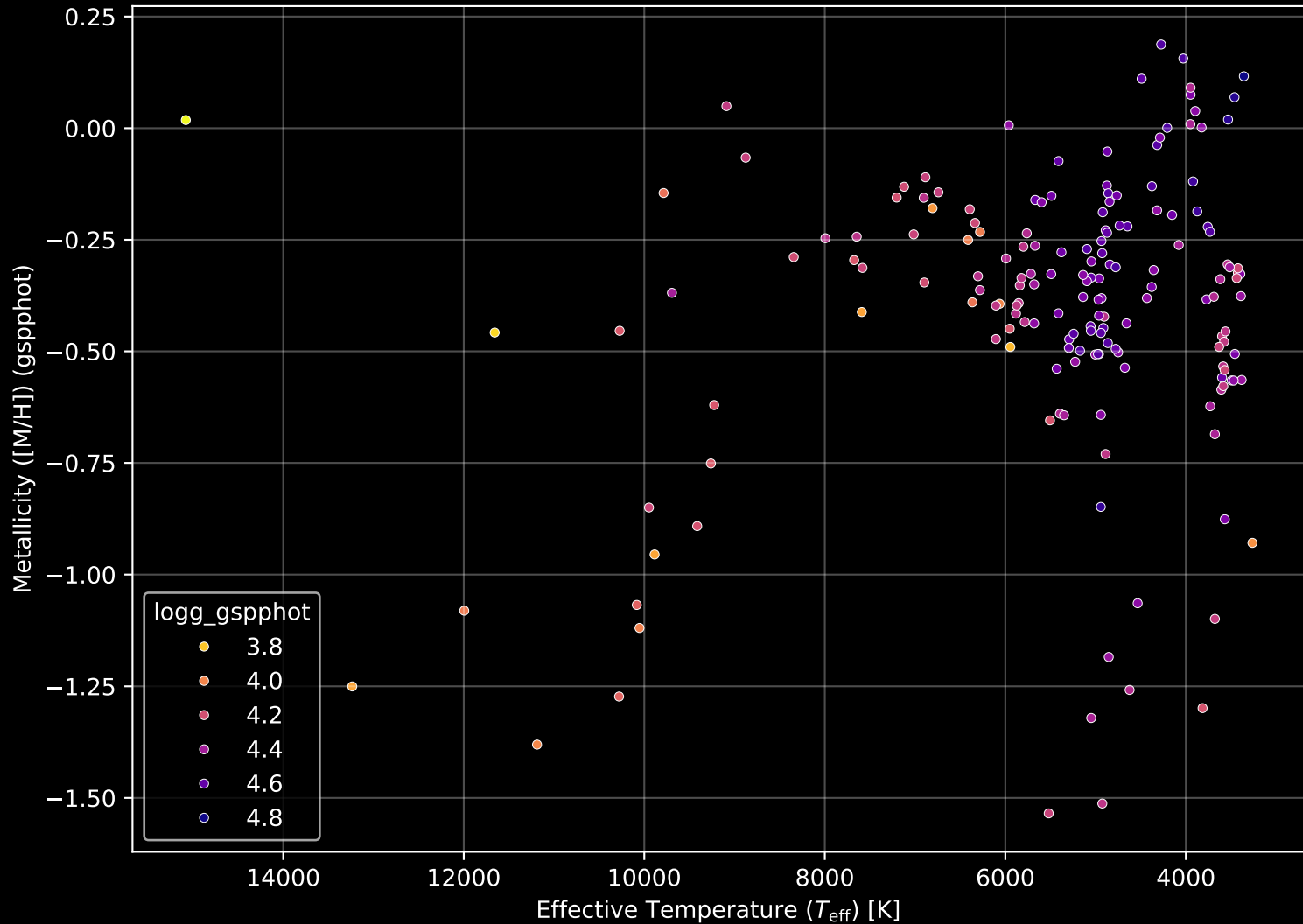
Gaia Cluster: [Alessi_21] Stellar Population Parameters (n= 174)
