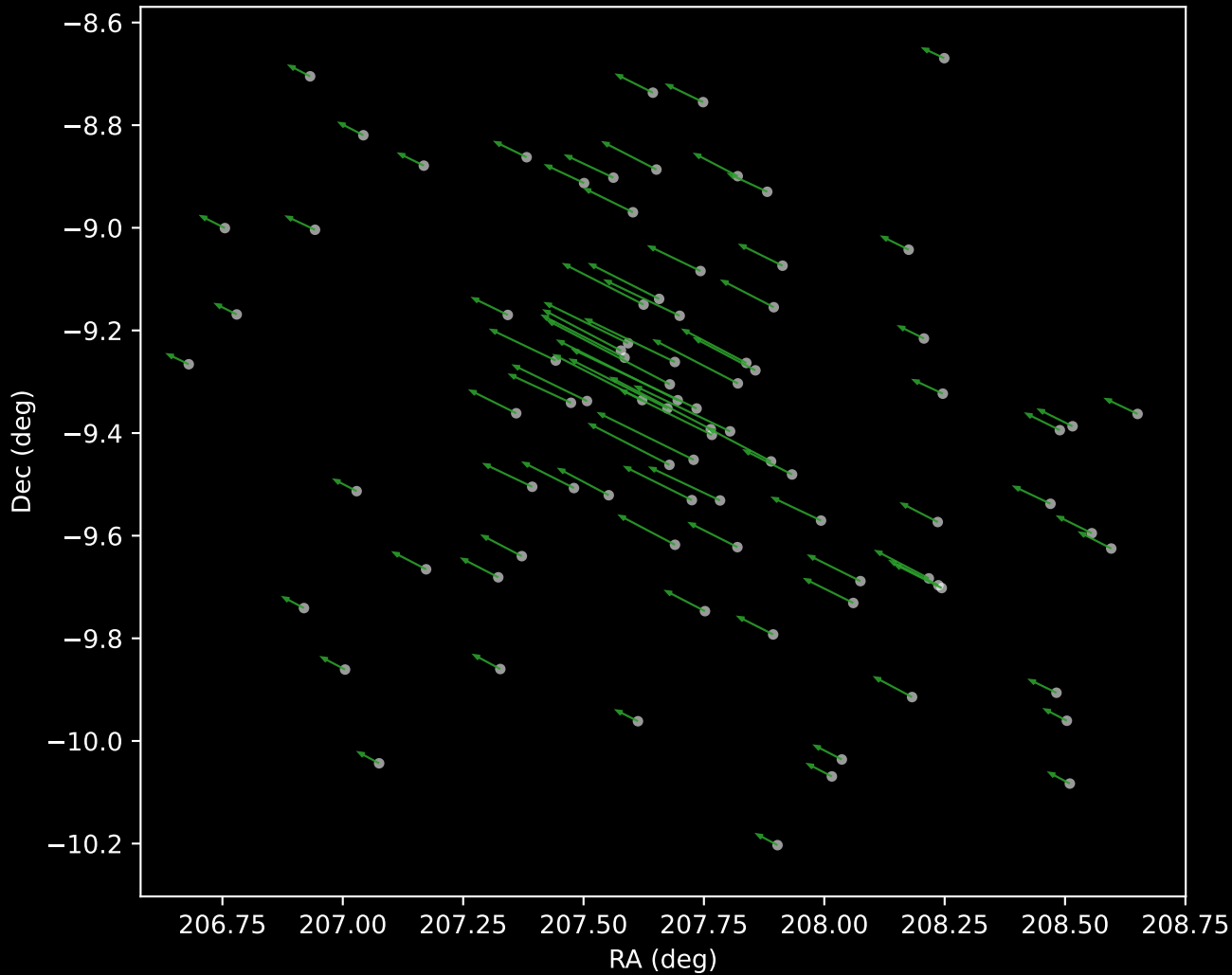
Gaia DR3 Cluster 4 Proper Motion Vectors (n=88)
