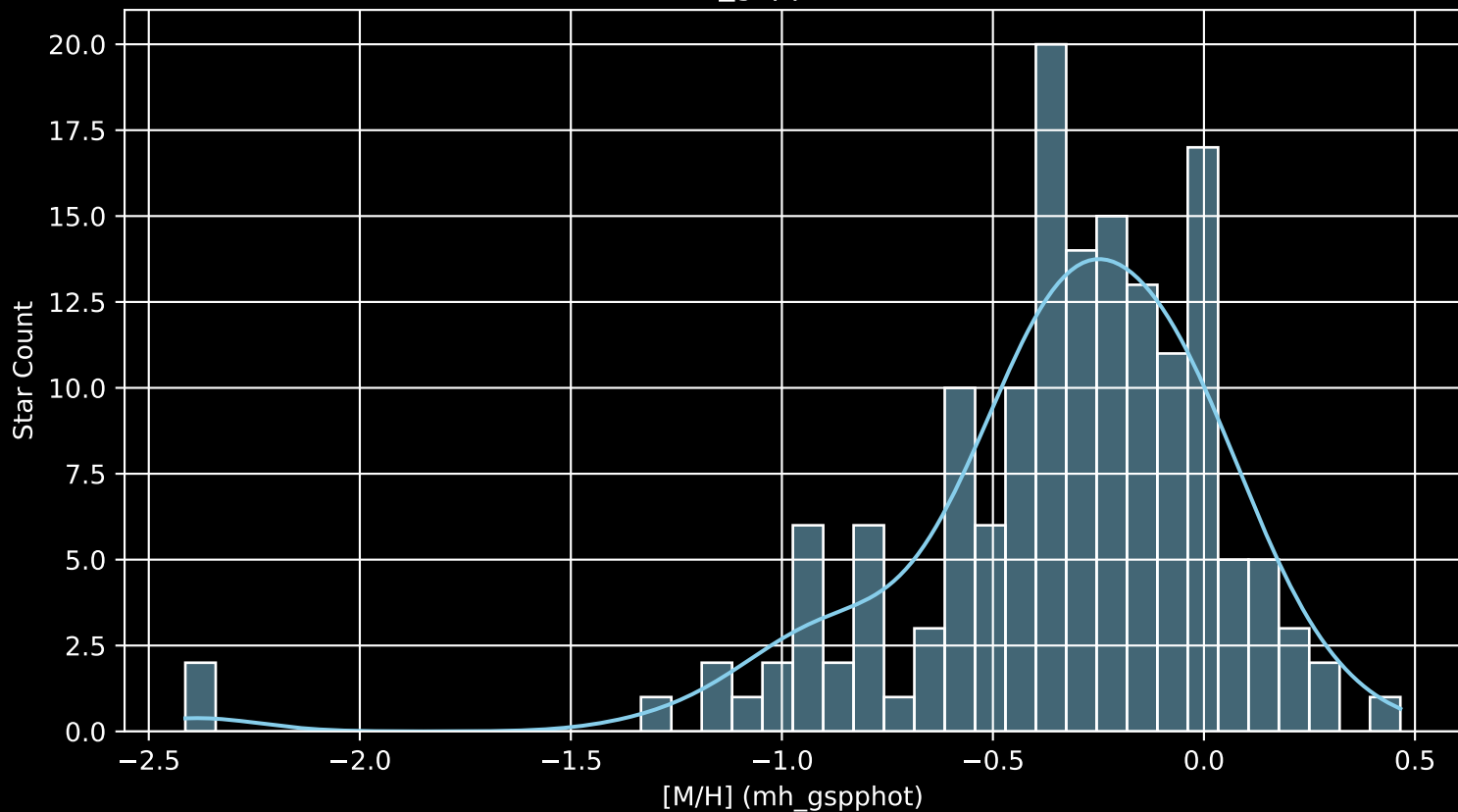
Gaia Cluster: [Alessi_37 [M/H] (mh_gspphot) (n= 158)
