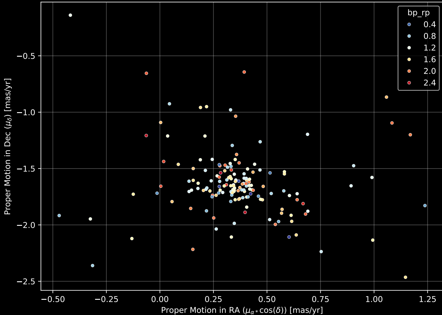
Gaia Cluster: [Alessi_37] Proper Motion Diagram (n= 158)
