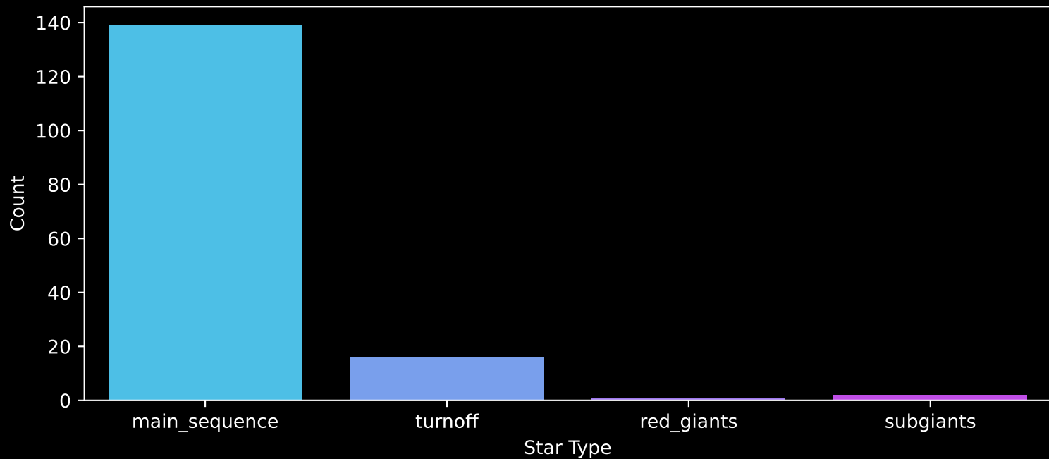
Gaia Cluster: [Alessi_37] Count plot of Star Type
