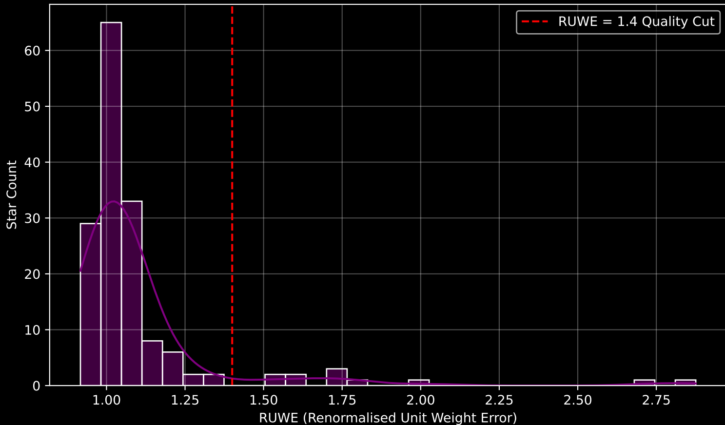
Gaia Cluster: [Alessi_37] RUWE Distribution (n= 156)
