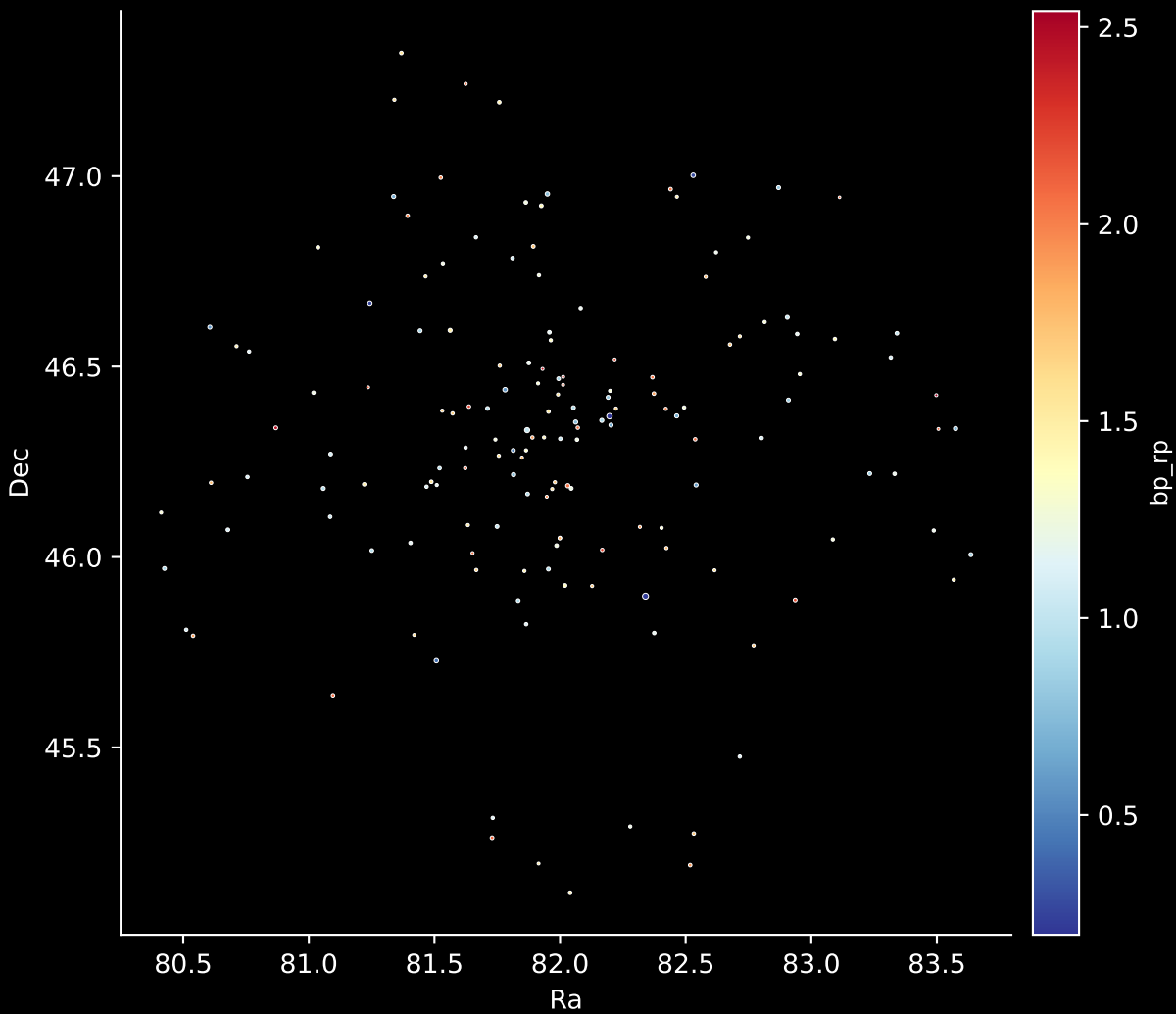
Gaia Cluster: [Alessi_37] Stars: 158
