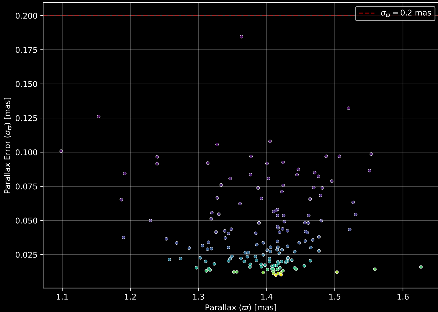
Gaia Cluster: [Alessi_37] Parallax Quality (n= 158)
