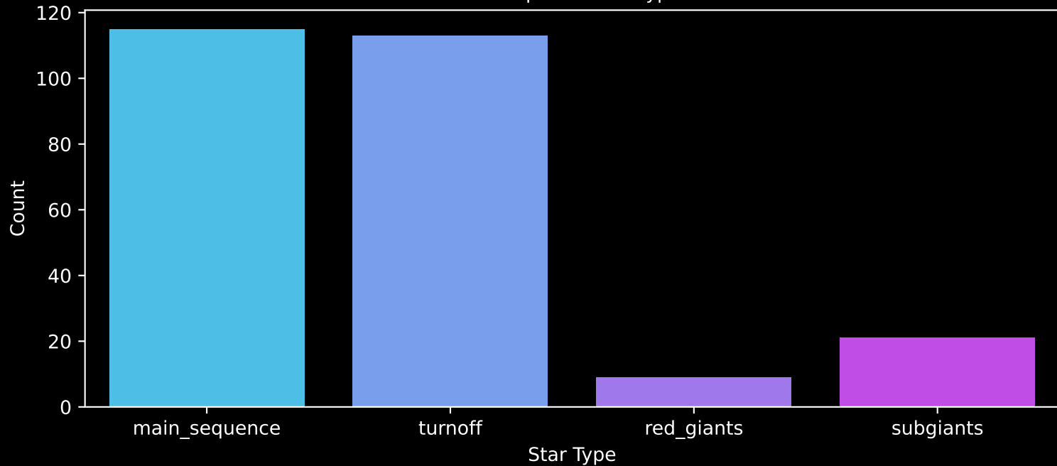
Gaia Cluster: [Alessi_43] Count plot of Star Type
