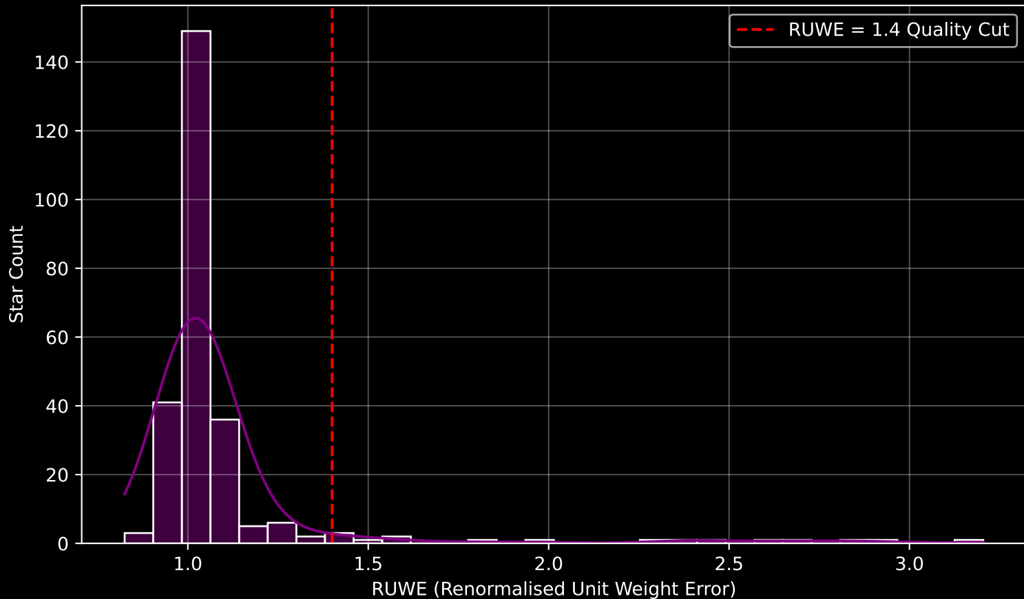
Gaia Cluster: [Alessi_43] RUWE Distribution (n= 258)
