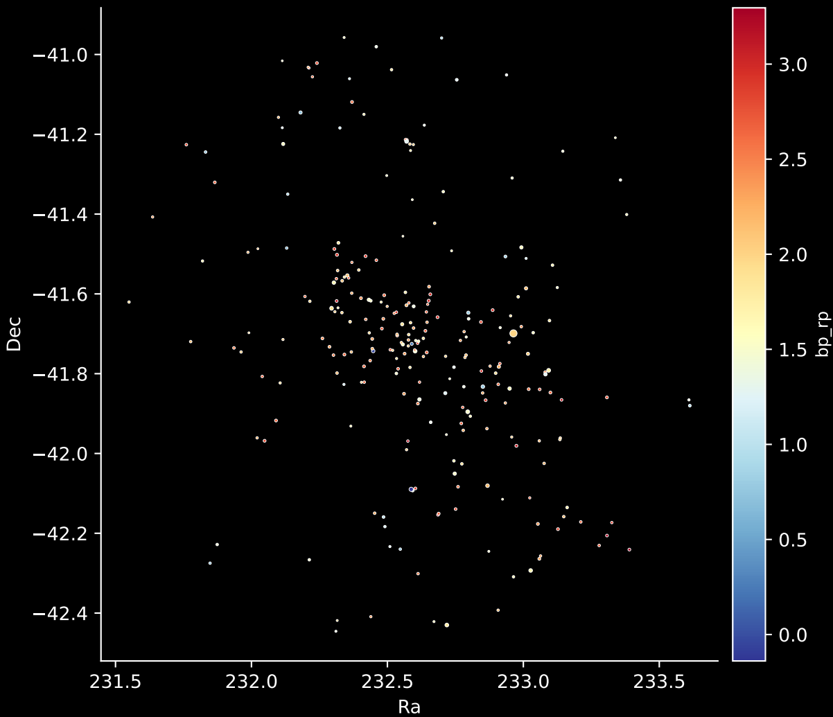
Gaia Cluster: [Alessi_43] Stars: 258
