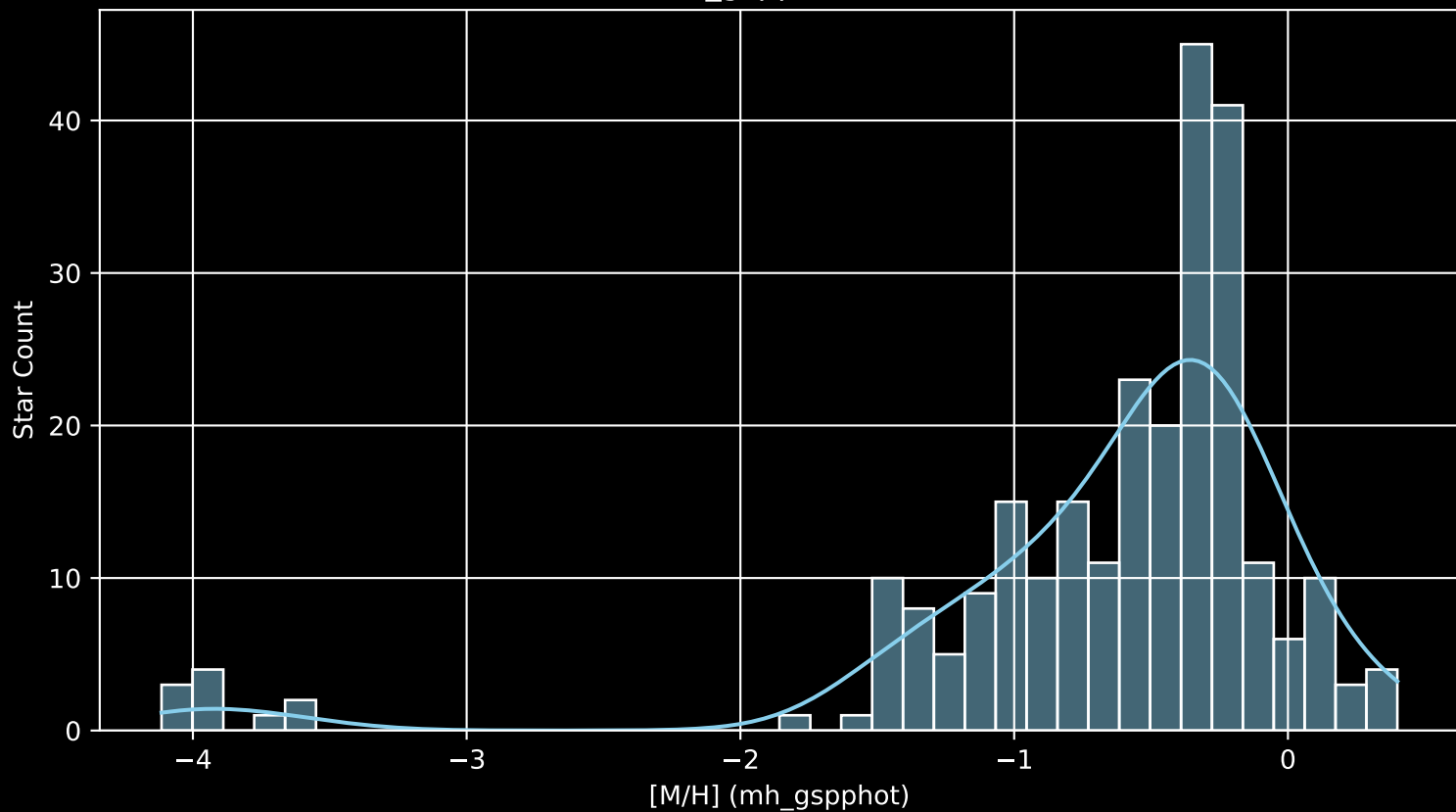
Gaia Cluster: [Alessi_43 [M/H] (mh_gspphot) (n= 258)
