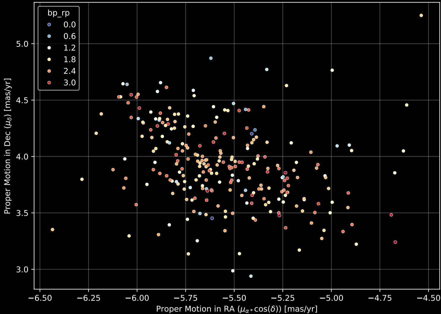
Gaia Cluster: [Alessi_43] Proper Motion Diagram (n= 258)
