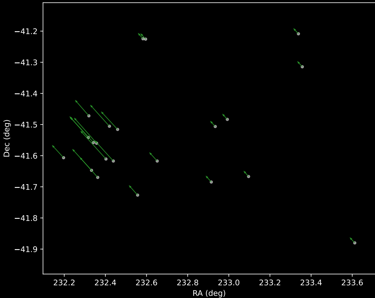
Gaia DR3 Cluster 4 Proper Motion Vectors (n=22)
