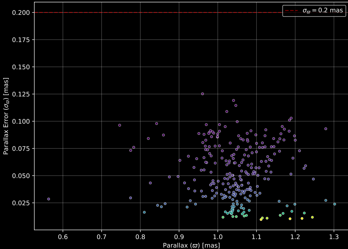
Gaia Cluster: [Alessi_43] Parallax Quality (n= 258)
