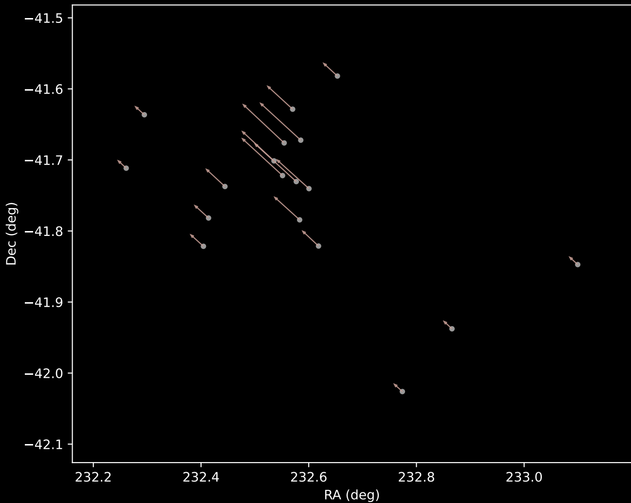
Gaia DR3 Cluster 11 Proper Motion Vectors (n=18)
