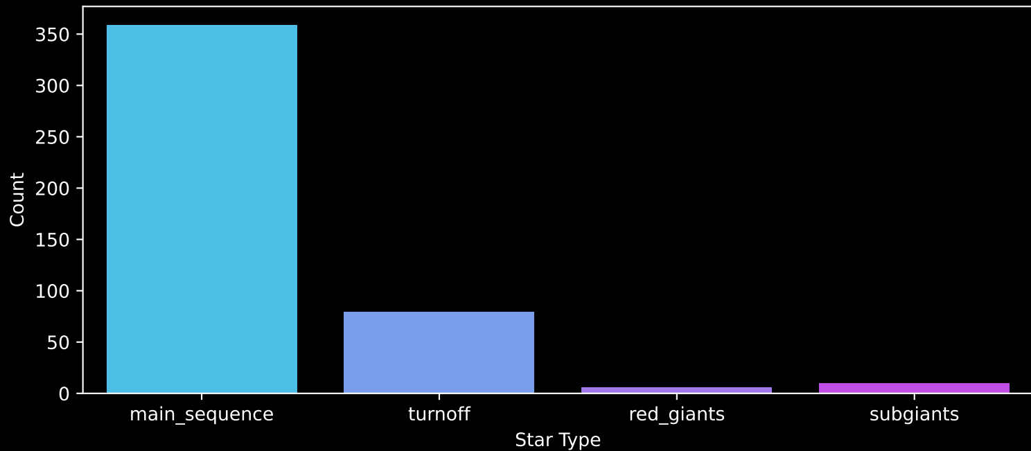
Gaia Cluster: [Alessi_44] Count plot of Star Type
