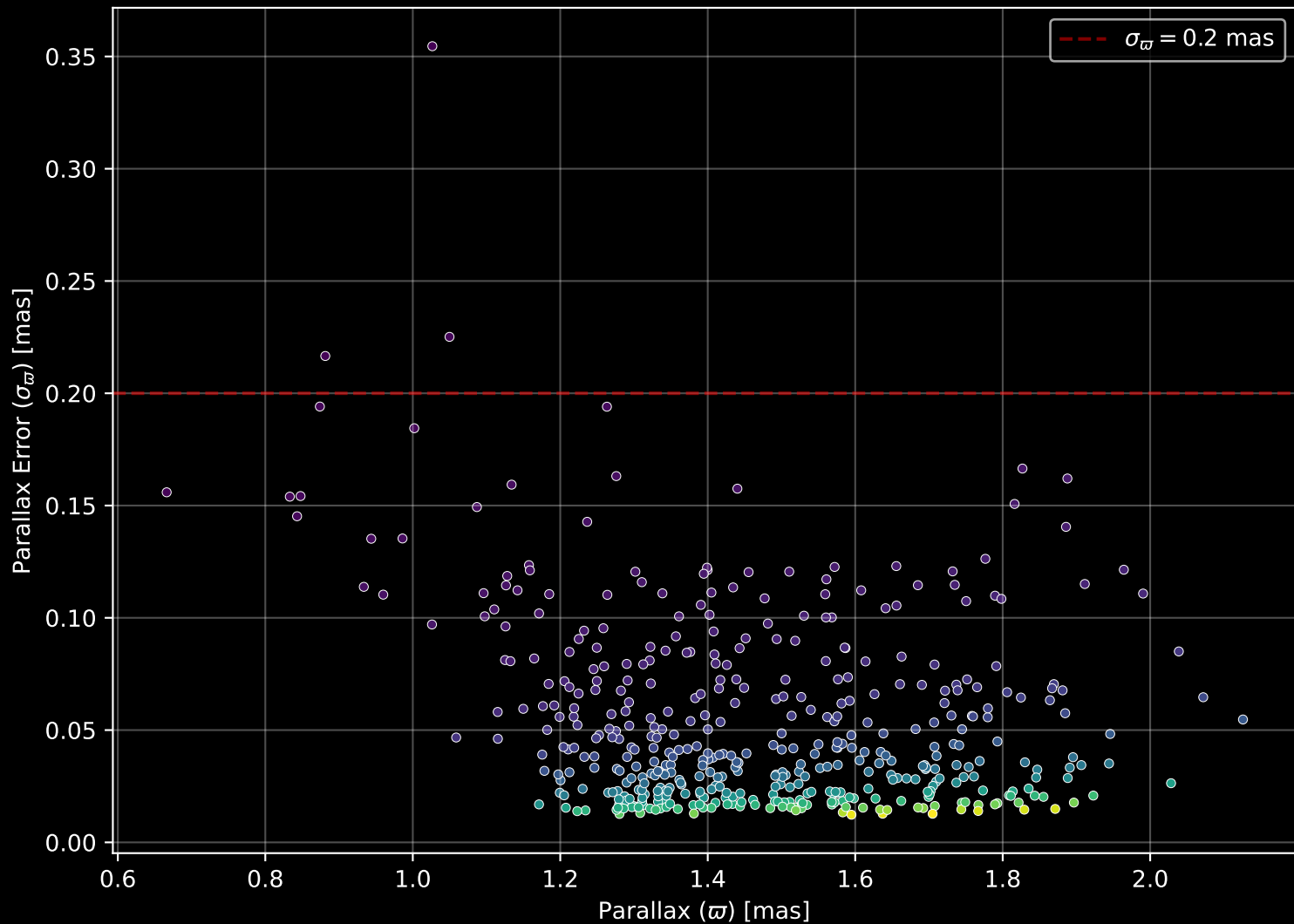
Gaia Cluster: [Alessi_44] Parallax Quality (n= 454)
