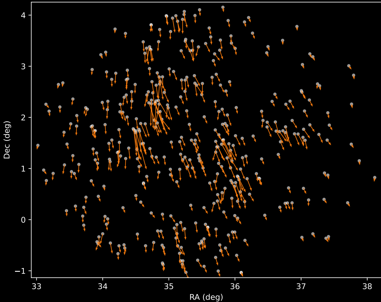
Gaia DR3 Cluster 2 Proper Motion Vectors (n=395)
