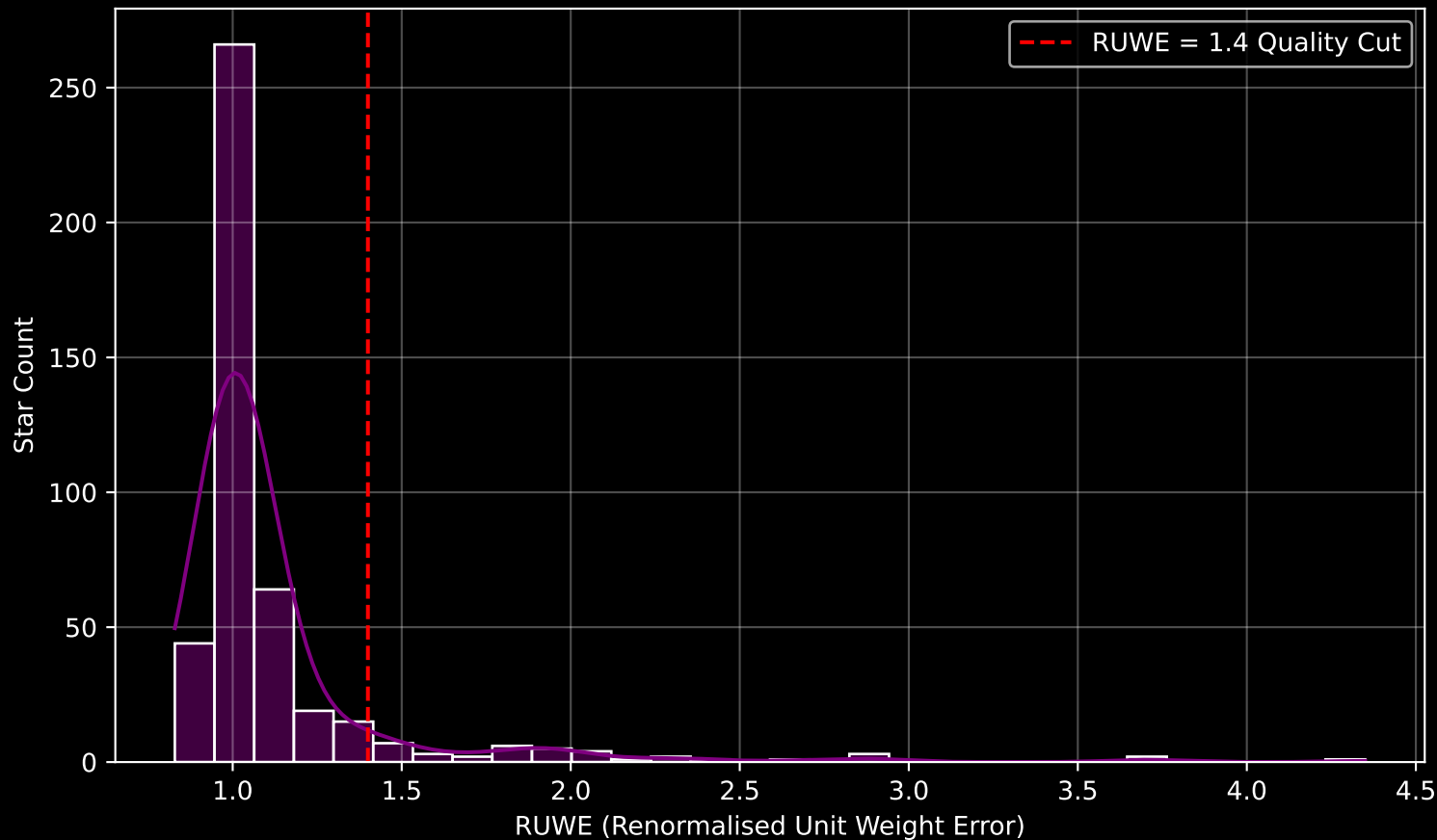
Gaia Cluster: [Alessi_44] RUWE Distribution (n= 446)
