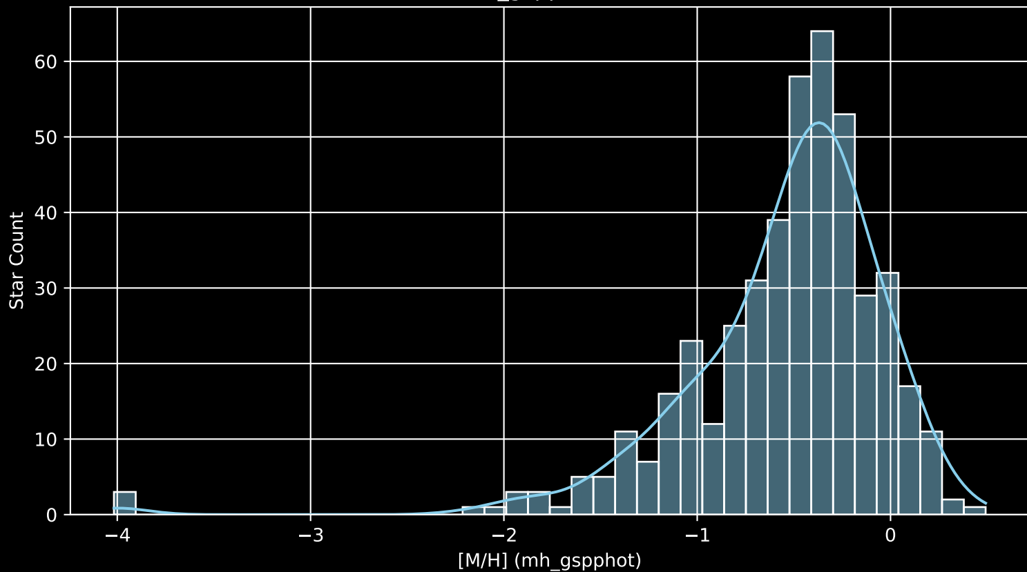
Gaia Cluster: [Alessi_44 [M/H] (mh_gspphot) (n= 453)
