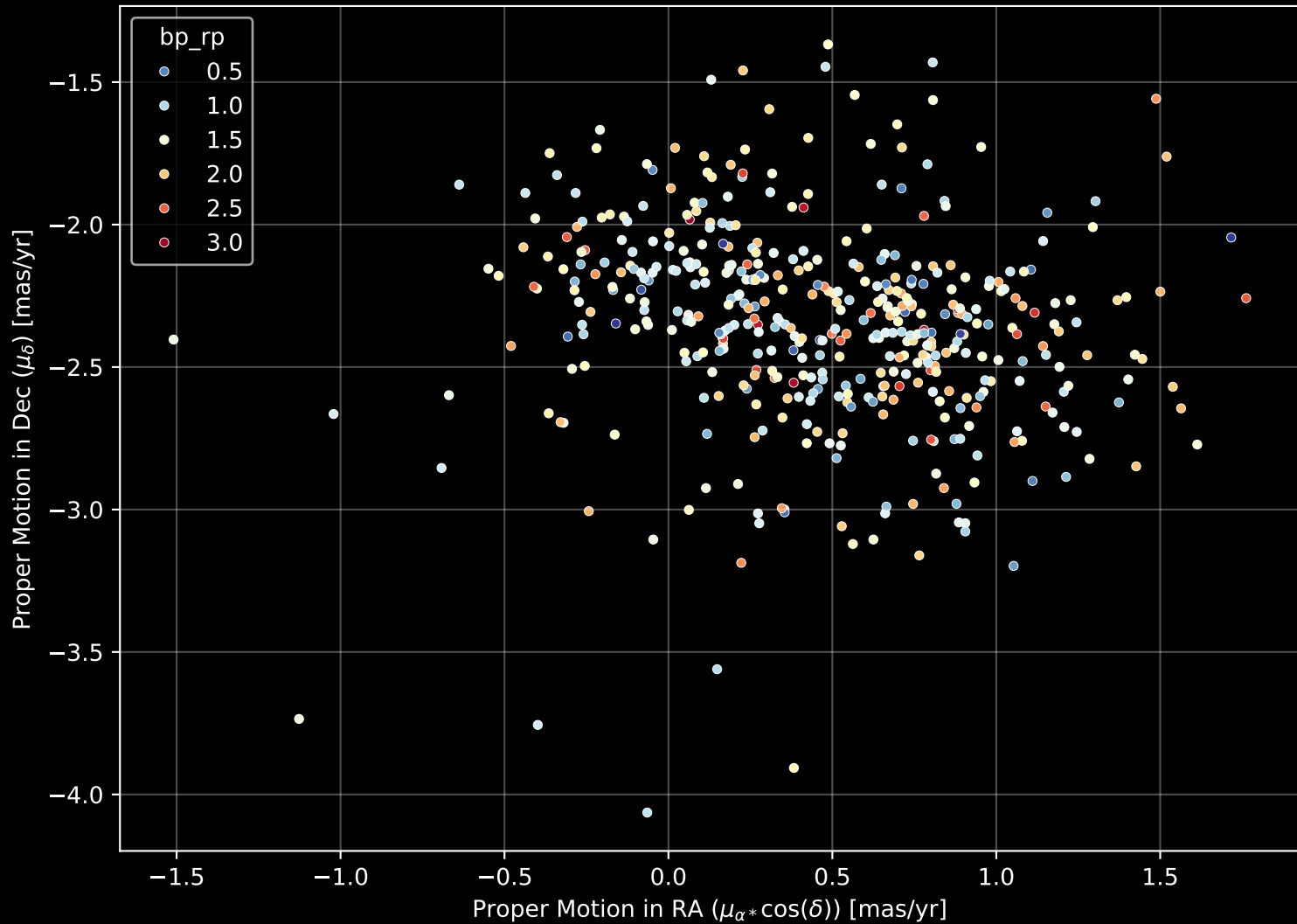
Gaia Cluster: [Alessi_44] Proper Motion Diagram (n= 454)
