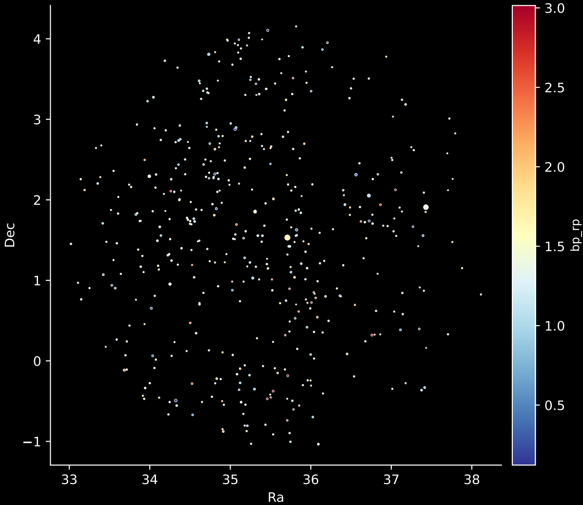
Gaia Cluster: [Alessi_44] Stars: 454
