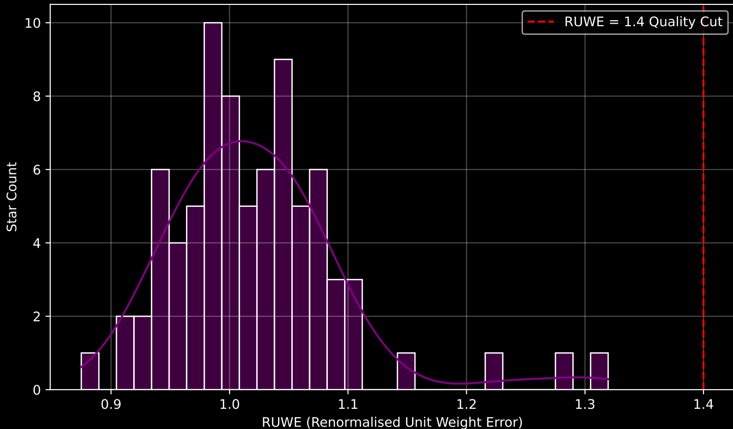
Gaia Cluster: [Alessi_53] RUWE Distribution (n= 79)
