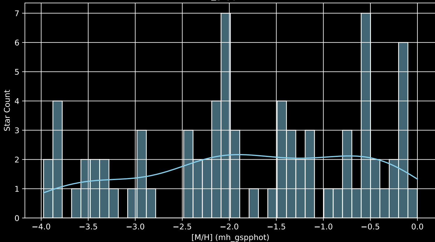
Gaia Cluster: [Alessi_53 [M/H] (mh_gspphot) (n= 79)
