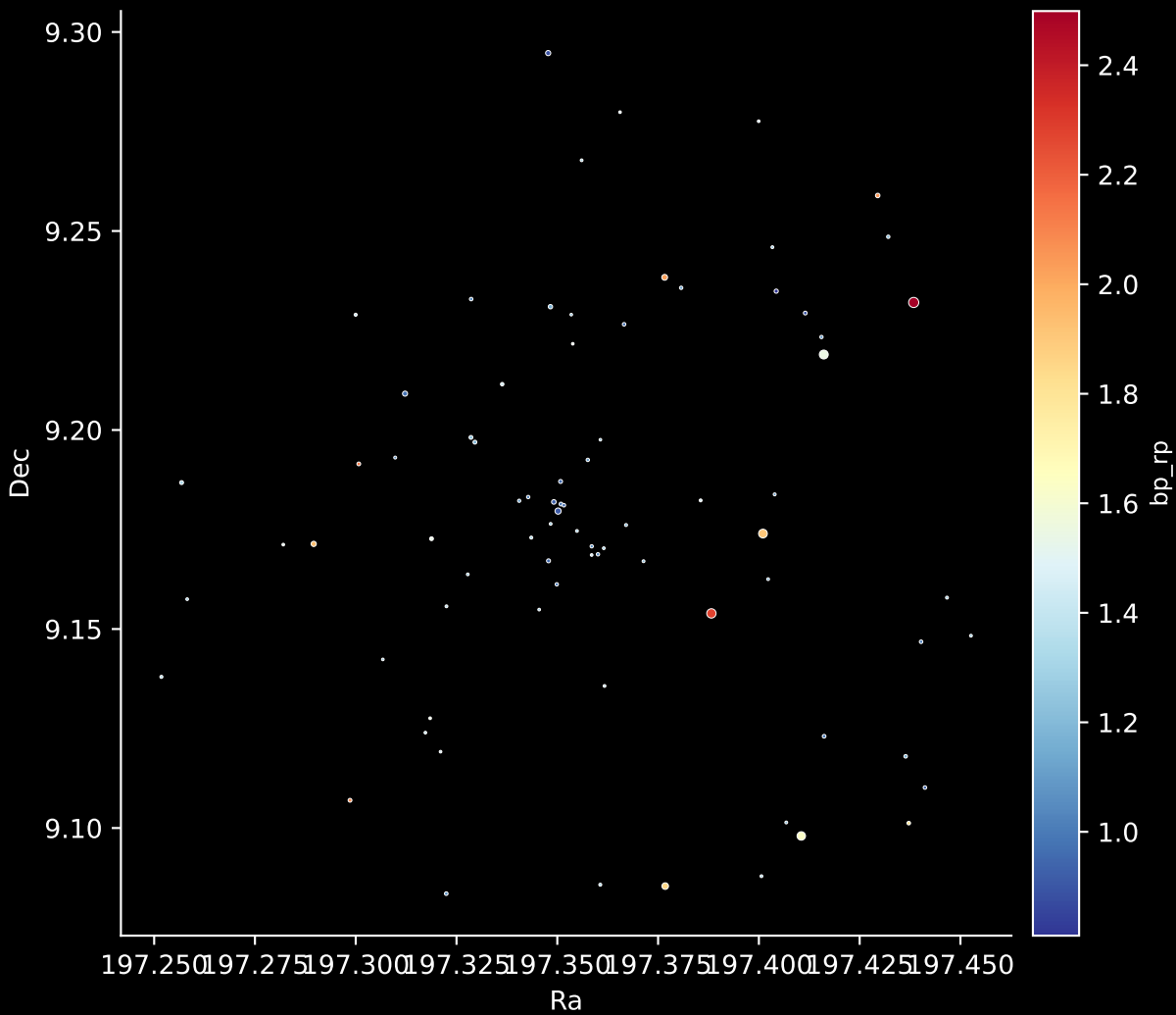
Gaia Cluster: [Alessi_53] Stars: 79
