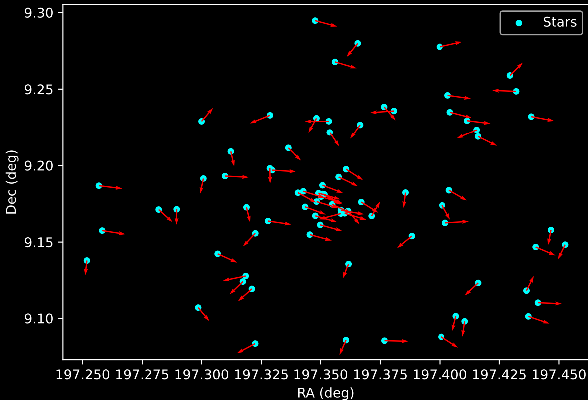
Gaia Cluster: [Alessi_53] Proper Motion Vectors for Gaia Star Field (n= 79)
