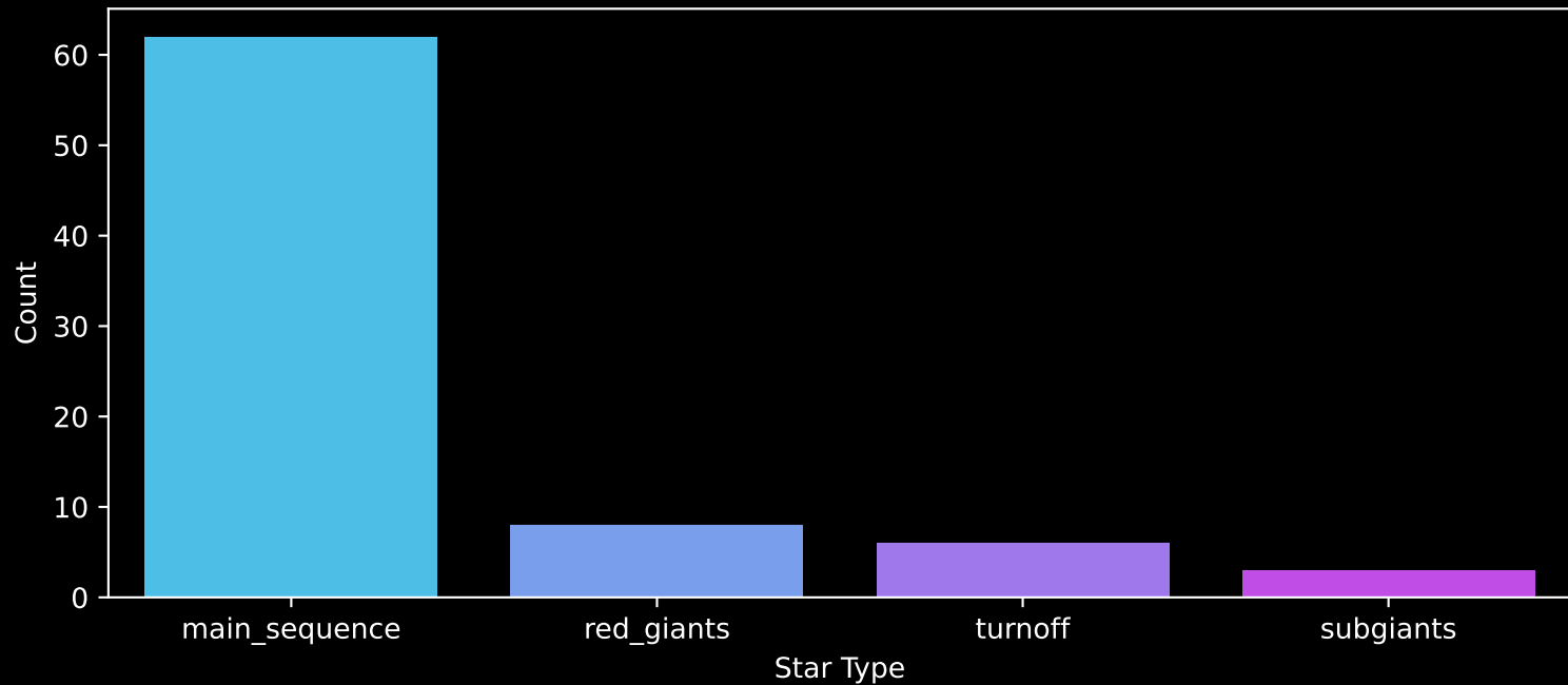
Gaia Cluster: [Alessi_53] Count plot of Star Type
