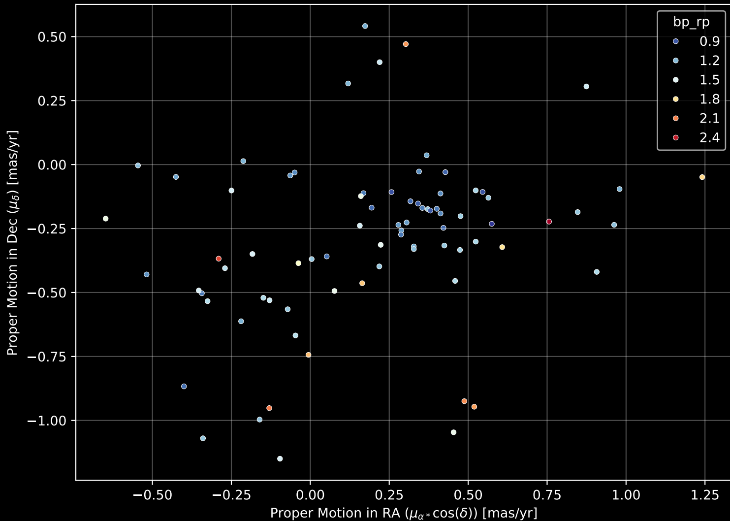
Gaia Cluster: [Alessi_53] Proper Motion Diagram (n= 79)
