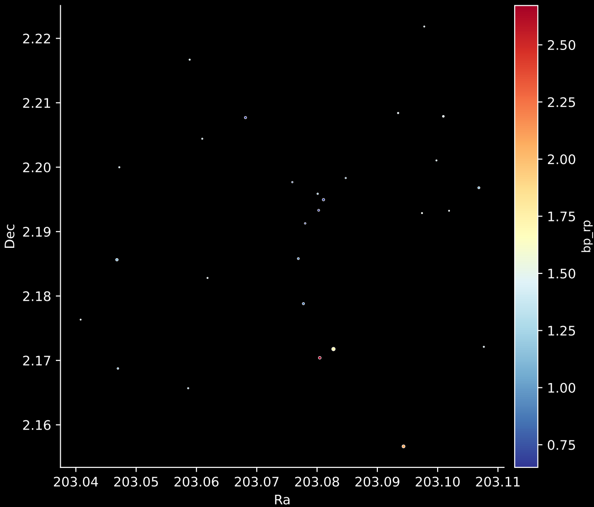
Gaia Cluster: [Alessi_59] Stars: 28
