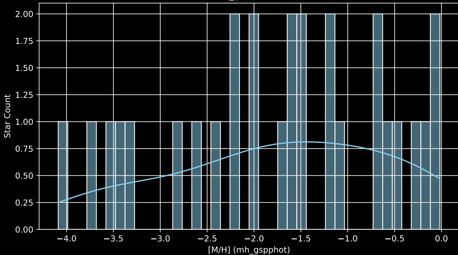
Gaia Cluster: [Alessi_59 [M/H] (mh_gspphot) (n= 28)
