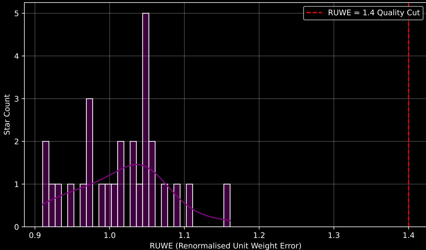
Gaia Cluster: [Alessi_59] RUWE Distribution (n= 28)
