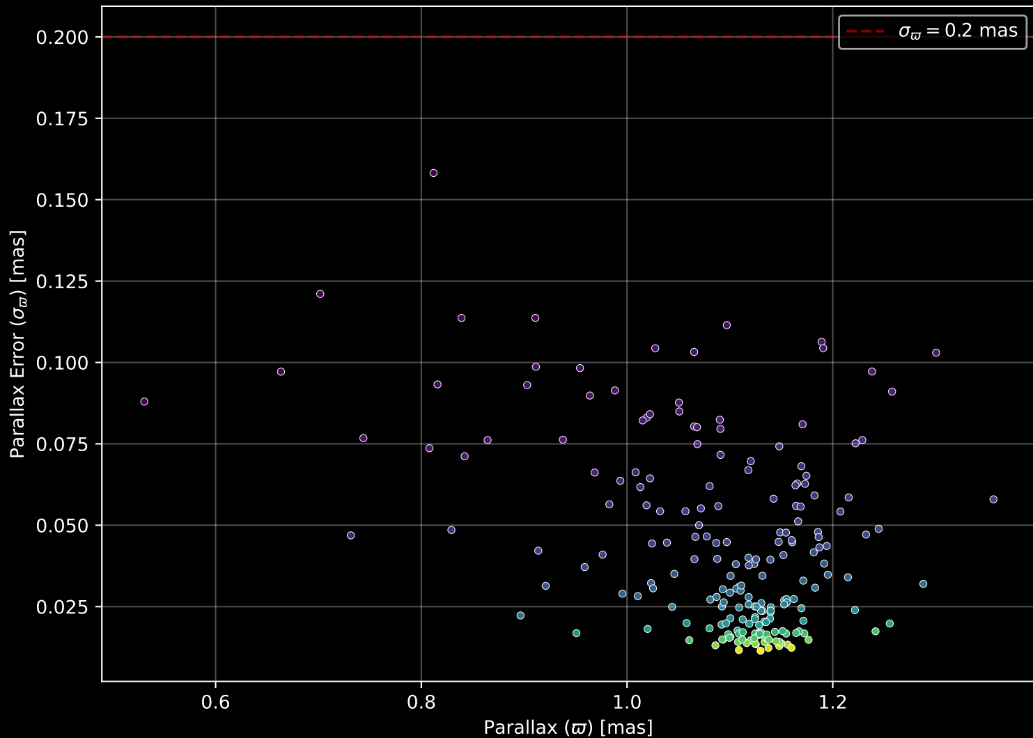
Gaia Cluster: [Alessi_6] Parallax Quality (n= 207)
