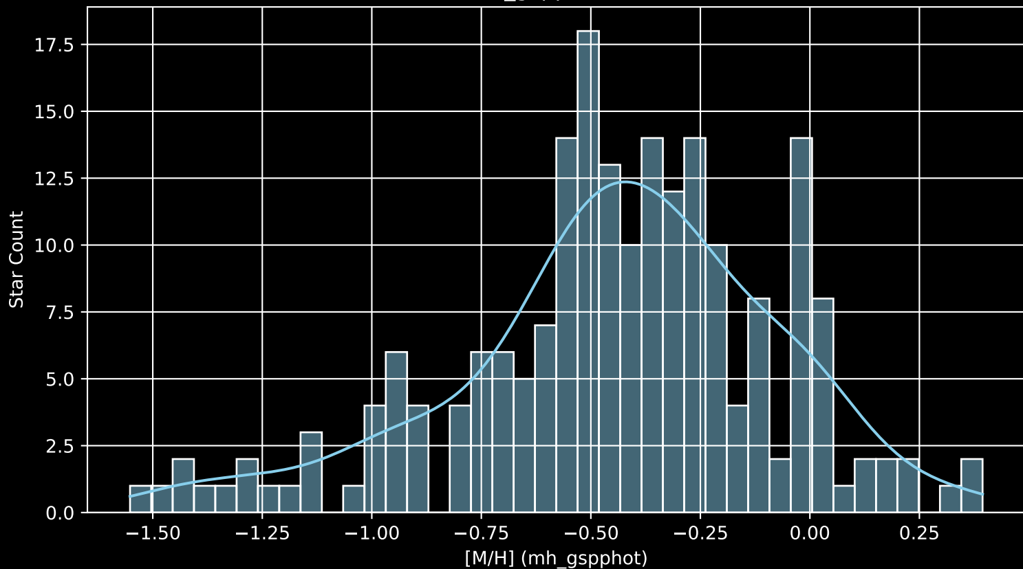
Gaia Cluster: [Alessi_6 [M/H] (mh_gspphot) (n= 207)
