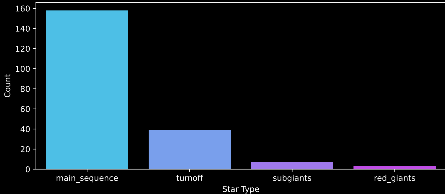
Gaia Cluster: [Alessi_6] Count plot of Star Type
