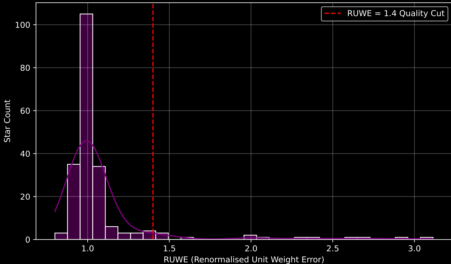
Gaia Cluster: [Alessi_6] RUWE Distribution (n= 206)
