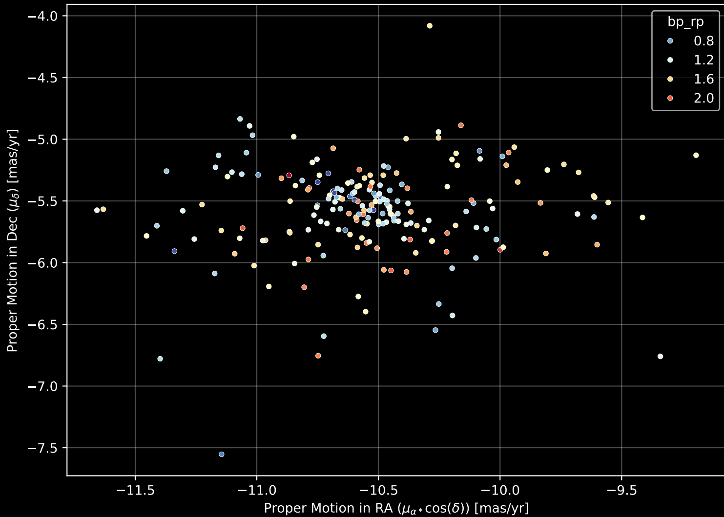
Gaia Cluster: [Alessi_6] Proper Motion Diagram (n= 207)
