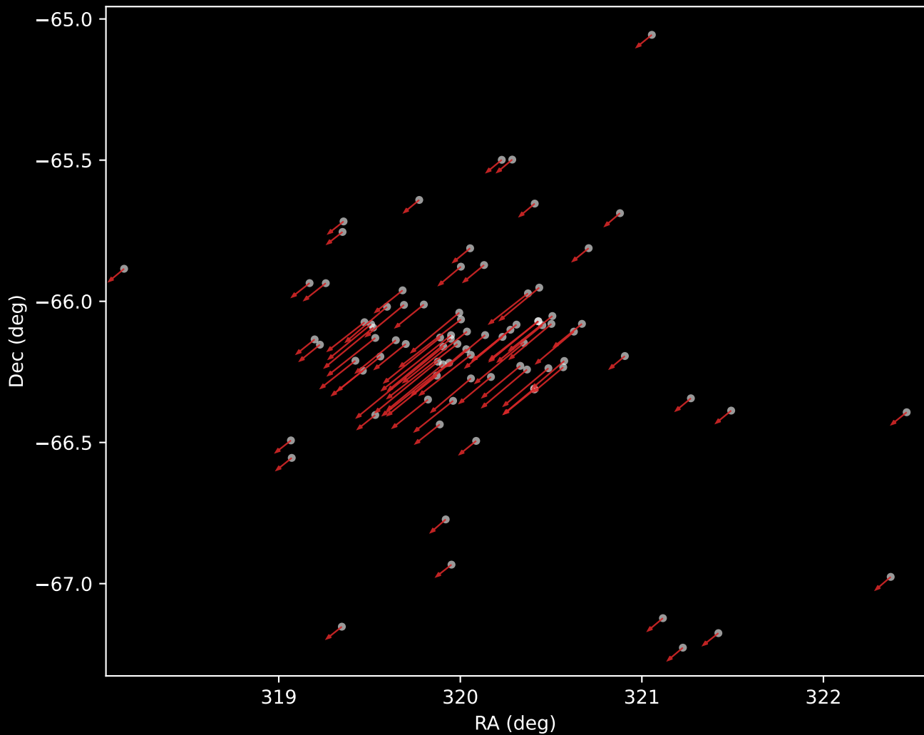
Gaia DR3 Cluster 6 Proper Motion Vectors (n=85)
