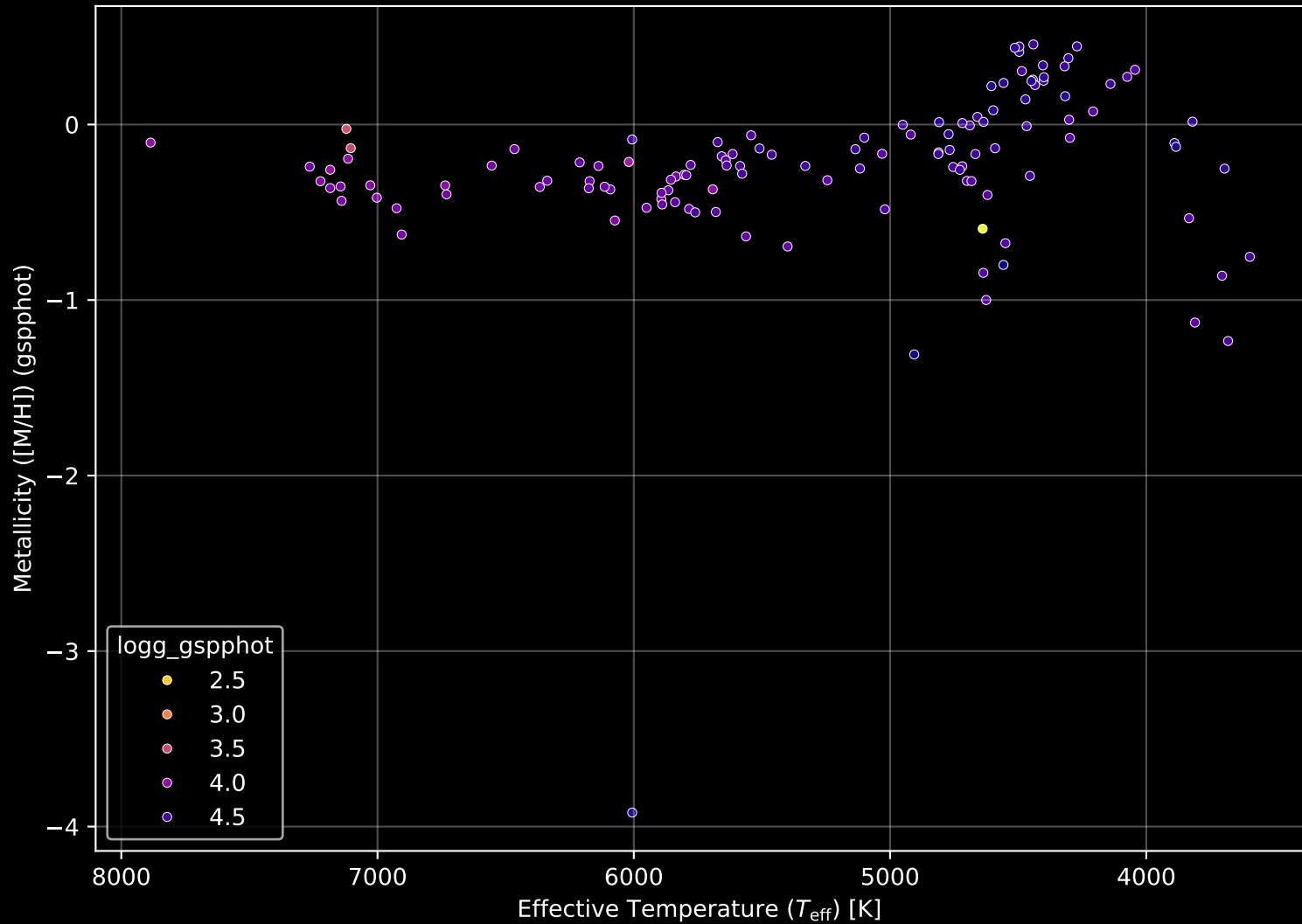
Gaia Cluster: [Alessi_62] Stellar Population Parameters (n= 125)
