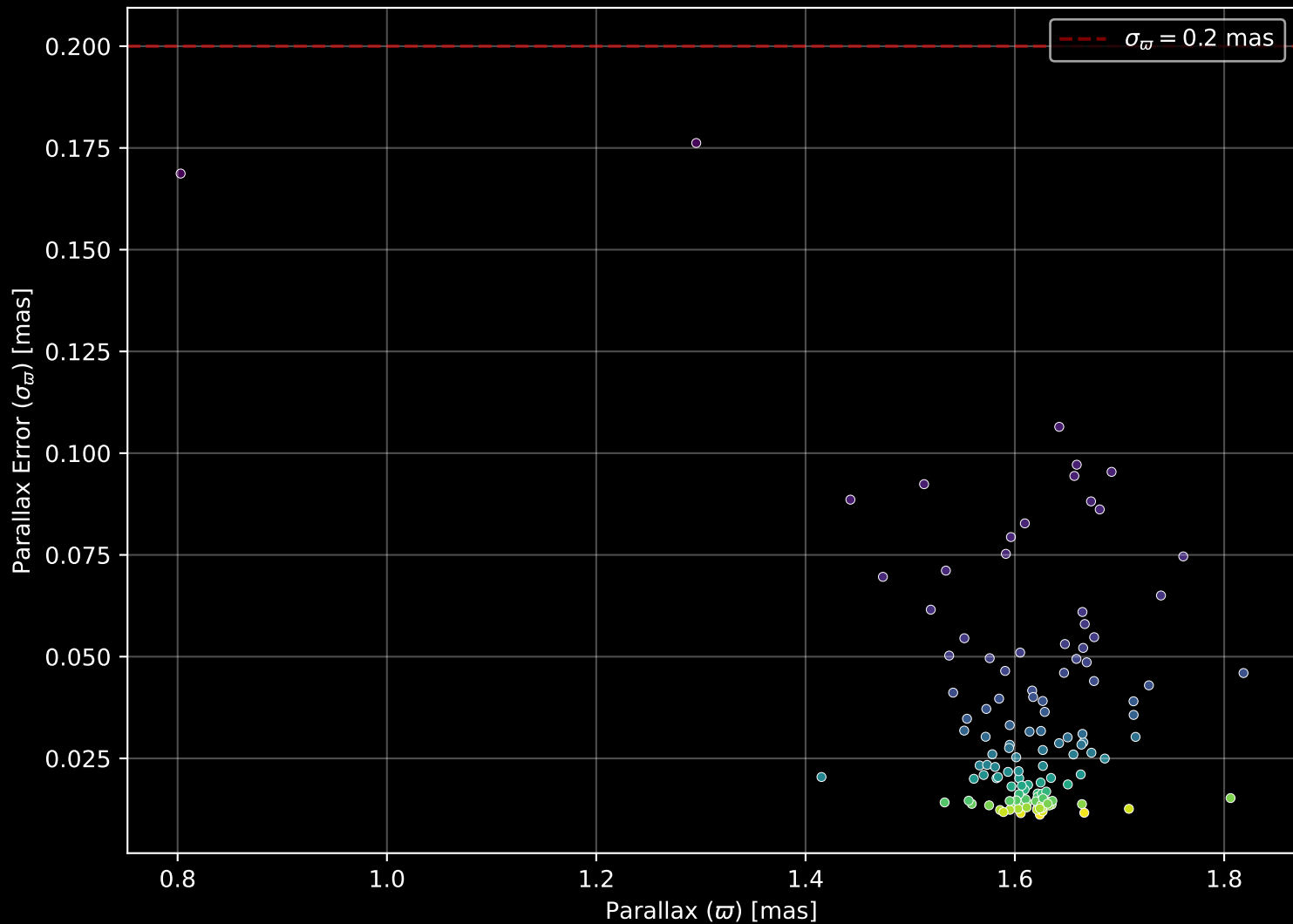
Gaia Cluster: [Alessi_62] Parallax Quality (n= 125)
