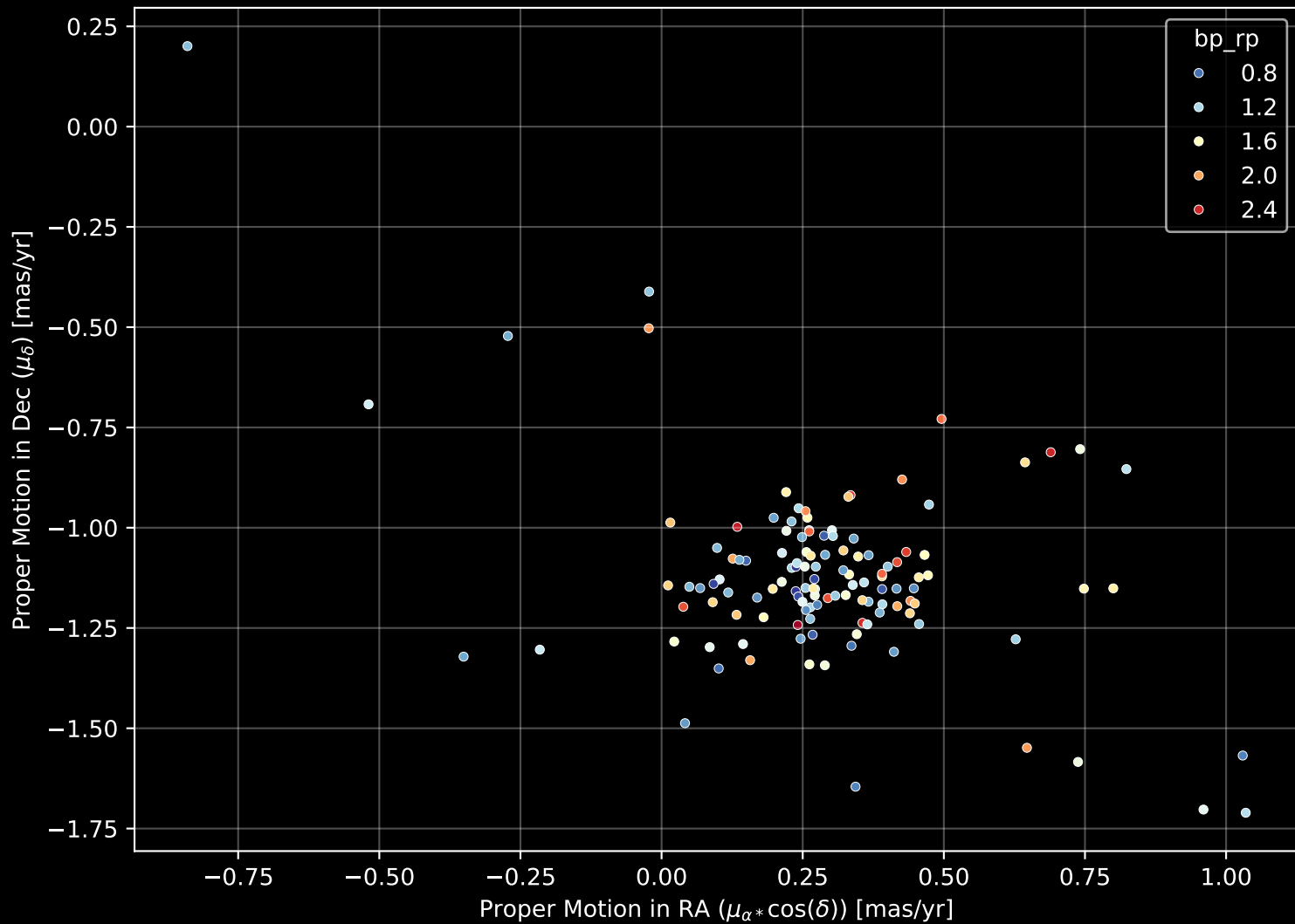
Gaia Cluster: [Alessi_62] Proper Motion Diagram (n= 125)
