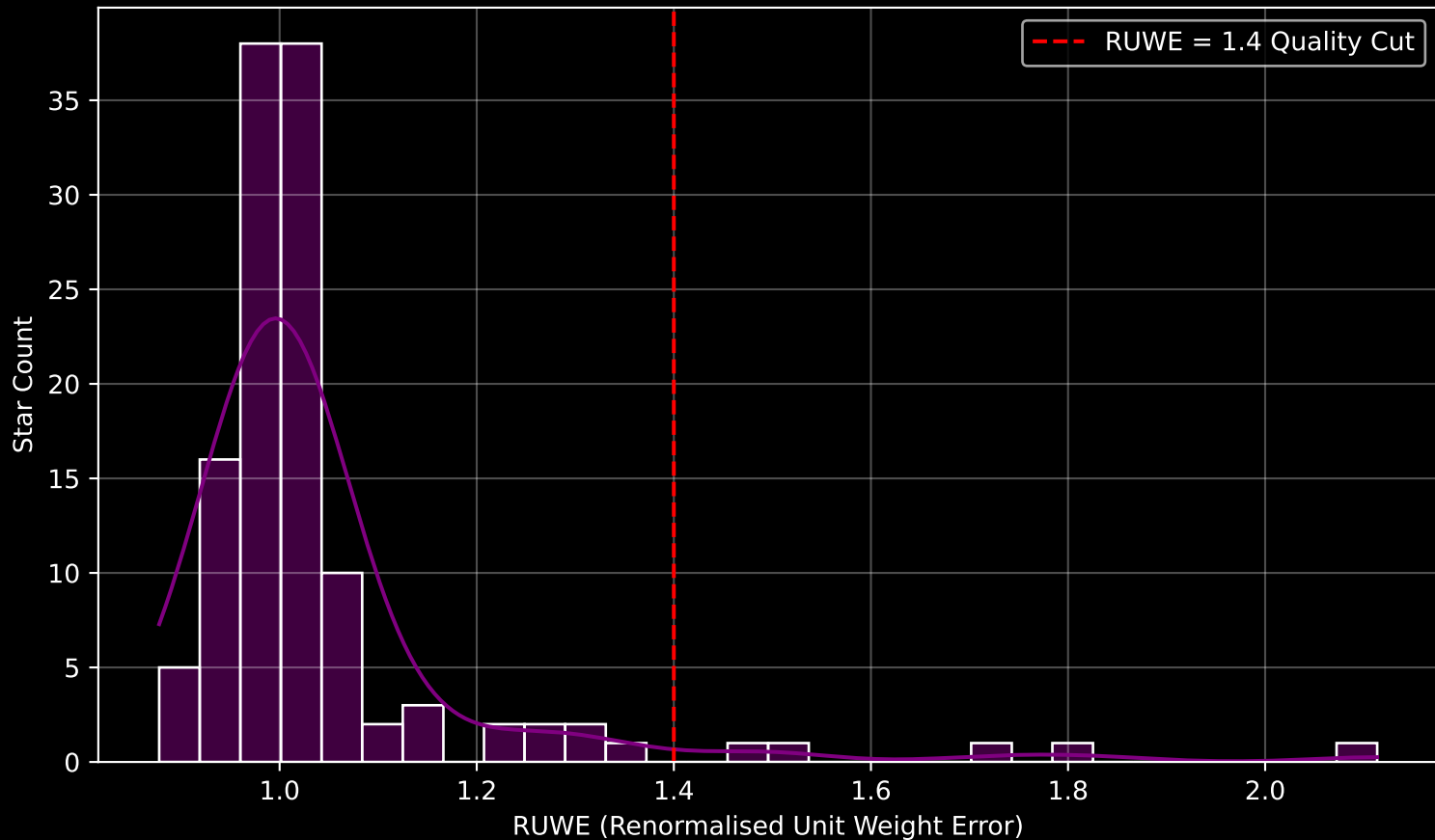
Gaia Cluster: [Alessi_62] RUWE Distribution (n= 124)
