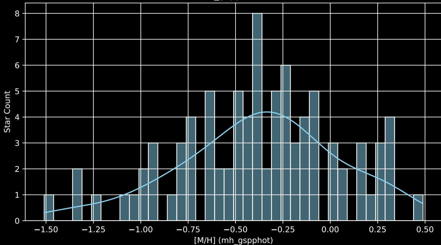
Gaia Cluster: [Alessi_Teutsch_12 [M/H] (mh_gspphot) (n= 87)
