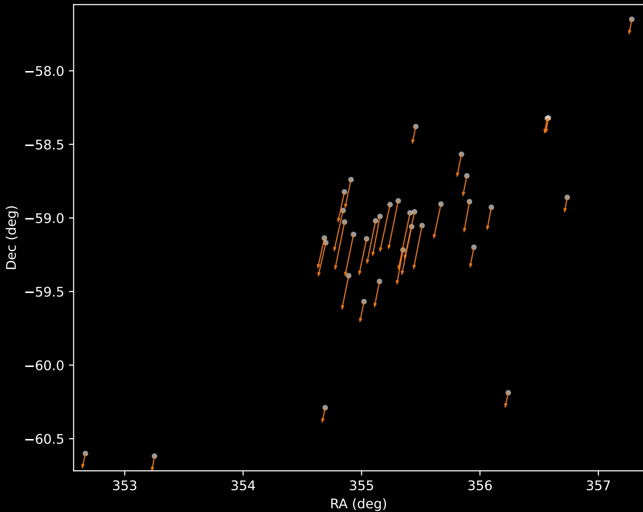
Gaia DR3 Cluster 2 Proper Motion Vectors (n=35)
