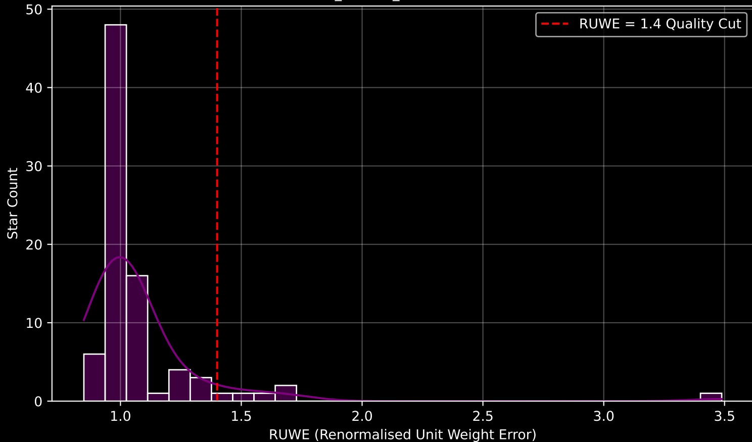
Gaia Cluster: [Alessi_Teutsch_12] RUWE Distribution (n= 84)
