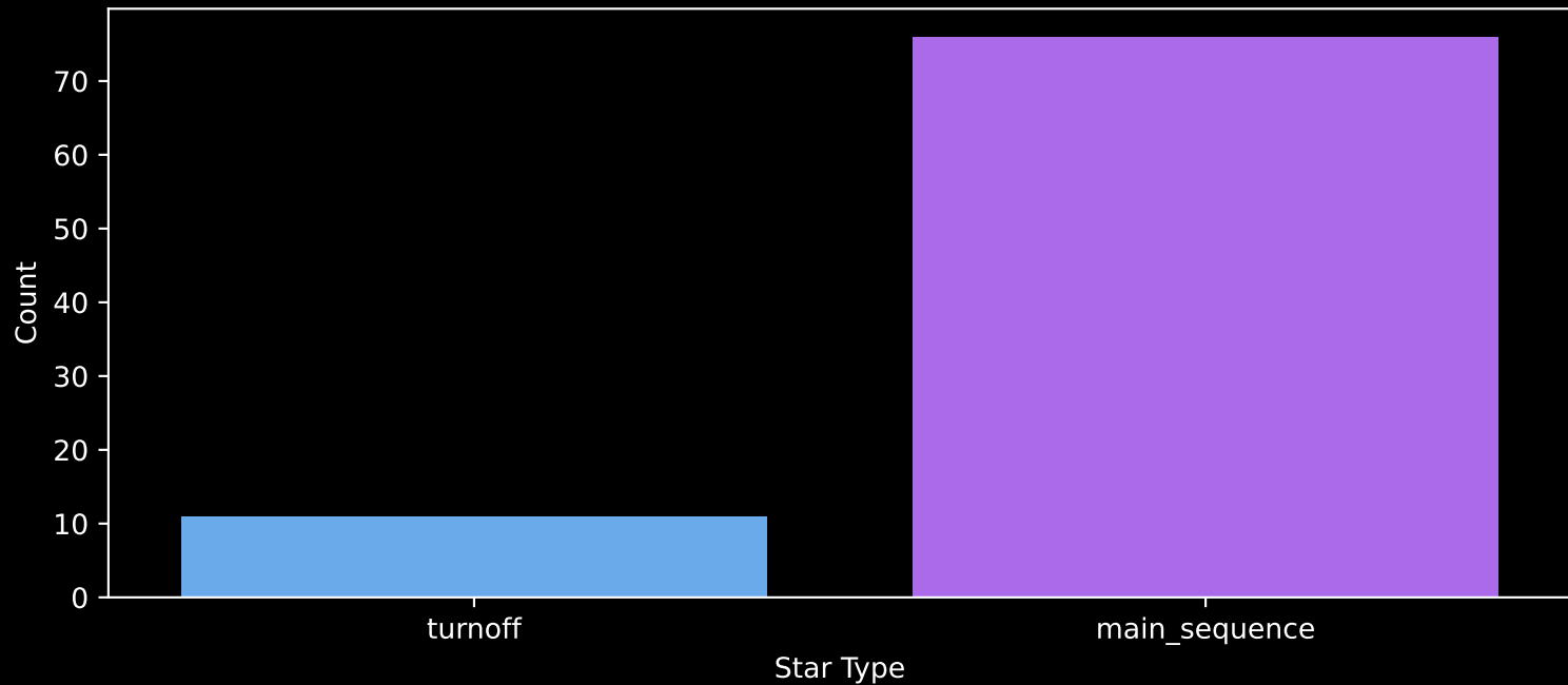
Gaia Cluster: [Alessi_Teutsch_12] Count plot of Star Type
