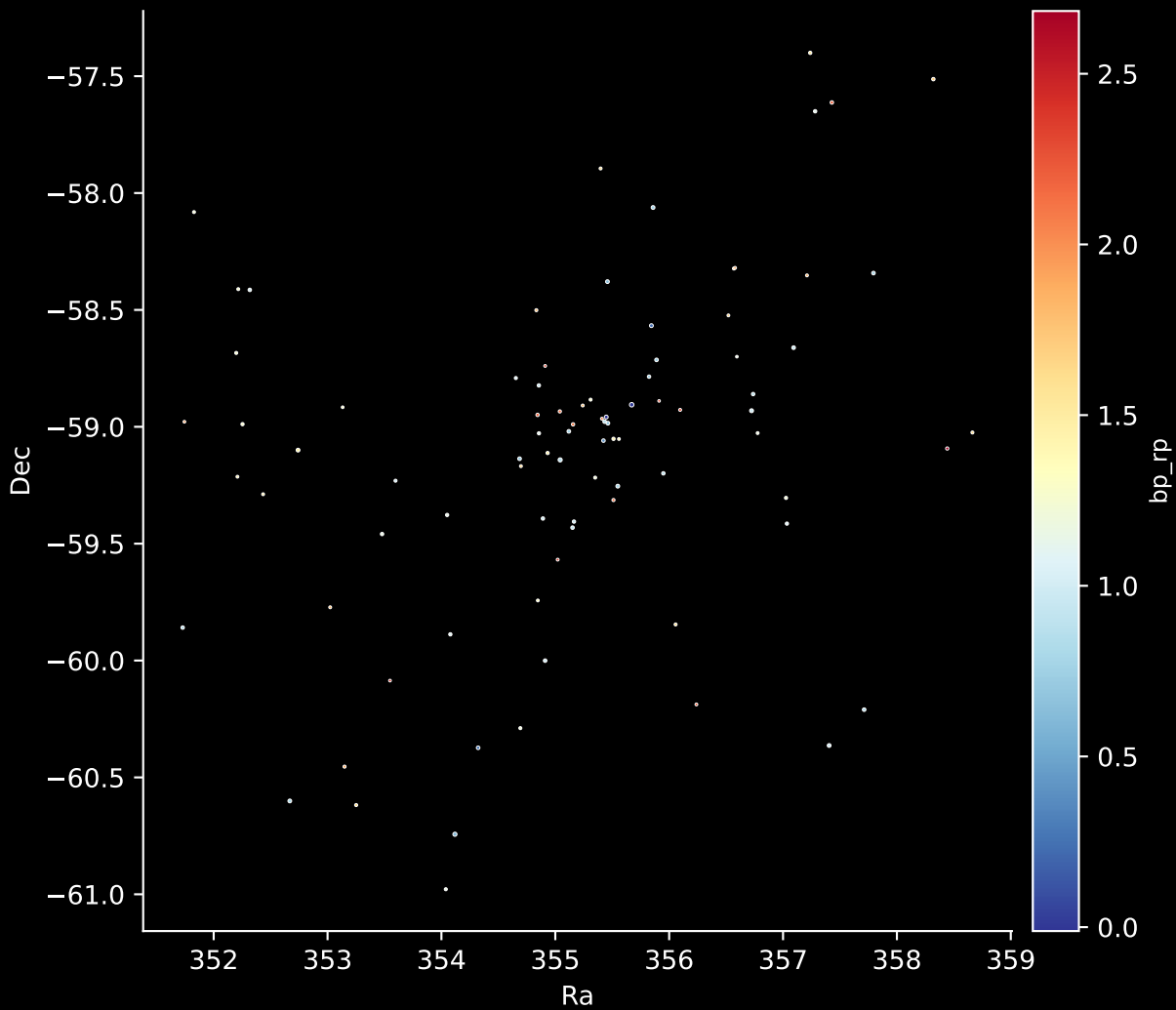
Gaia Cluster: [Alessi_Teutsch_12] Stars: 87
