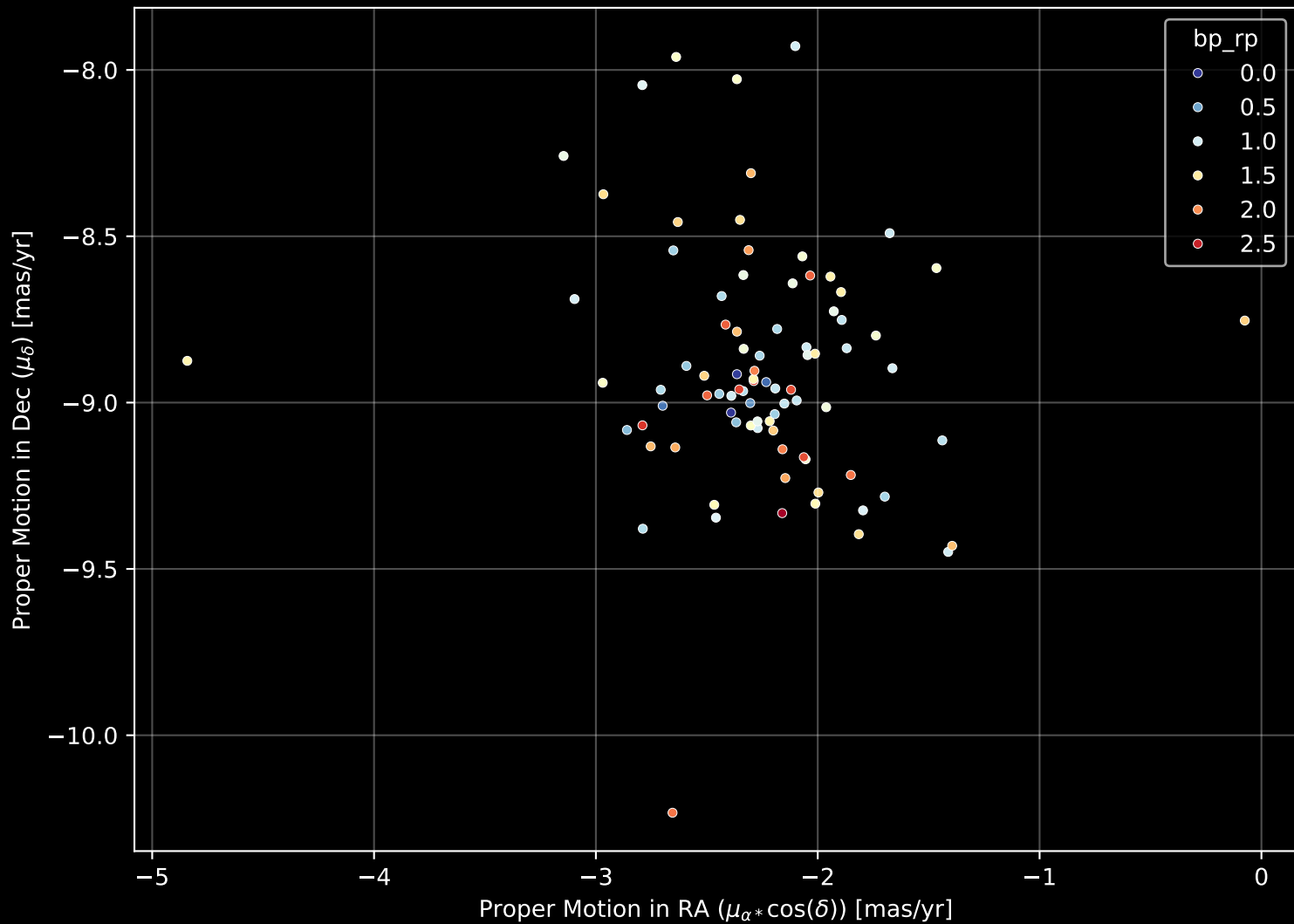
Gaia Cluster: [Alessi_Teutsch_12] Proper Motion Diagram (n= 87)
