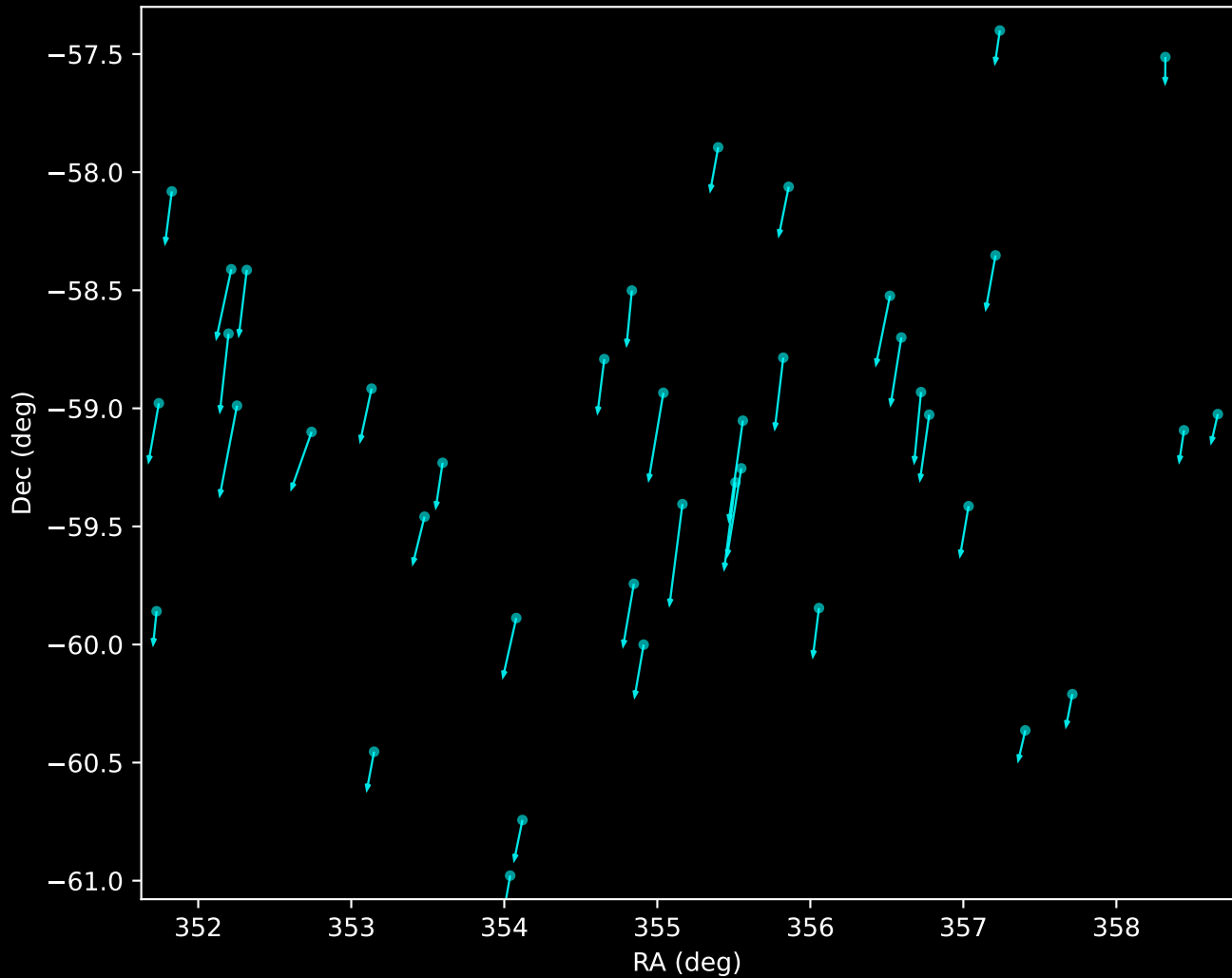
Gaia DR3 Noise Stream Proper Motion Vectors (n=40)
