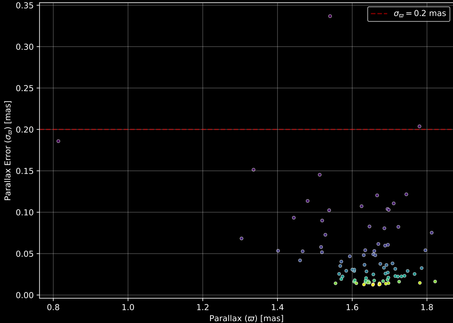
Gaia Cluster: [Alessi_Teutsch_12] Parallax Quality (n= 87)
