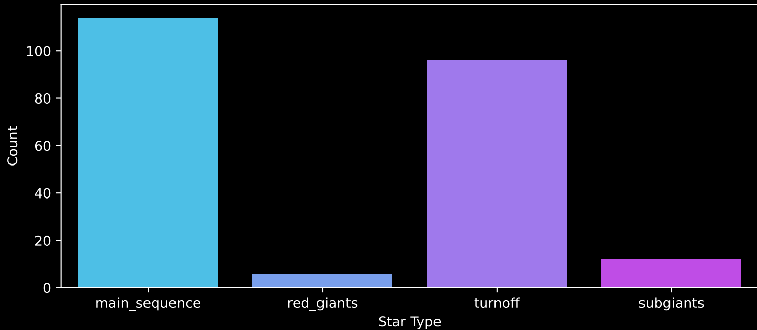
Gaia Cluster: [Alessi_Teutsch_5] Count plot of Star Type
