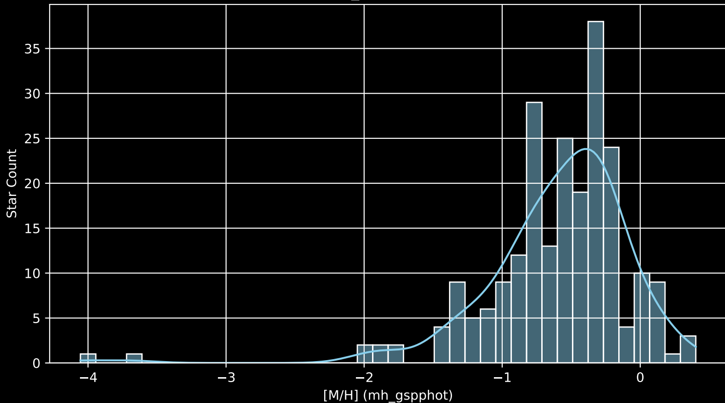
Gaia Cluster: [Alessi_Teutsch_5 [M/H] (mh_gspphot) (n= 228)
