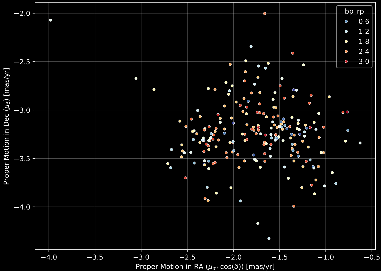
Gaia Cluster: [Alessi_Teutsch_5] Proper Motion Diagram (n= 228)
