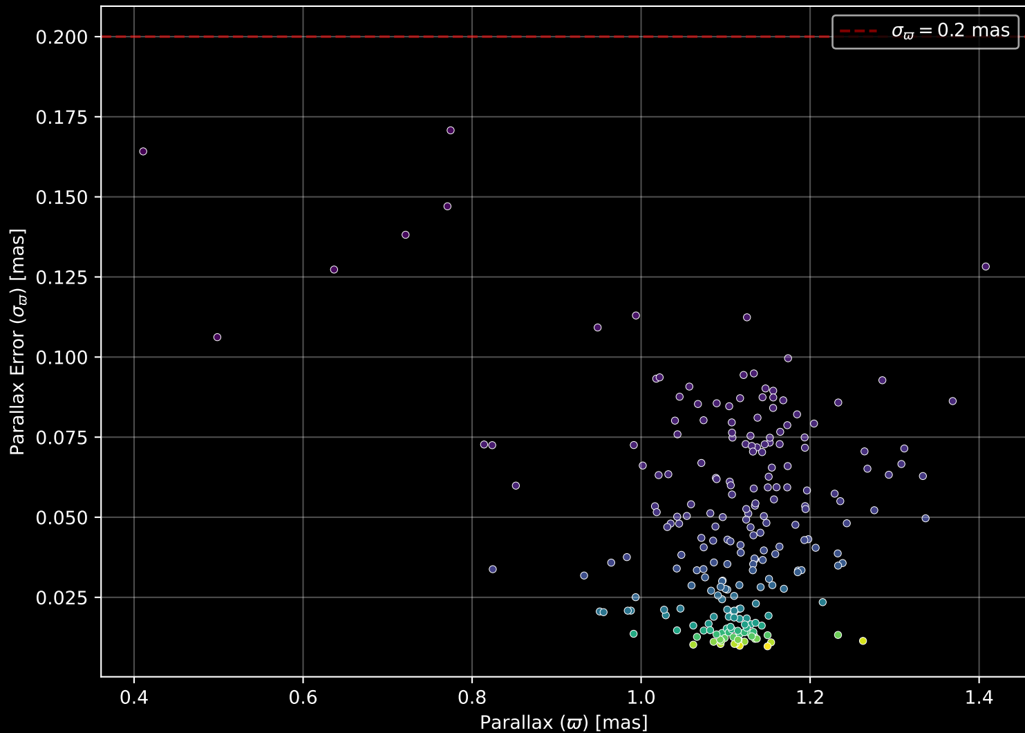
Gaia Cluster: [Alessi_Teutsch_5] Parallax Quality (n= 228)
