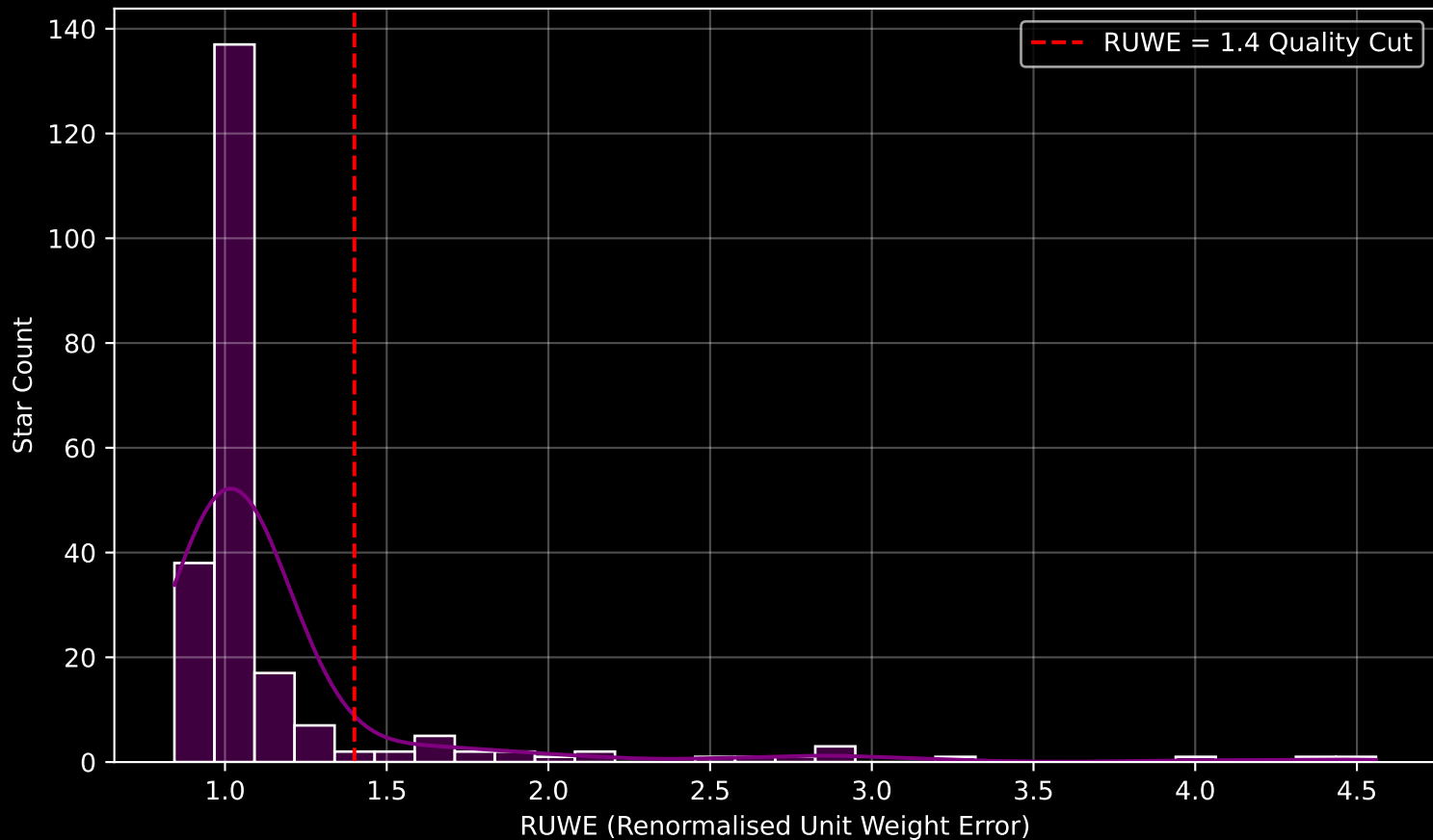
Gaia Cluster: [Alessi_Teutsch_5] RUWE Distribution (n= 225)
