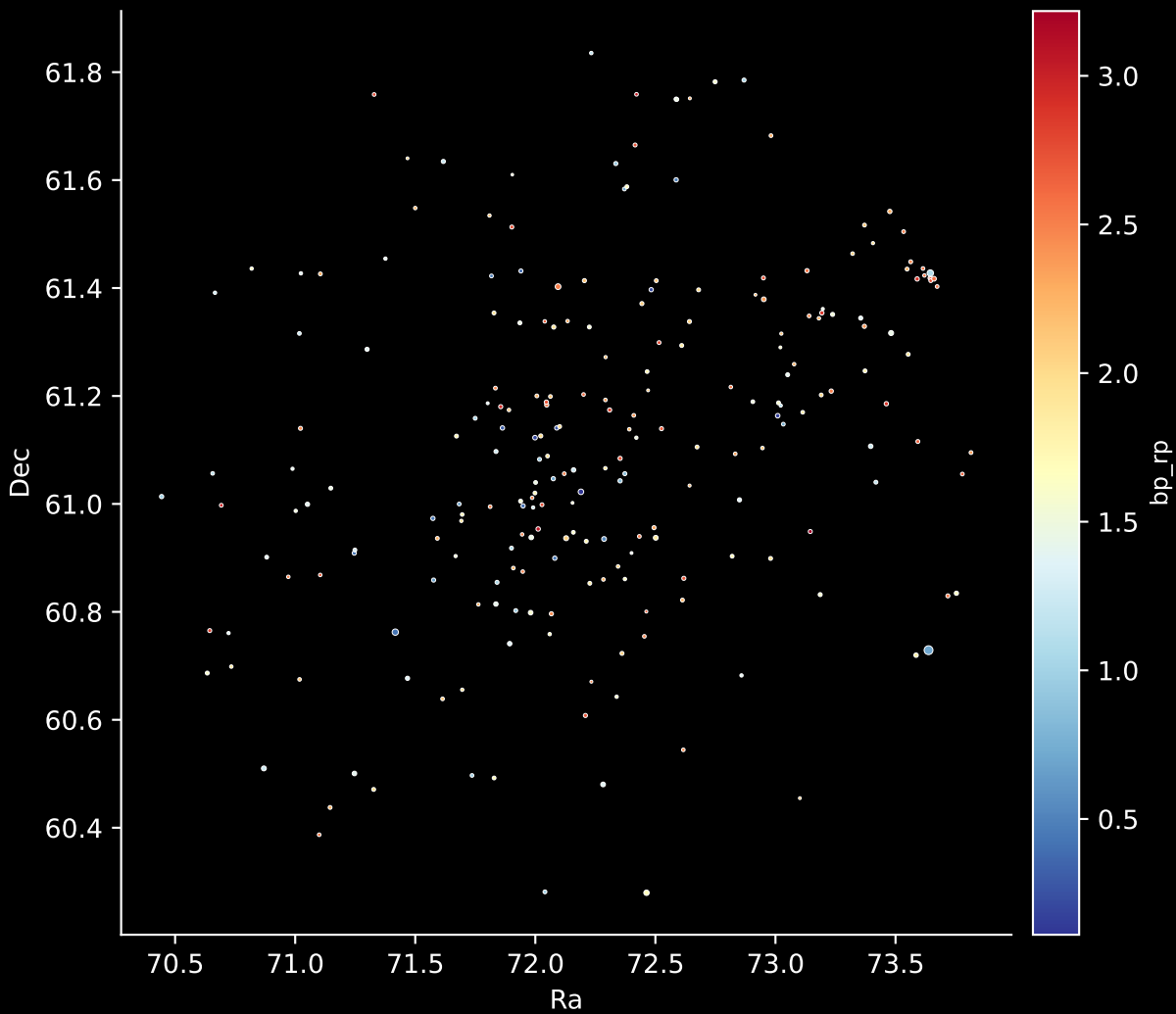
Gaia Cluster: [Alessi_Teutsch_5] Stars: 228
