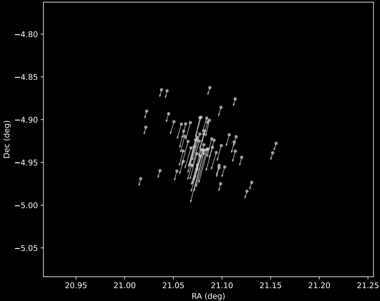
Gaia DR3 Cluster 15 Proper Motion Vectors (n=64)
