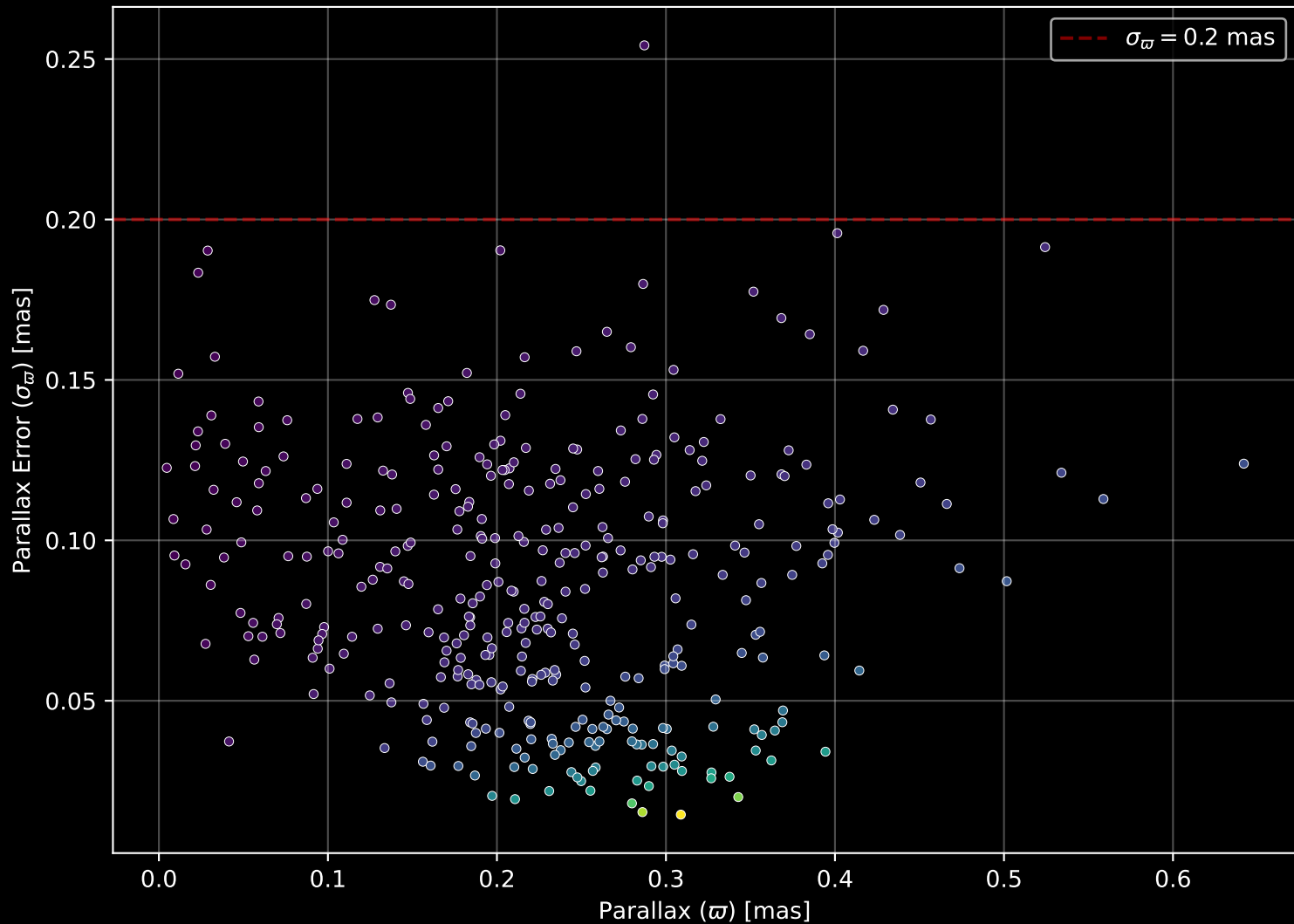
Gaia Cluster: [Andrews_Lindsay_5] Parallax Quality (n= 369)
