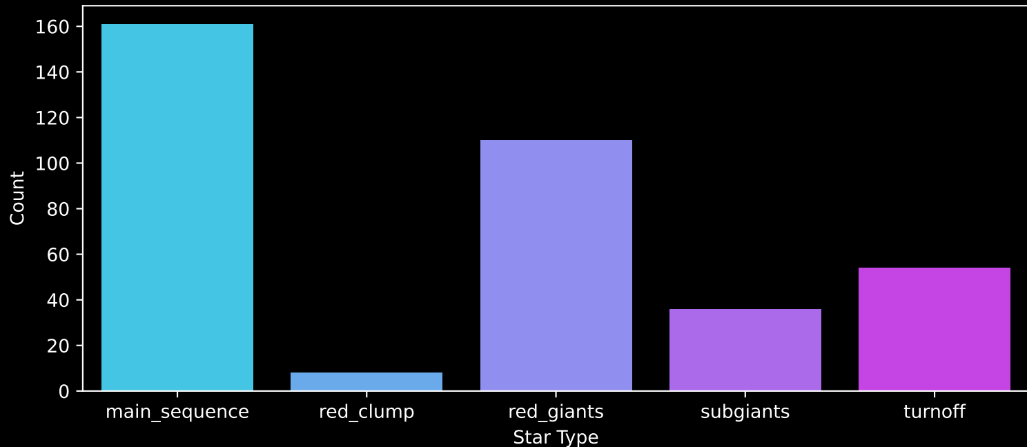
Gaia Cluster: [Andrews_Lindsay_5] Count plot of Star Type
