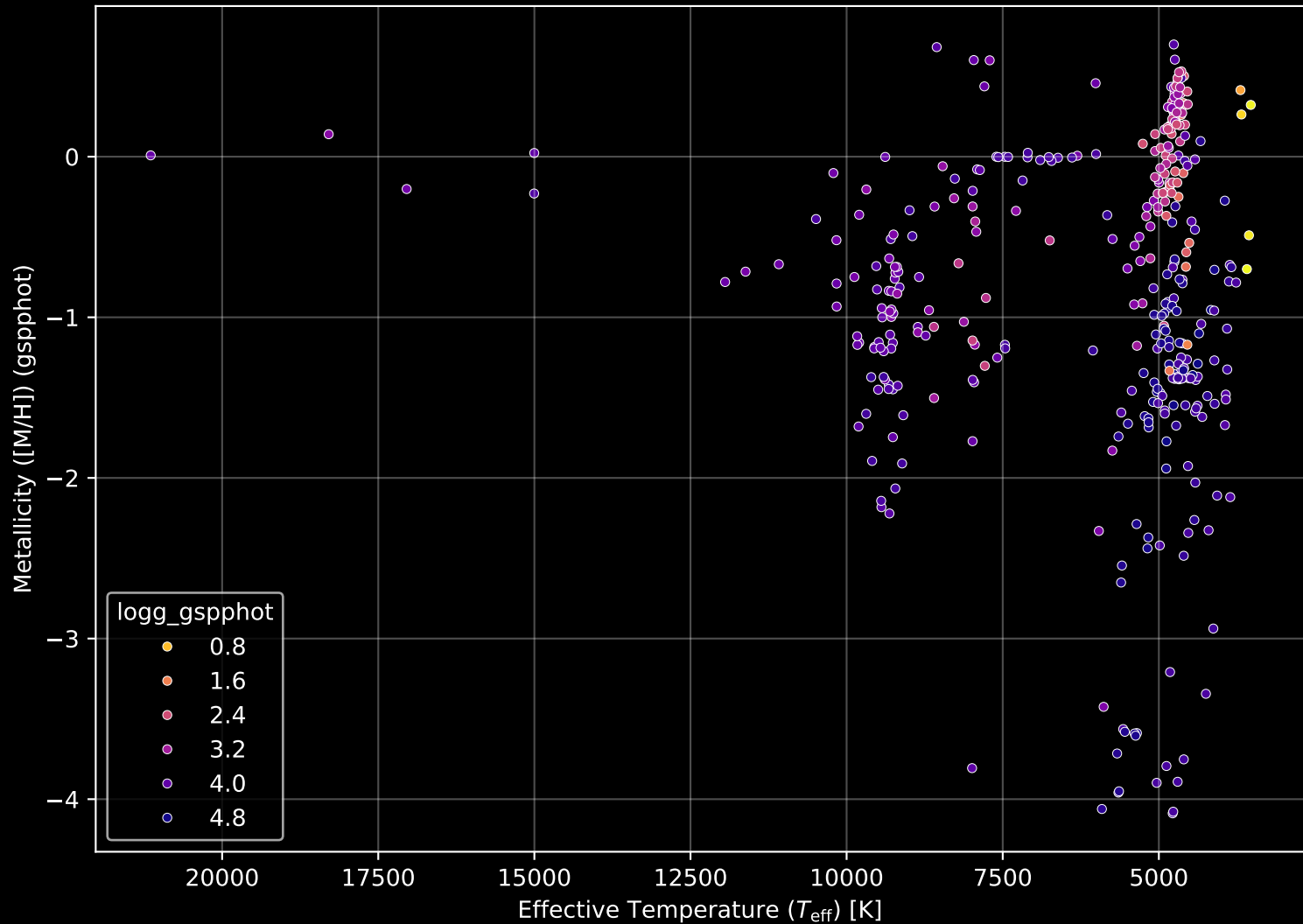
Gaia Cluster: [Andrews_Lindsay_5] Stellar Population Parameters (n= 369)
