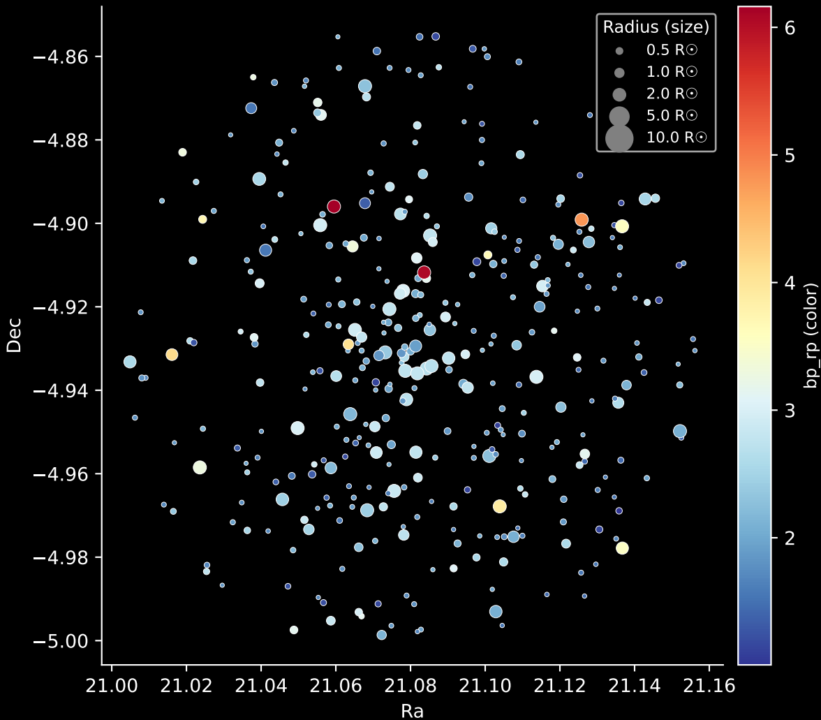
Gaia Cluster: [Andrews_Lindsay_5] Stars: 369
