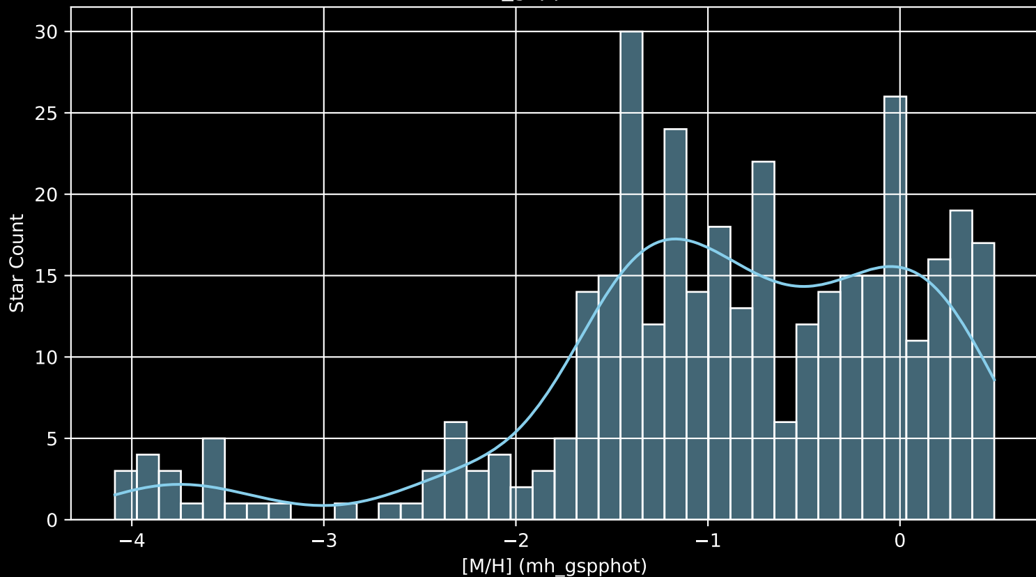
Gaia Cluster: [Andrews_Lindsay_5 [M/H] (mh_gspphot) (n= 361)
