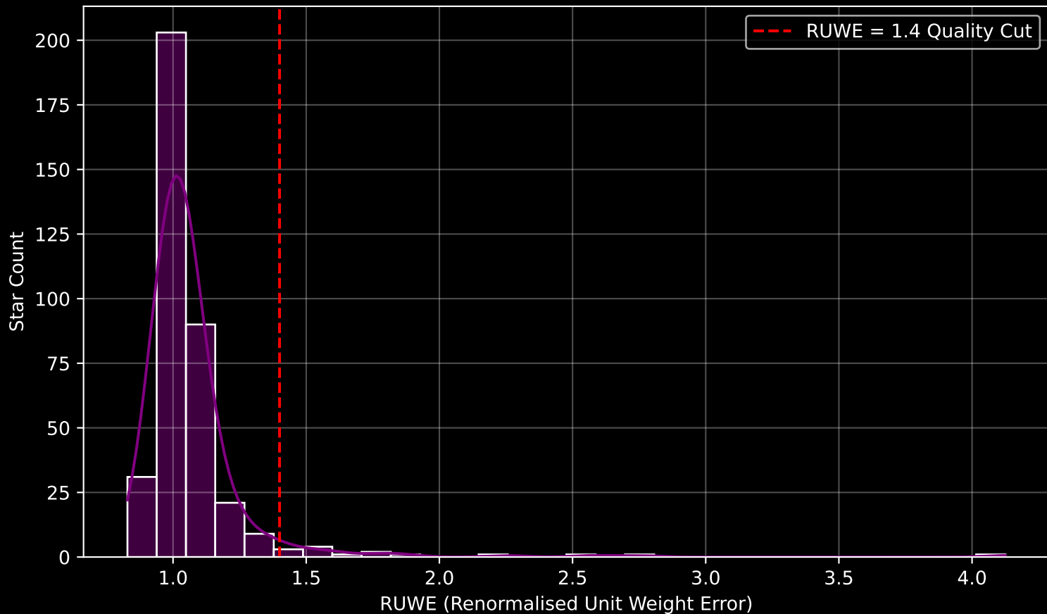
Gaia Cluster: [Andrews_Lindsay_5] RUWE Distribution (n= 369)
