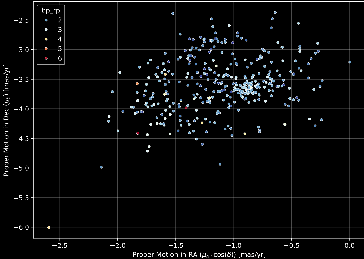
Gaia Cluster: [Andrews_Lindsay_5] Proper Motion Diagram (n= 369)
