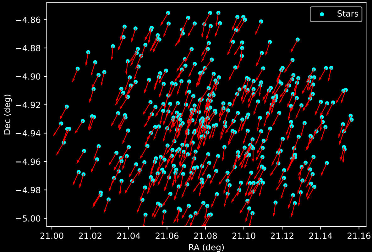
Gaia Cluster: [Andrews_Lindsay_5] Proper Motion Vectors for Gaia Star Field (n= 369)
