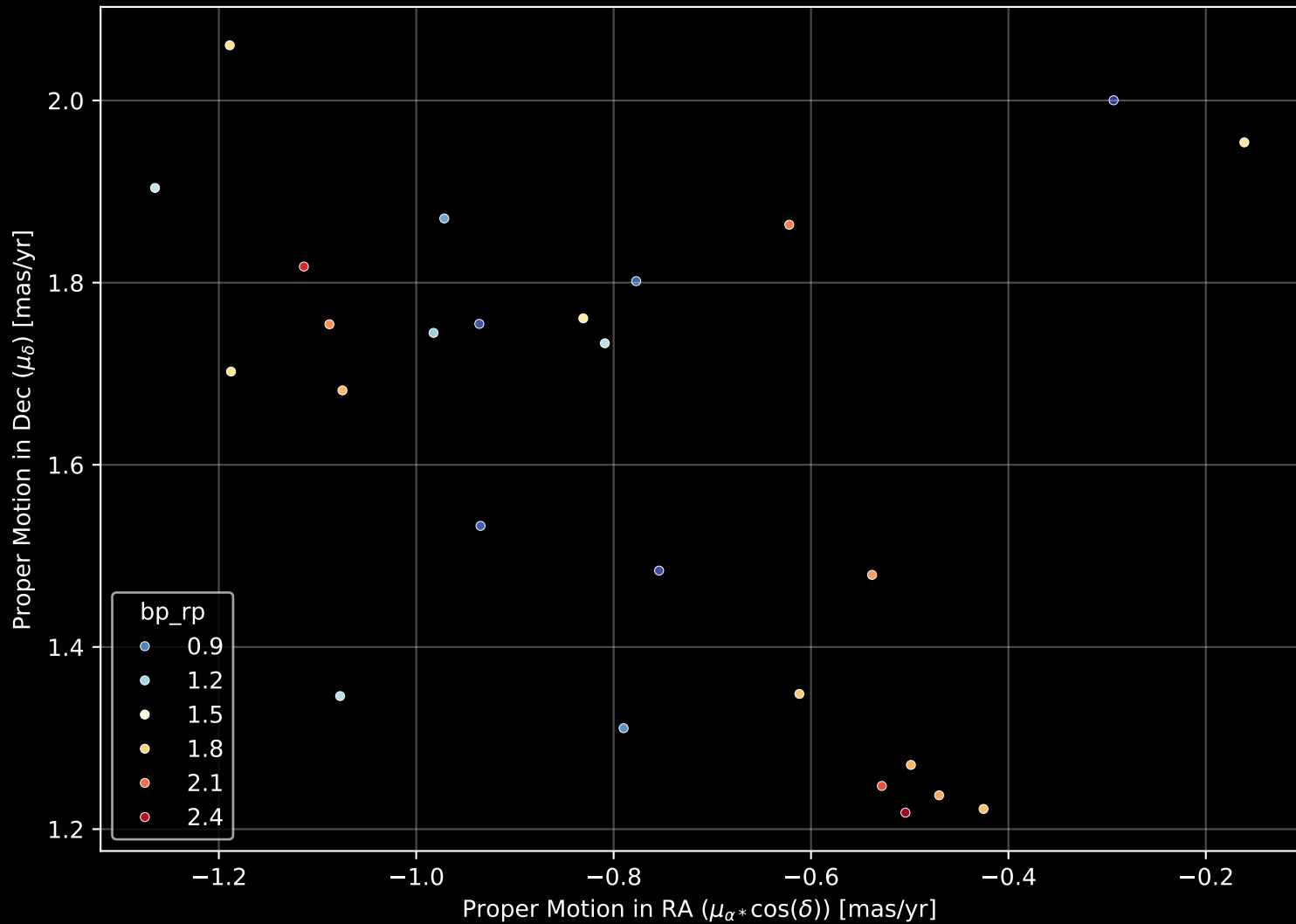
Gaia Cluster: [Arp_Madore_2] Proper Motion Diagram (n= 26)
