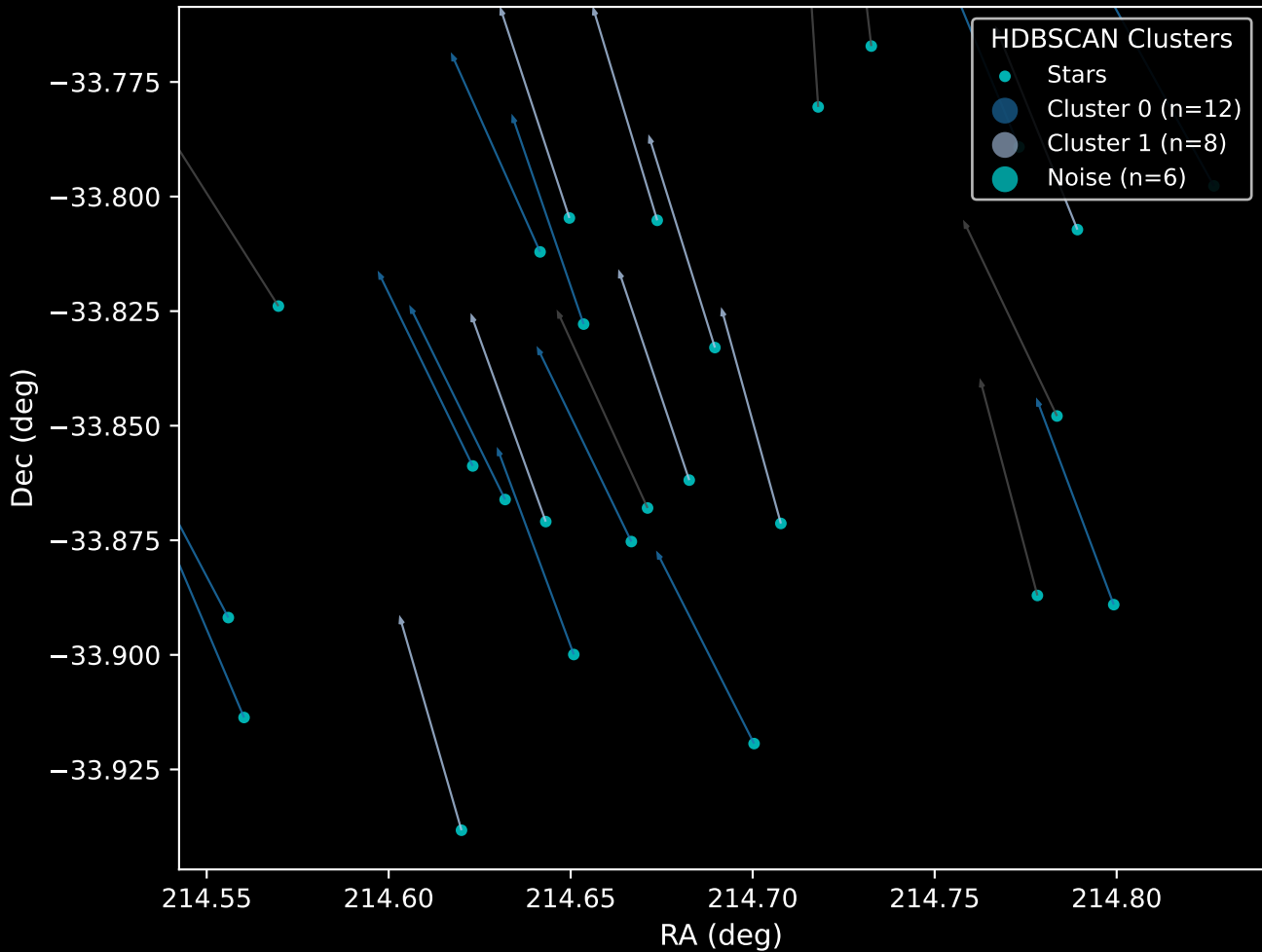
Gaia Cluster: [Arp_Madore_2] Proper Motion Vectors with HDBSCAN (n=26)
