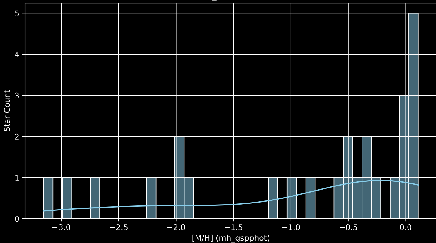
Gaia Cluster: [Arp_Madore_2 [M/H] (mh_gspphot) (n= 26)
