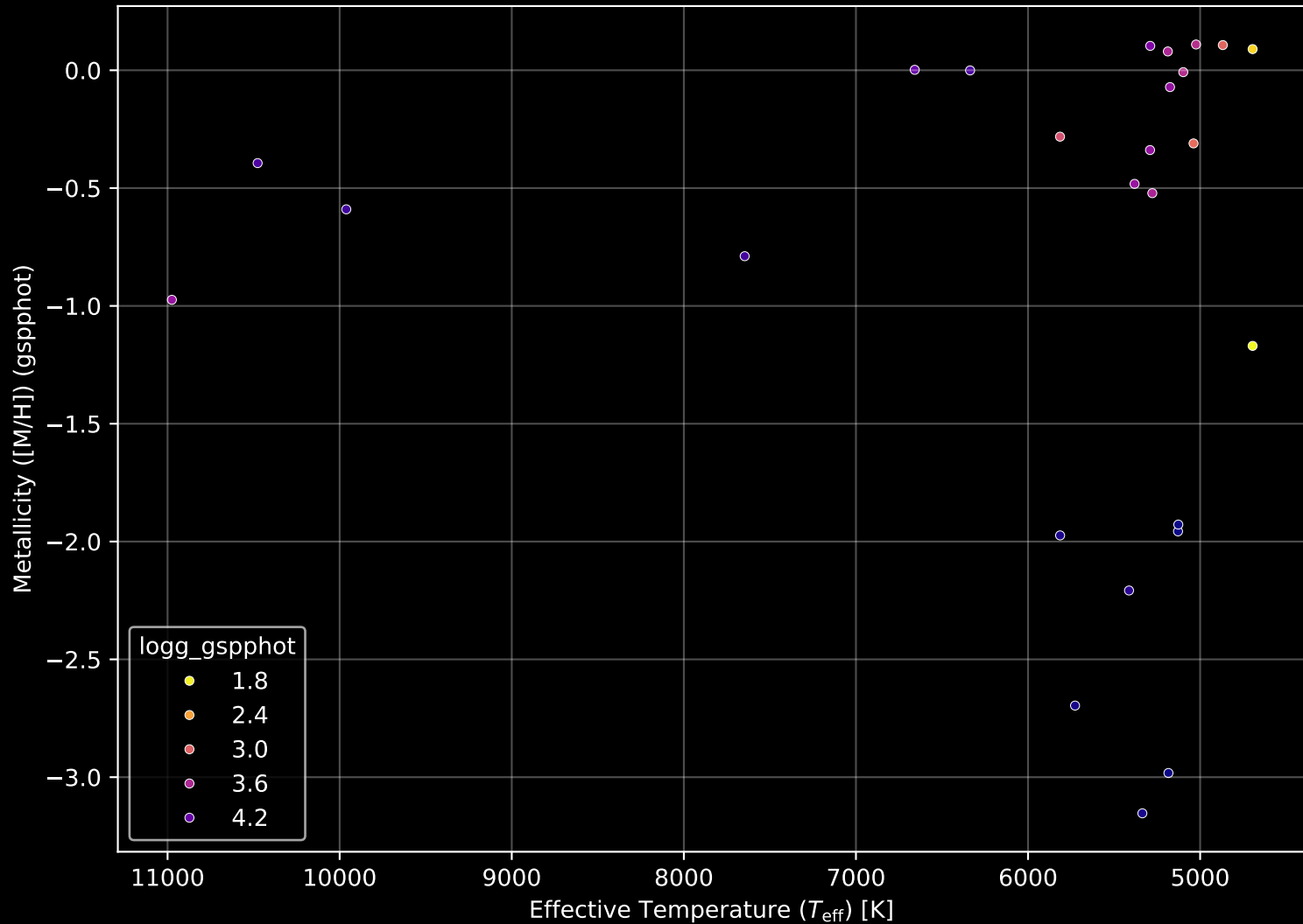
Gaia Cluster: [Arp_Madore_2] Stellar Population Parameters (n= 26)
