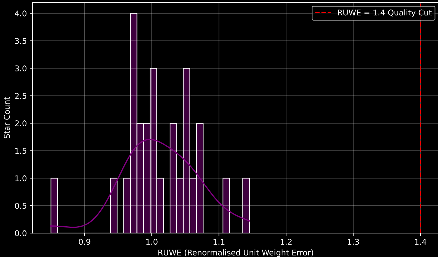
Gaia Cluster: [Arp_Madore_2] RUWE Distribution (n= 26)
