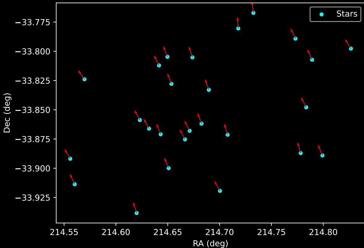
Gaia Cluster: [Arp_Madore_2] Proper Motion Vectors for Gaia Star Field (n= 26)
