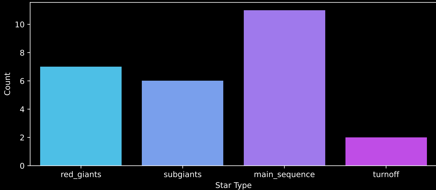
Gaia Cluster: [Arp_Madore_2] Count plot of Star Type
