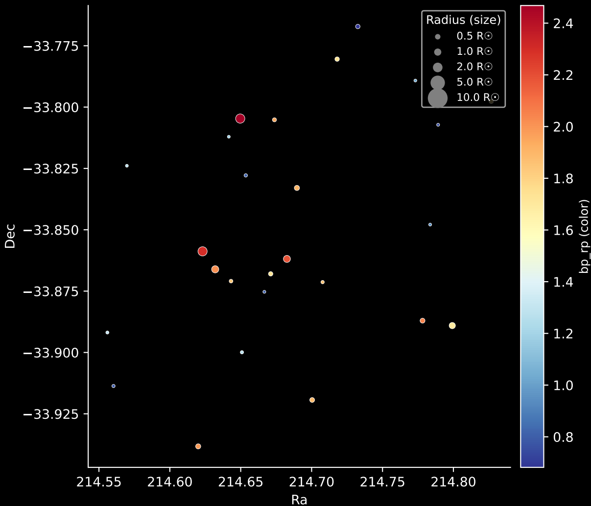
Gaia Cluster: [Arp_Madore_2] Stars: 26
