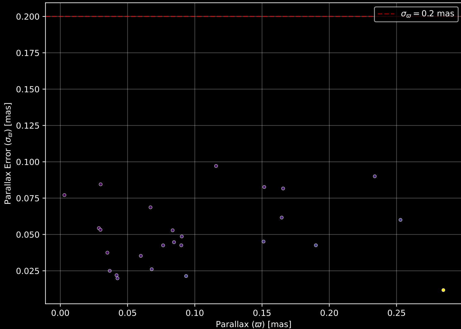
Gaia Cluster: [Arp_Madore_2] Parallax Quality (n= 26)
