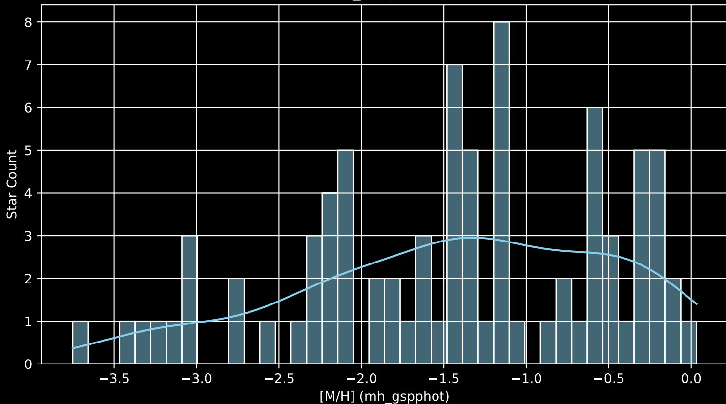
Gaia Cluster: [Auner_1 [M/H] (mh_gspphot) (n= 82)
