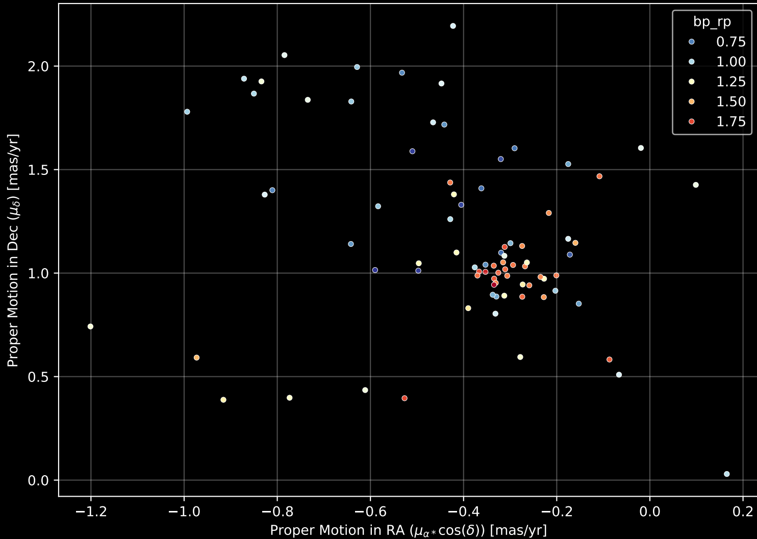
Gaia Cluster: [Auner_1] Proper Motion Diagram (n= 82)
