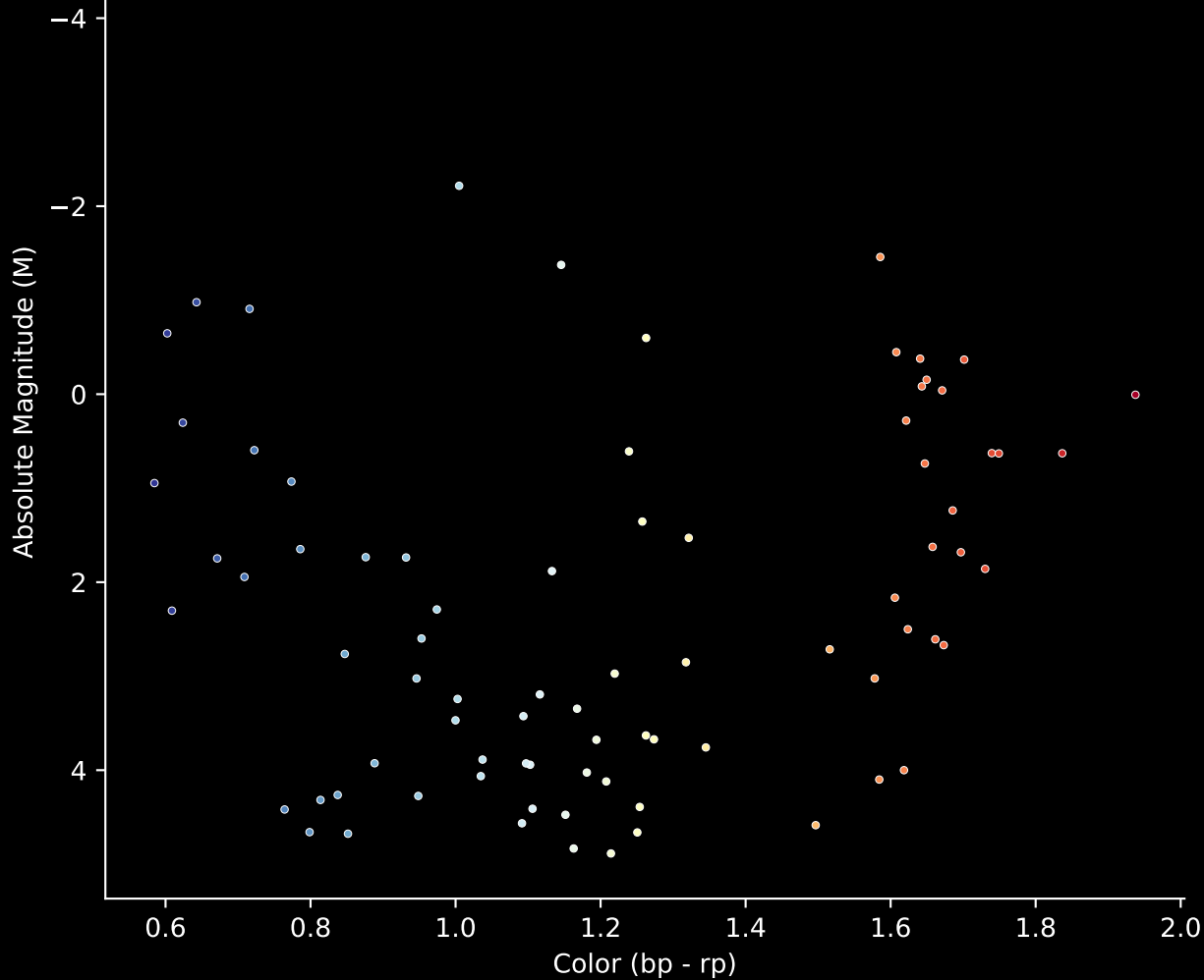
Gaia Cluster: [Auner_1] Stars (n= 82) Hertzsprung-Russel Diagram
