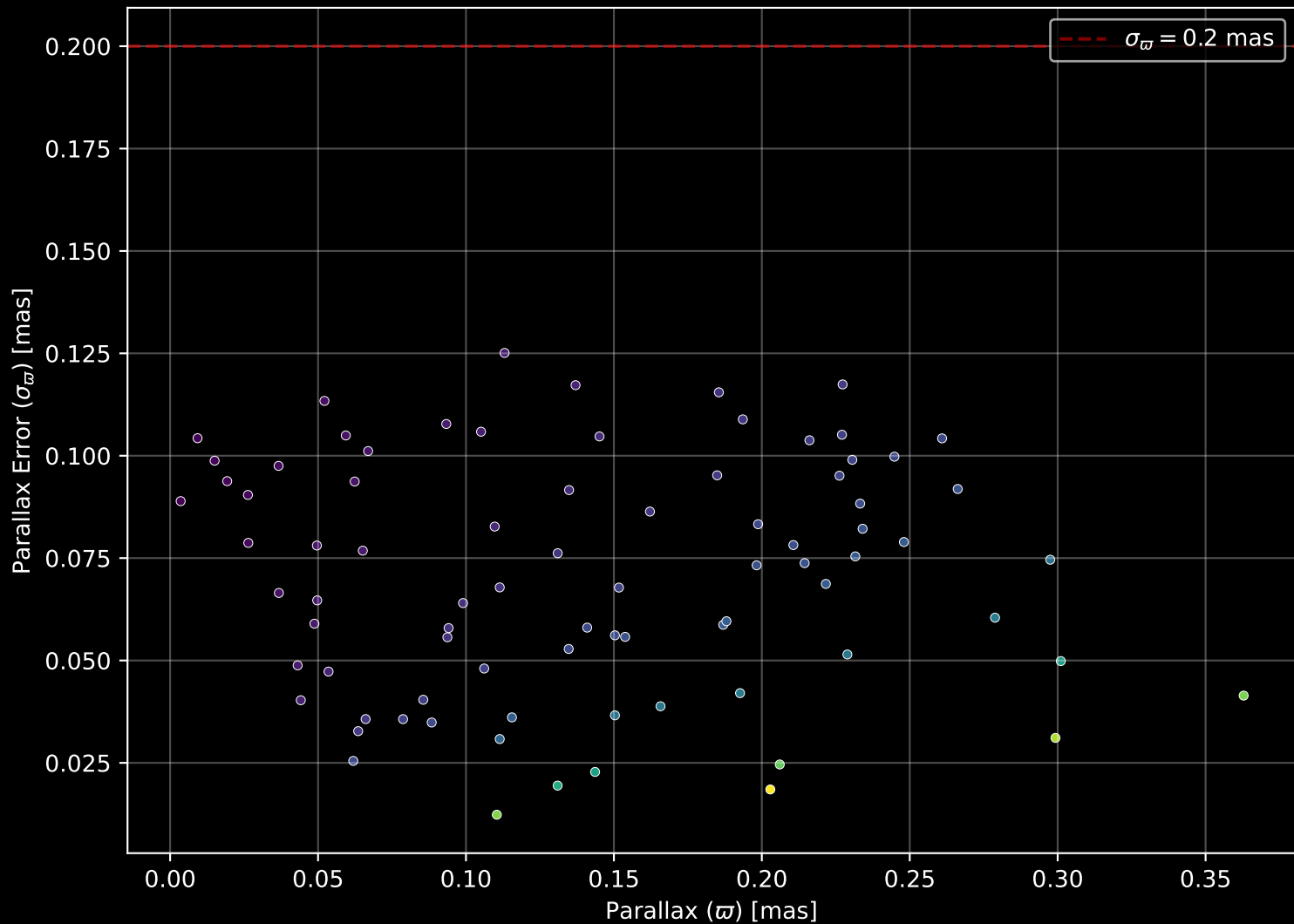
Gaia Cluster: [Auner_1] Parallax Quality (n= 82)
