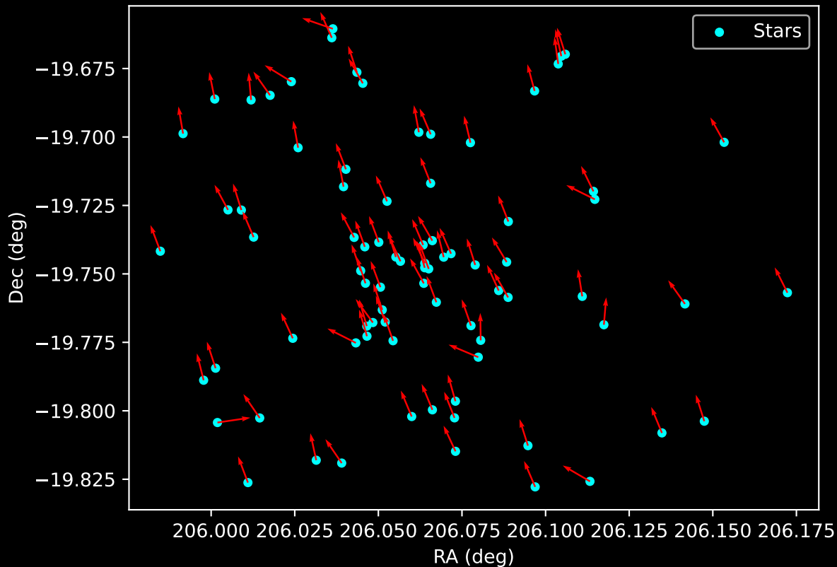
Gaia Cluster: [Auner_1] Proper Motion Vectors for Gaia Star Field (n= 82)
