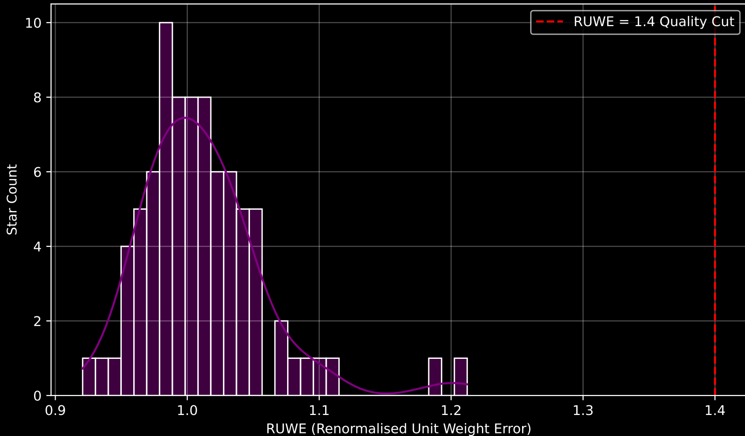
Gaia Cluster: [Auner_1] RUWE Distribution (n= 82)
