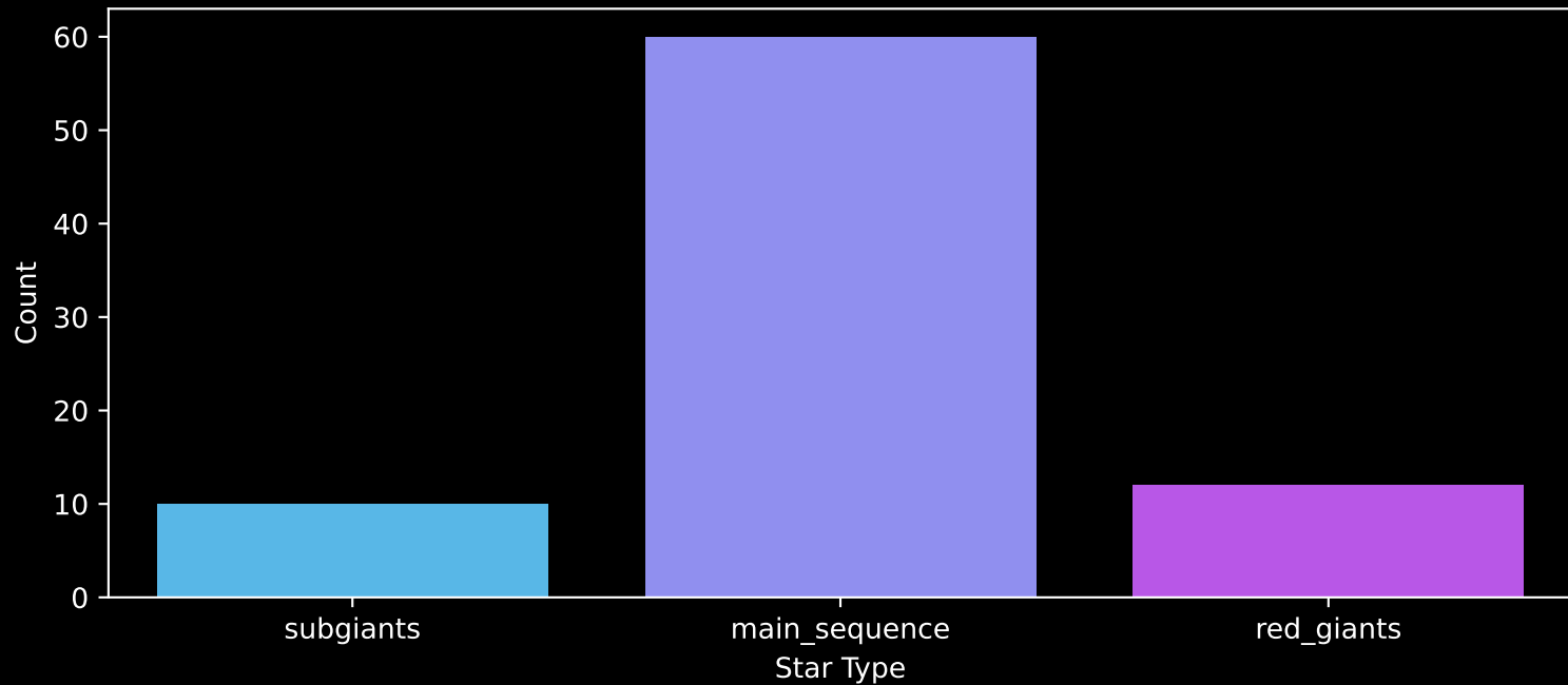
Gaia Cluster: [Auner_1] Count plot of Star Type
