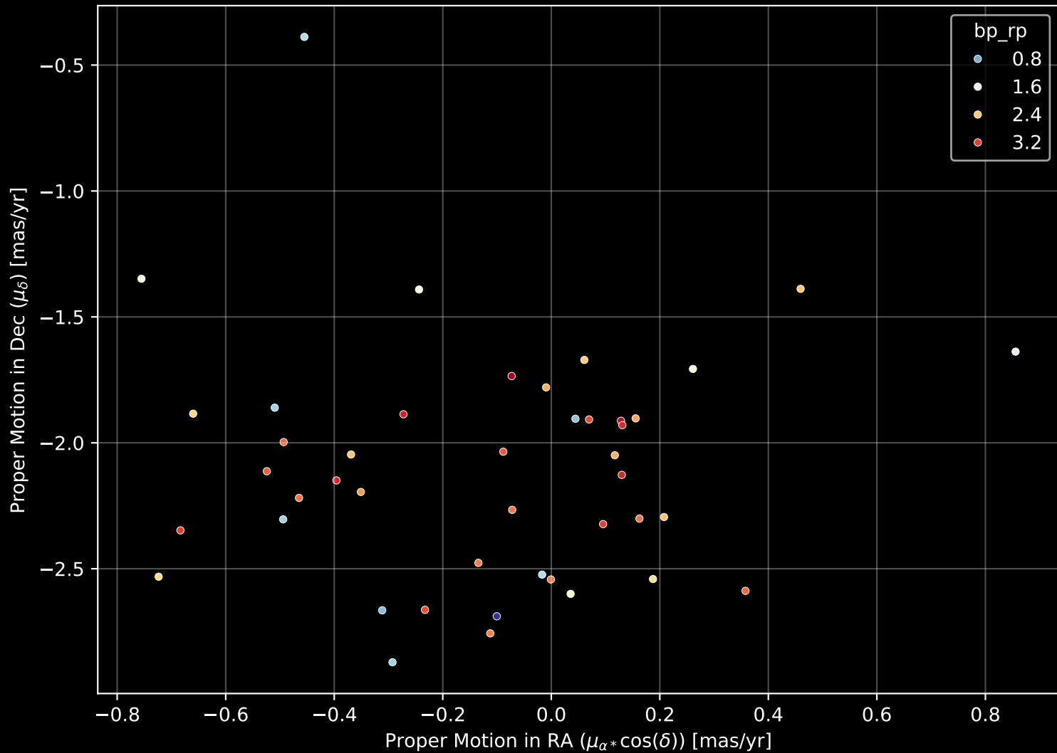
Gaia Cluster: [Aveni_Hunter_1] Proper Motion Diagram (n= 44)
