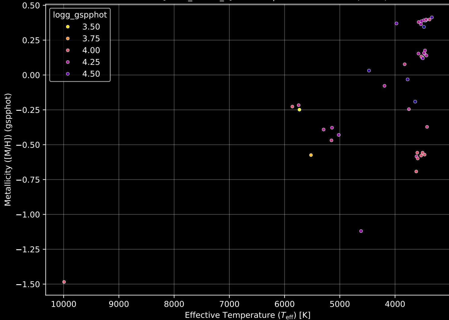
Gaia Cluster: [Aveni_Hunter_1] Stellar Population Parameters (n= 44)
