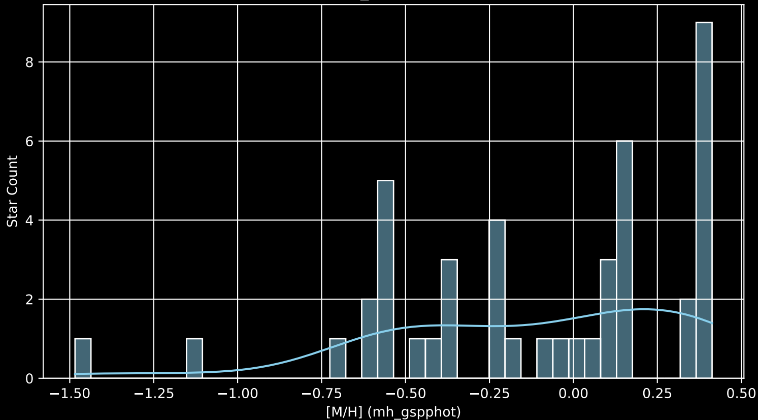
Gaia Cluster: [Aveni_Hunter_1 [M/H] (mh_gspphot) (n= 44)
