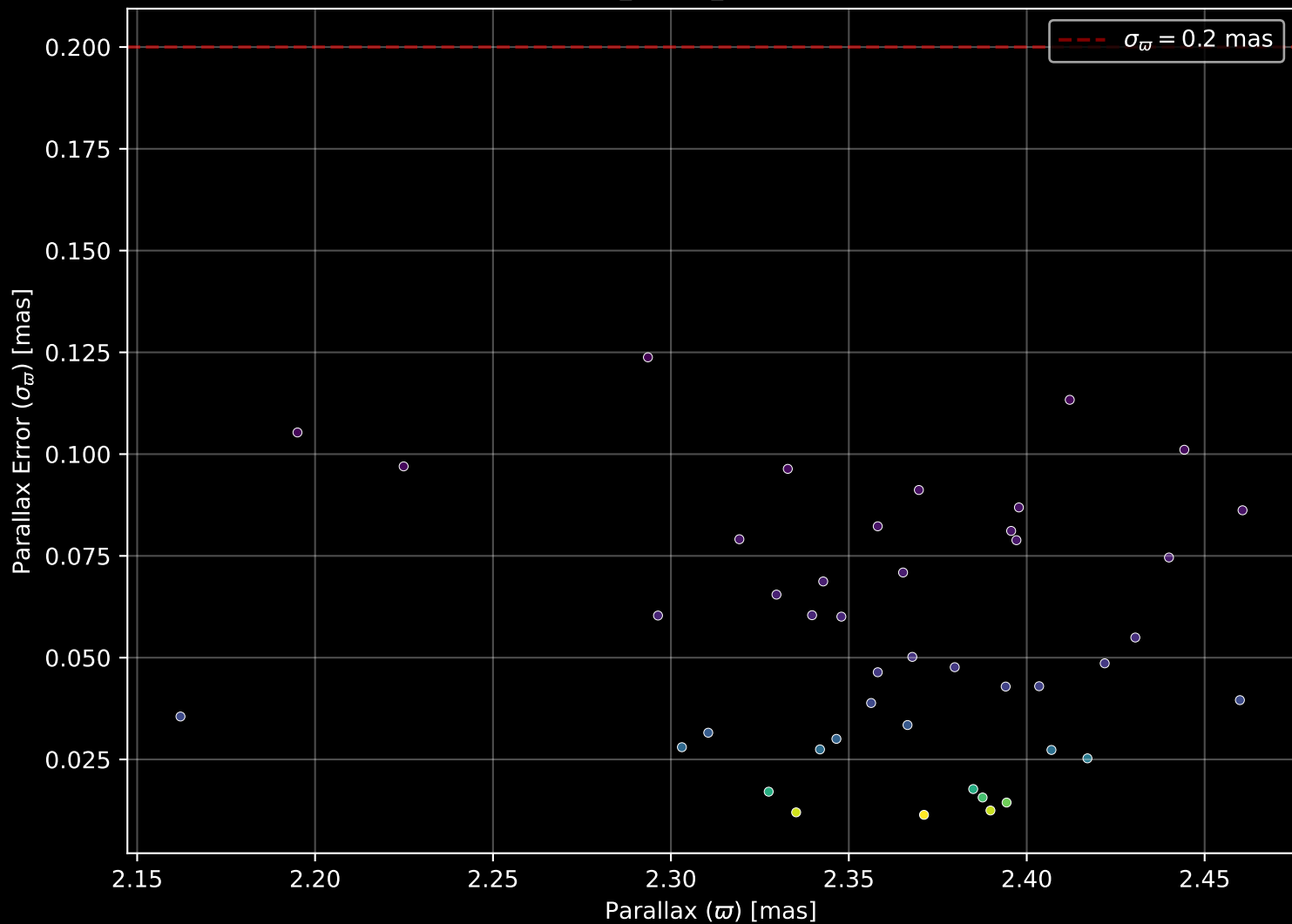
Gaia Cluster: [Aveni_Hunter_1] Parallax Quality (n= 44)
