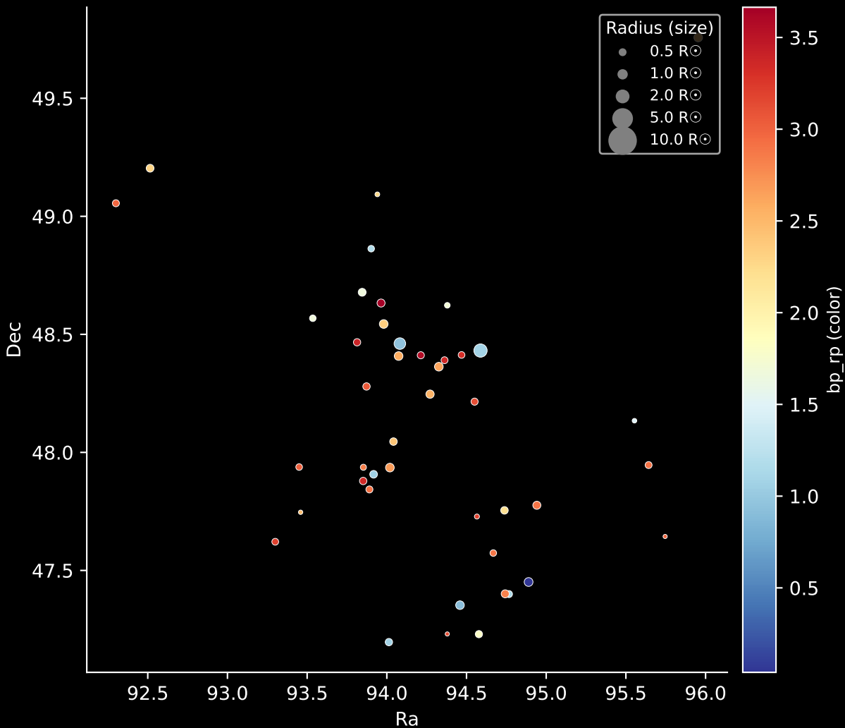
Gaia Cluster: [Aveni_Hunter_1] Stars: 44
