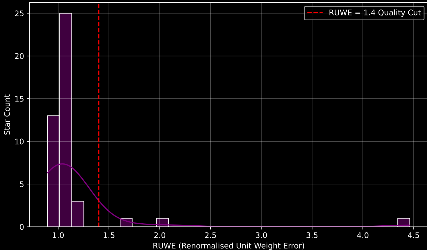
Gaia Cluster: [Aveni_Hunter_1] RUWE Distribution (n= 44)
