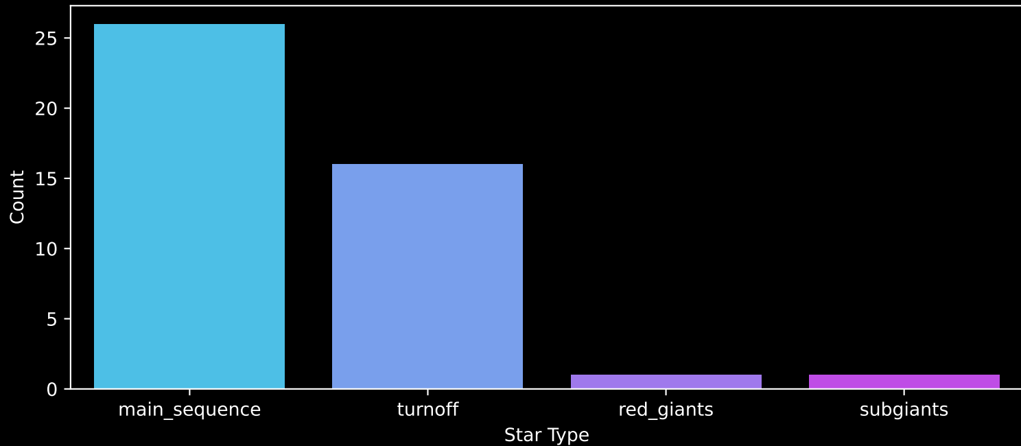
Gaia Cluster: [Aveni_Hunter_1] Count plot of Star Type
