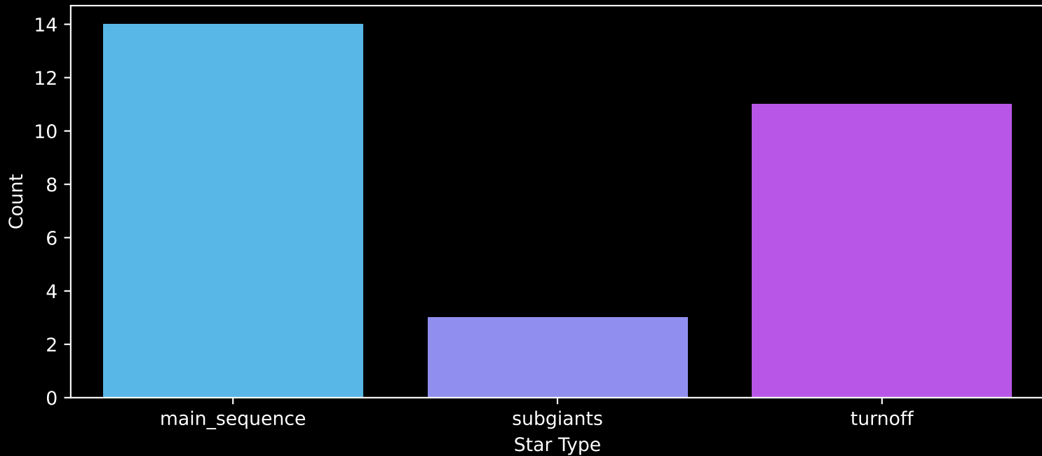
Gaia Cluster: [BDSB91] Count plot of Star Type
