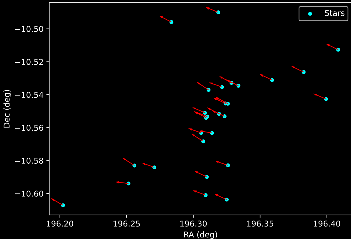
Gaia Cluster: [BDSB91] Proper Motion Vectors for Gaia Star Field (n= 28)
