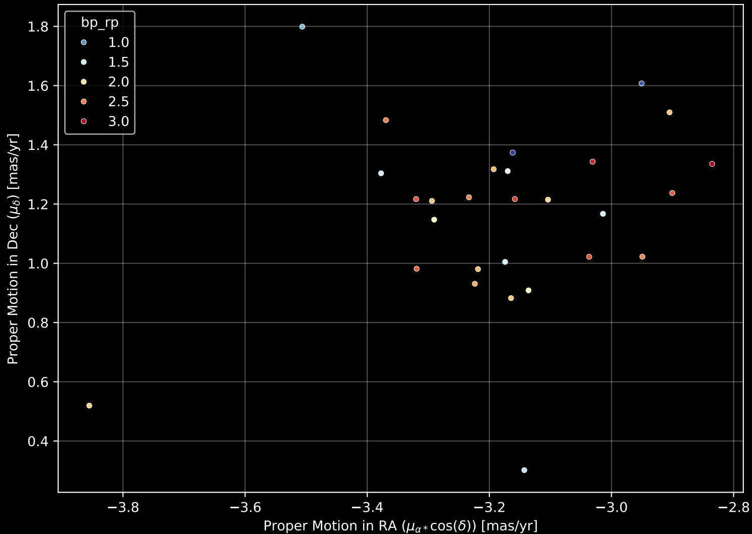
Gaia Cluster: [BDSB91] Proper Motion Diagram (n= 28)
