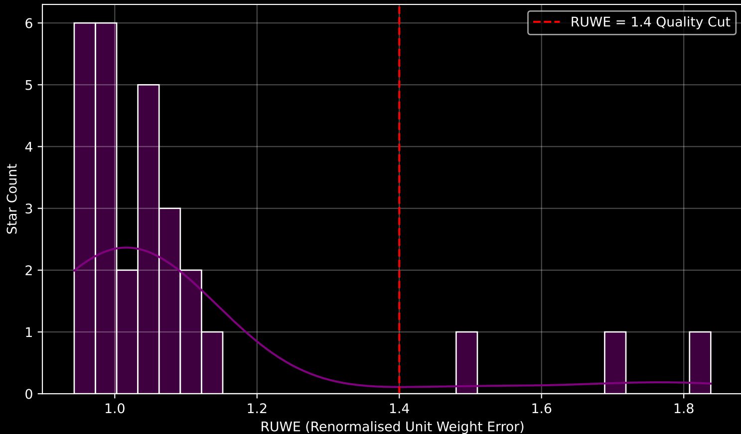
Gaia Cluster: [BDSB91] RUWE Distribution (n= 28)
