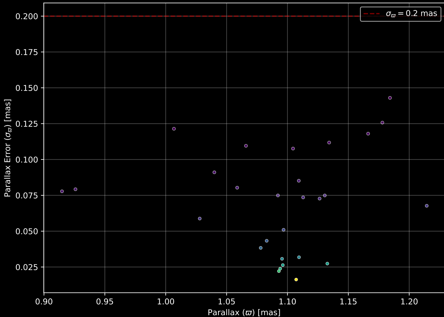
Gaia Cluster: [BDSB91] Parallax Quality (n= 28)
