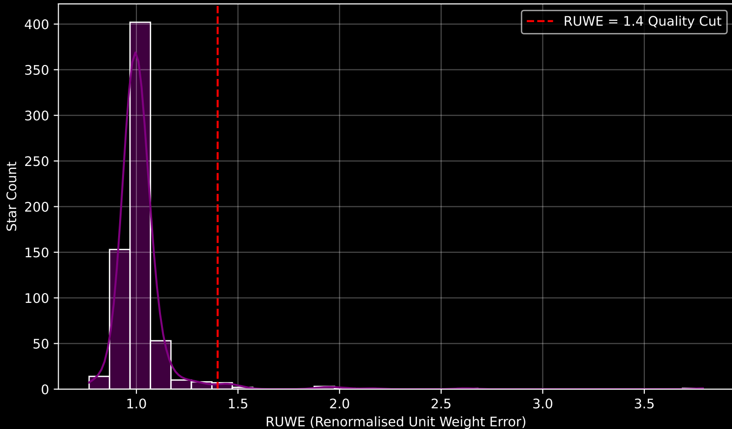
Gaia Cluster: [BH_121] RUWE Distribution (n= 656)
