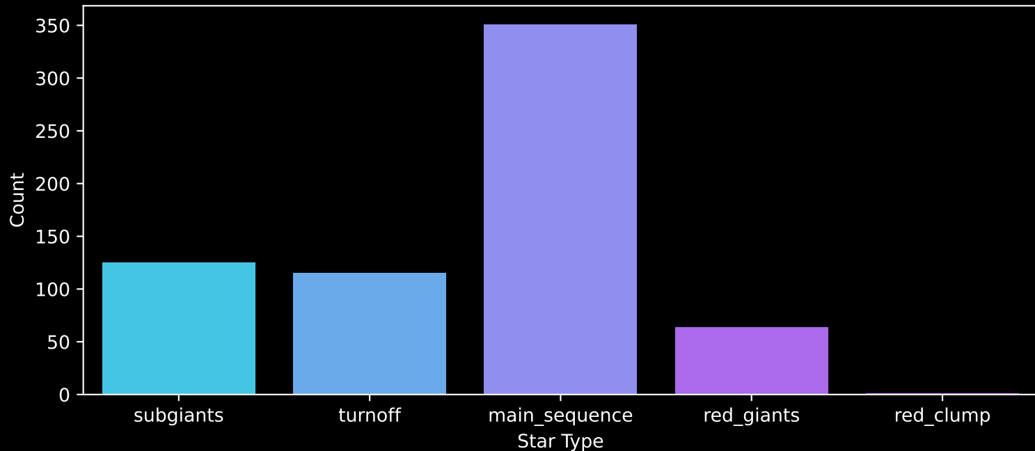
Gaia Cluster: [BH_121] Count plot of Star Type
