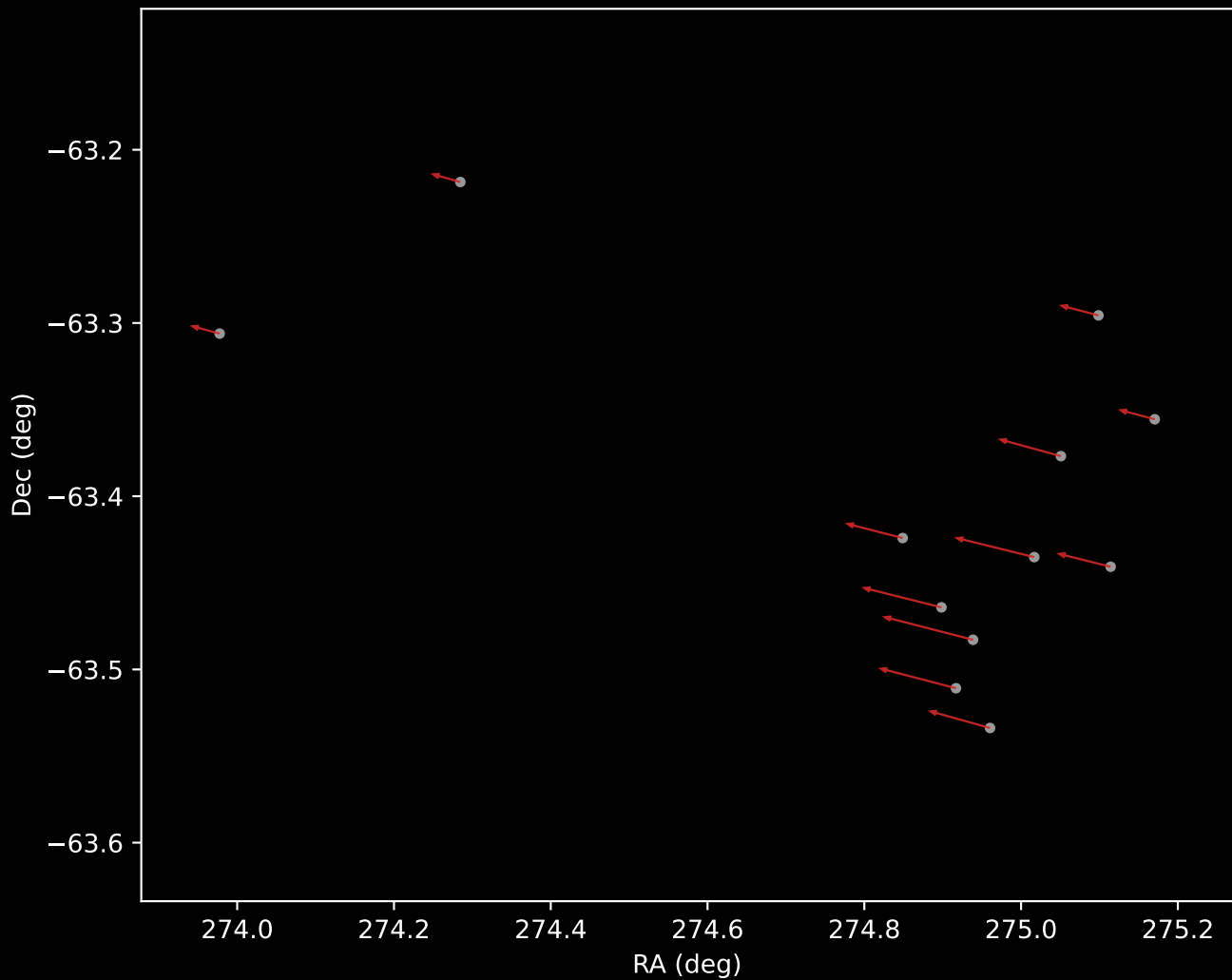
Gaia DR3 Cluster 26 Proper Motion Vectors (n=12)
