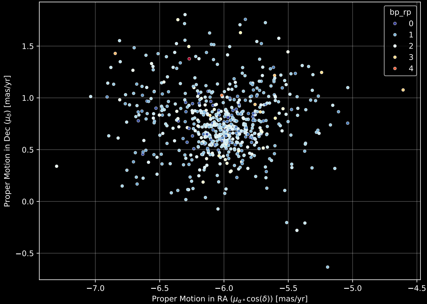
Gaia Cluster: [BH_121] Proper Motion Diagram (n= 656)
