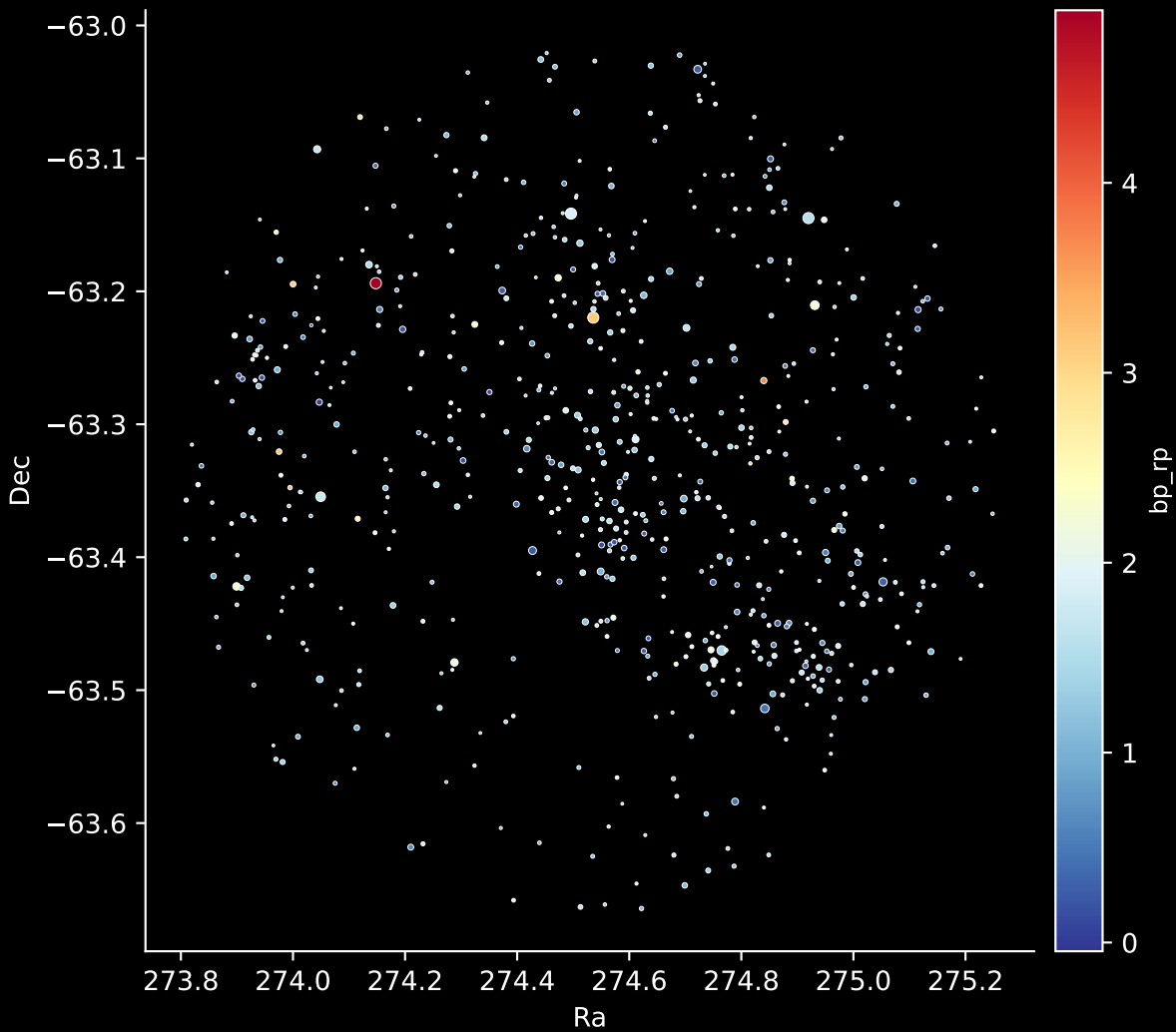
Gaia Cluster: [BH_121] Stars: 656
