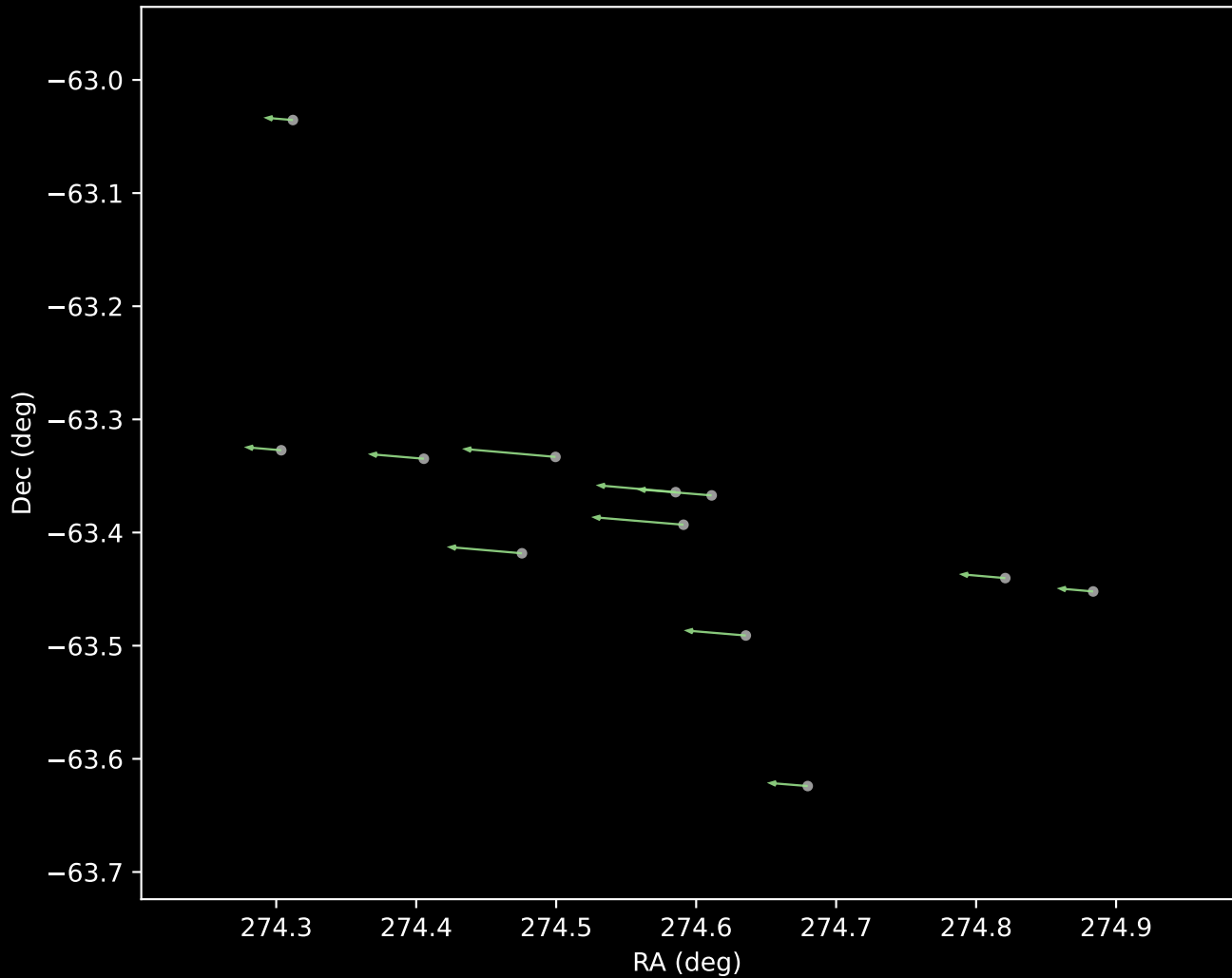
Gaia DR3 Cluster 25 Proper Motion Vectors (n=12)
