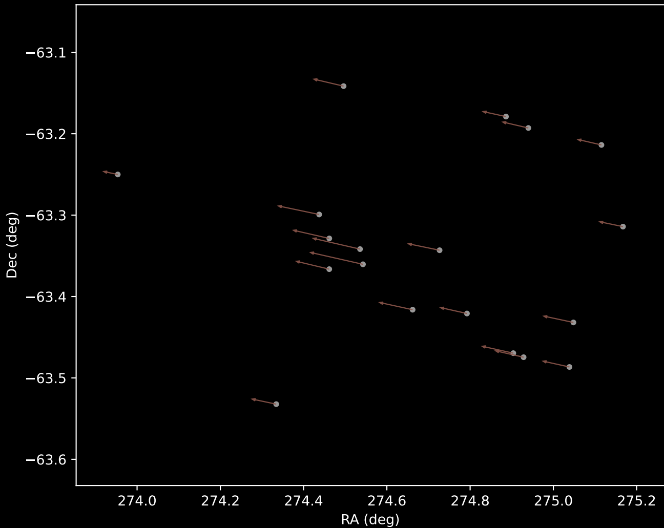
Gaia DR3 Cluster 30 Proper Motion Vectors (n=19)
