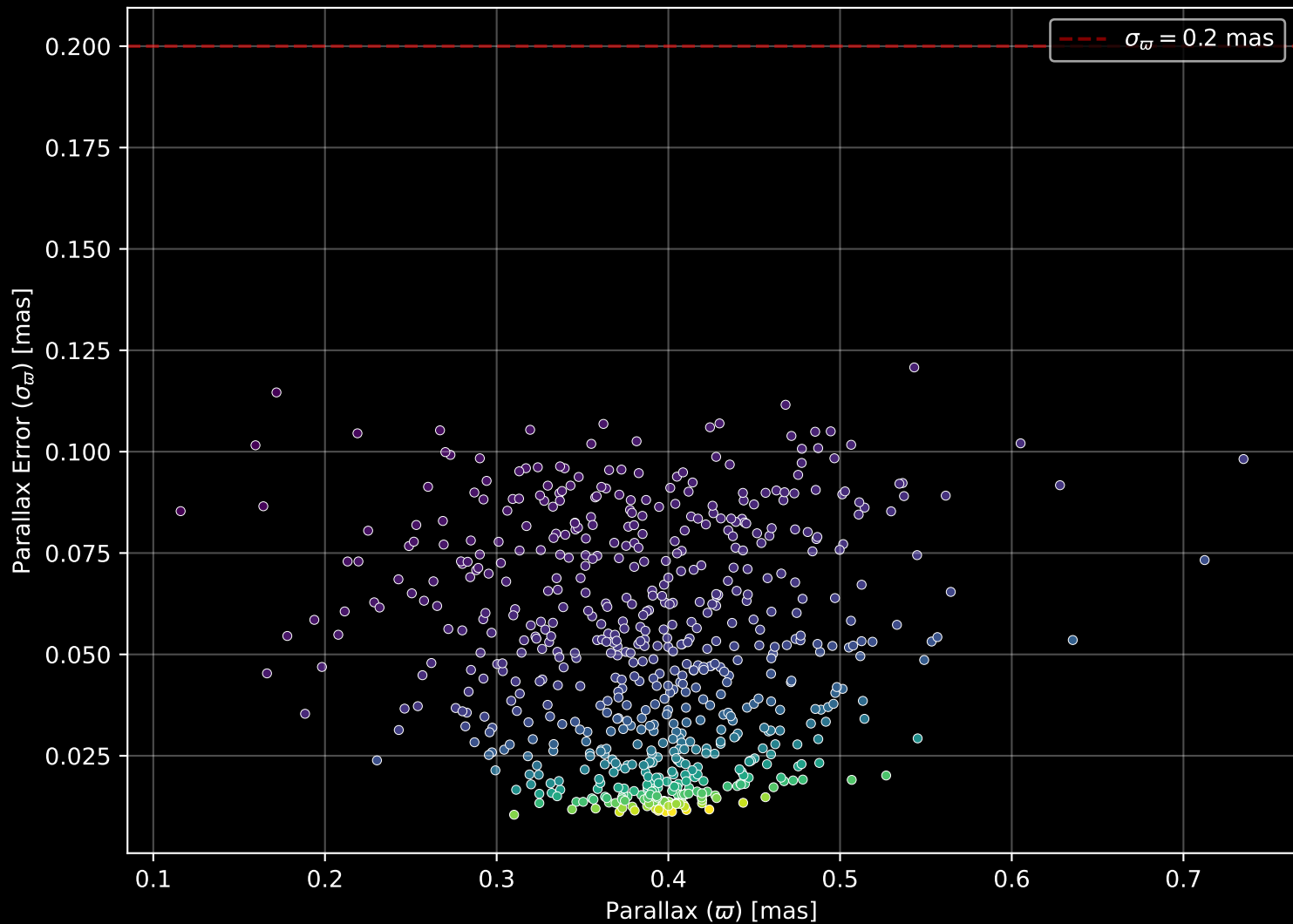
Gaia Cluster: [BH_121] Parallax Quality (n= 656)
