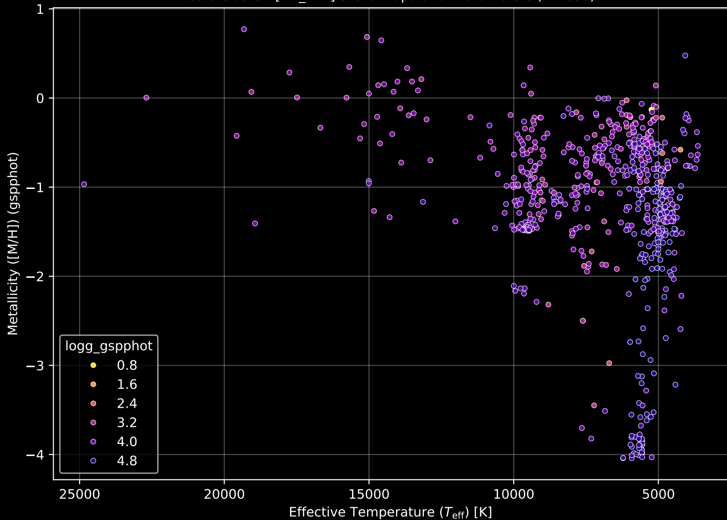
Gaia Cluster: [BH_121] Stellar Population Parameters (n= 656)
