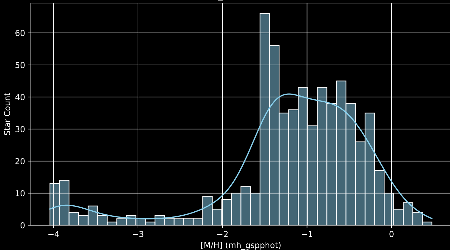
Gaia Cluster: [BH_121 [M/H] (mh_gspphot) (n= 653)
