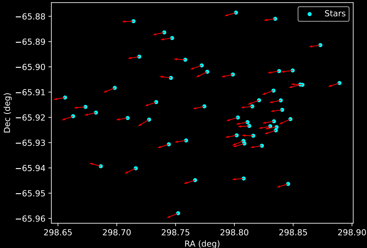
Gaia Cluster: [BH_144] Proper Motion Vectors for Gaia Star Field (n= 52)
