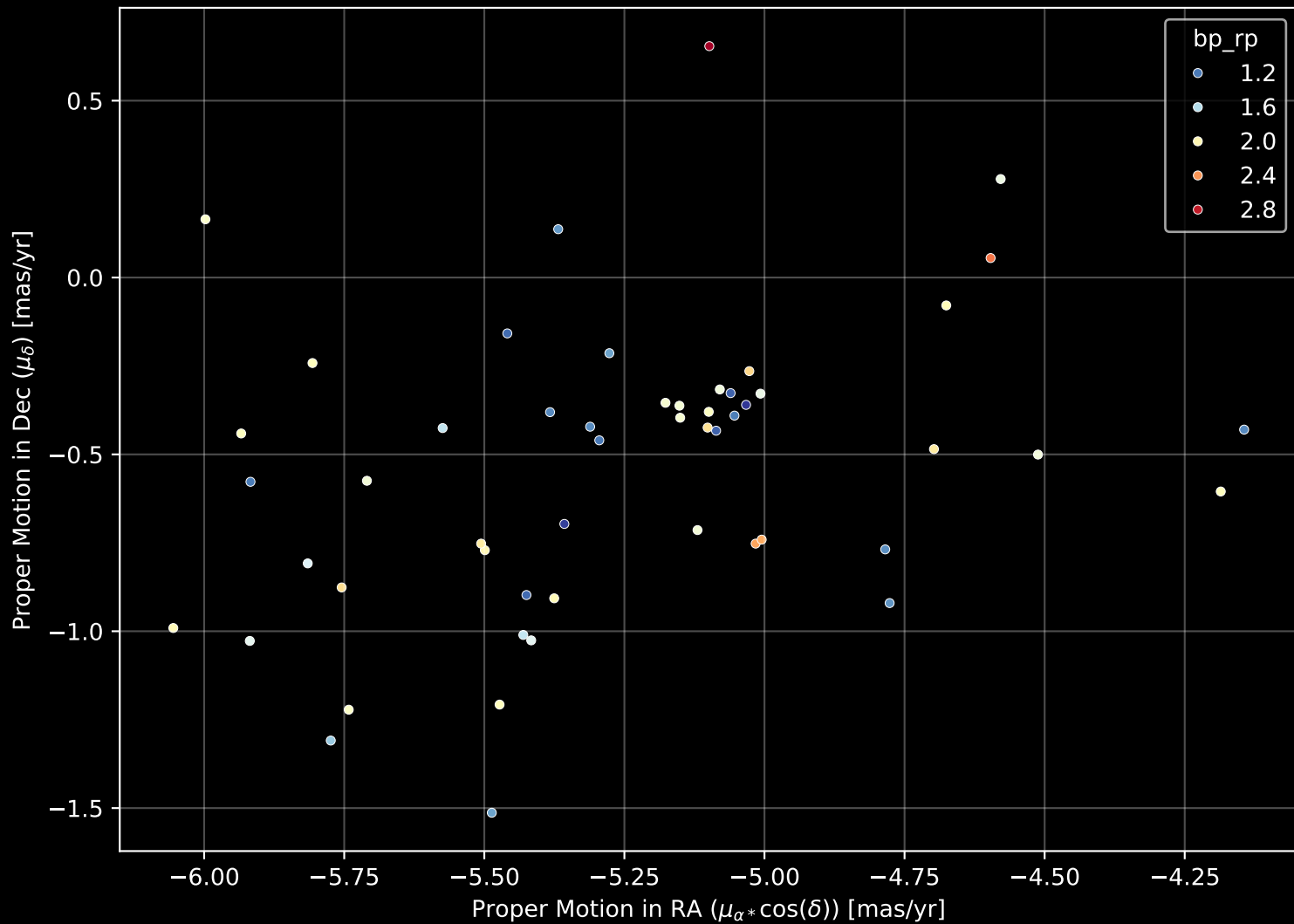
Gaia Cluster: [BH_144] Proper Motion Diagram (n= 52)
