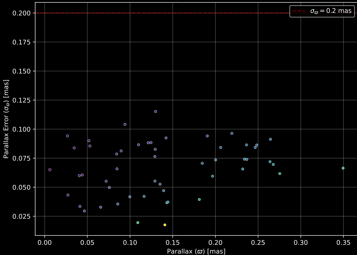
Gaia Cluster: [BH_144] Parallax Quality (n= 52)
