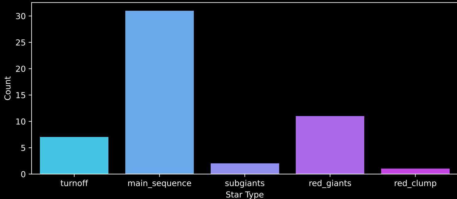
Gaia Cluster: [BH_144] Count plot of Star Type
