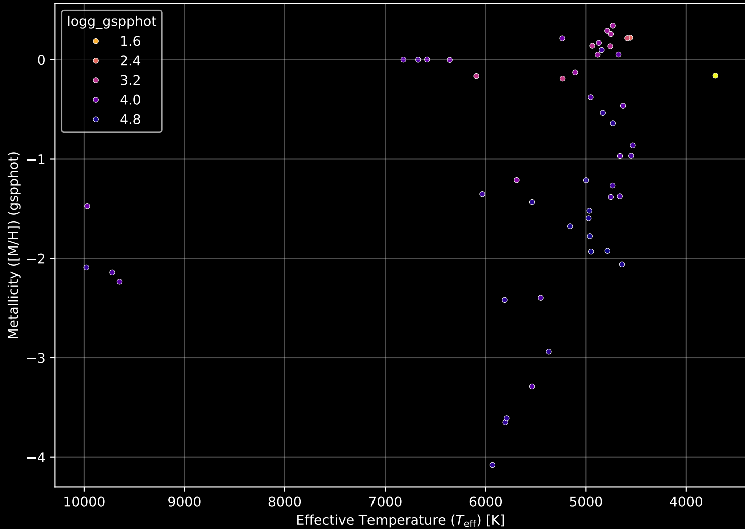
Gaia Cluster: [BH_144] Stellar Population Parameters (n= 52)
