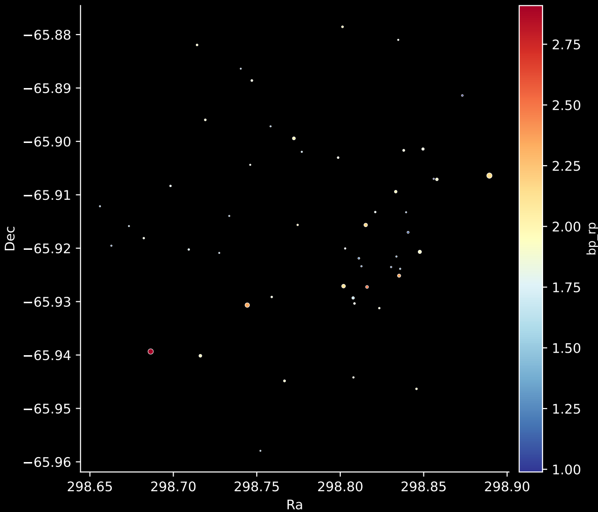
Gaia Cluster: [BH_144] Stars: 52
