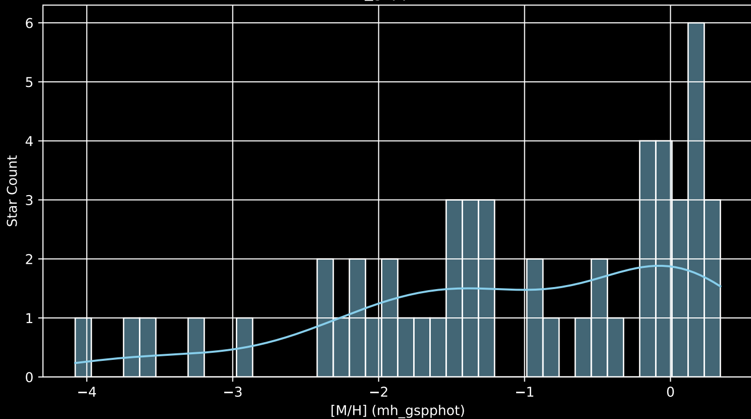
Gaia Cluster: [BH_144 [M/H] (mh_gspphot) (n= 52)
