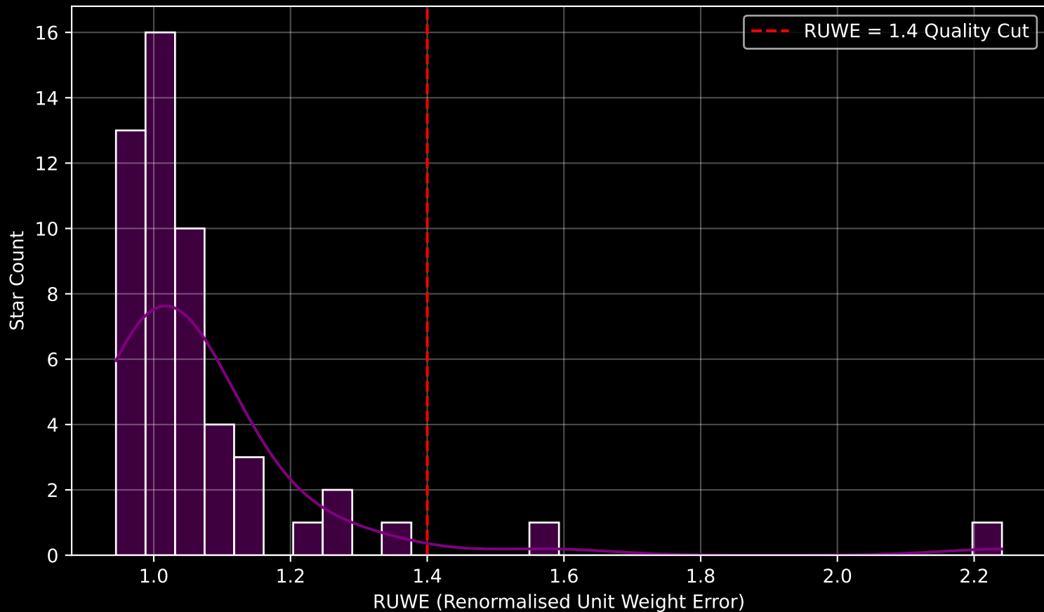
Gaia Cluster: [BH_144] RUWE Distribution (n= 52)
