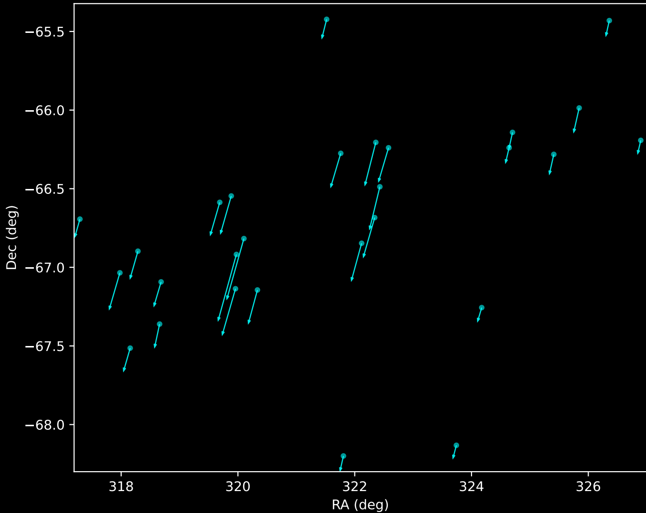
Gaia DR3 Noise Stream Proper Motion Vectors (n=28)
