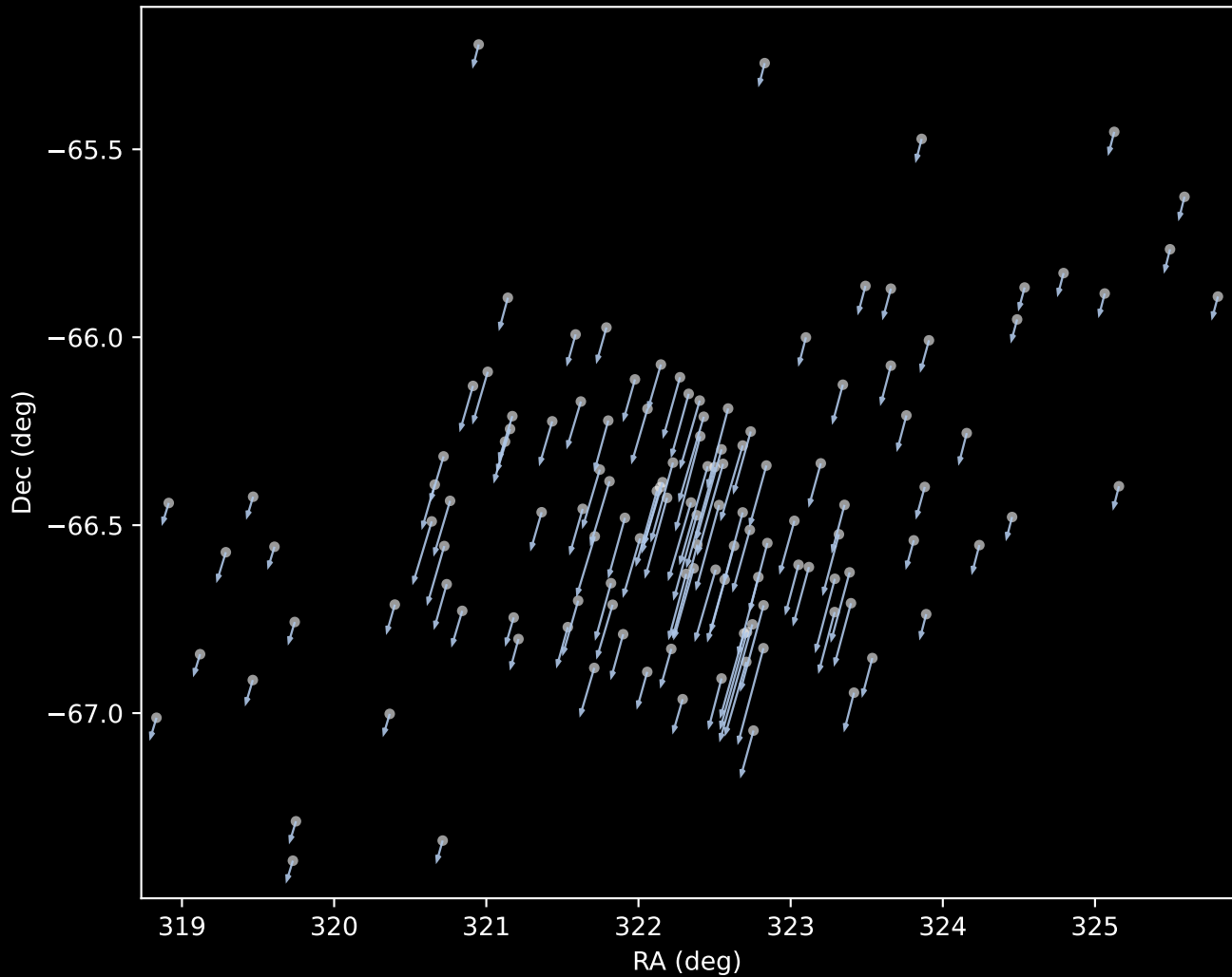
Gaia DR3 Cluster 1 Proper Motion Vectors (n=128)
