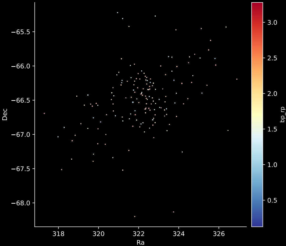
Gaia Cluster: [BH_164] Stars: 164
