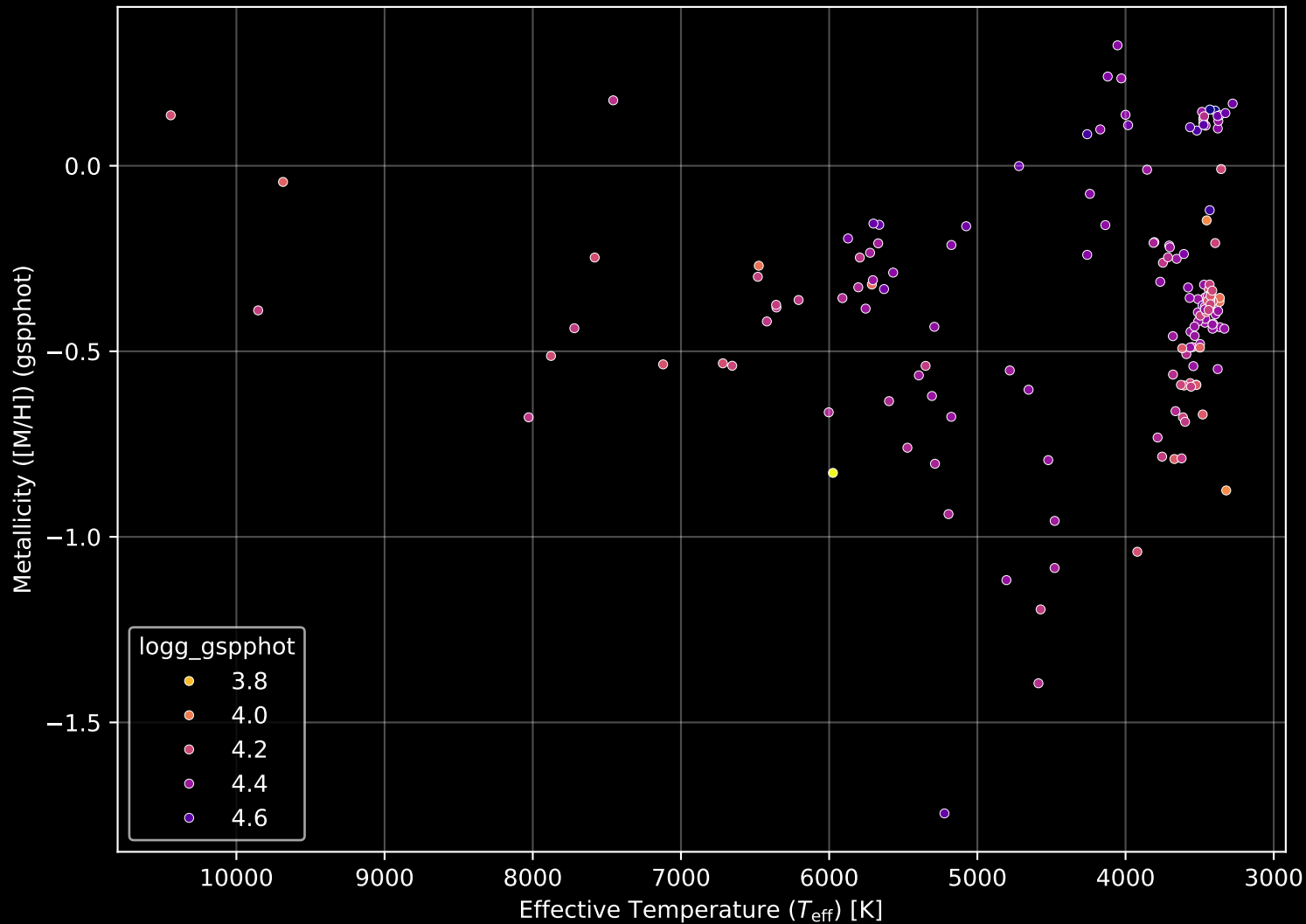
Gaia Cluster: [BH_164] Stellar Population Parameters (n= 164)
