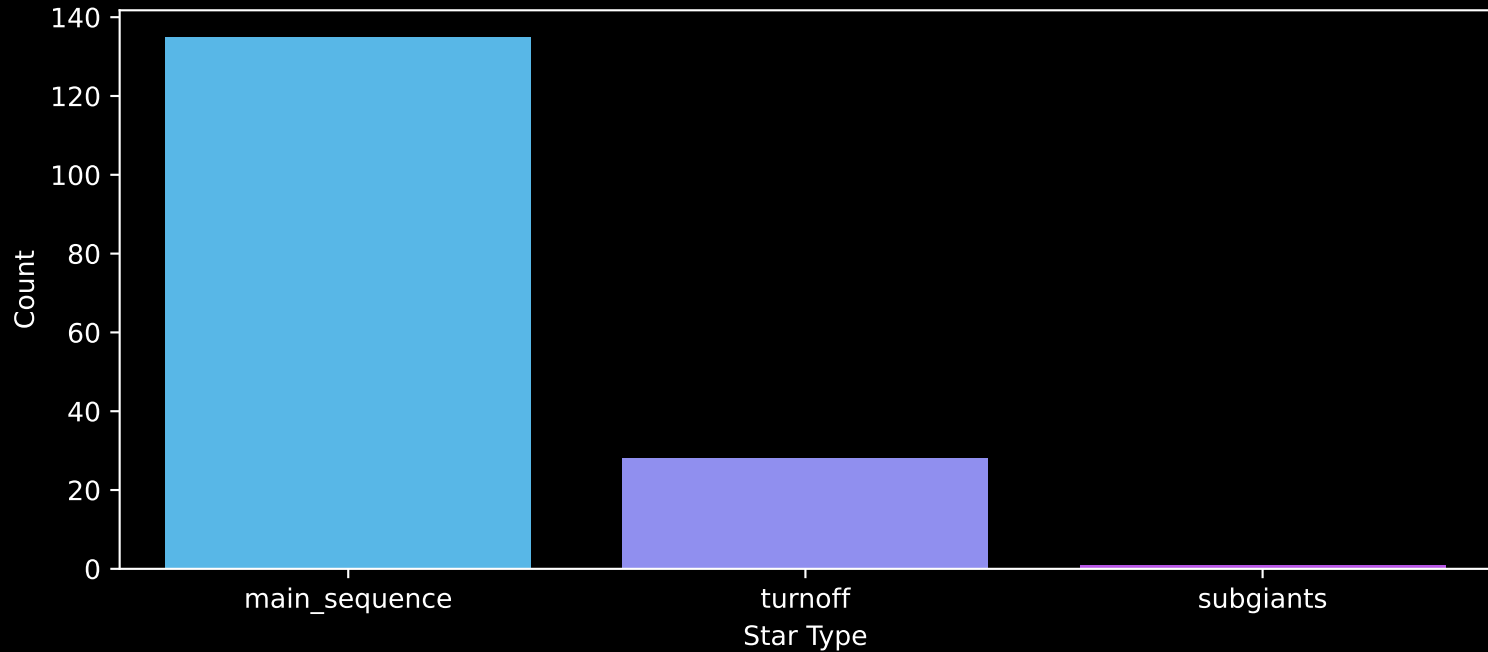
Gaia Cluster: [BH_164] Count plot of Star Type
