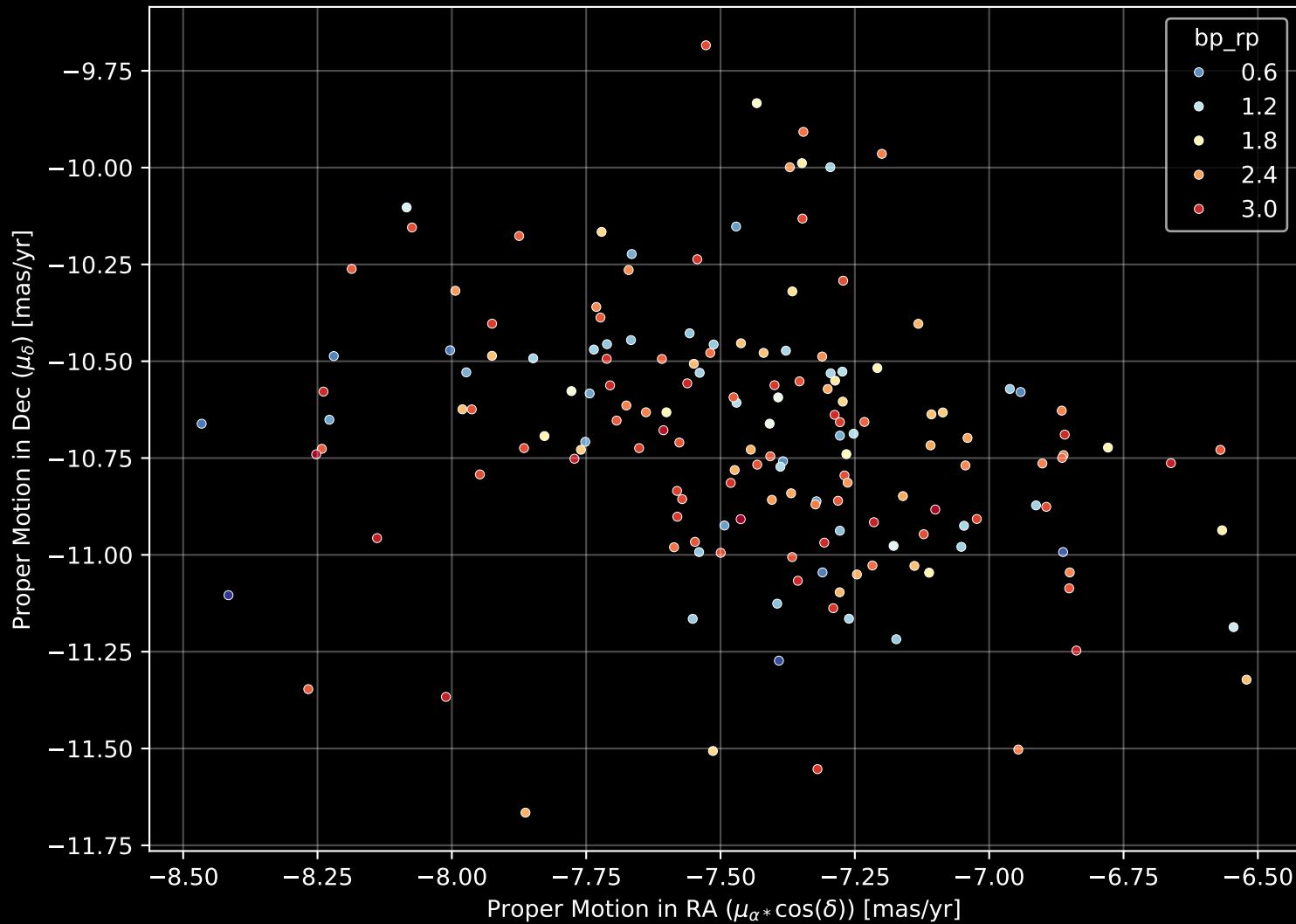
Gaia Cluster: [BH_164] Proper Motion Diagram (n= 164)
