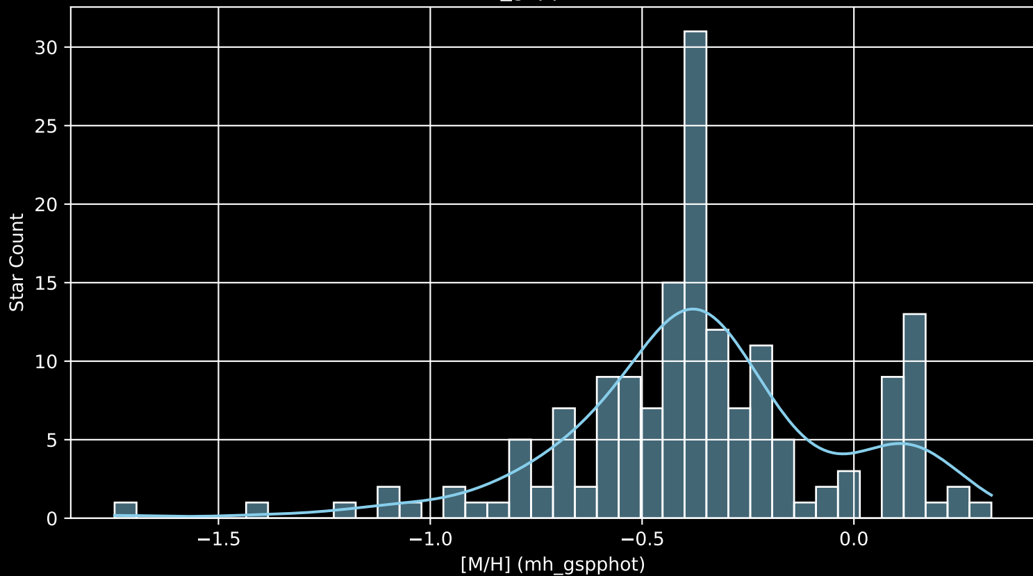
Gaia Cluster: [BH_164 [M/H] (mh_gspphot) (n= 164)
