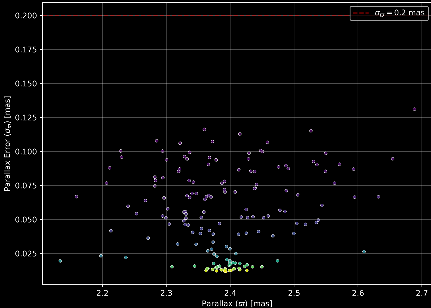
Gaia Cluster: [BH_164] Parallax Quality (n= 164)
