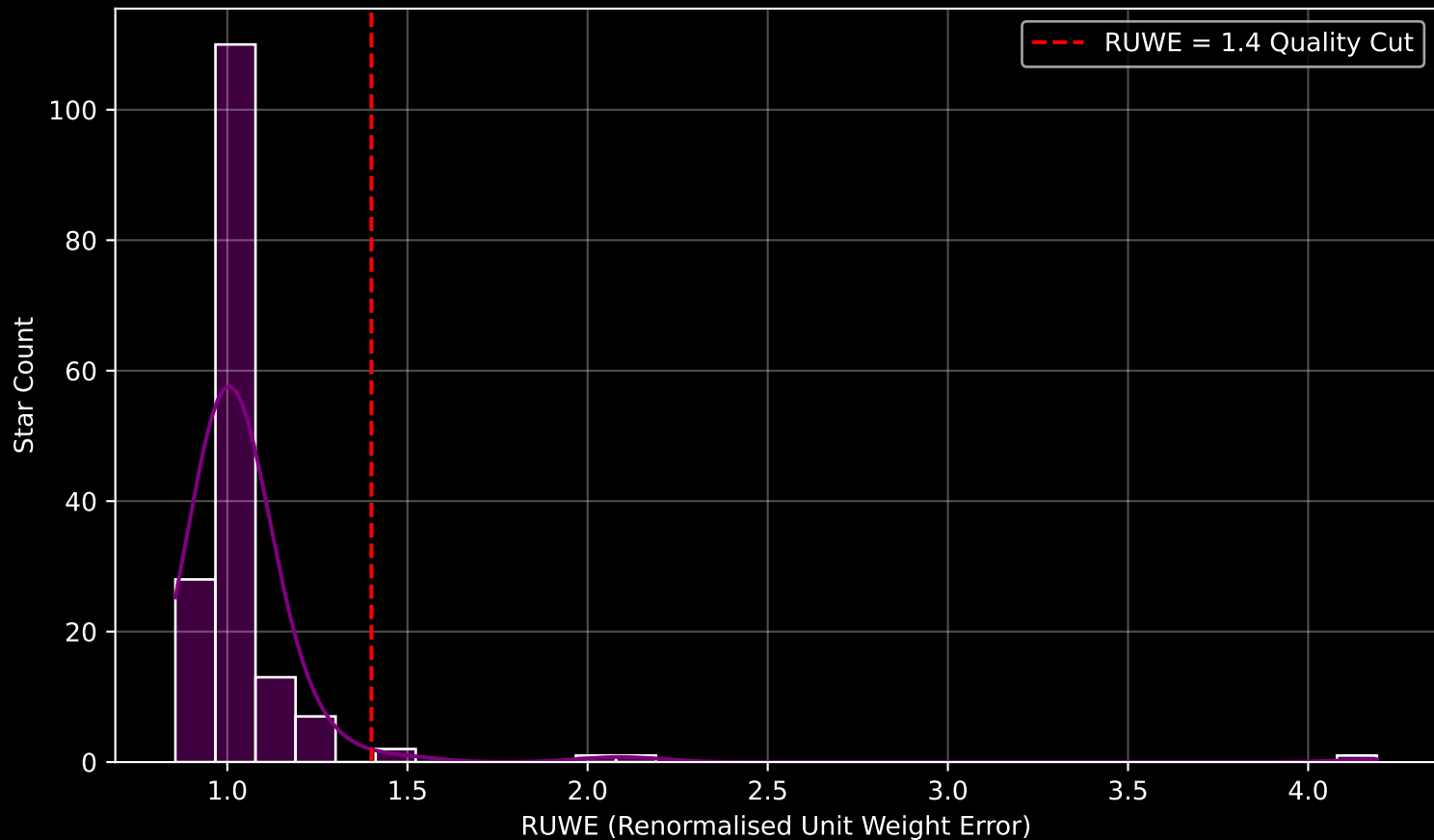
Gaia Cluster: [BH_164] RUWE Distribution (n= 163)
