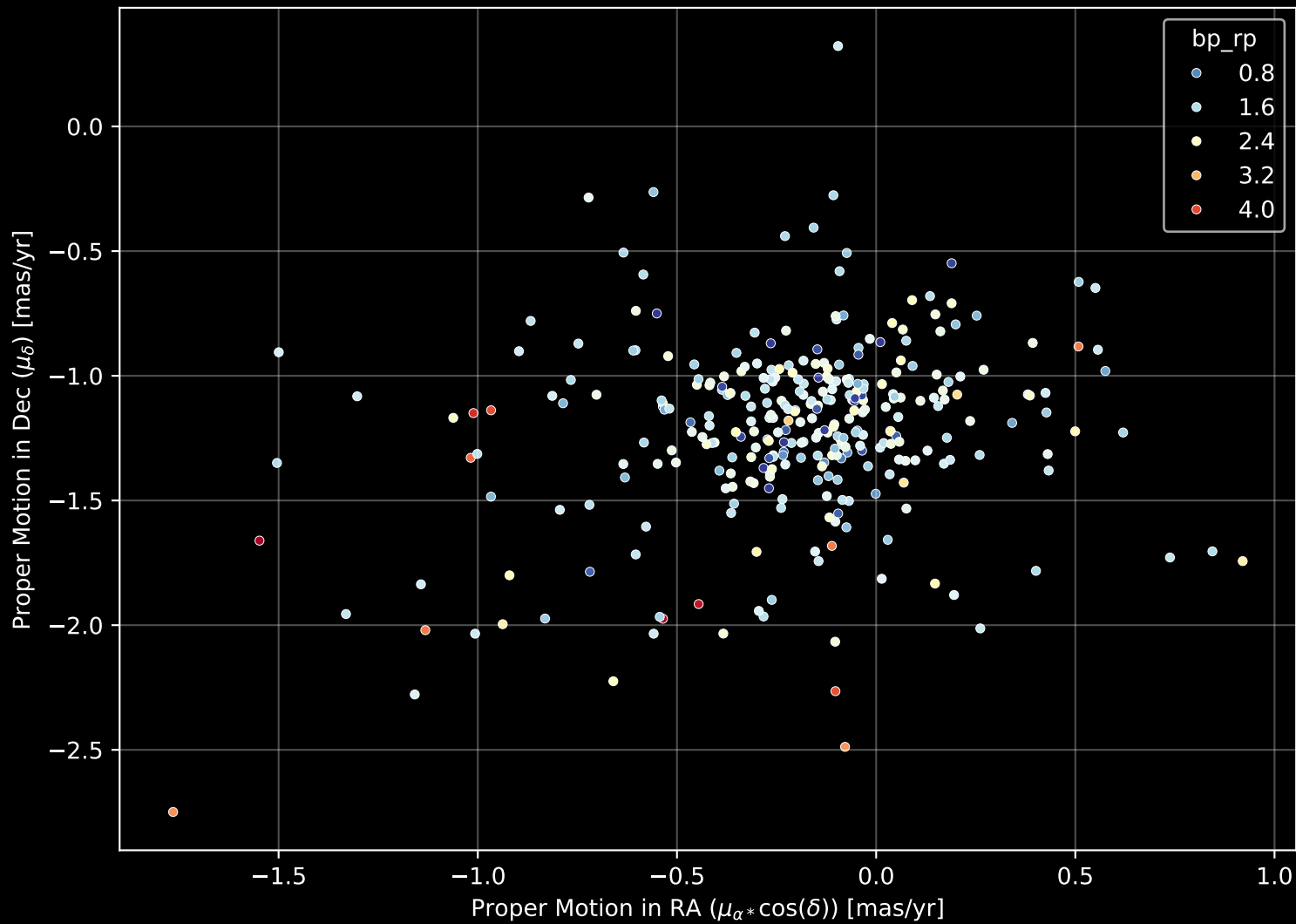
Gaia Cluster: [BH_205] Proper Motion Diagram (n= 317)
