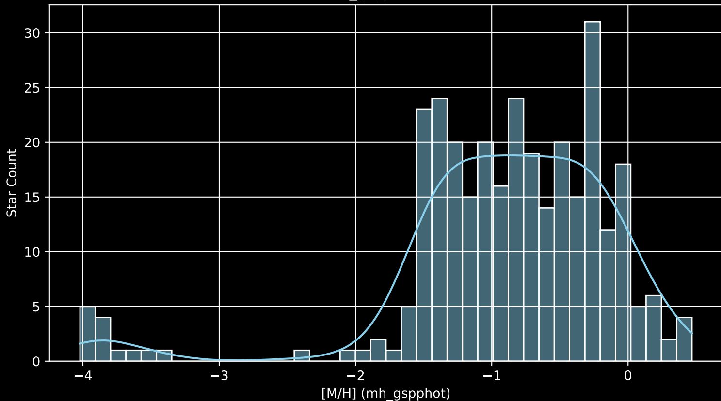
Gaia Cluster: [BH_205 [M/H] (mh_gspphot) (n= 312)
