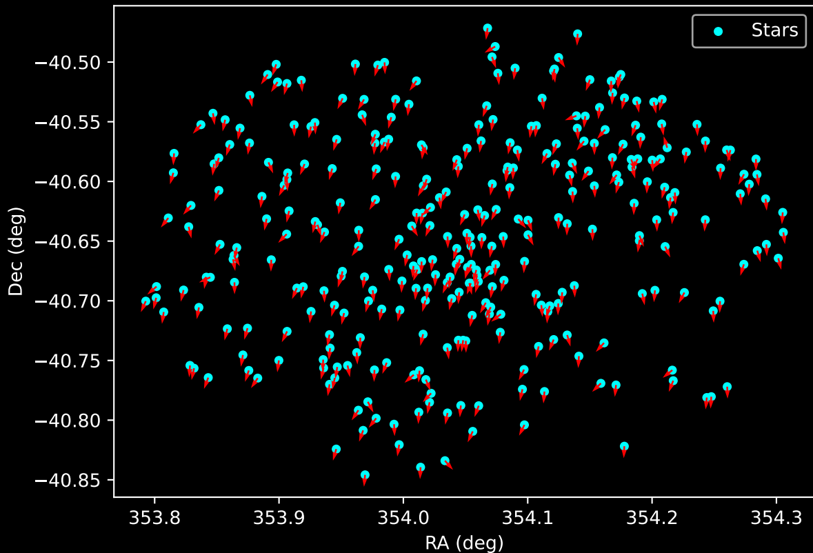
Gaia Cluster: [BH_205] Proper Motion Vectors for Gaia Star Field (n= 317)
