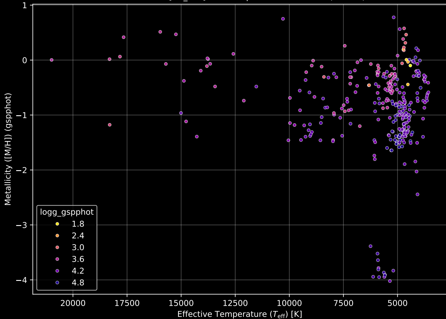
Gaia Cluster: [BH_205] Stellar Population Parameters (n= 317)
