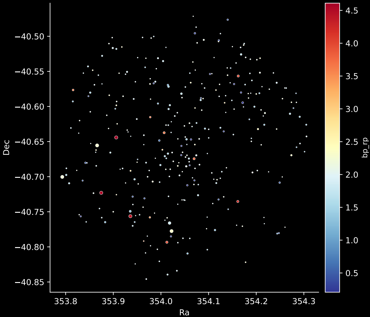
Gaia Cluster: [BH_205] Stars: 317
