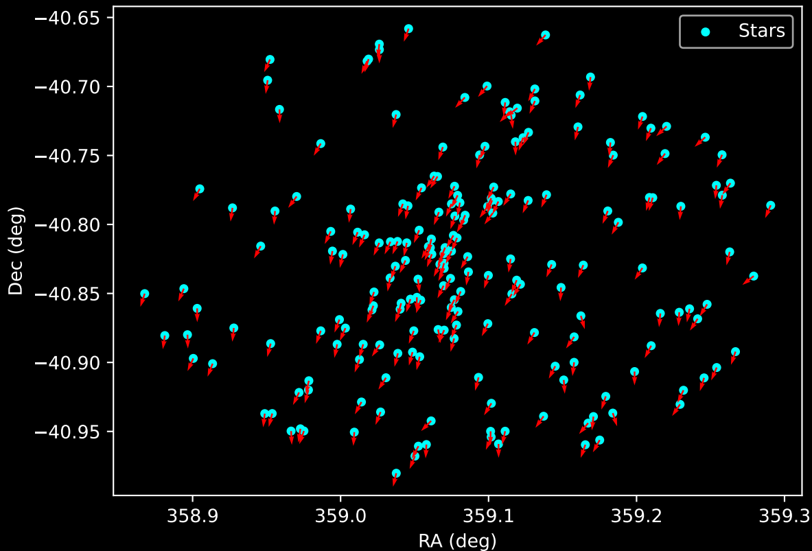
Gaia Cluster: [BH_217] Proper Motion Vectors for Gaia Star Field (n= 199)
