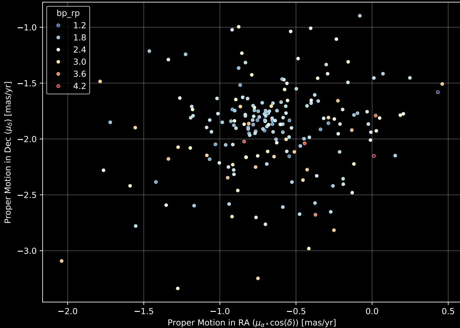
Gaia Cluster: [BH_217] Proper Motion Diagram (n= 199)
