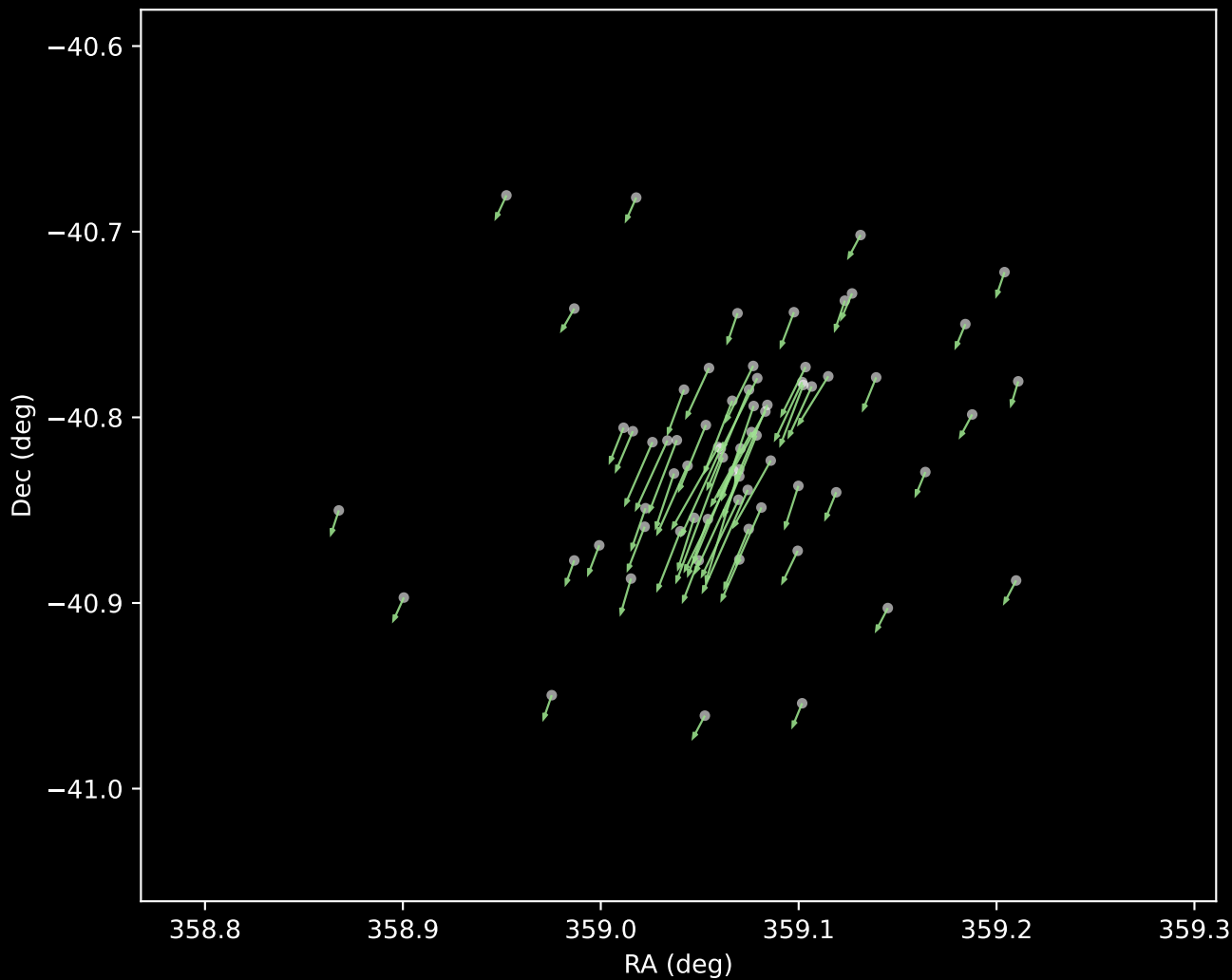
Gaia DR3 Cluster 5 Proper Motion Vectors (n=70)
