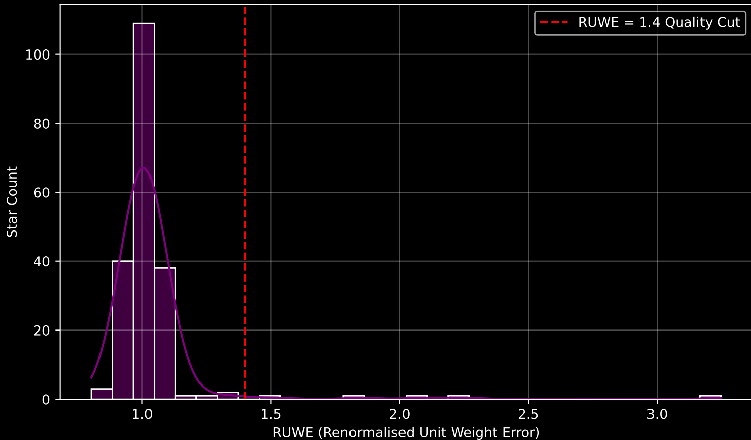
Gaia Cluster: [BH_217] RUWE Distribution (n= 199)
