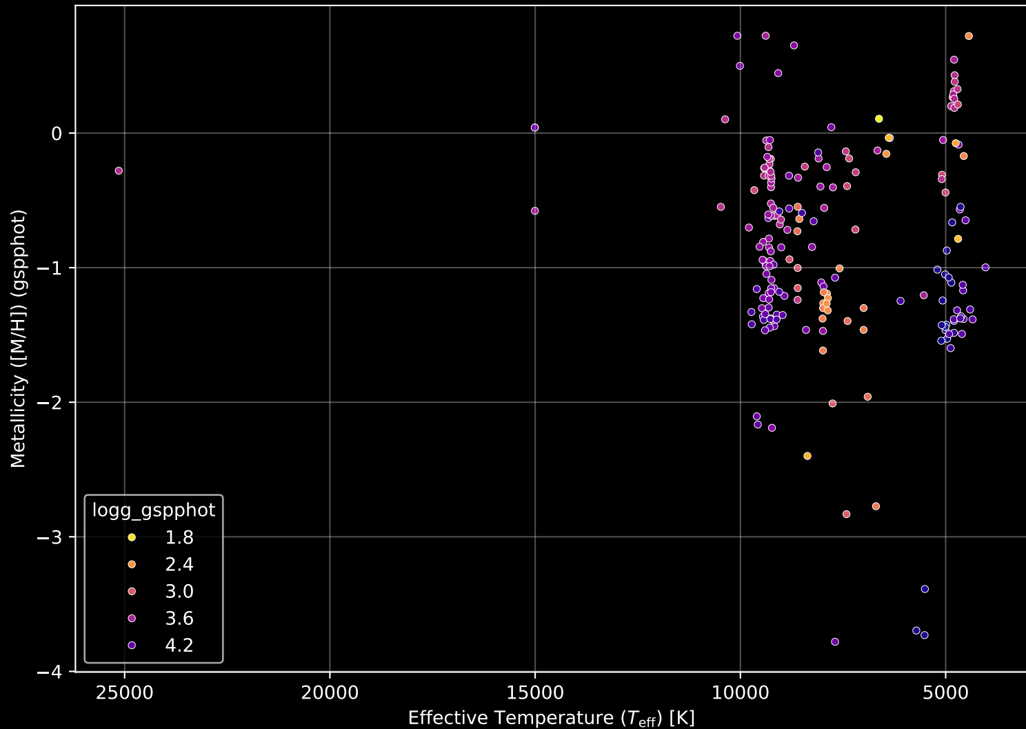
Gaia Cluster: [BH_217] Stellar Population Parameters (n= 199)
