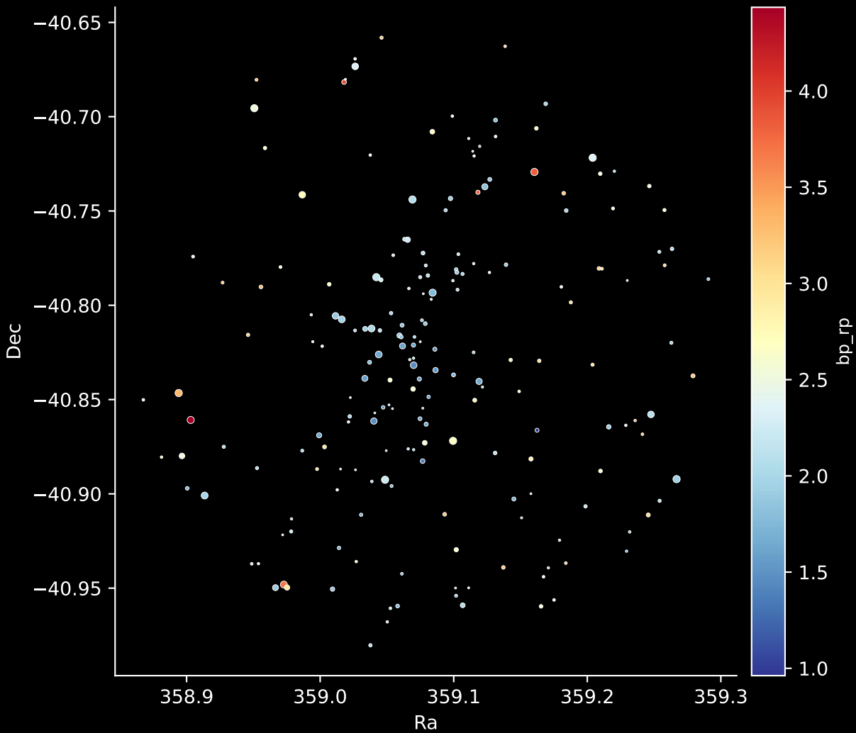
Gaia Cluster: [BH_217] Stars: 199
