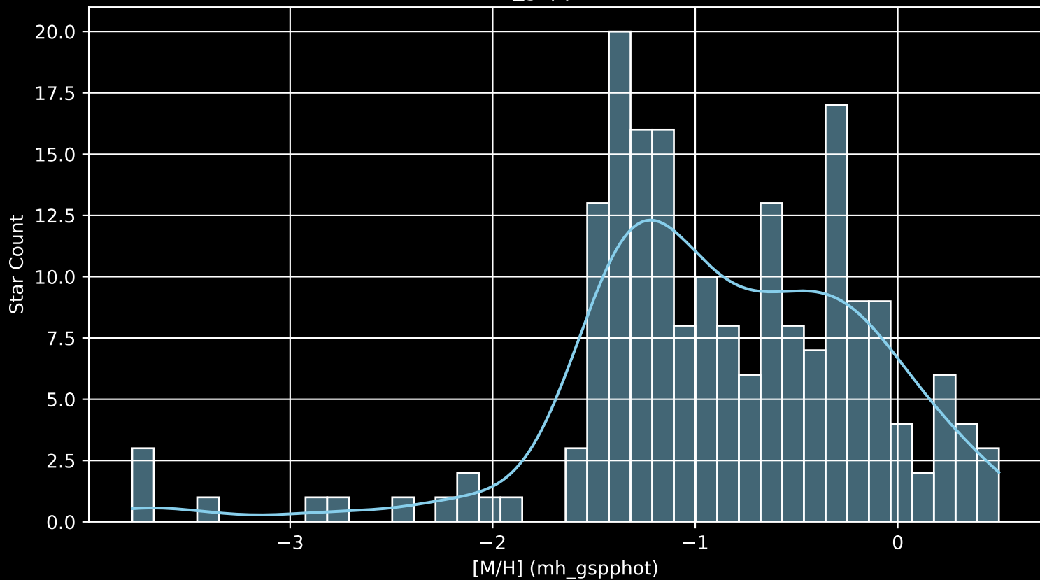
Gaia Cluster: [BH_217 [M/H] (mh_gspphot) (n= 194)
