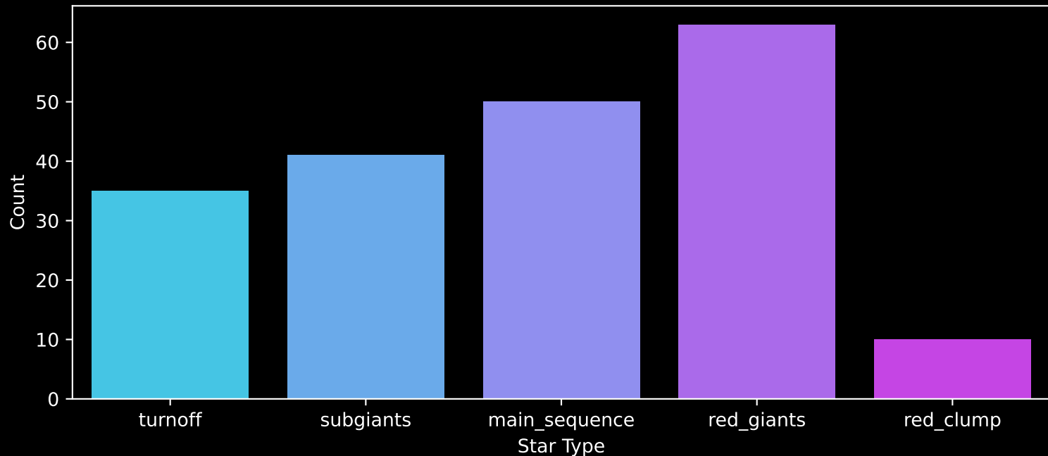
Gaia Cluster: [BH_217] Count plot of Star Type
