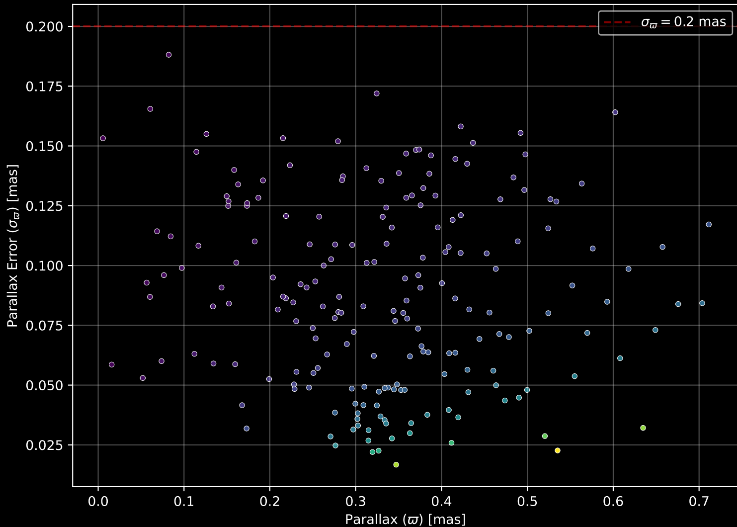
Gaia Cluster: [BH_217] Parallax Quality (n= 199)
