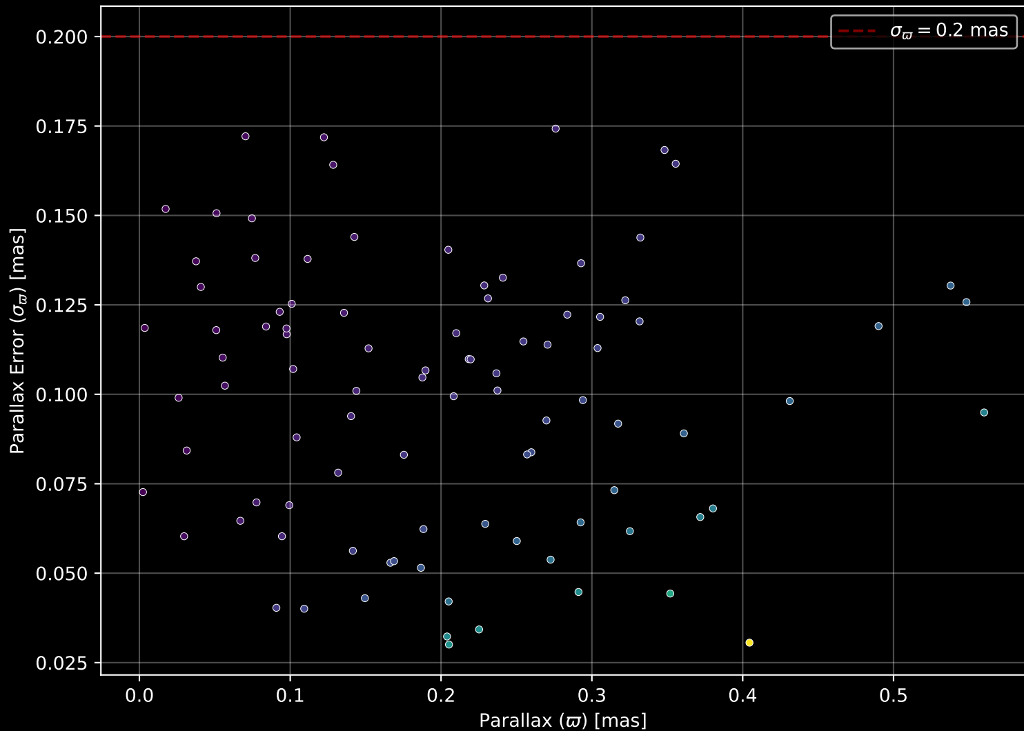
Gaia Cluster: [BH_222] Parallax Quality (n= 94)
