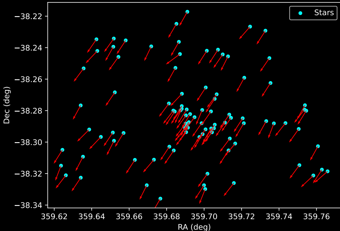
Gaia Cluster: [BH_222] Proper Motion Vectors for Gaia Star Field (n= 94)
