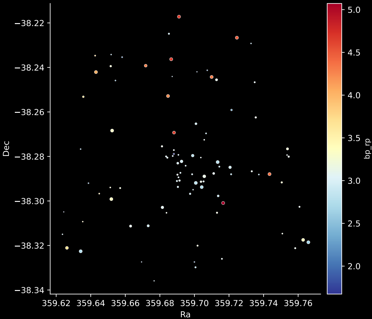
Gaia Cluster: [BH_222] Stars: 94
