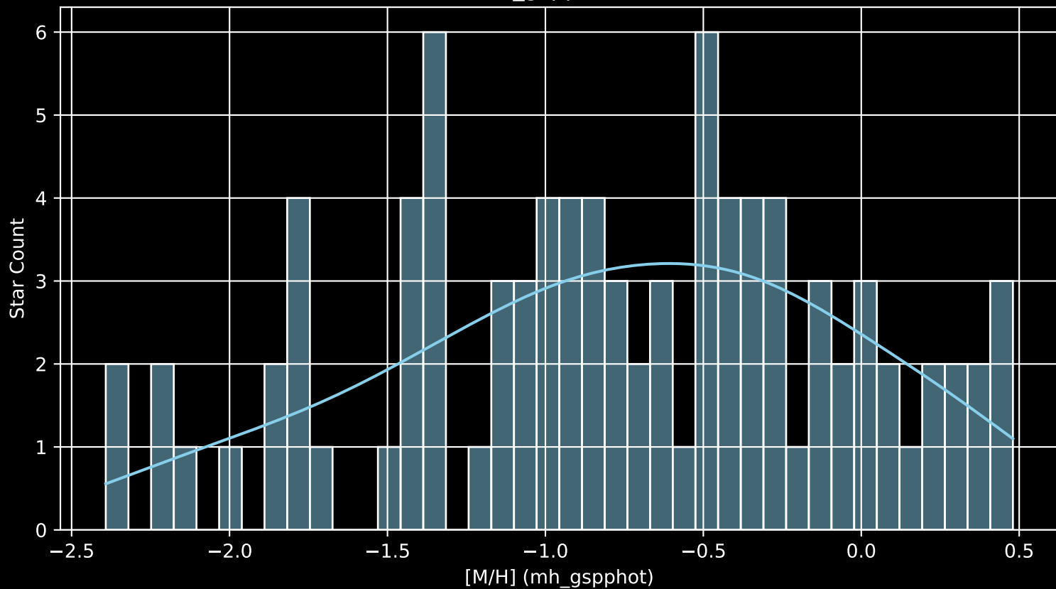
Gaia Cluster: [BH_222 [M/H] (mh_gspphot) (n= 91)
