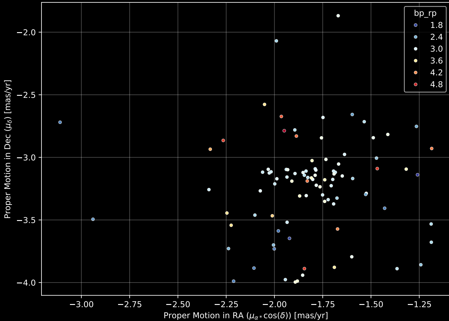
Gaia Cluster: [BH_222] Proper Motion Diagram (n= 94)
