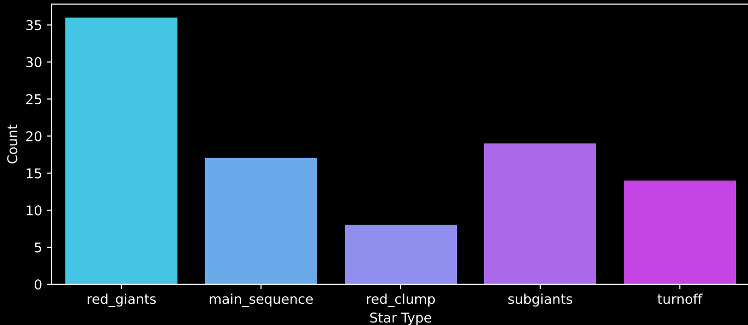
Gaia Cluster: [BH_222] Count plot of Star Type
