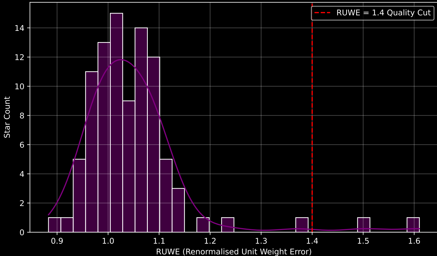
Gaia Cluster: [BH_222] RUWE Distribution (n= 94)
