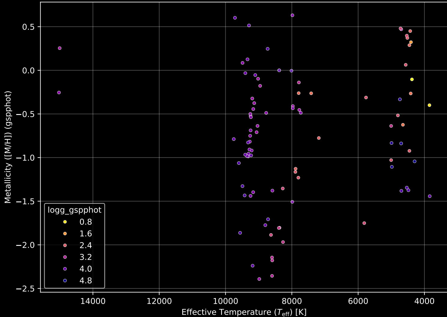
Gaia Cluster: [BH_222] Stellar Population Parameters (n= 94)
