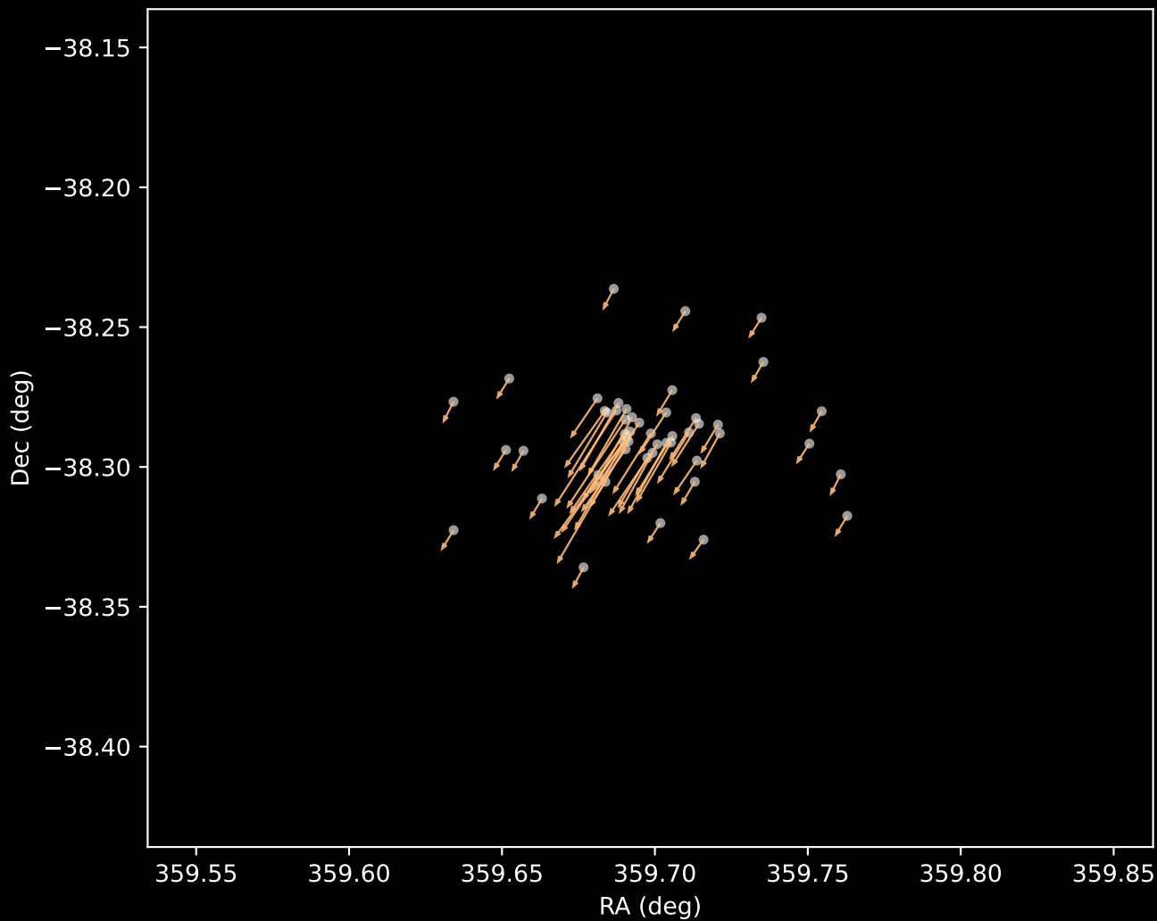
Gaia DR3 Cluster 3 Proper Motion Vectors (n=50)
