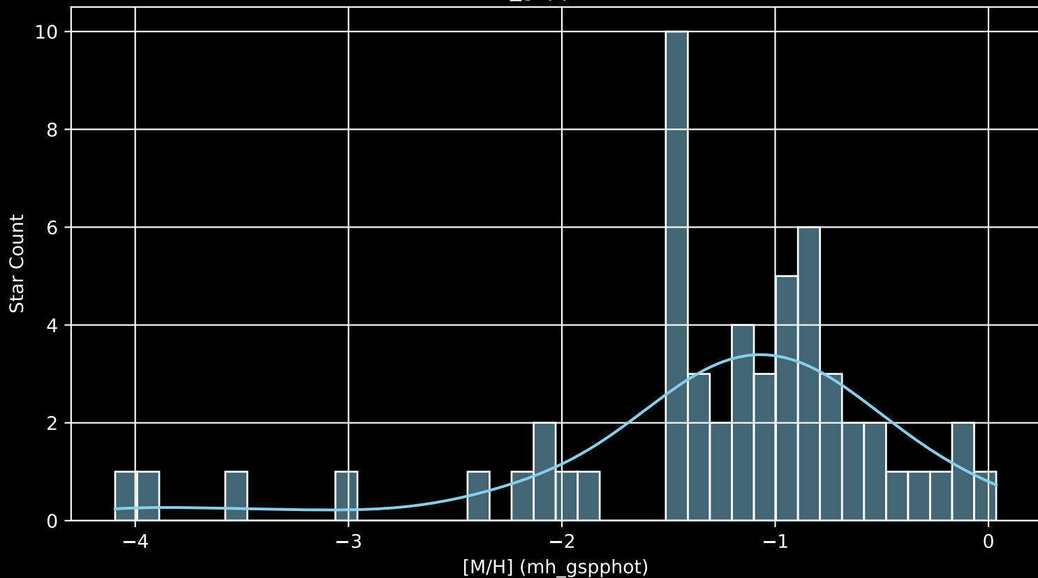
Gaia Cluster: [BH_37 [M/H] (mh_gspphot) (n= 56)
