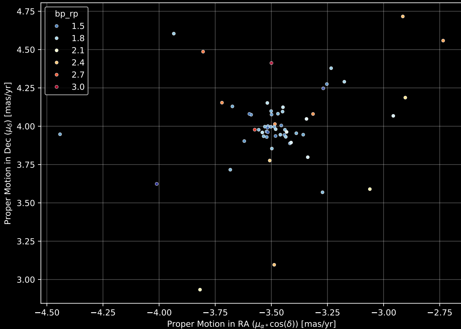
Gaia Cluster: [BH_37] Proper Motion Diagram (n= 59)
