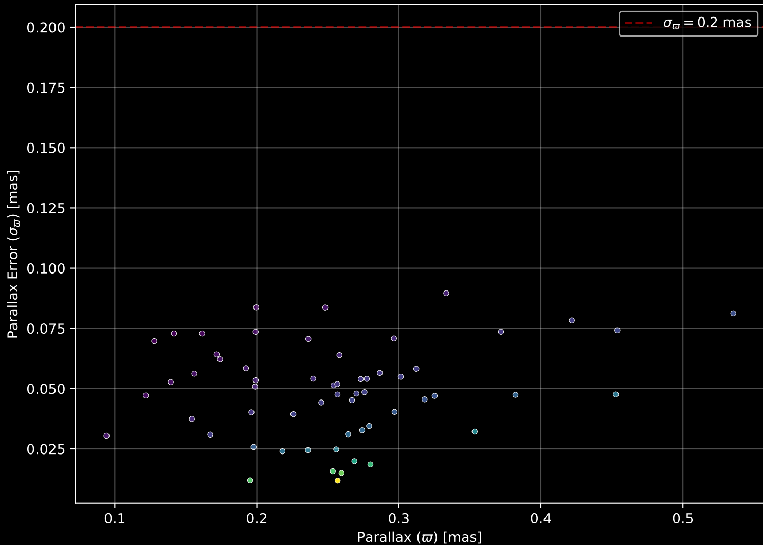
Gaia Cluster: [BH 37] Parallax Quality (n= 59)
