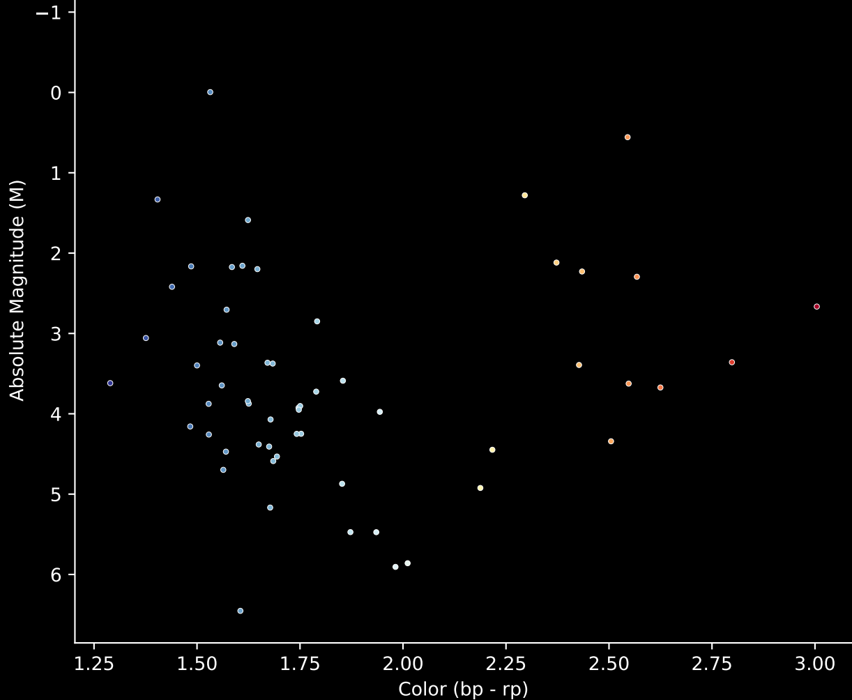
Gaia Cluster: [BH_37] Stars (n= 59) Hertzsprung-Russel Diagram
