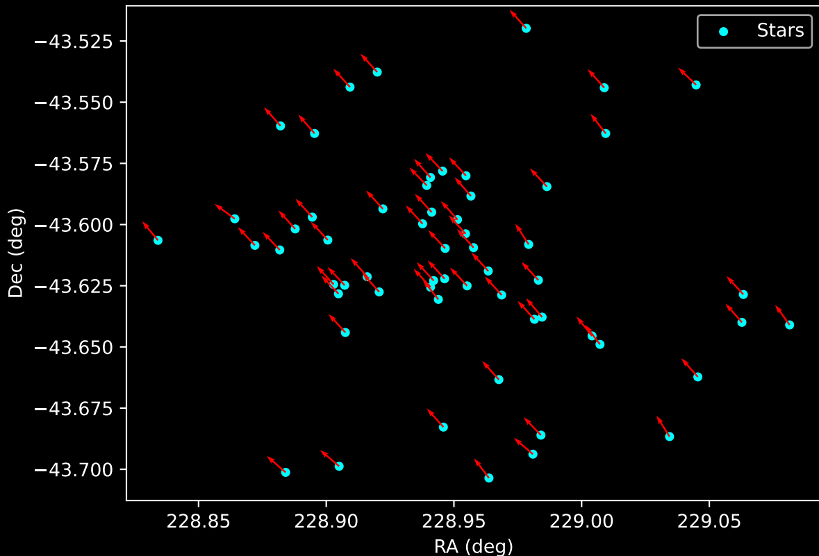
Gaia Cluster: [BH_37] Proper Motion Vectors for Gaia Star Field (n= 59)
