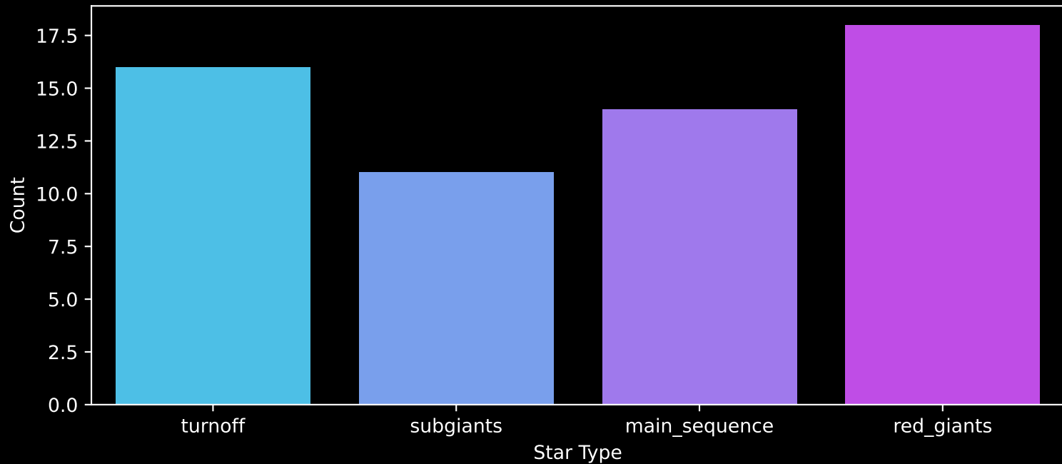
Gaia Cluster: [BH_37] Count plot of Star Type
