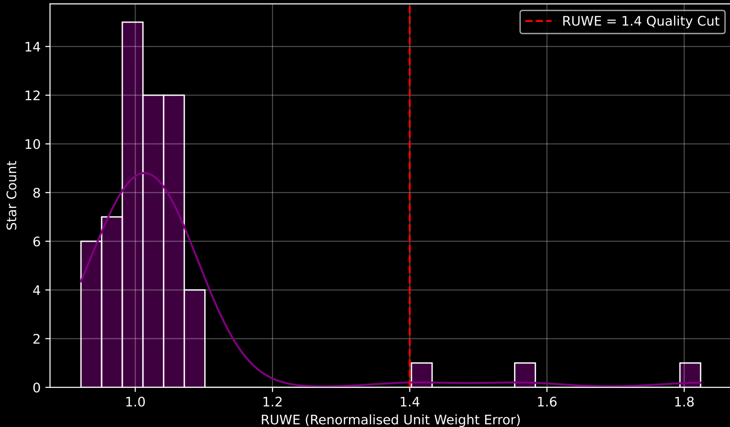
Gaia Cluster: [BH_37] RUWE Distribution (n= 59)
