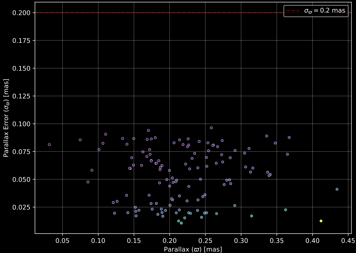
Gaia Cluster: [BH_55] Parallax Quality (n= 126)
