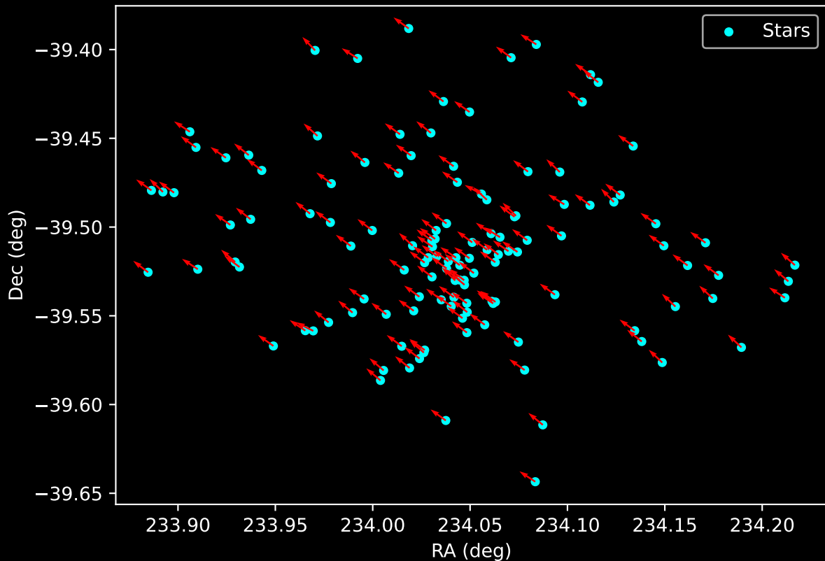
Gaia Cluster: [BH_55] Proper Motion Vectors for Gaia Star Field (n= 126)
