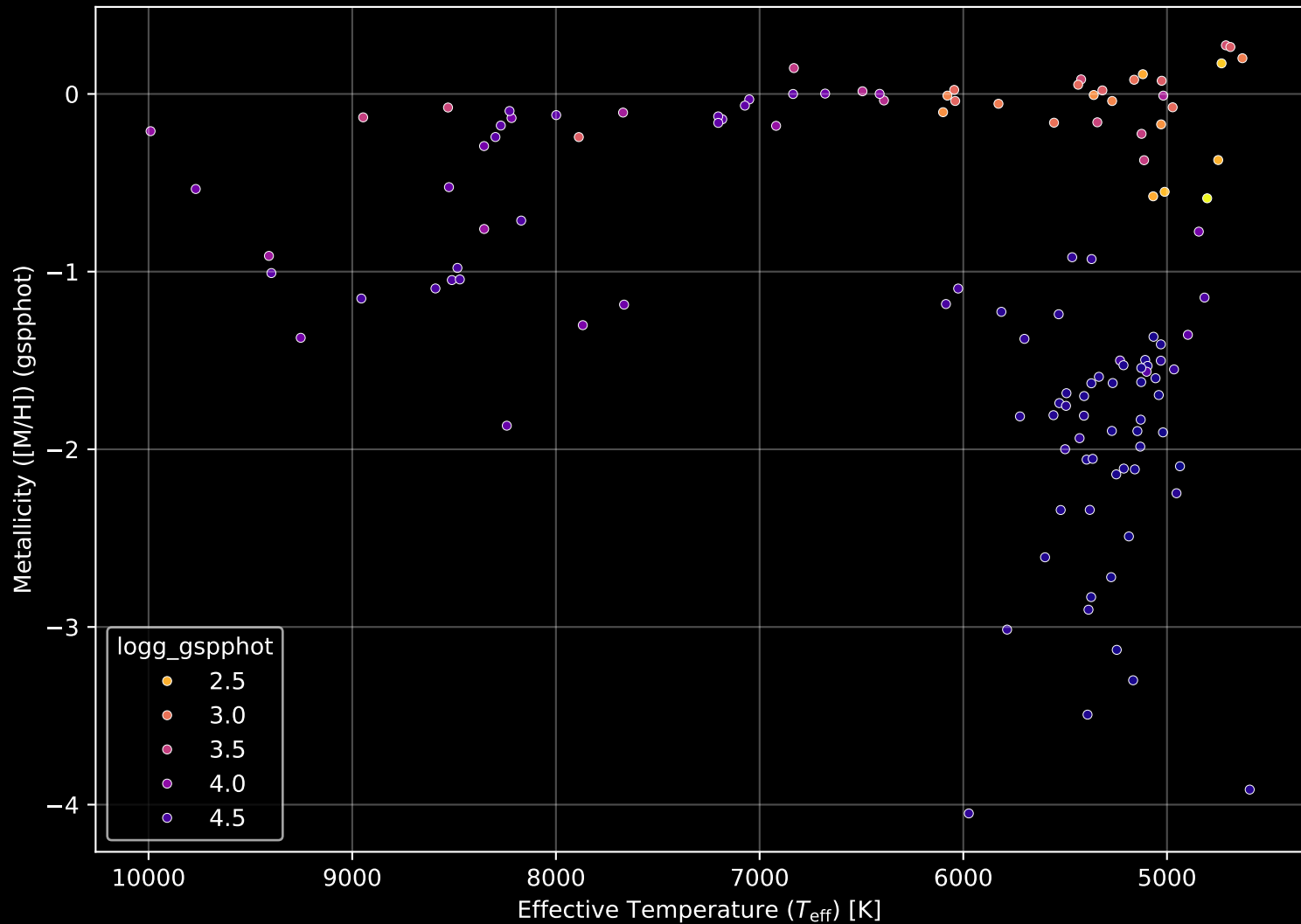
Gaia Cluster: [BH_55] Stellar Population Parameters (n= 126)
