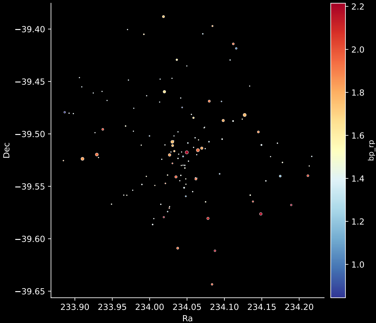
Gaia Cluster: [BH_55] Stars: 126
