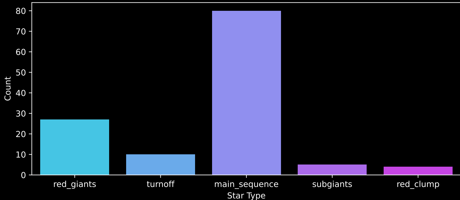
Gaia Cluster: [BH_55] Count plot of Star Type
