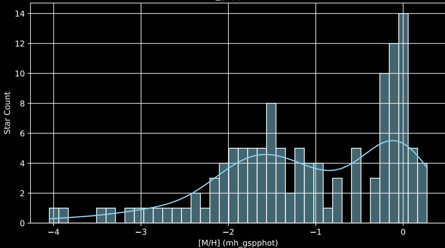
Gaia Cluster: [BH_55 [M/H] (mh_gspphot) (n= 126)
