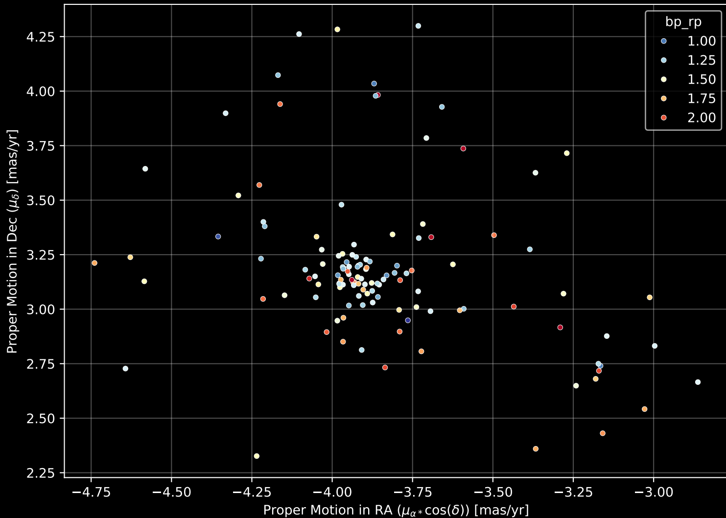
Gaia Cluster: [BH_55] Proper Motion Diagram (n= 126)
