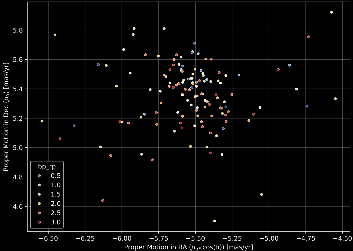
Gaia Cluster: [BH_56] Proper Motion Diagram (n= 133)
