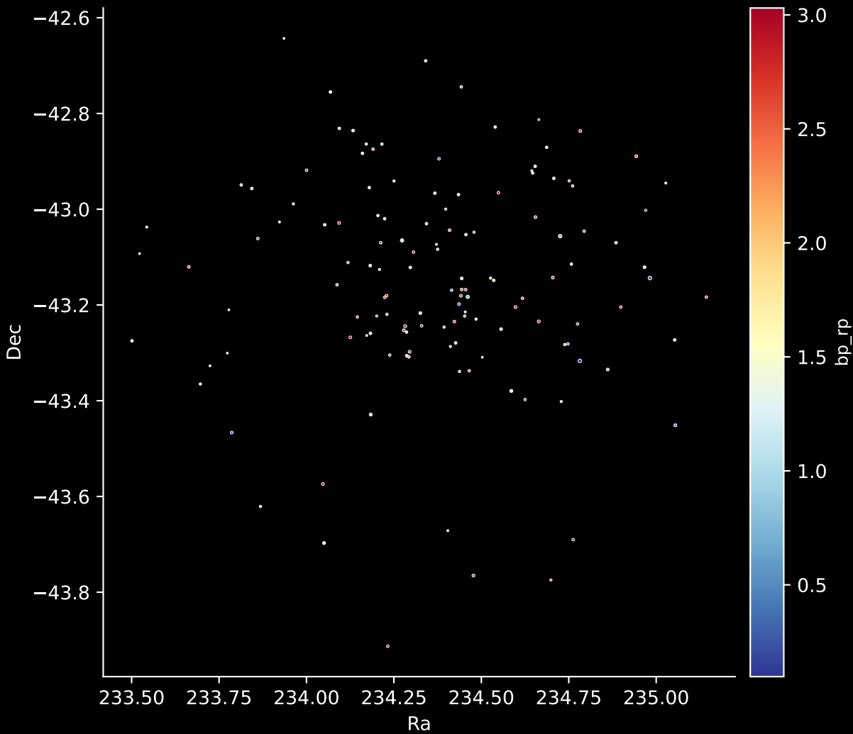
Gaia Cluster: [BH_56] Stars: 133
