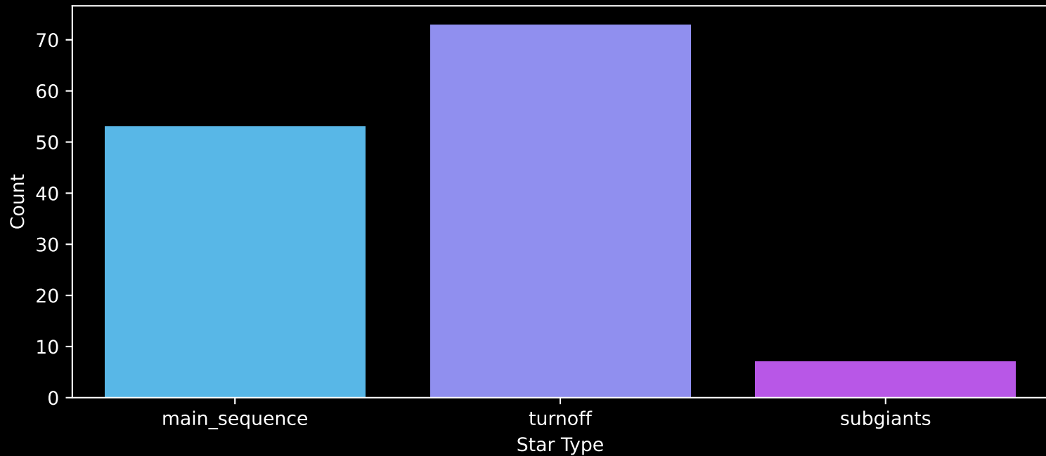
Gaia Cluster: [BH_56] Count plot of Star Type
