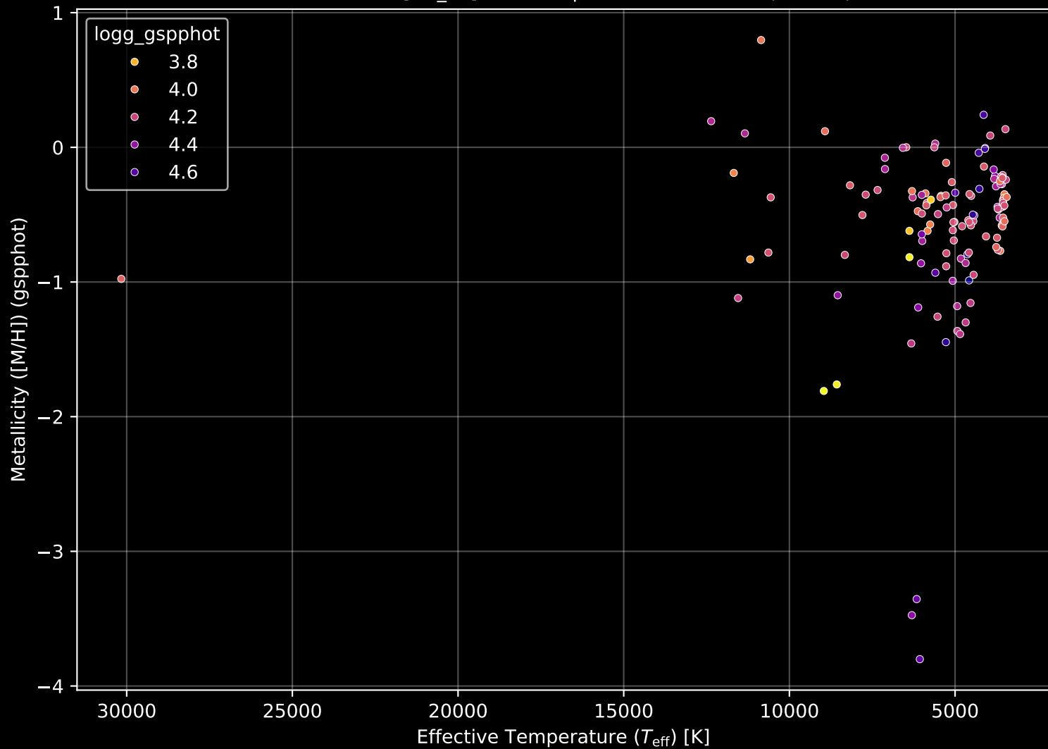
Gaia Cluster: [BH_56] Stellar Population Parameters (n= 133)
