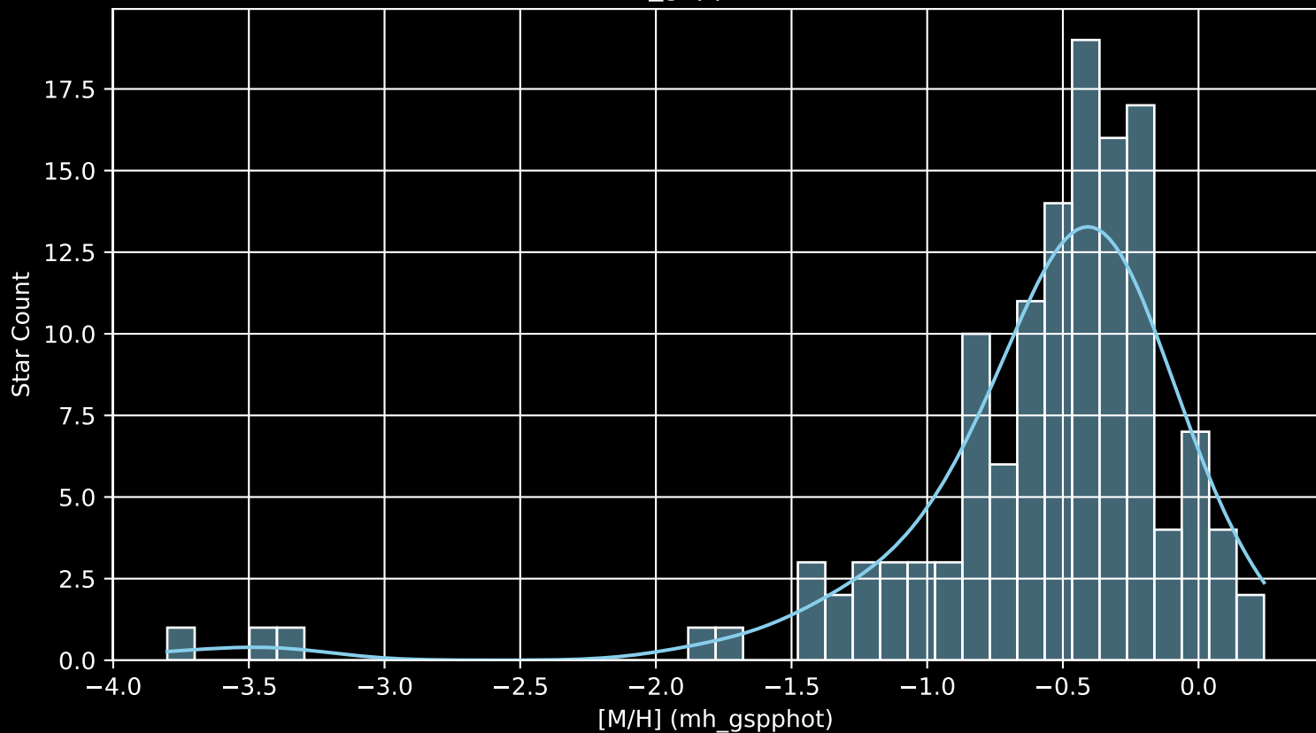
Gaia Cluster: [BH_56 [M/H] (mh_gspphot) (n= 132)
