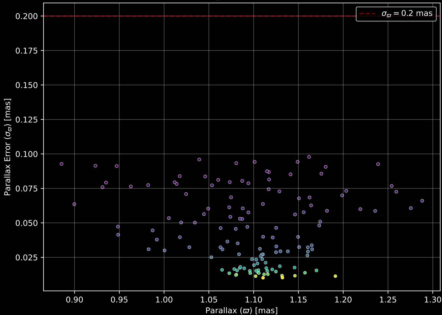
Gaia Cluster: [BH_56] Parallax Quality (n= 133)
