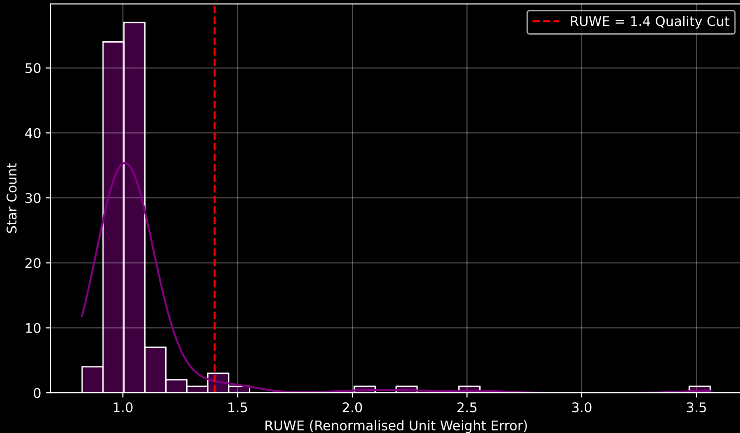
Gaia Cluster: [BH_56] RUWE Distribution (n= 133)
