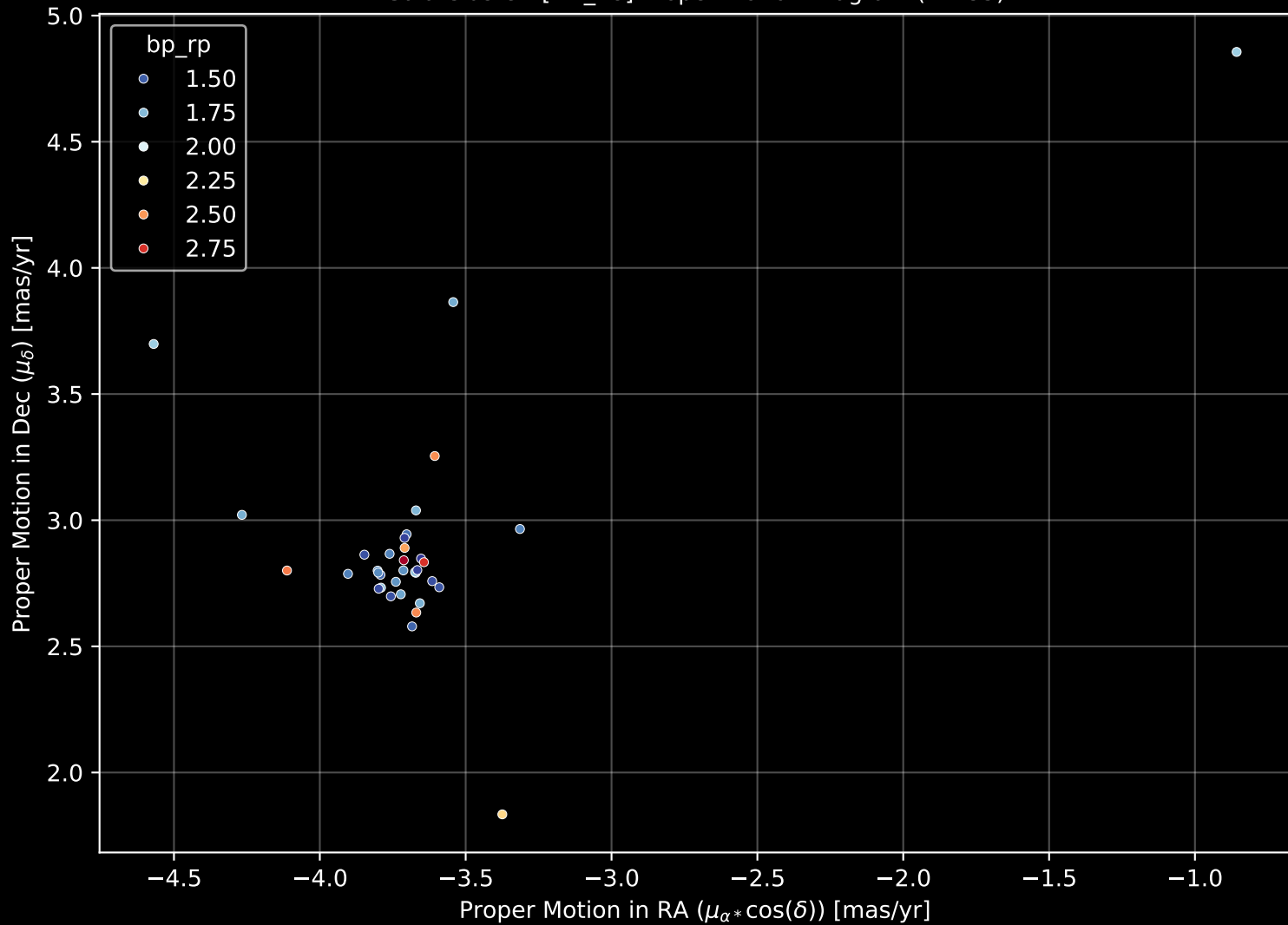
Gaia Cluster: [BH 78] Proper Motion Diagram (n= 35)
