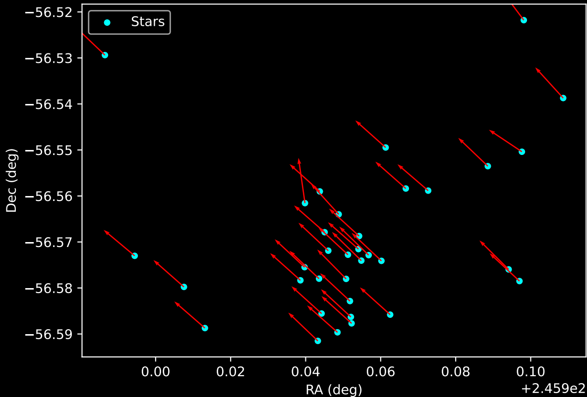
Gaia Cluster: [BH_78] Proper Motion Vectors for Gaia Star Field (n= 35)
