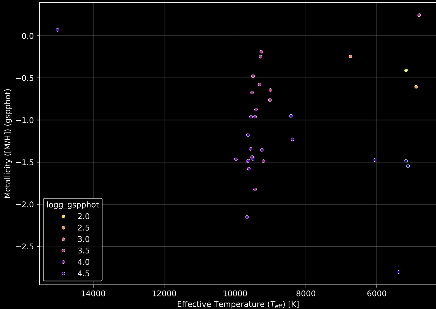
Gaia Cluster: [BH_78] Stellar Population Parameters (n= 35)
