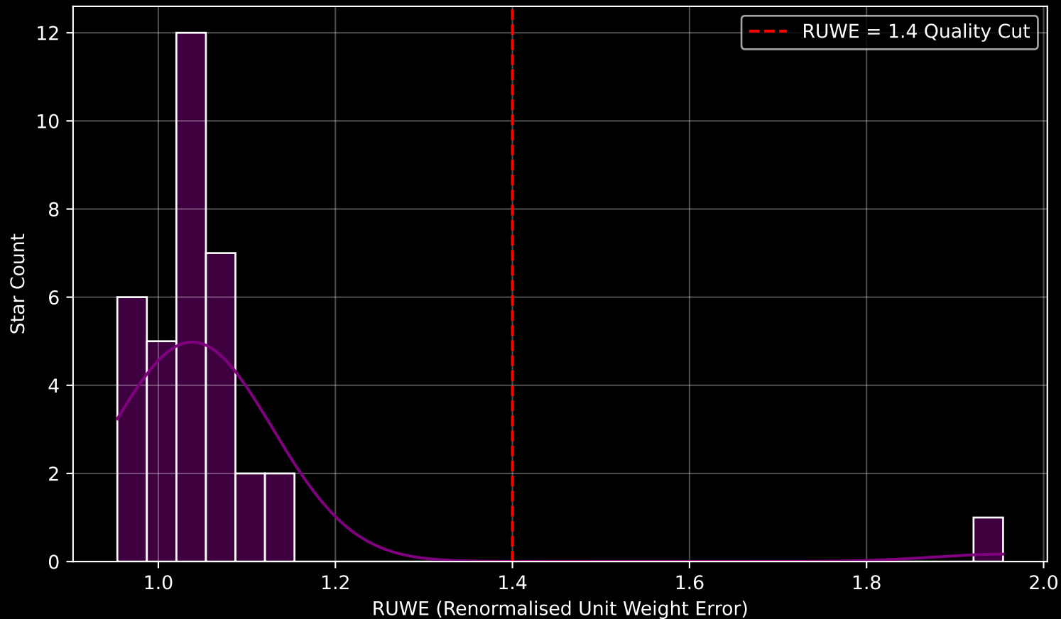
Gaia Cluster: [BH_78] RUWE Distribution (n= 35)
