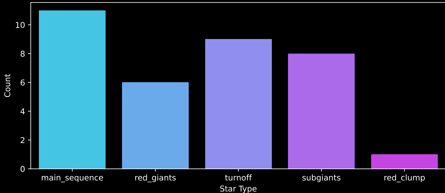
Gaia Cluster: [BH_78] Count plot of Star Type
