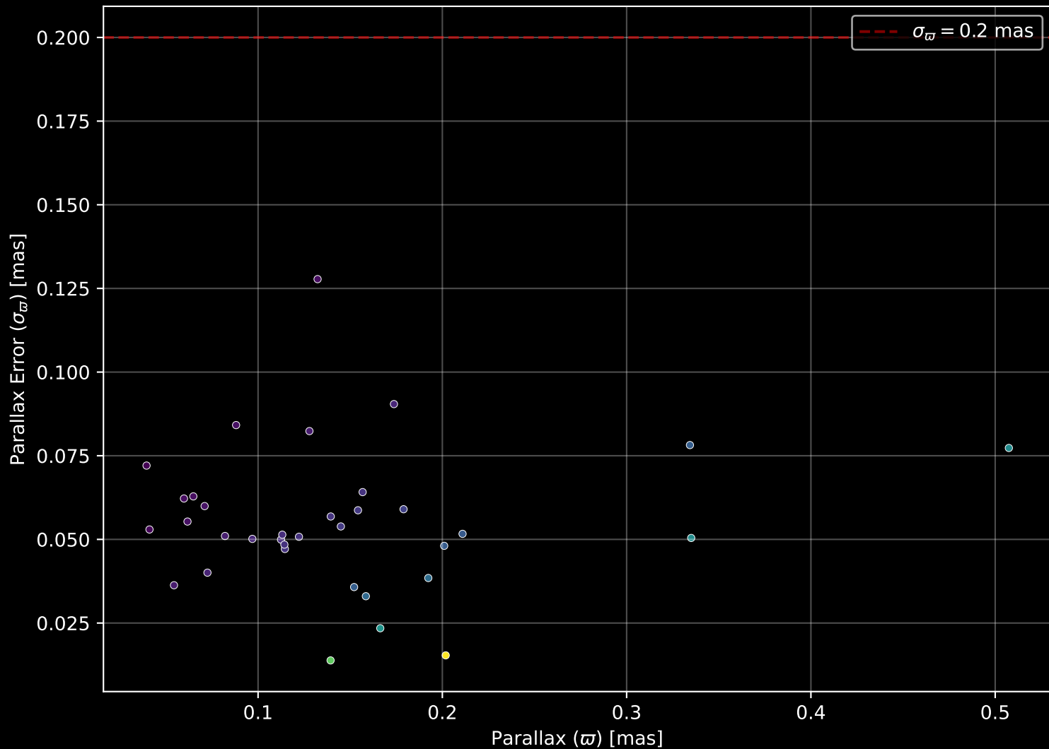
Gaia Cluster: [BH_78] Parallax Quality (n= 35)
