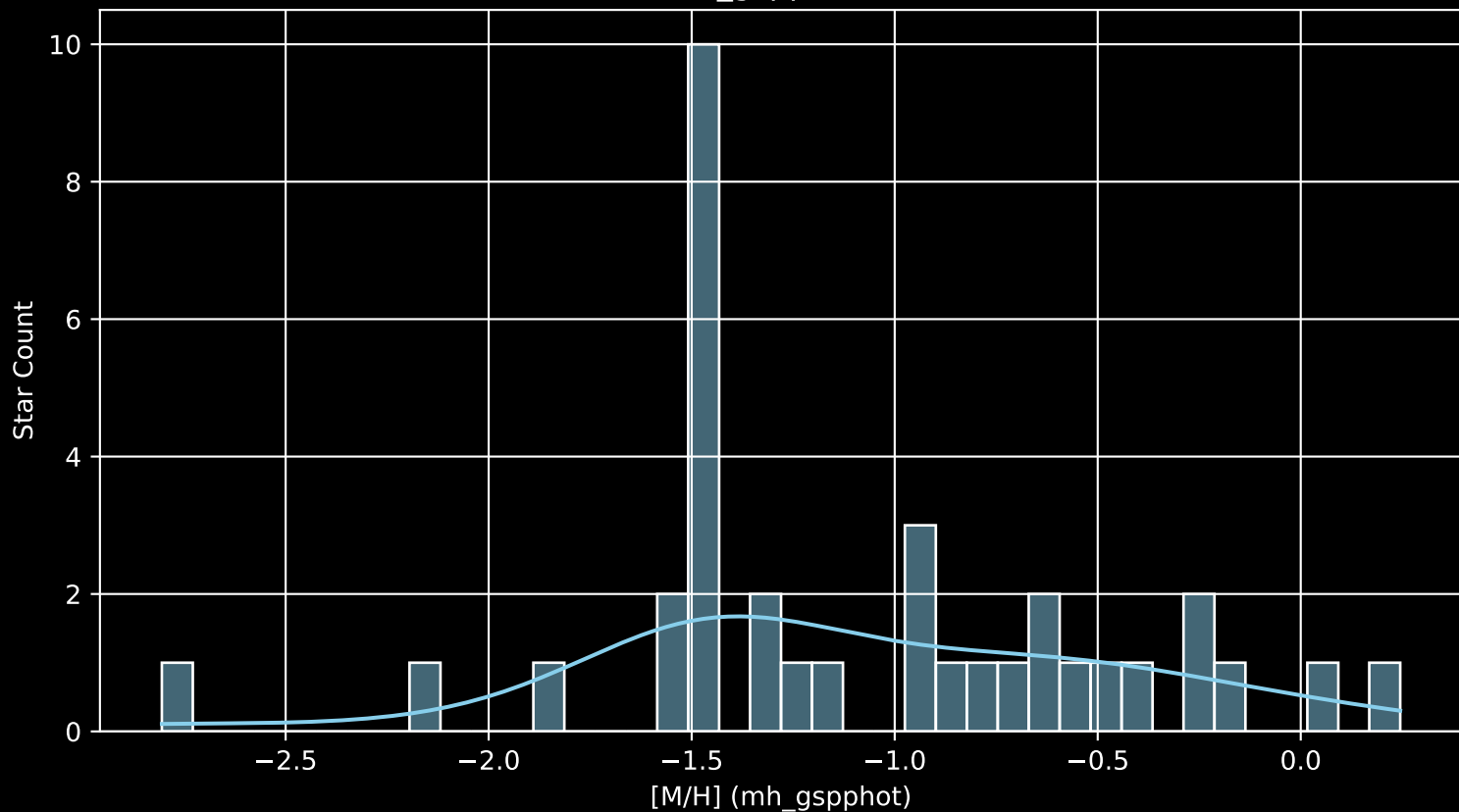
Gaia Cluster: [BH_78 [M/H] (mh_gspphot) (n= 35)
