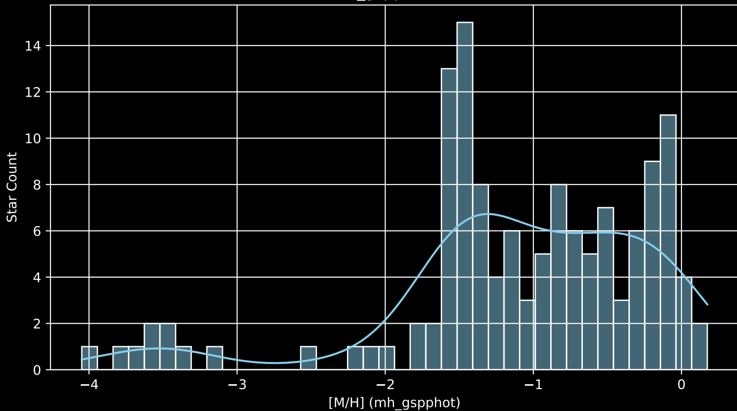
Gaia Cluster: [BH_84 [M/H] (mh_gspphot) ( \bar{n}= 132 )
