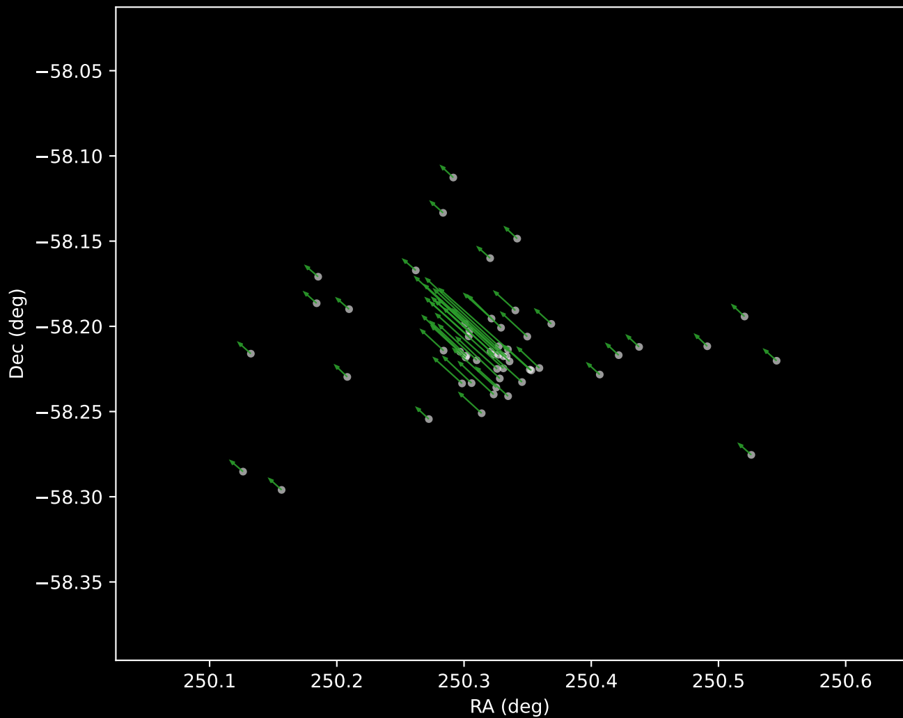
Gaia DR3 Cluster 4 Proper Motion Vectors (n=54)
