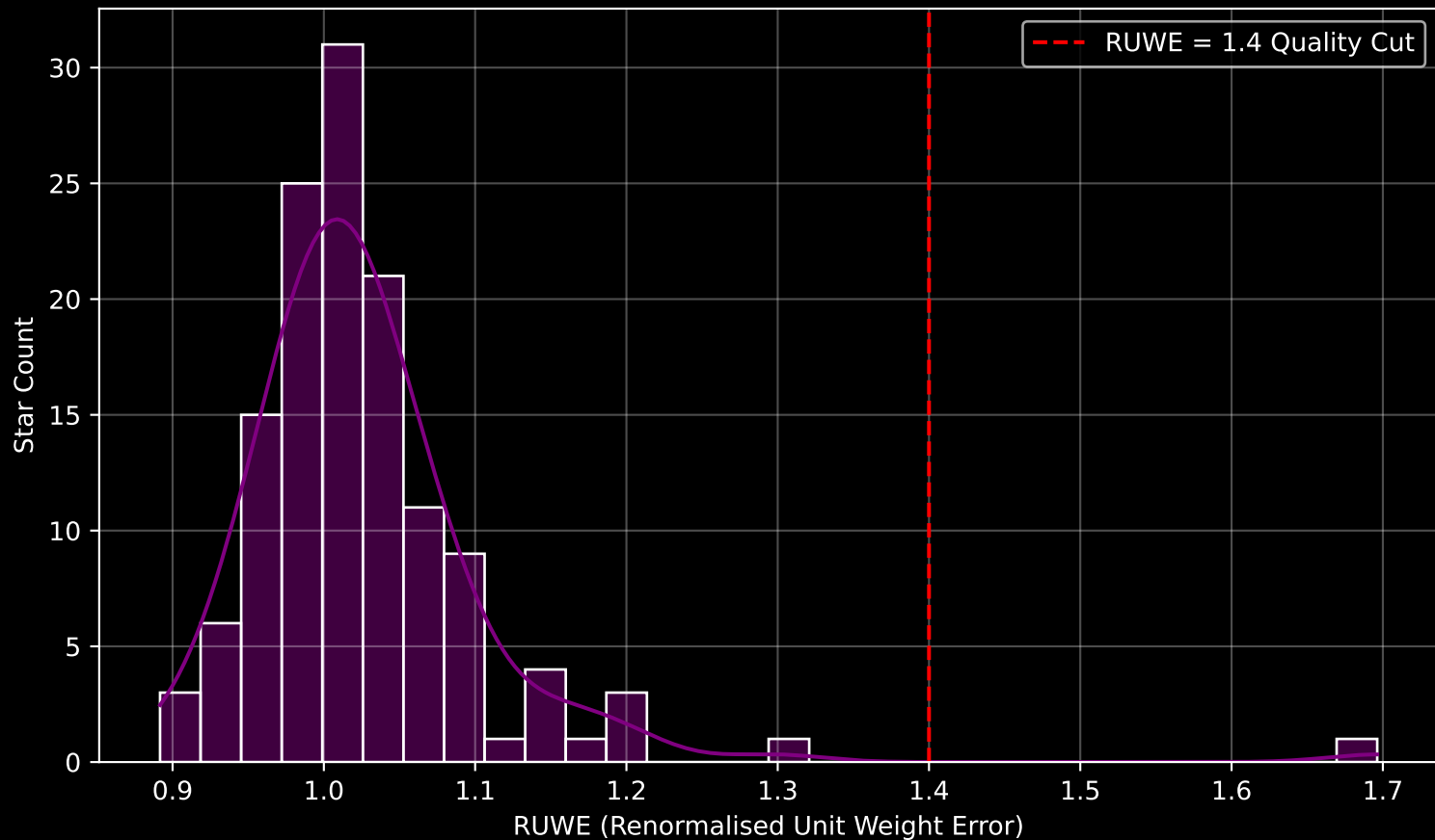
Gaia Cluster: [BH_84] RUWE Distribution (n= 132)
