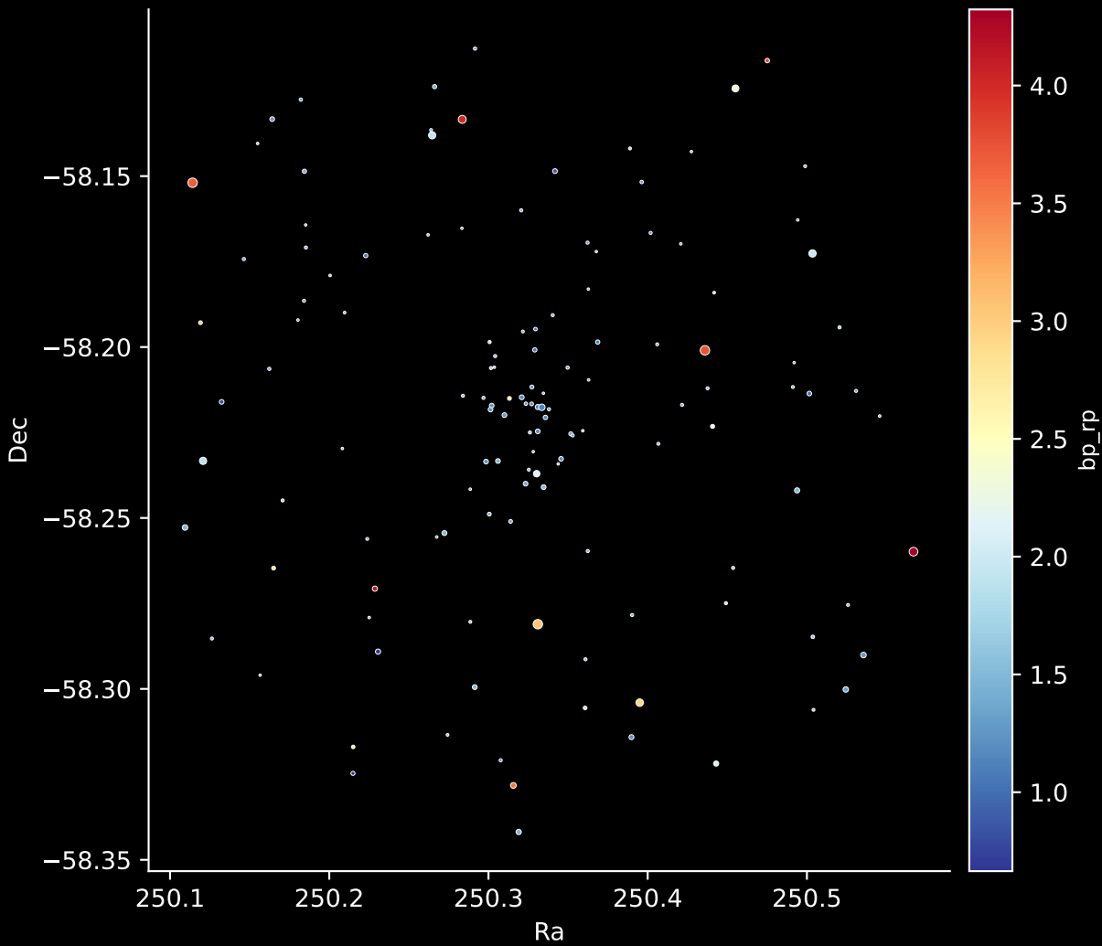
Gaia Cluster: [BH_84] Stars: 132
