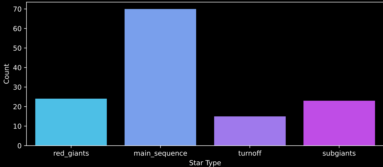
Gaia Cluster: [BH_84] Count plot of Star Type
