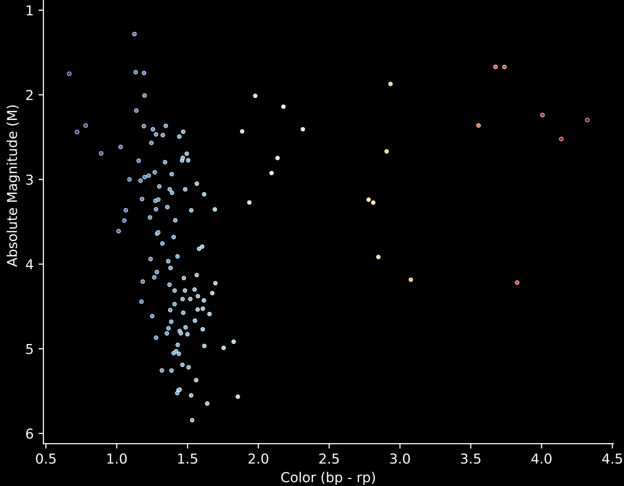
Gaia Cluster: [BH_84] Stars (n= 132) Hertzsprung-Russel Diagram
