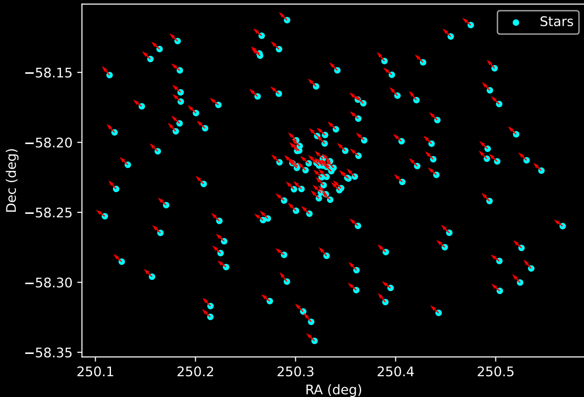
Gaia Cluster: [BH_84] Proper Motion Vectors for Gaia Star Field (n= 132)
