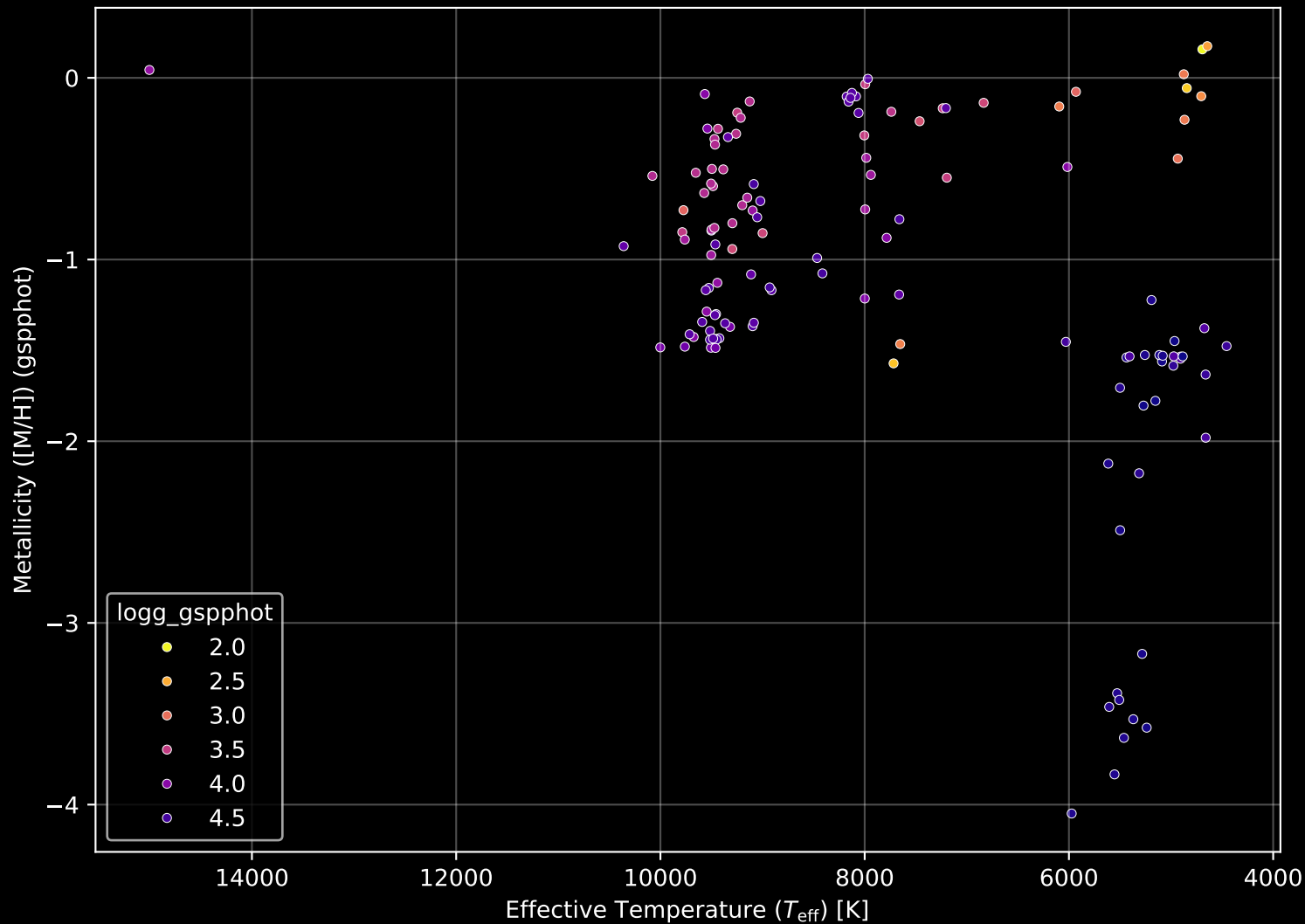
Gaia Cluster: [BH_84] Stellar Population Parameters (n= 132)
