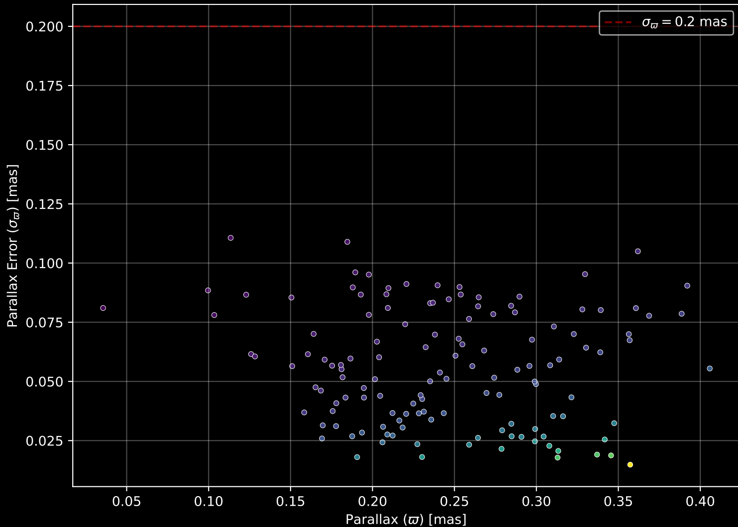
Gaia Cluster: [BH_84] Parallax Quality (n= 132)
