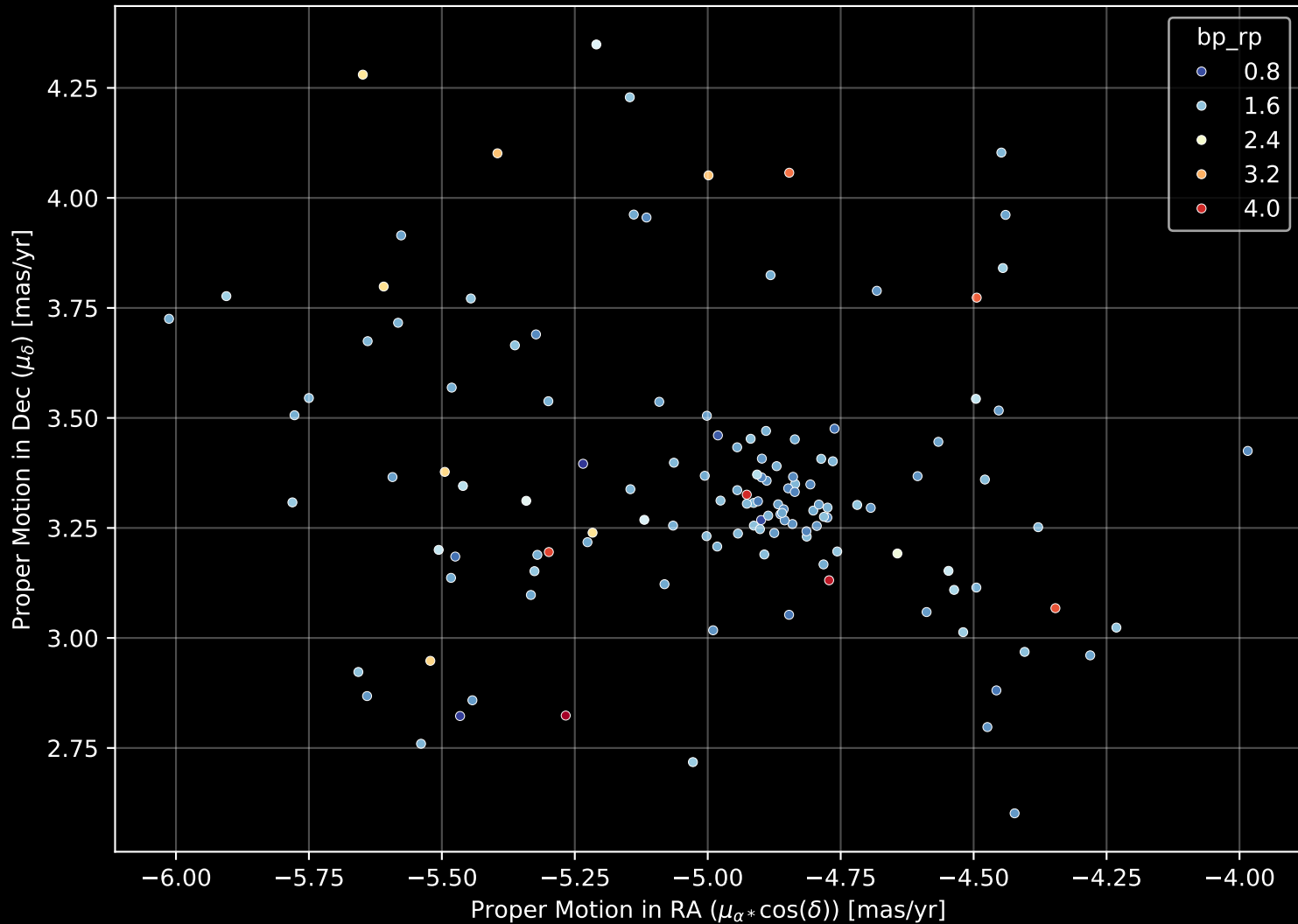
Gaia Cluster: [BH_84] Proper Motion Diagram (n= 132)
