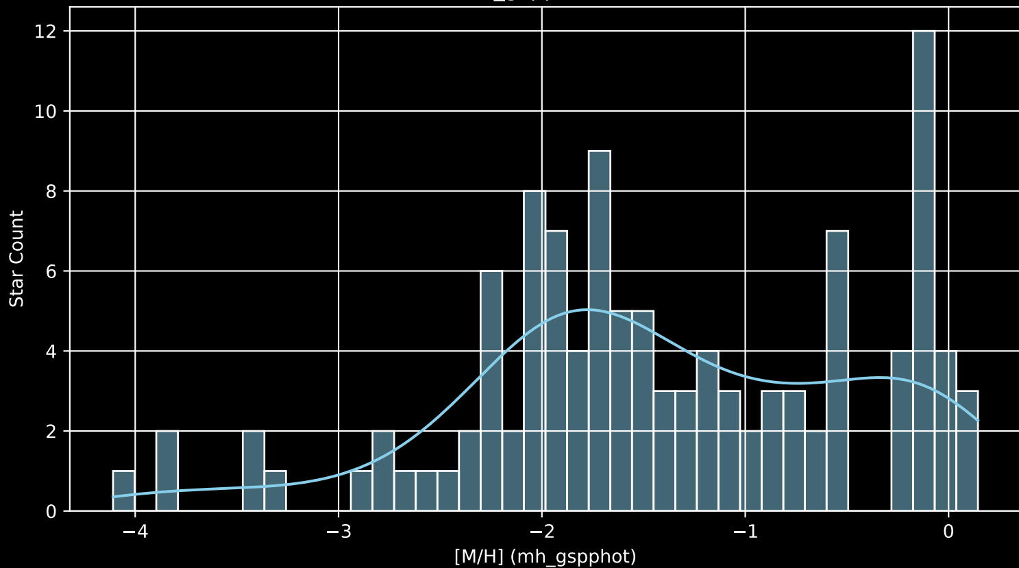
Gaia Cluster: [BH_85 [M/H] (mh_gspphot) (n= 113)
