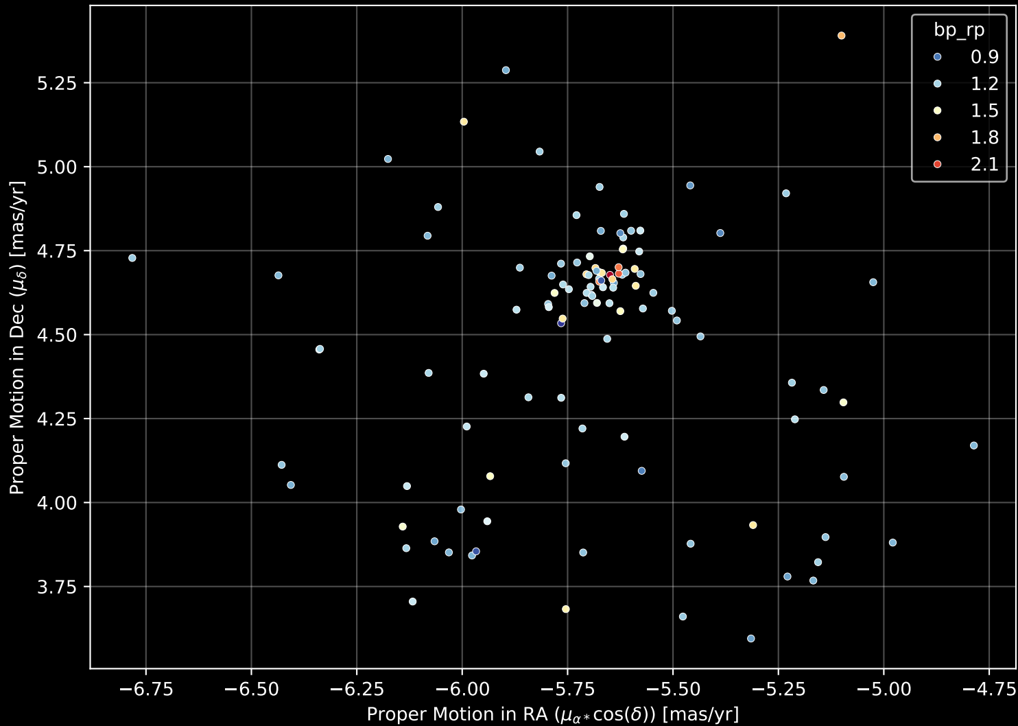
Gaia Cluster: [BH_85] Proper Motion Diagram (n= 113)
