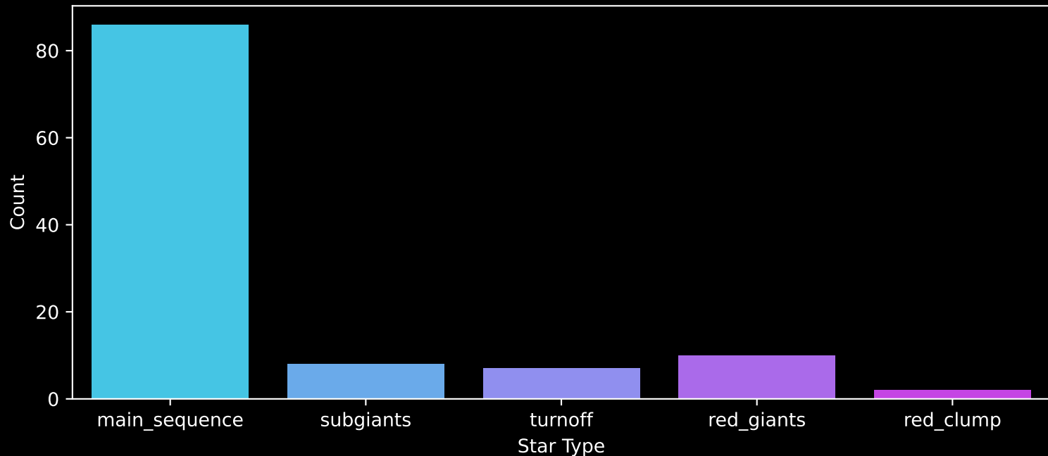
Gaia Cluster: [BH_85] Count plot of Star Type
