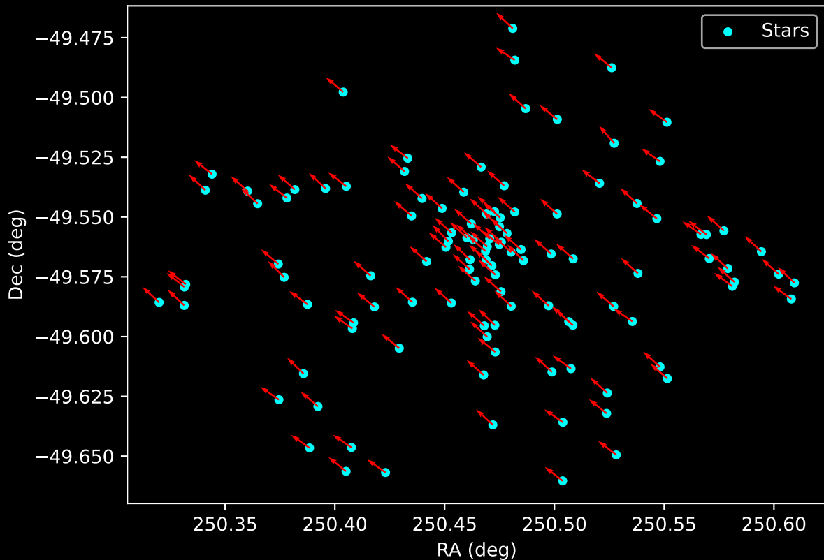
Gaia Cluster: [BH_85] Proper Motion Vectors for Gaia Star Field (n= 113)
