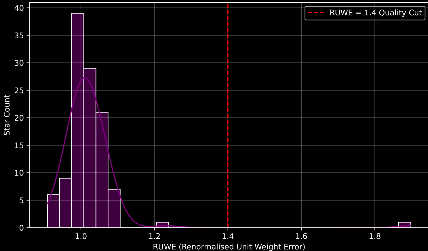
Gaia Cluster: [BH_85] RUWE Distribution (n= 113)
