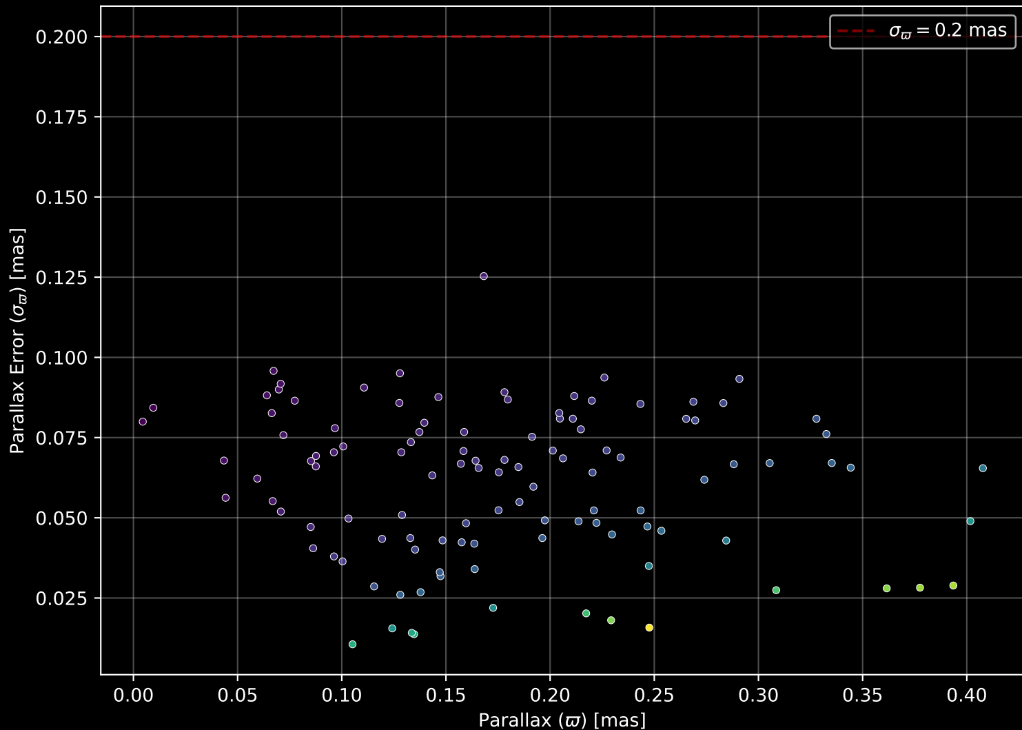
Gaia Cluster: [BH_85] Parallax Quality (n= 113)
