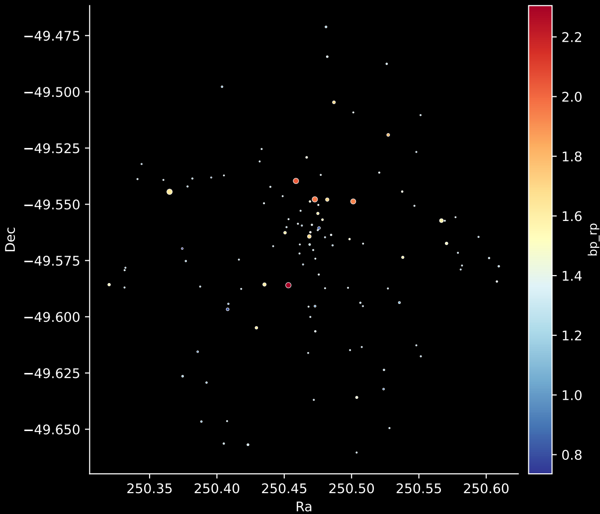
Gaia Cluster: [BH_85] Stars: 113
