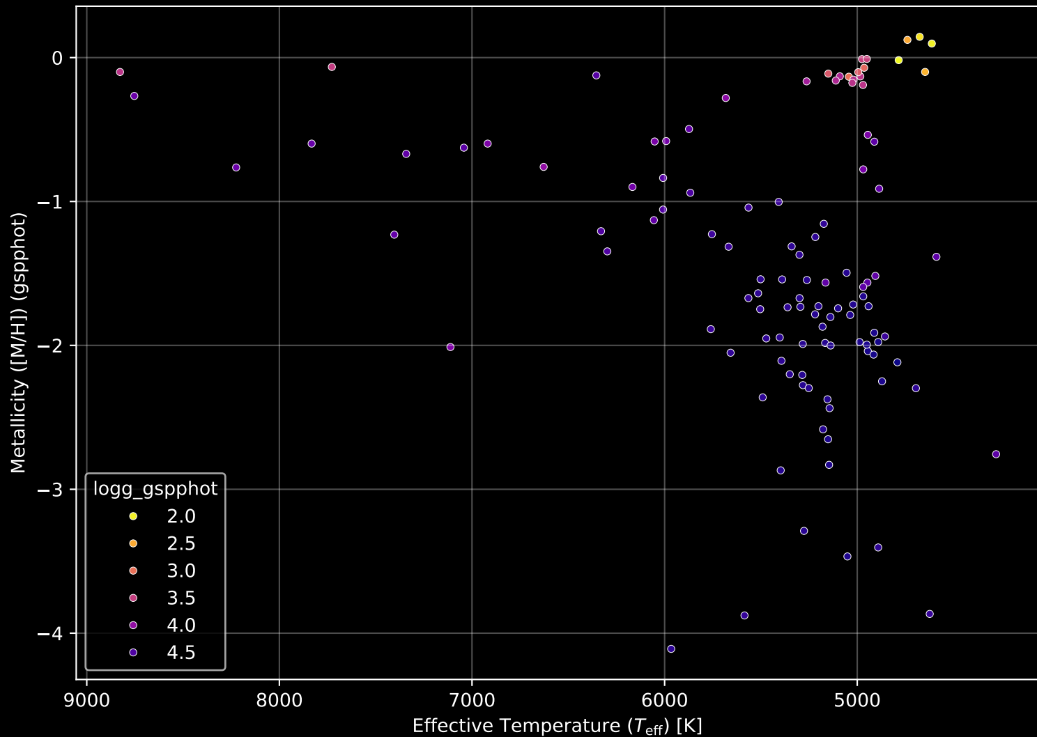
Gaia Cluster: [BH_85] Stellar Population Parameters (n= 113)
