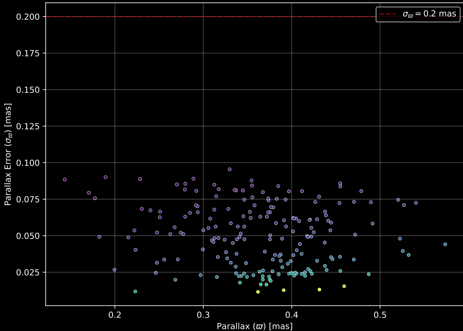
Gaia Cluster: [BH_90] Parallax Quality (n= 190)
