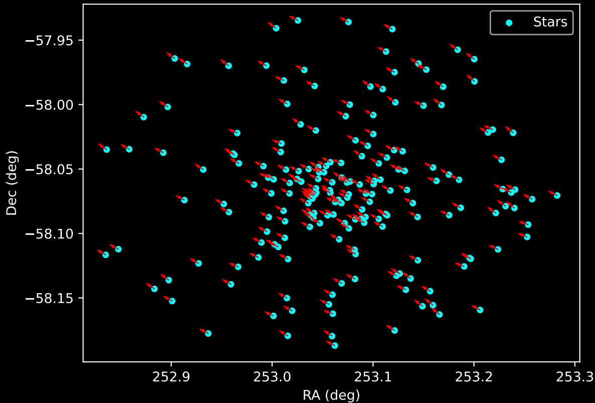
Gaia Cluster: [BH_90] Proper Motion Vectors for Gaia Star Field (n= 190)
