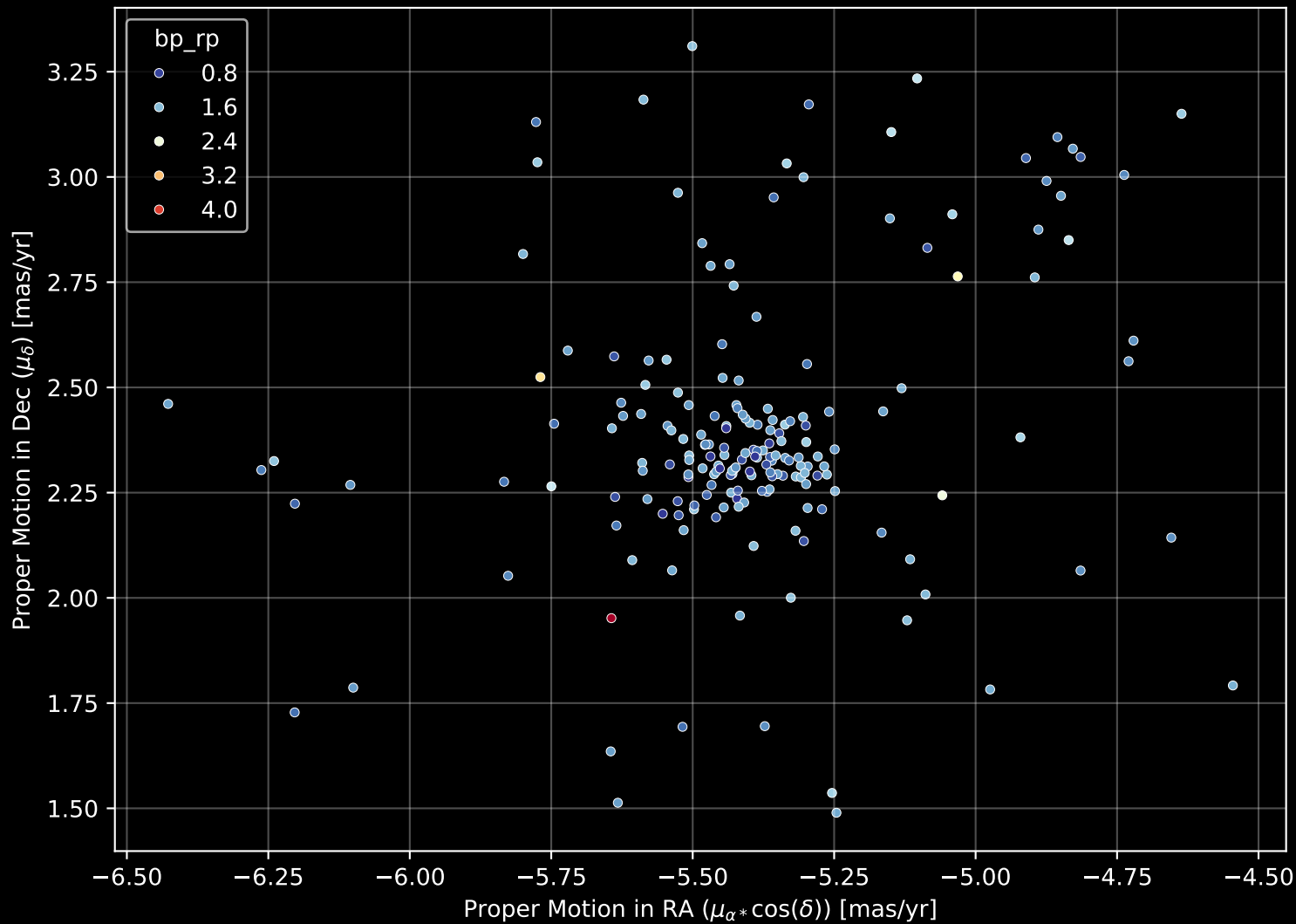
Gaia Cluster: [BH_90] Proper Motion Diagram (n= 190)
