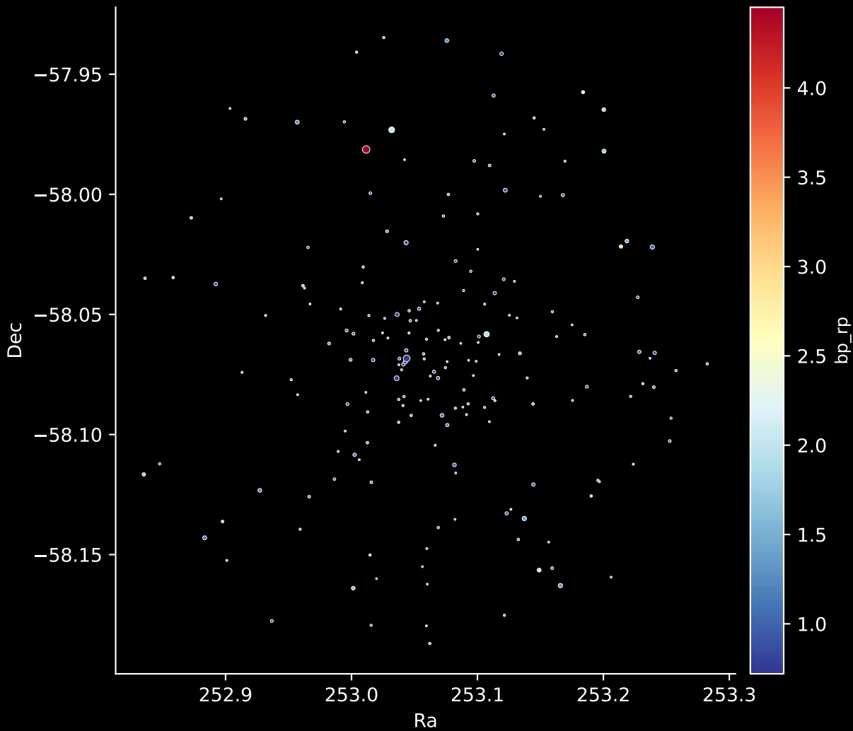
Gaia Cluster: [BH_90] Stars: 190
