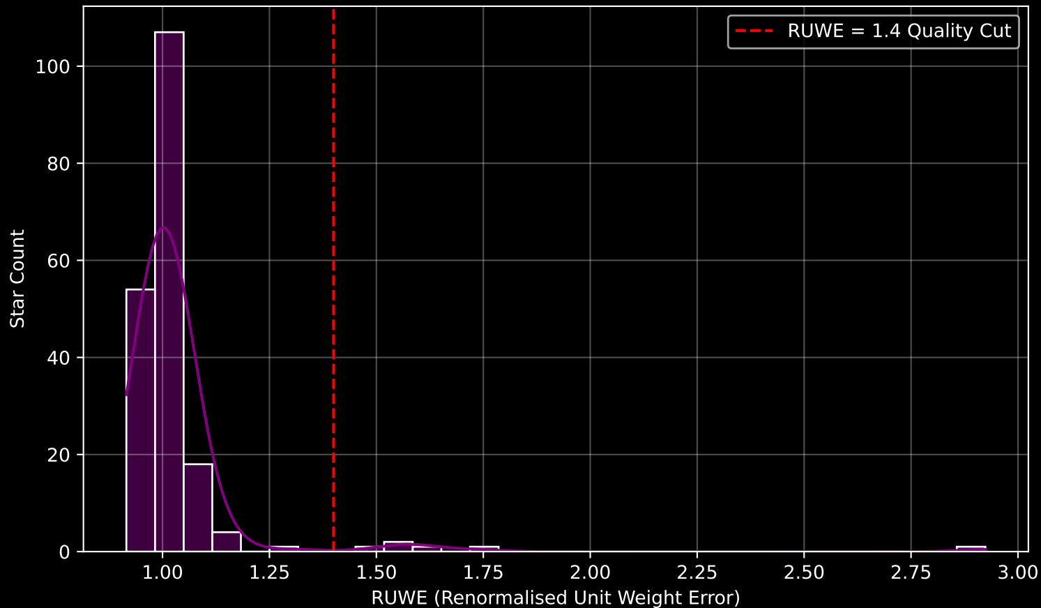
Gaia Cluster: [BH_90] RUWE Distribution (n= 190)
