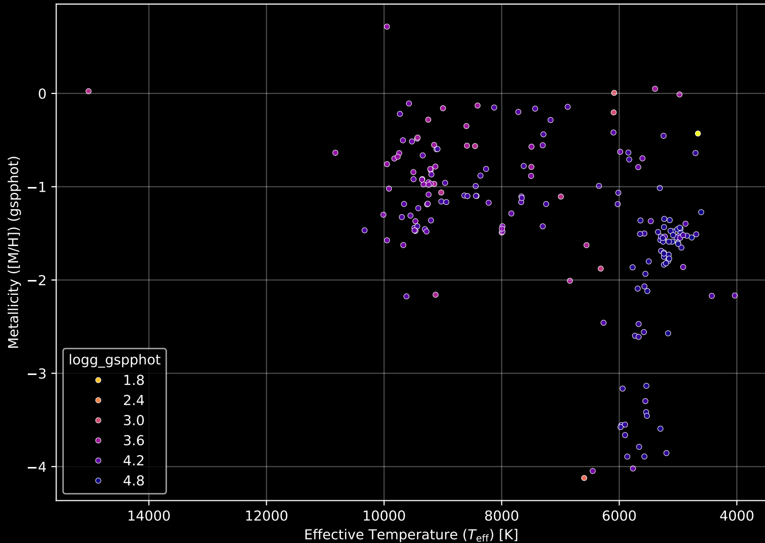
Gaia Cluster: [BH_90] Stellar Population Parameters (n= 190)
