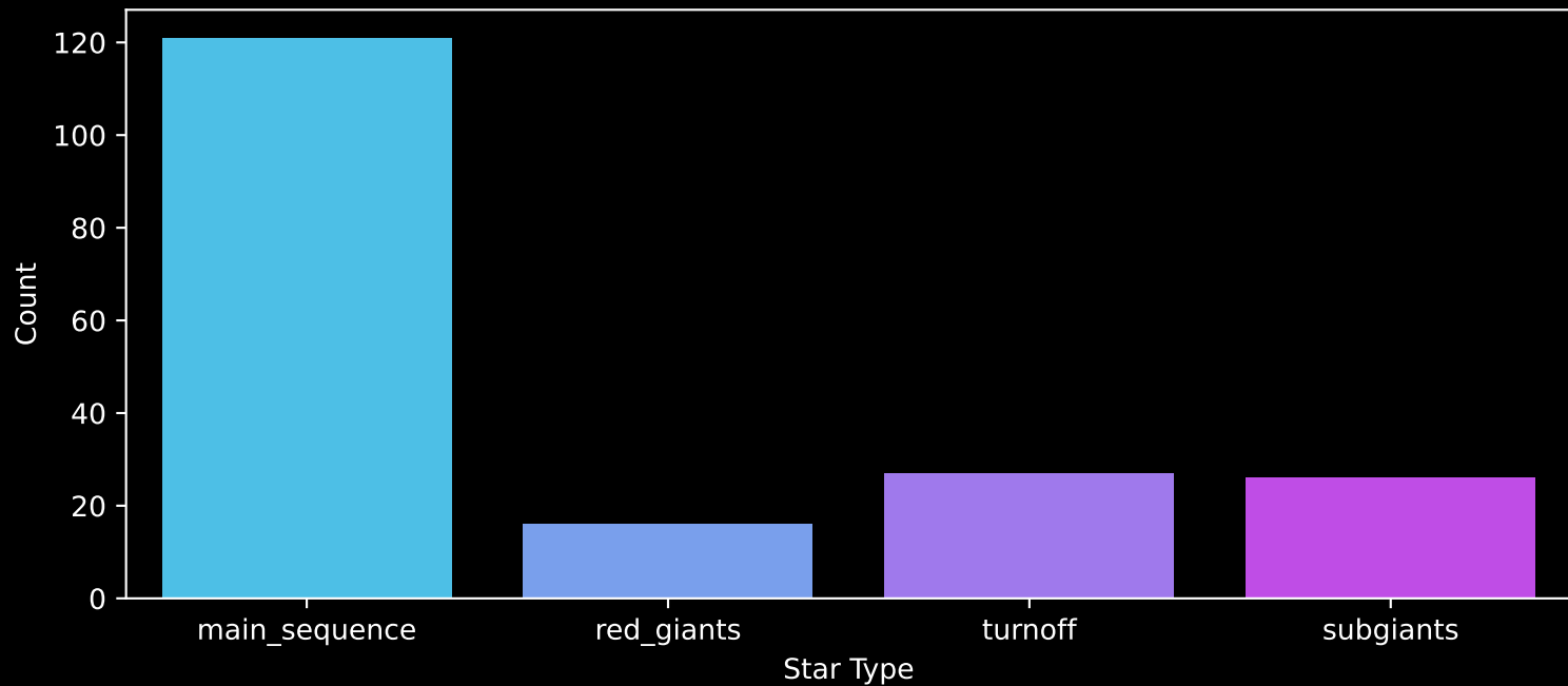
Gaia Cluster: [BH_90] Count plot of Star Type
