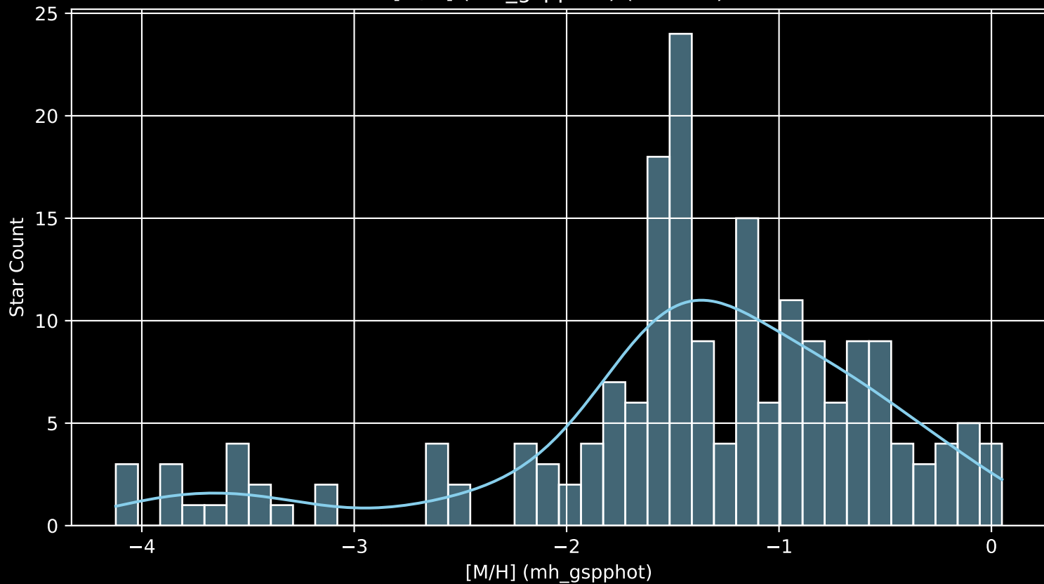
Gaia Cluster: [BH_90 [M/H] (mh_gspphot) (n= 189)
