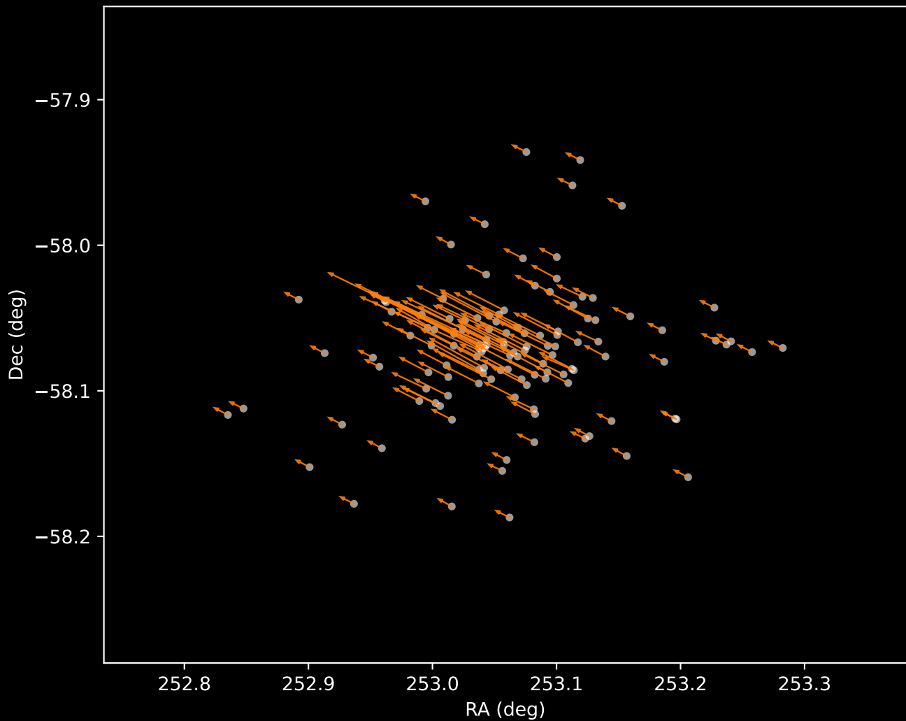
Gaia DR3 Cluster 2 Proper Motion Vectors (n=125)
