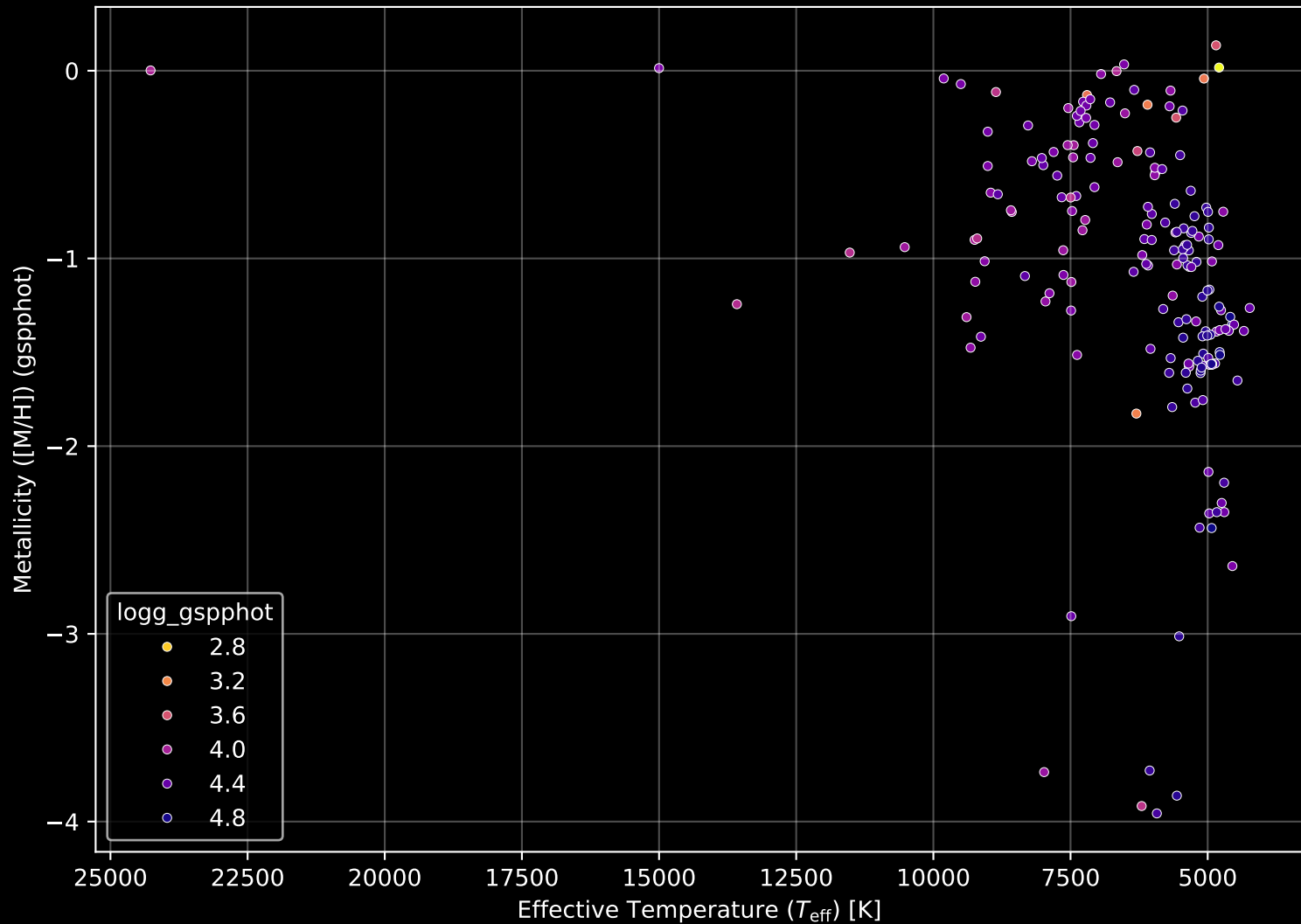
Gaia Cluster: [Barkhatova_1] Stellar Population Parameters (n= 186)
