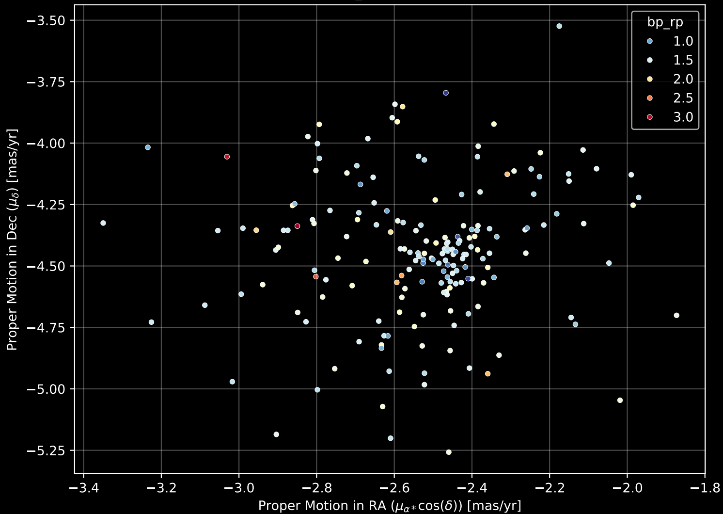
Gaia Cluster: [Barkhatova_1] Proper Motion Diagram (n= 186)
