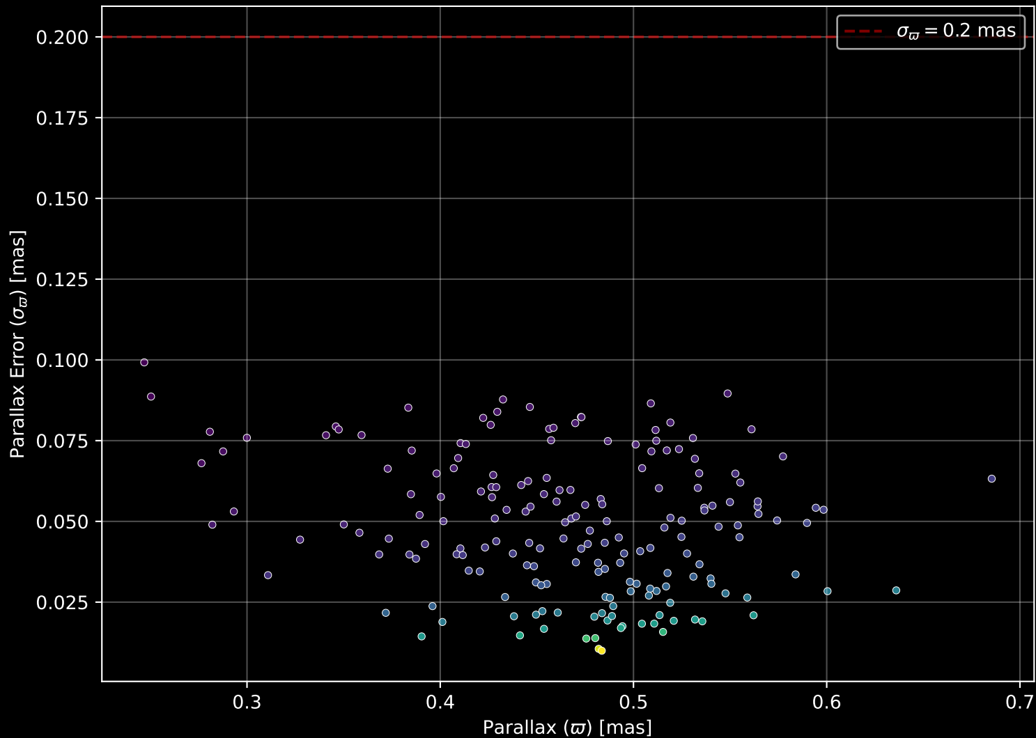
Gaia Cluster: [Barkhatova_1] Parallax Quality (n= 186)
