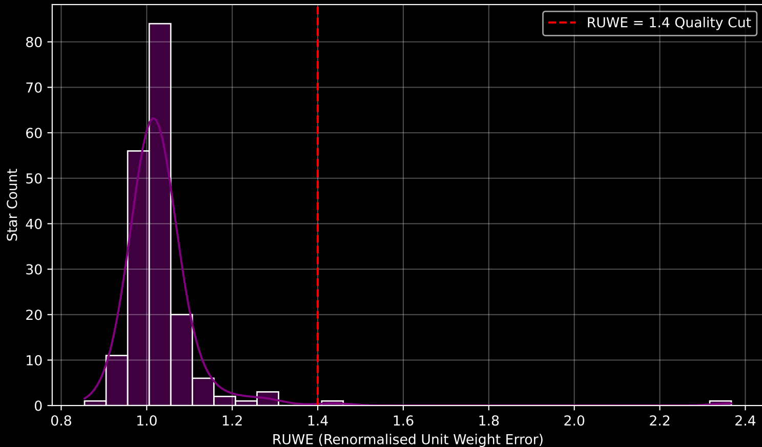
Gaia Cluster: [Barkhatova_1] RUWE Distribution (n= 186)
