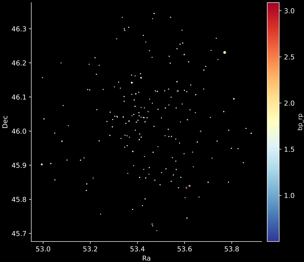
Gaia Cluster: [Barkhatova_1] Stars: 186
