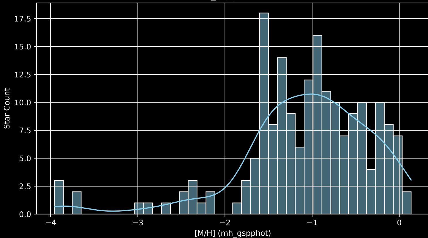
Gaia Cluster: [Barkhatova_1 [M/H] (mh_gspphot) (n= 186)
