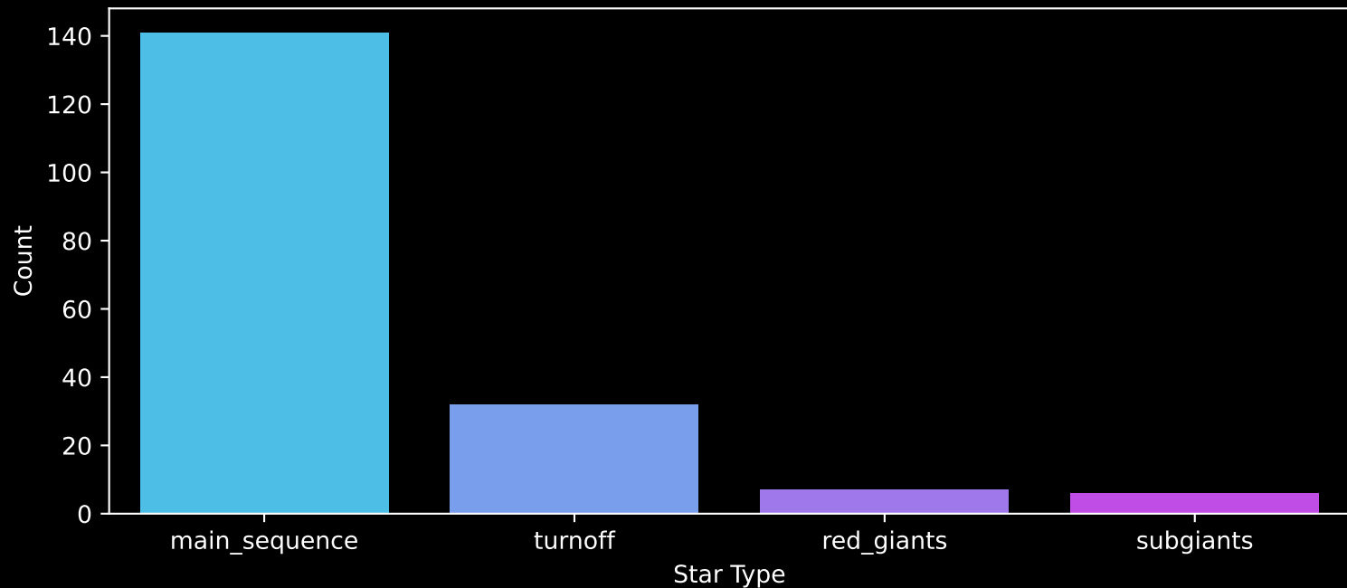
Gaia Cluster: [Barkhatova_1] Count plot of Star Type
