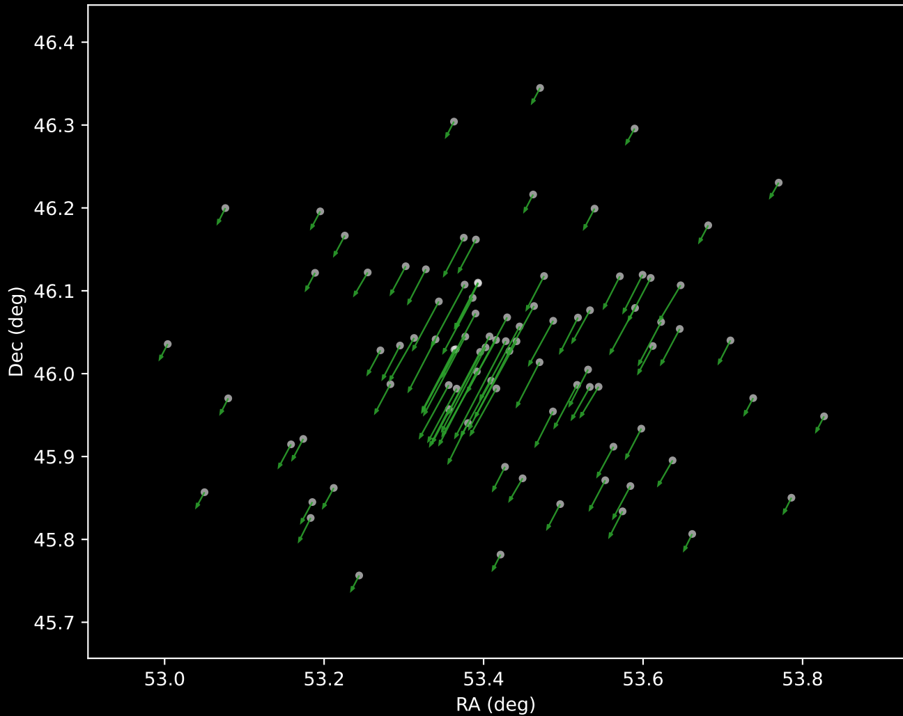
Gaia DR3 Cluster 4 Proper Motion Vectors (n=89)
