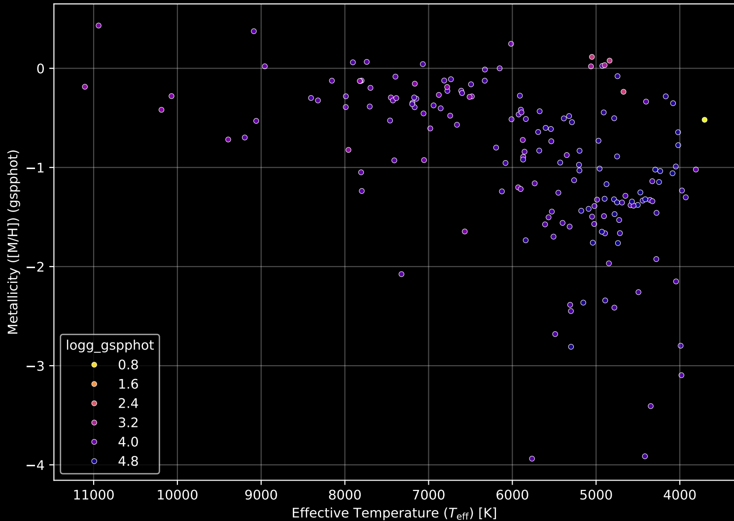
Gaia Cluster: [Basel_1] Stellar Population Parameters (n= 172)
