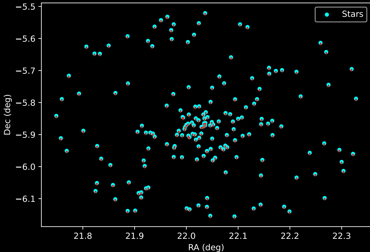
Gaia Cluster: [Basel_1] Proper Motion Vectors for Gaia Star Field (n= 172)
