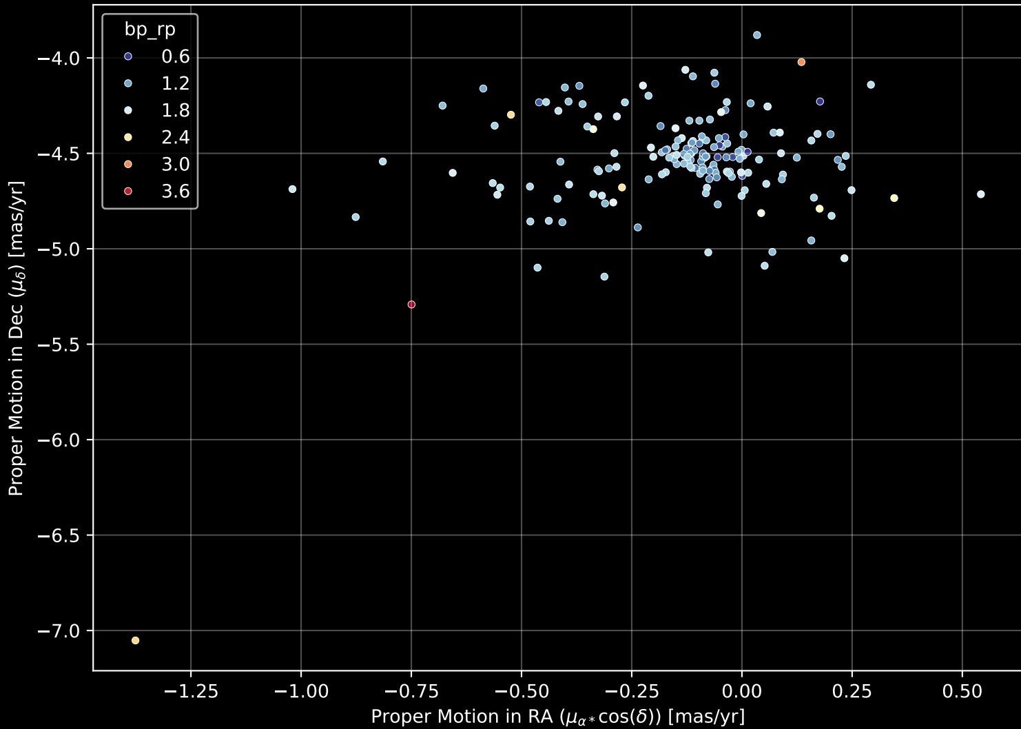
Gaia Cluster: [Basel_1] Proper Motion Diagram (n= 172)
