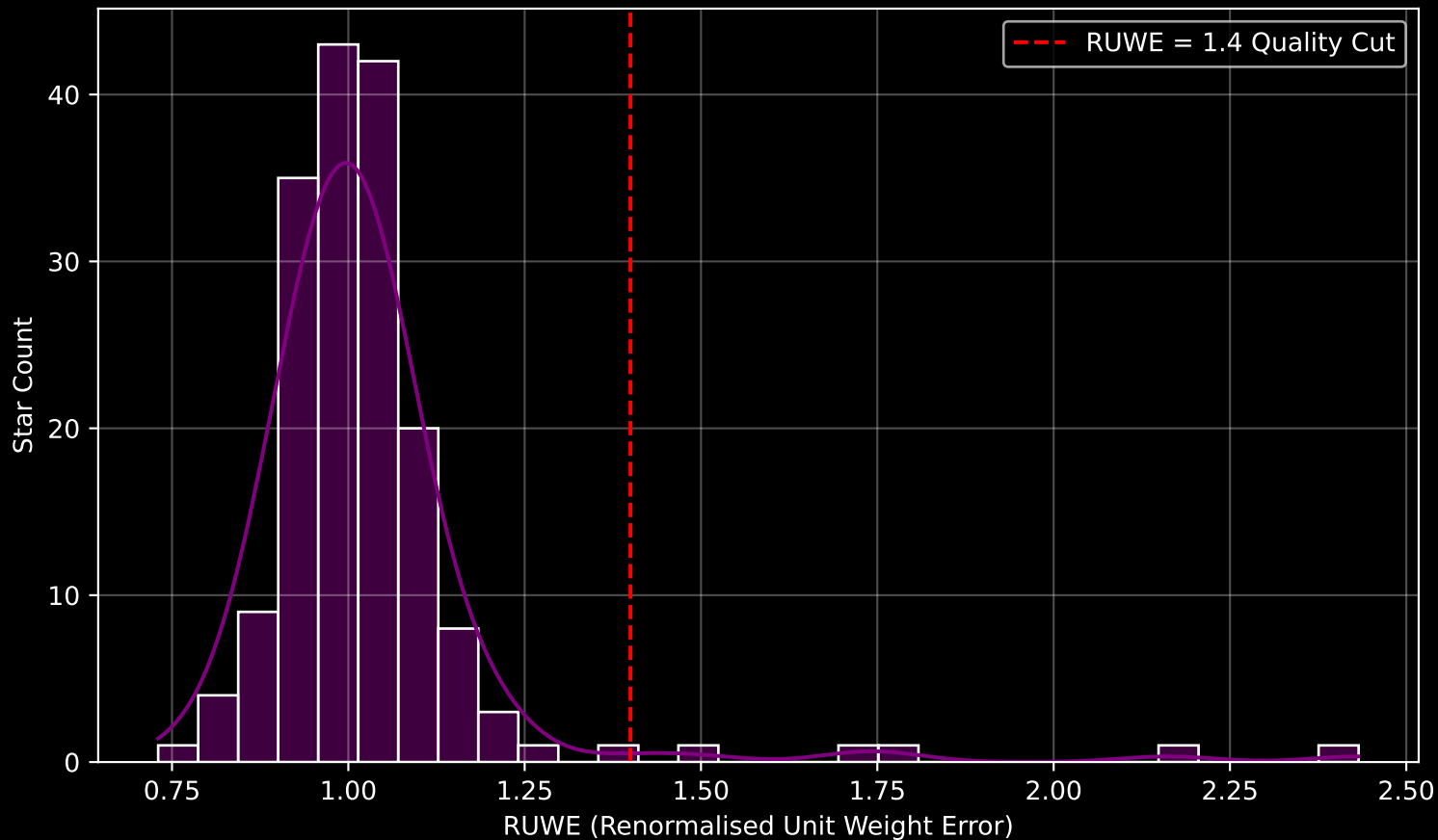
Gaia Cluster: [Basel_1] RUWE Distribution (n= 172)
