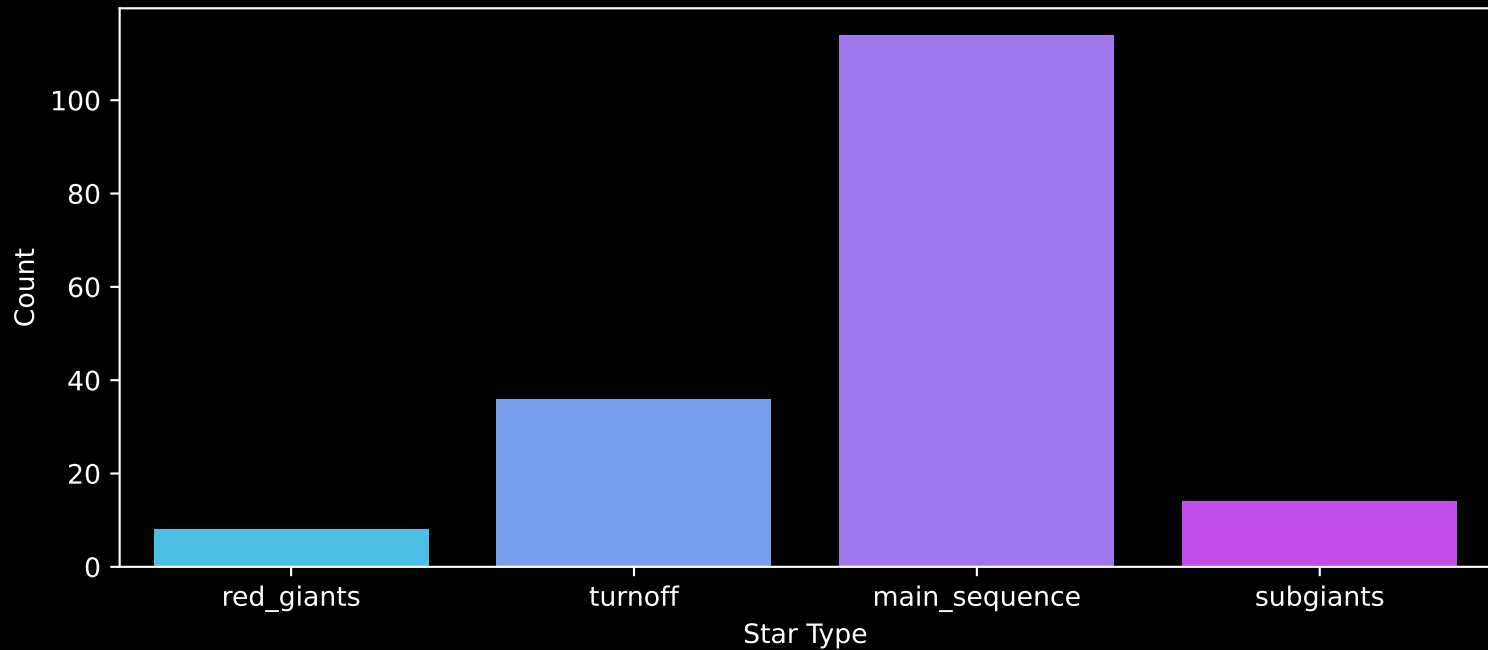
Gaia Cluster: [Basel_1] Count plot of Star Type
