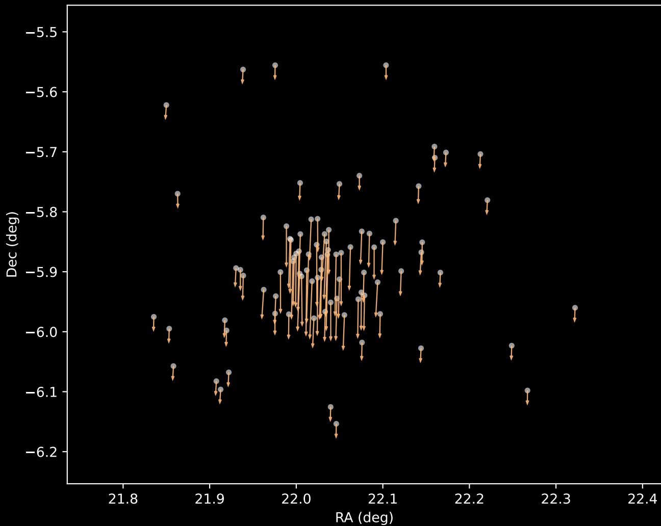
Gaia DR3 Cluster 3 Proper Motion Vectors (n=86)
