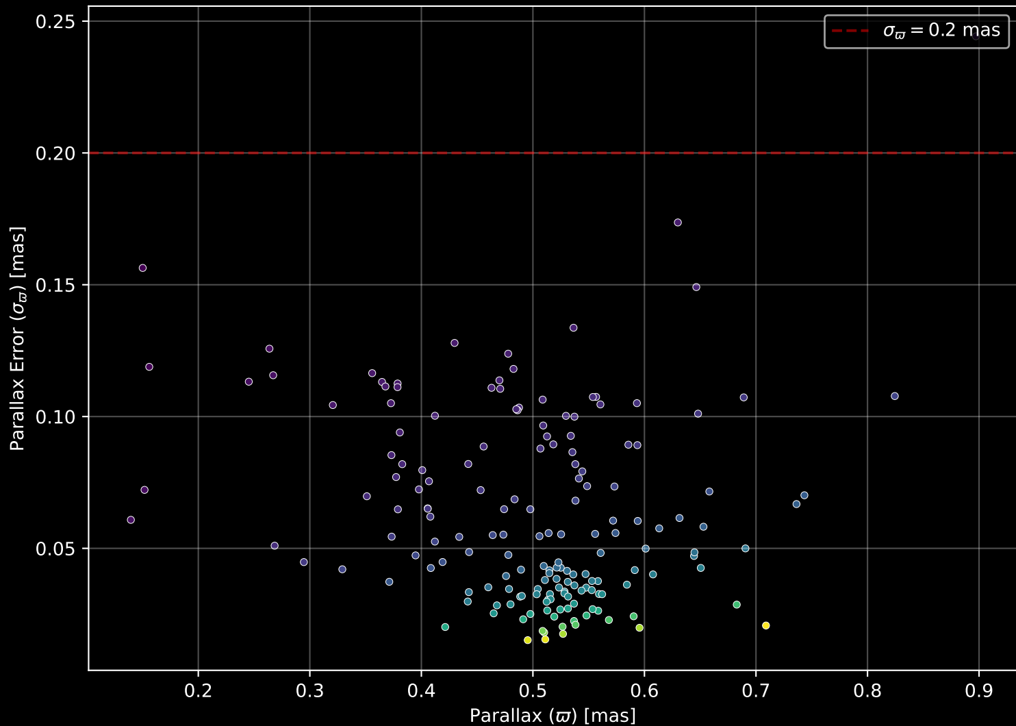
Gaia Cluster: [Basel_1] Parallax Quality (n= 172)
