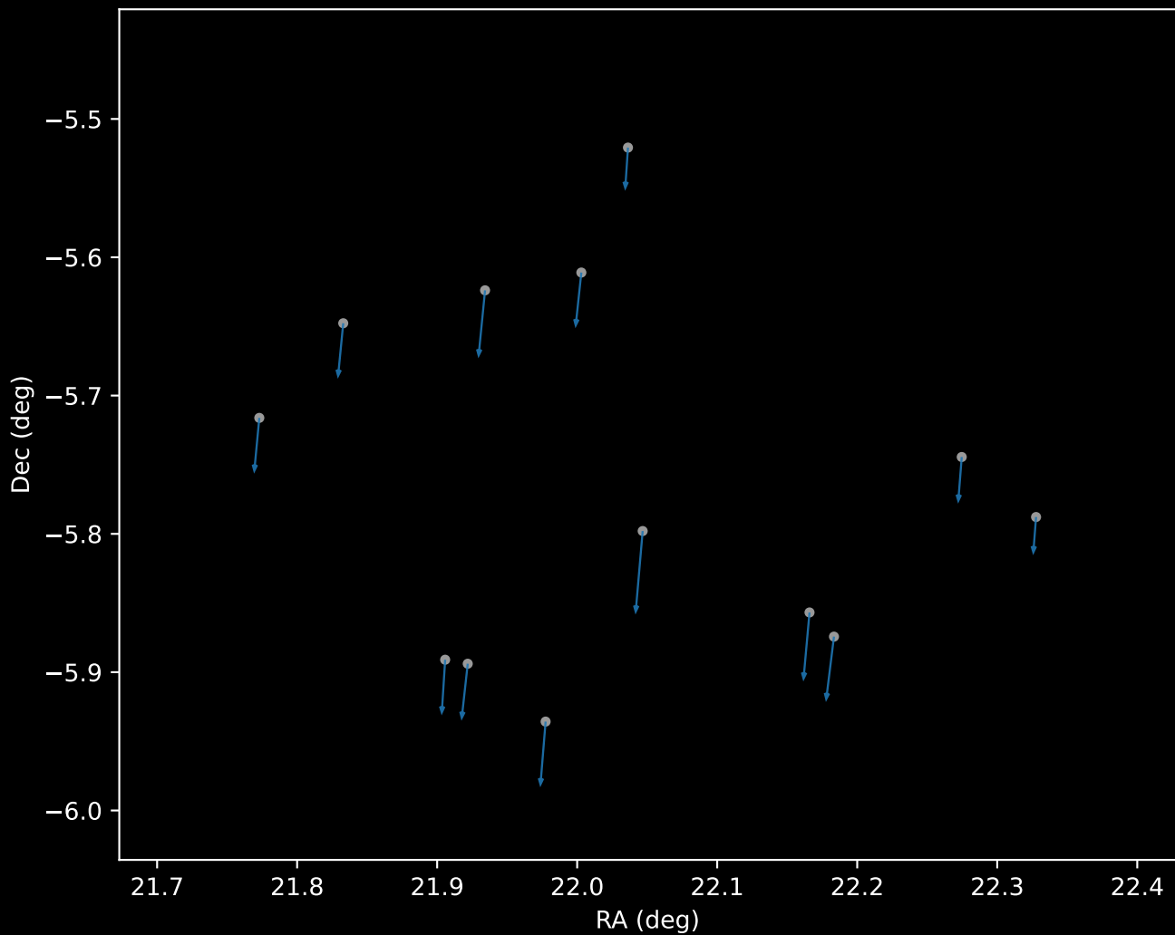
Gaia DR3 Cluster 0 Proper Motion Vectors (n=13)
