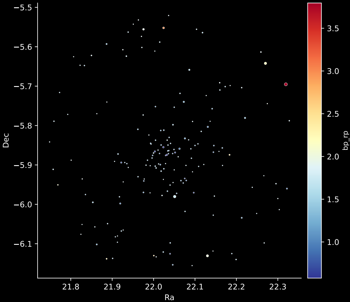
Gaia Cluster: [Basel_1] Stars: 172
