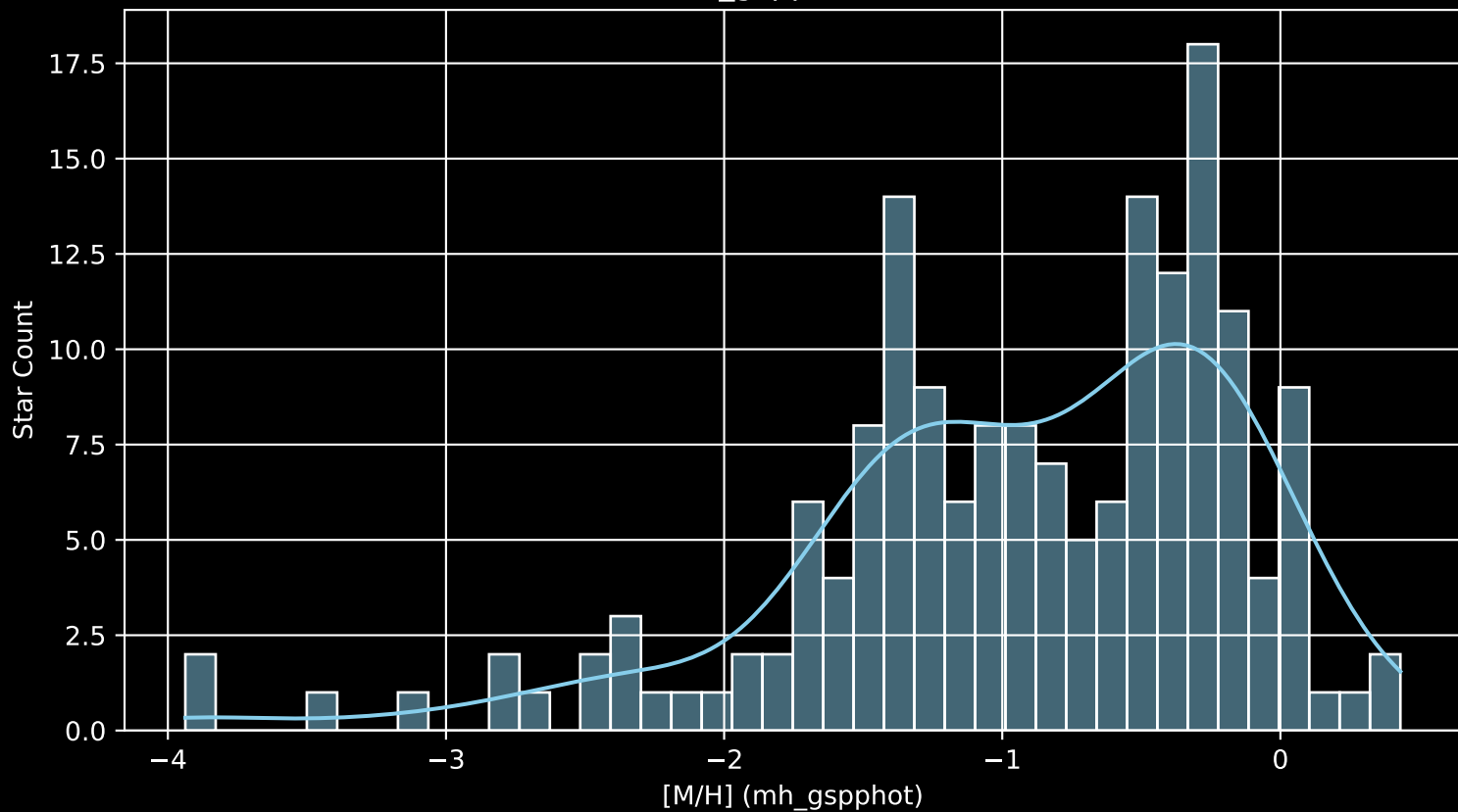
Gaia Cluster: [Basel_1 [M/H] (mh_gspphot) (n= 172)
