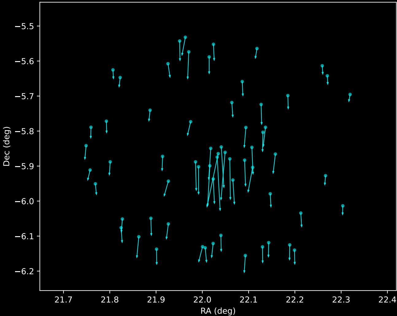
Gaia DR3 Noise Stream Proper Motion Vectors (n=63)
