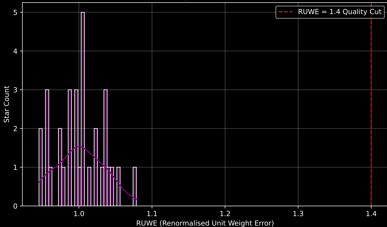
Gaia Cluster: [Basel_10] RUWE Distribution (n= 32)
