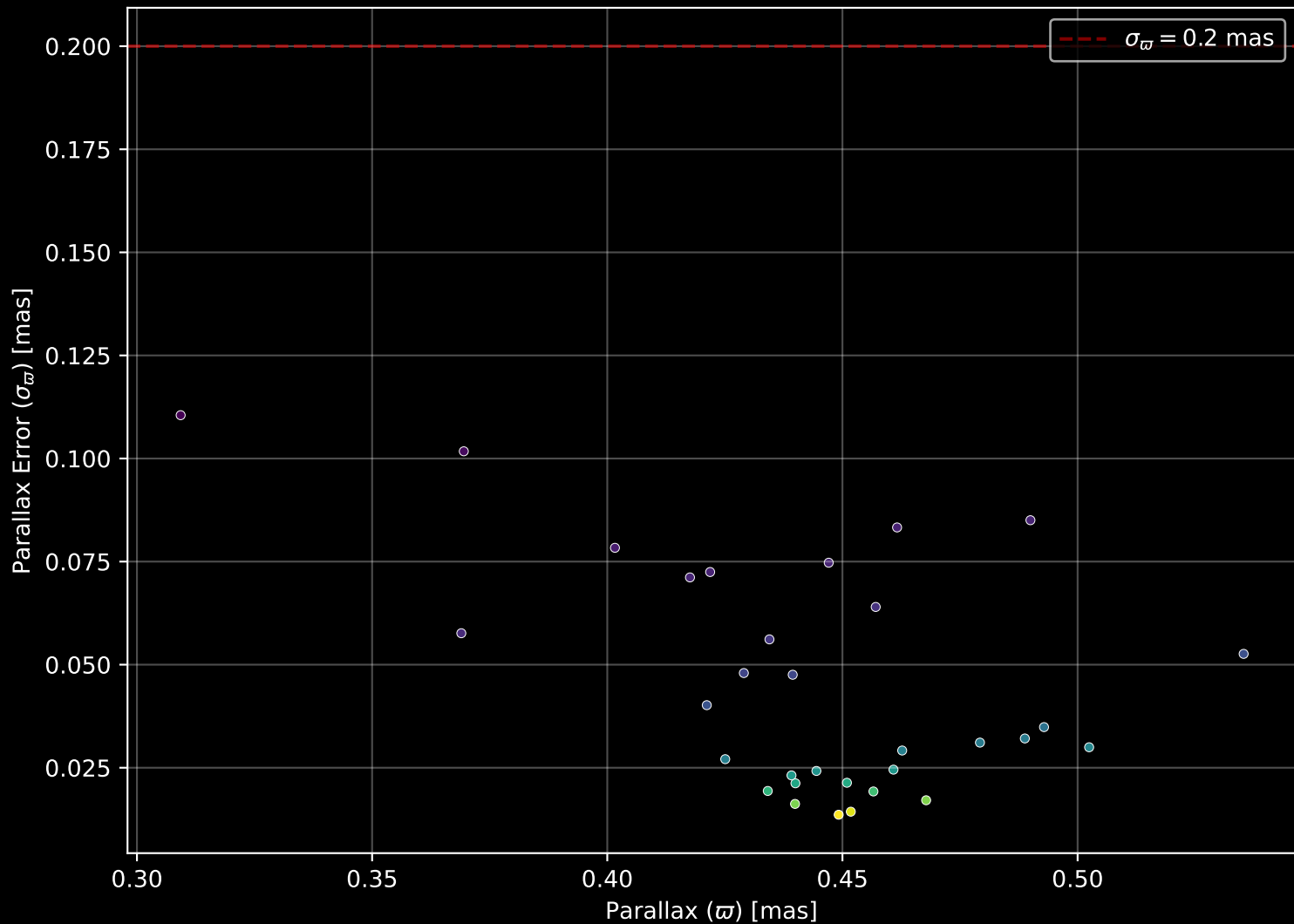
Gaia Cluster: [Basel_10] Parallax Quality (n= 32)
