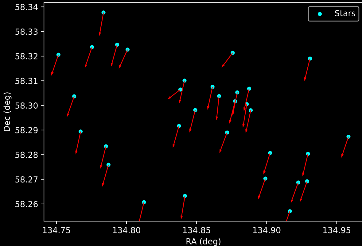
Gaia Cluster: [Basel_10] Proper Motion Vectors for Gaia Star Field (n= 32)
