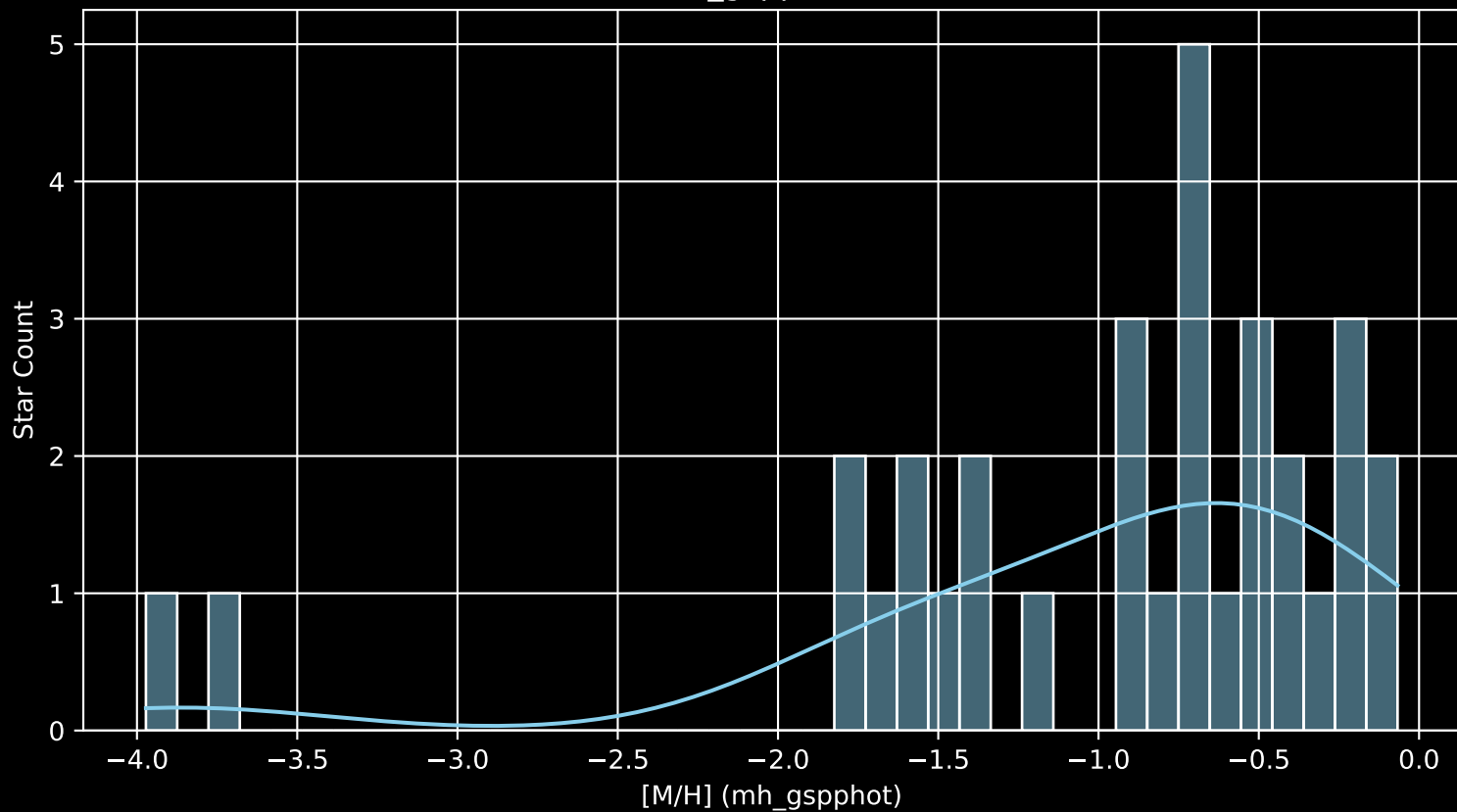
Gaia Cluster: [Basel_10 [M/H] (mh_gspphot) (n= 32)
