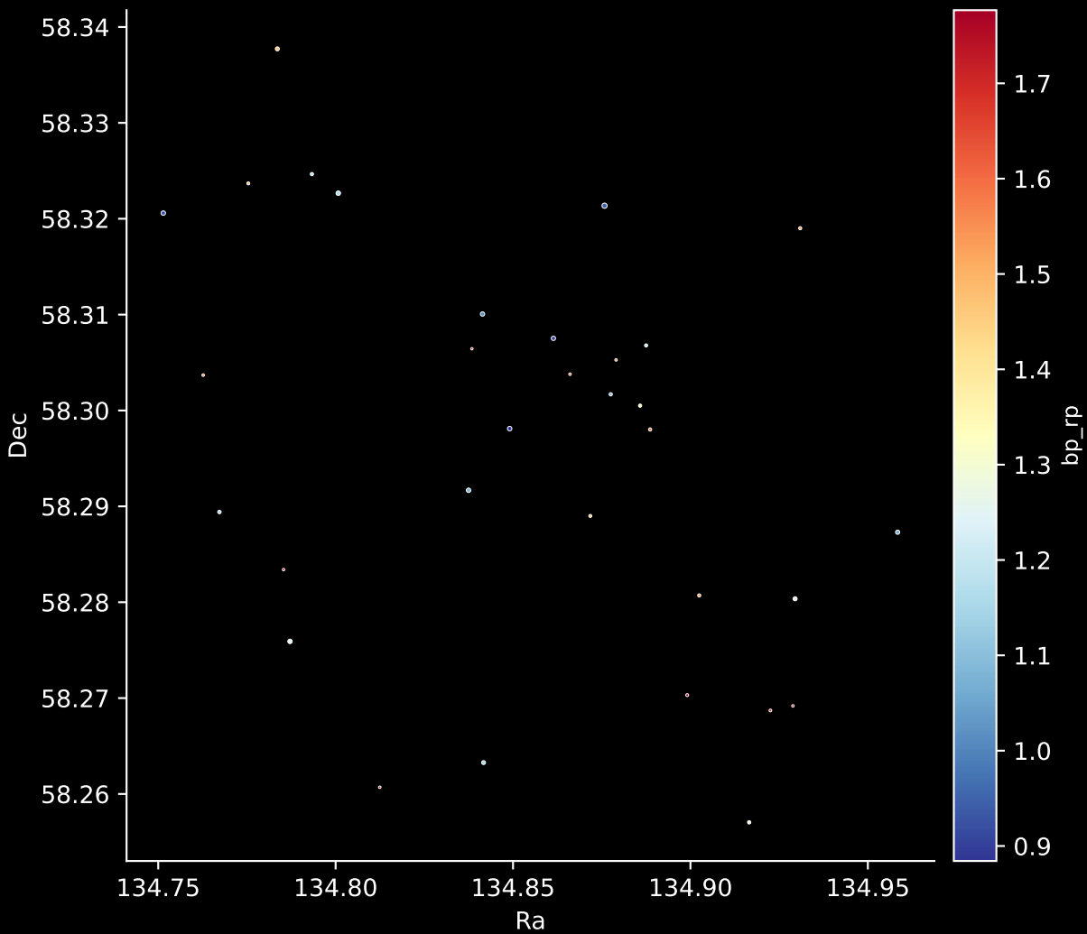
Gaia Cluster: [Basel_10] Stars: 32
