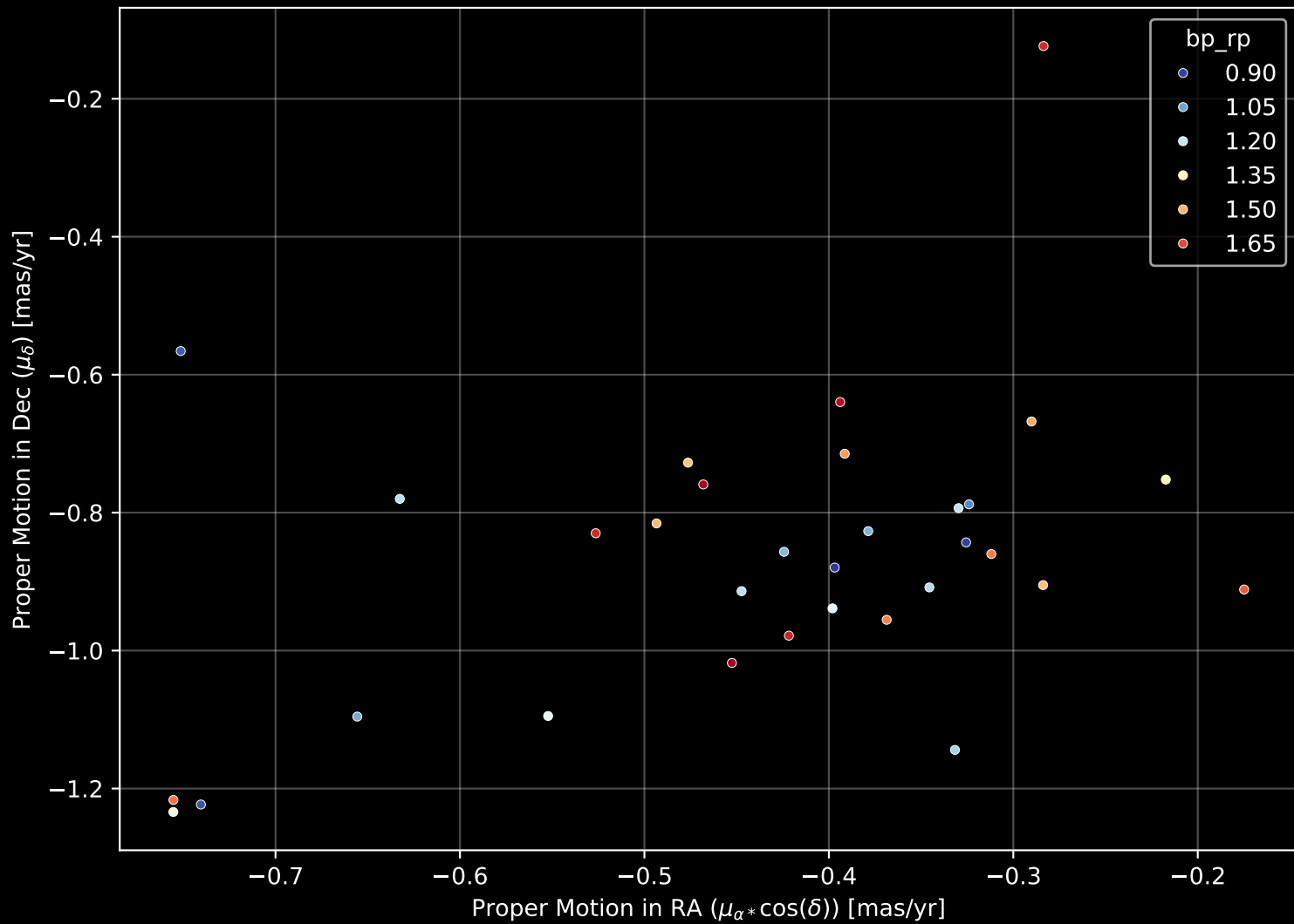
Gaia Cluster: [Basel_10] Proper Motion Diagram (n= 32)
