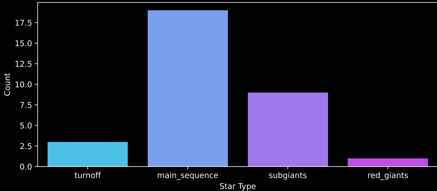
Gaia Cluster: [Basel_10] Count plot of Star Type
