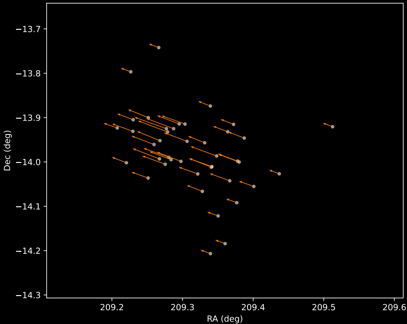
Gaia DR3 Cluster 2 Proper Motion Vectors (n=41)
