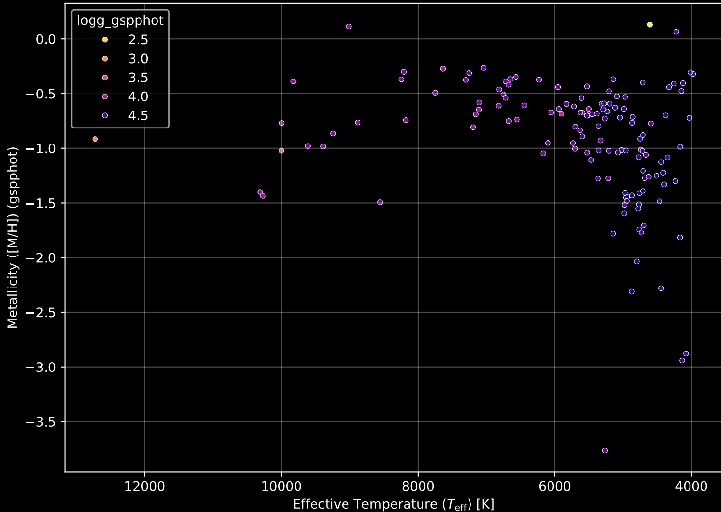
Gaia Cluster: [Basel_11a] Stellar Population Parameters (n= 135)
