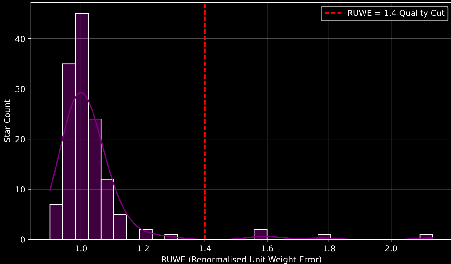
Gaia Cluster: [Basel_11a] RUWE Distribution (n= 135)
