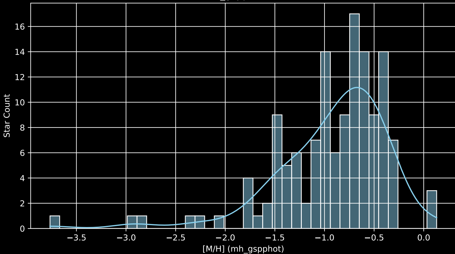
Gaia Cluster: [Basel_11a [M/H] (mh_gspphot) (n= 135)
