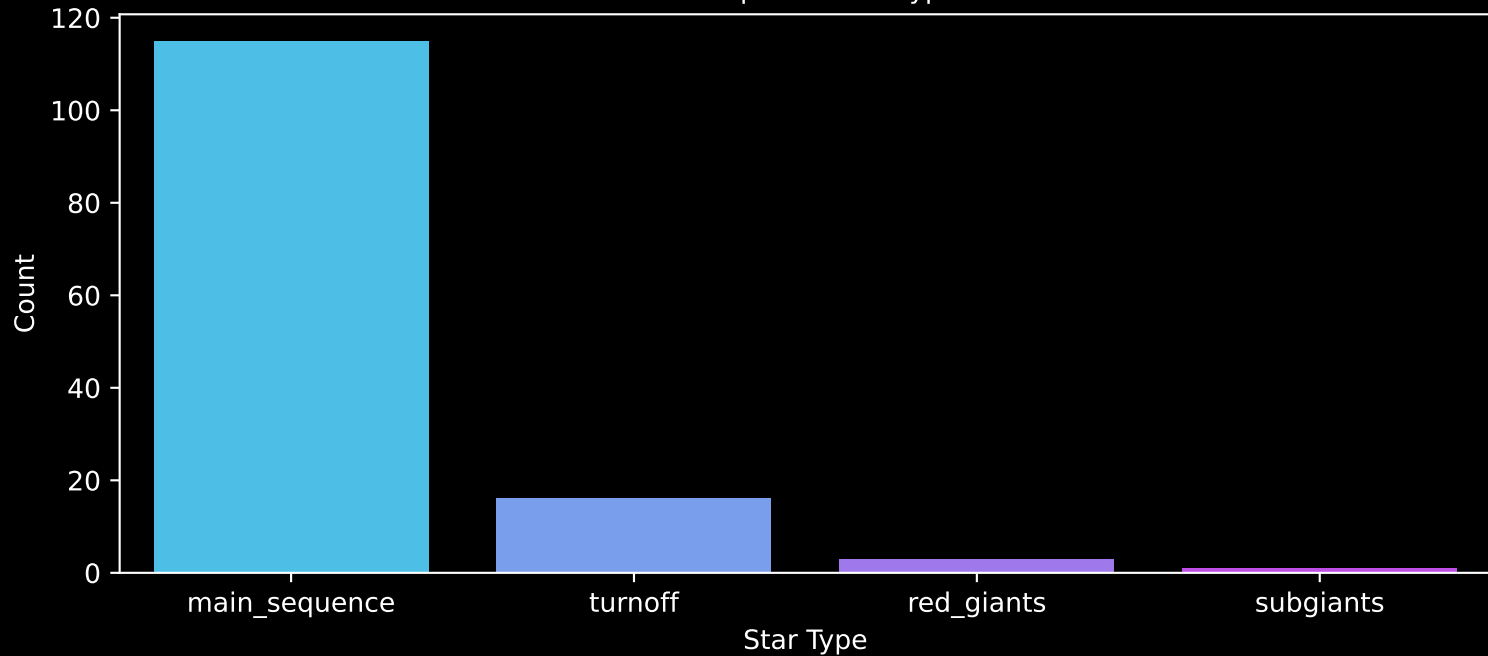
Gaia Cluster: [Basel_11a] Count plot of Star Type
