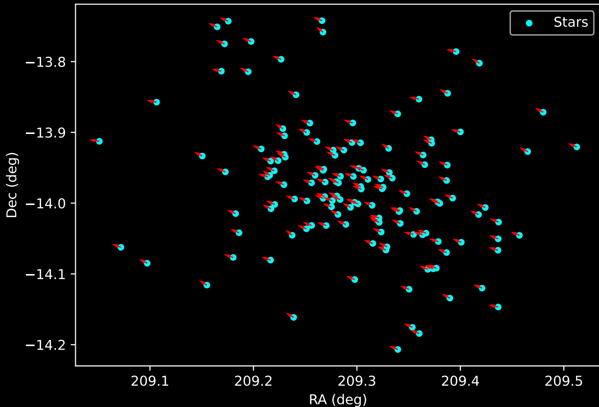
Gaia Cluster: [Basel_11a] Proper Motion Vectors for Gaia Star Field (n= 135)
