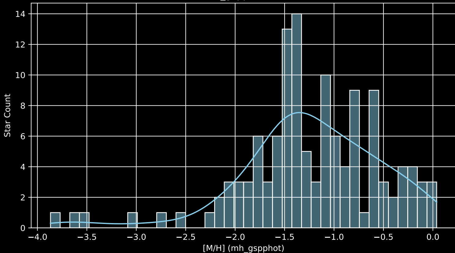
Gaia Cluster: [Basel_11b [M/H] (mh_gspphot) (n= 126)
