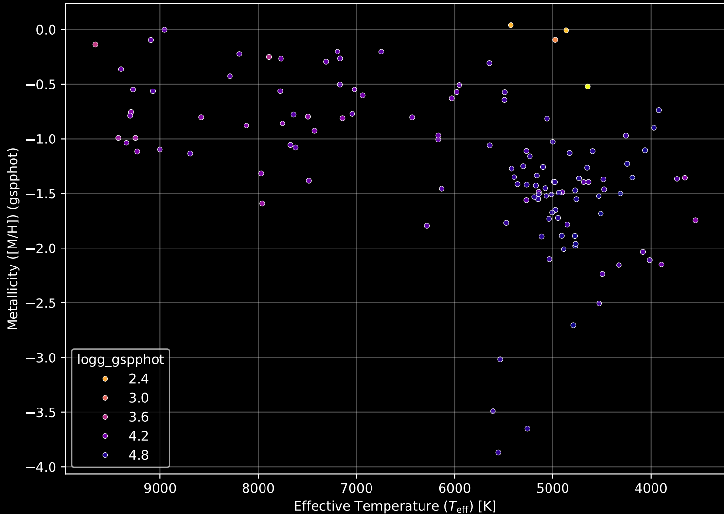
Gaia Cluster: [Basel_11b] Stellar Population Parameters (n= 126)
