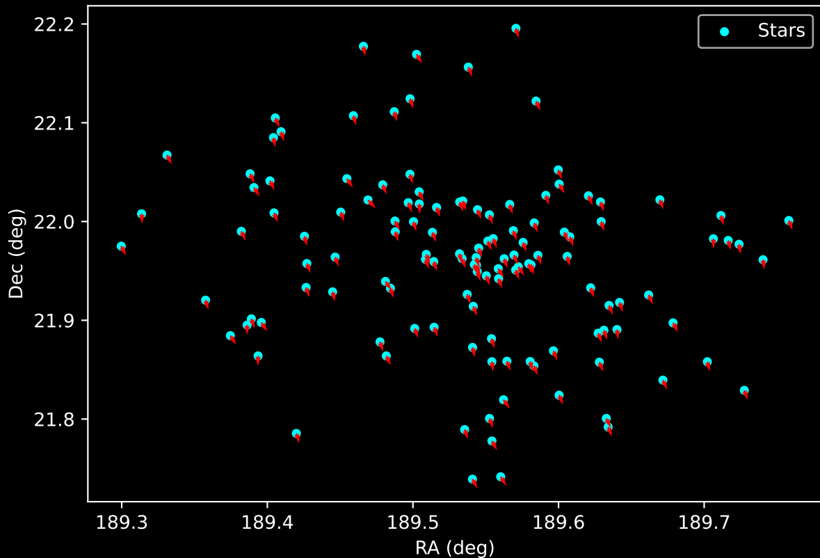
Gaia Cluster: [Basel_11b] Proper Motion Vectors for Gaia Star Field (n= 126)
