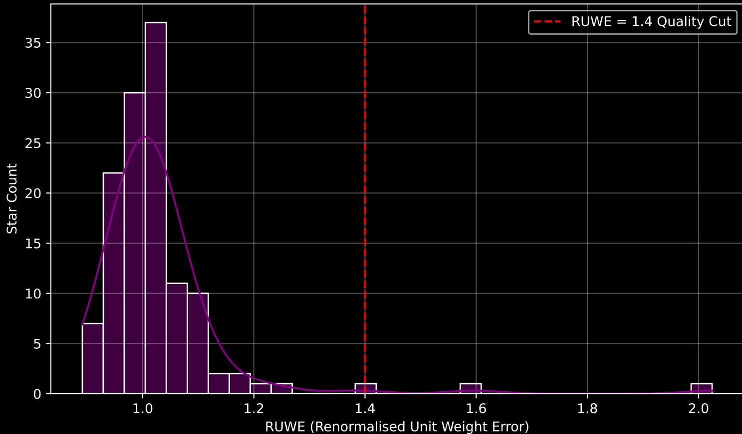
Gaia Cluster: [Basel_11b] RUWE Distribution (n= 126)
