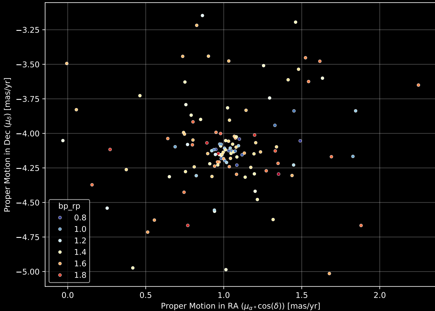
Gaia Cluster: [Basel_11b] Proper Motion Diagram (n= 126)
