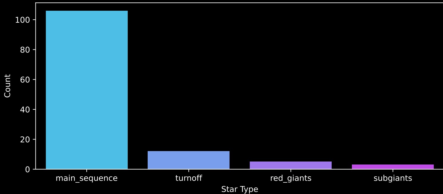
Gaia Cluster: [Basel_11b] Count plot of Star Type
