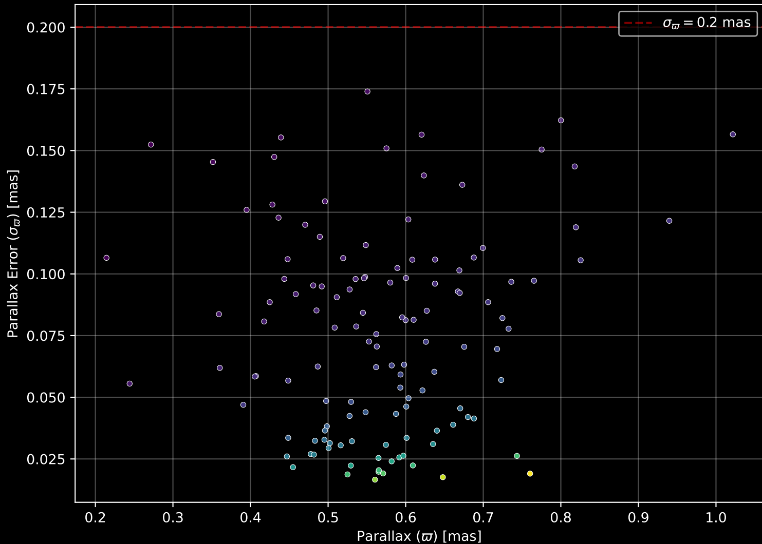
Gaia Cluster: [Basel_11b] Parallax Quality (n= 126)
