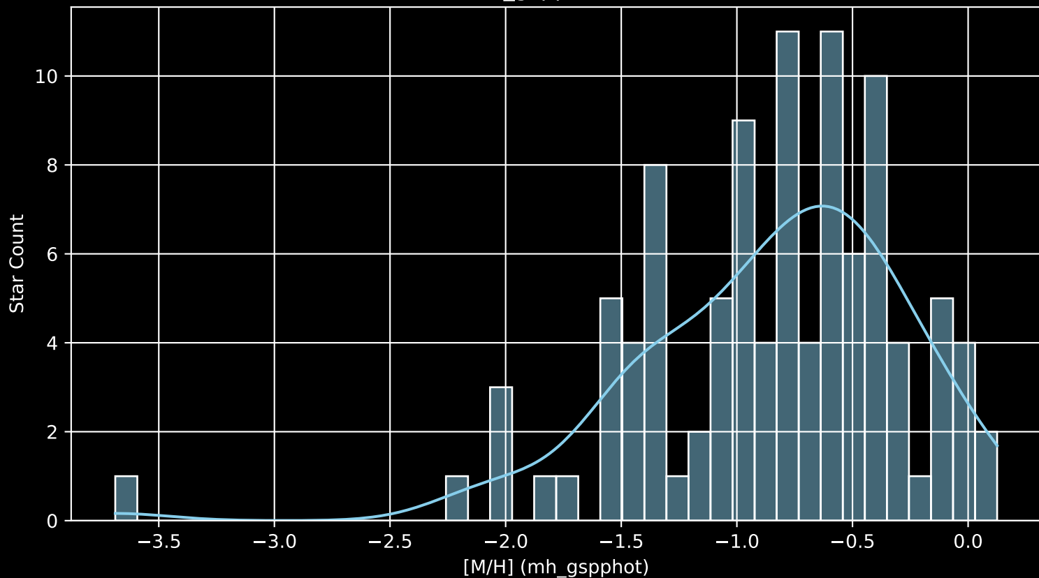
Gaia Cluster: [Basel_18 [M/H] (mh_gspphot) (n= 103)
