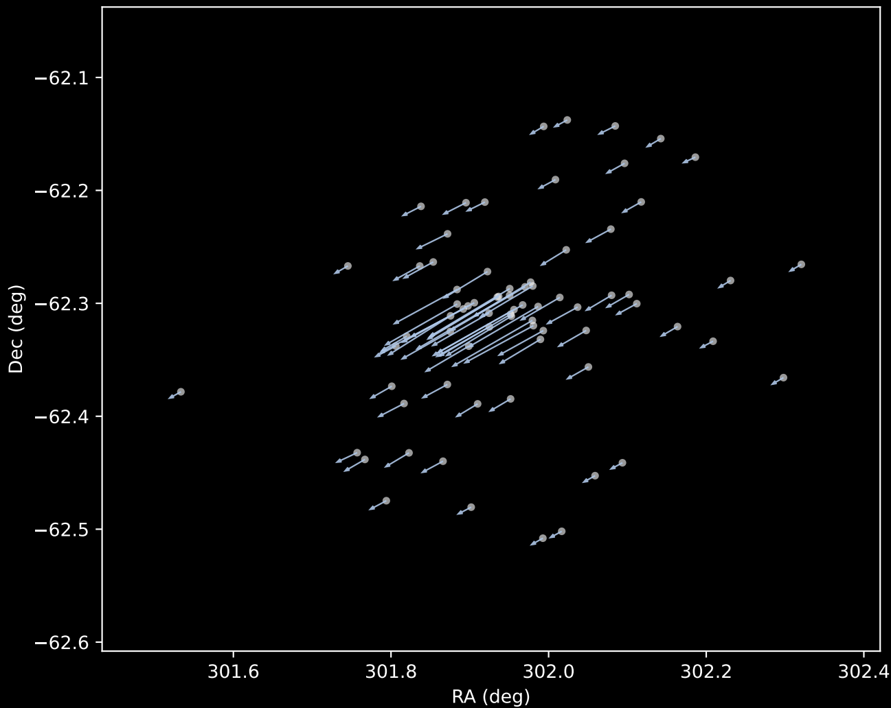
Gaia DR3 Cluster 1 Proper Motion Vectors (n=74)
