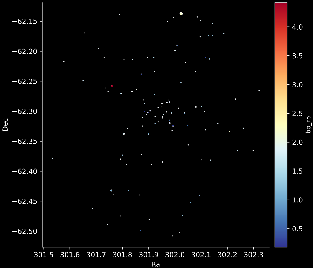
Gaia Cluster: [Basel_18] Stars: 104
