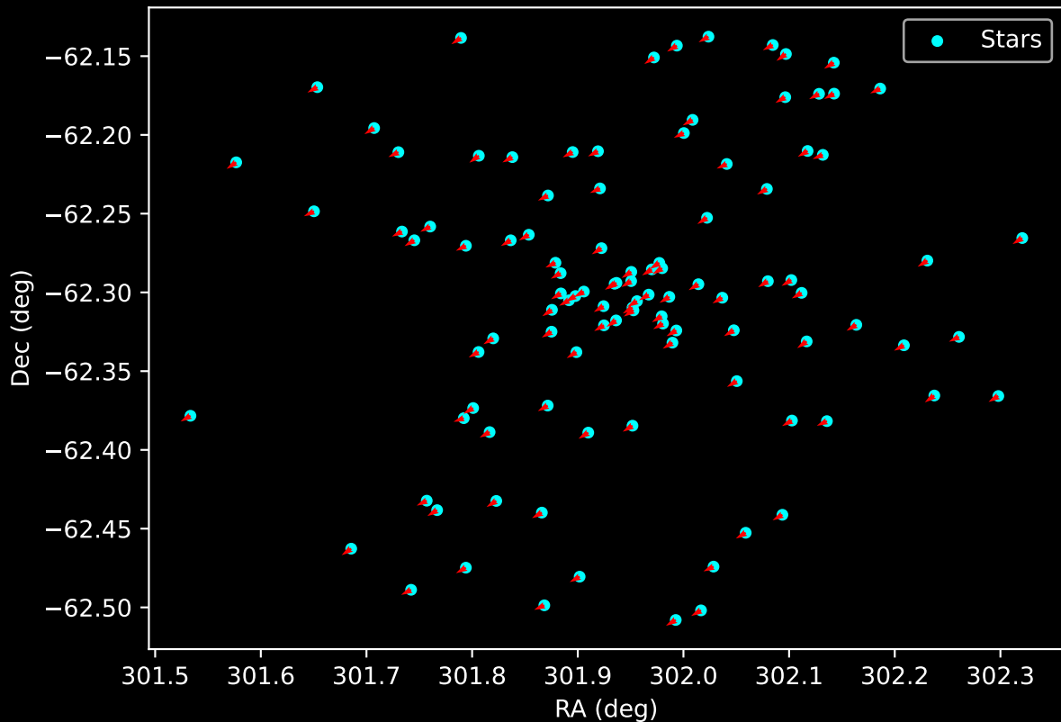
Gaia Cluster: [Basel_18] Proper Motion Vectors for Gaia Star Field (n= 104)
