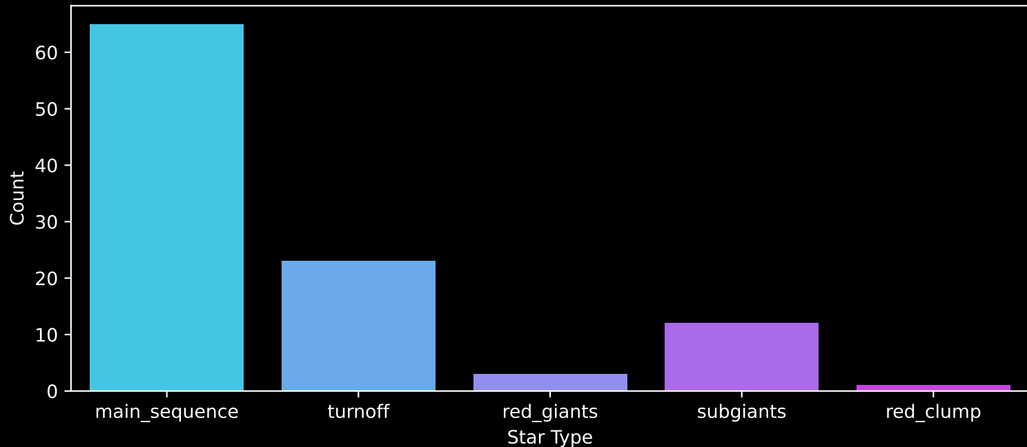
Gaia Cluster: [Basel_18] Count plot of Star Type
