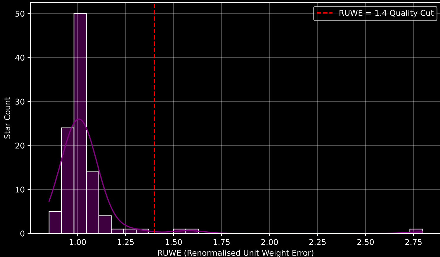
Gaia Cluster: [Basel_18] RUWE Distribution (n= 103)
