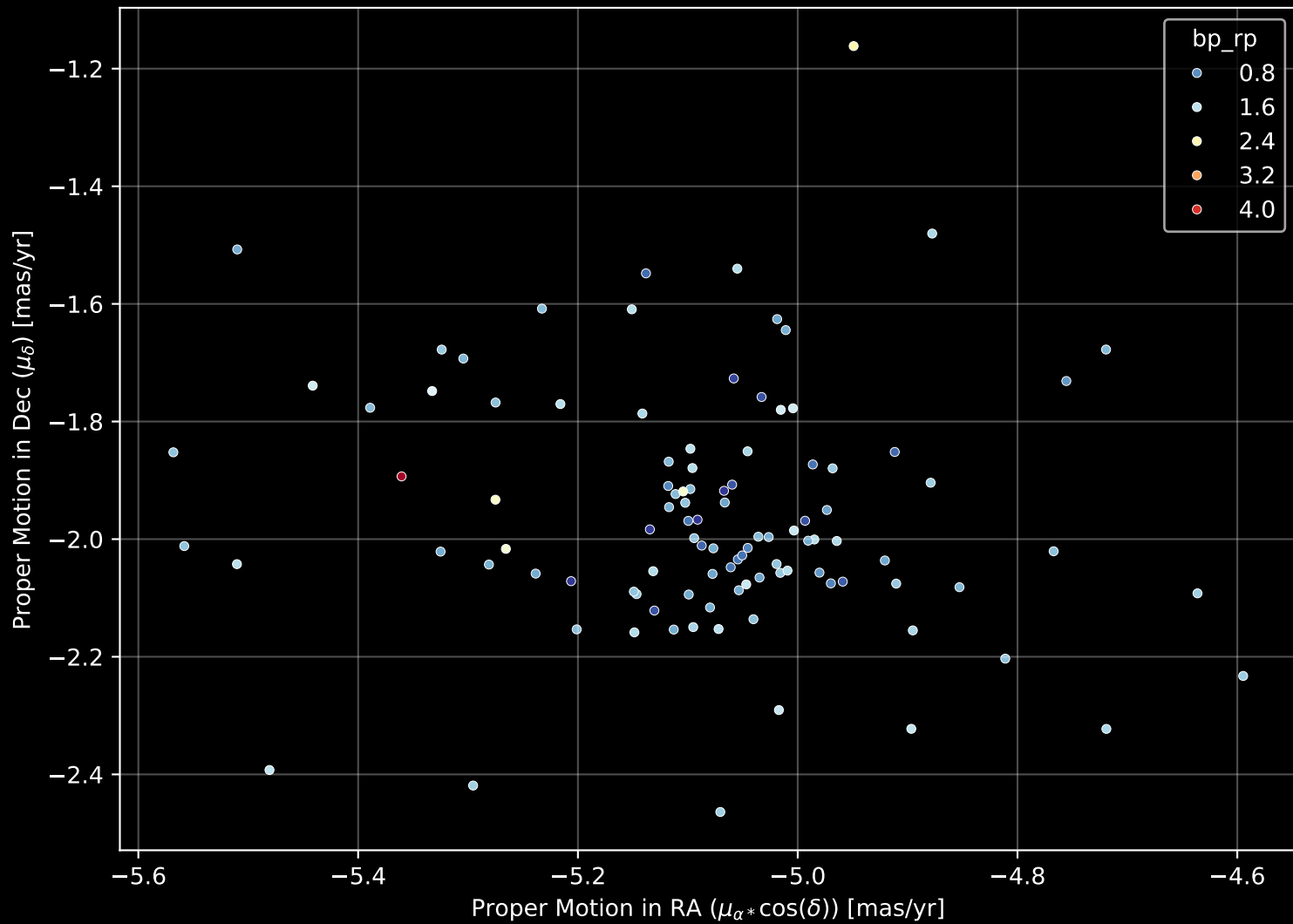
Gaia Cluster: [Basel_18] Proper Motion Diagram (n= 104)
