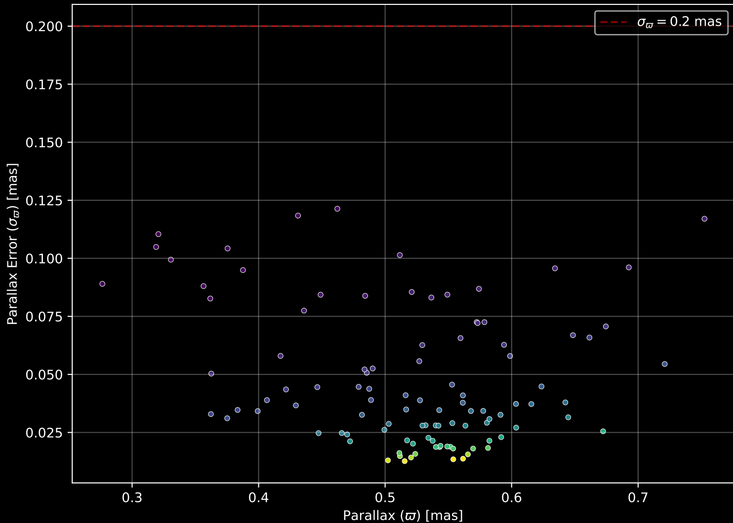
Gaia Cluster: [Basel_18] Parallax Quality (n= 104)
