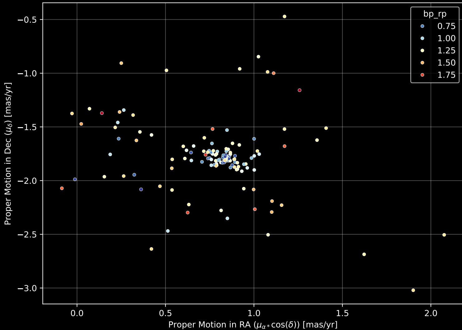
Gaia Cluster: [Basel_4] Proper Motion Diagram (n= 132)
