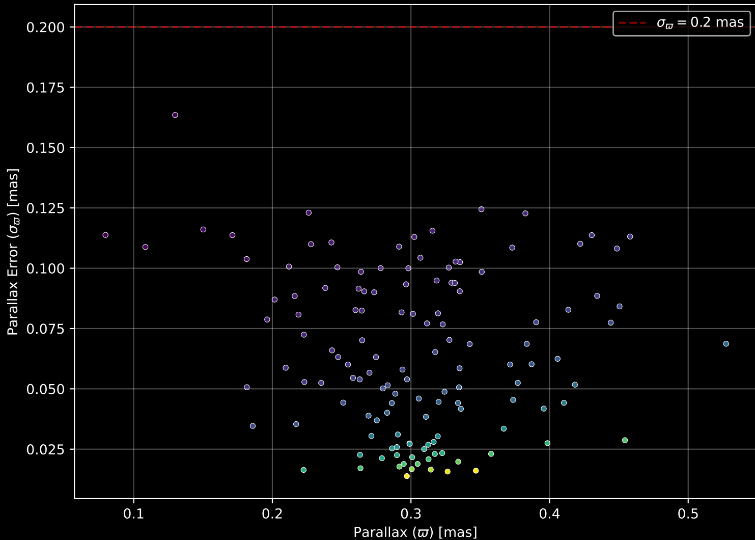
Gaia Cluster: [Basel_4] Parallax Quality (n= 132)
