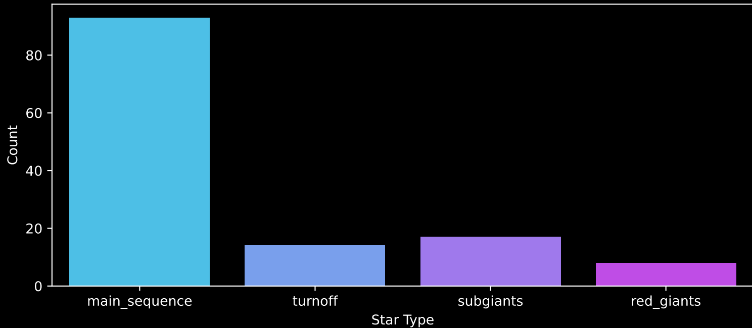
Gaia Cluster: [Basel_4] Count plot of Star Type
