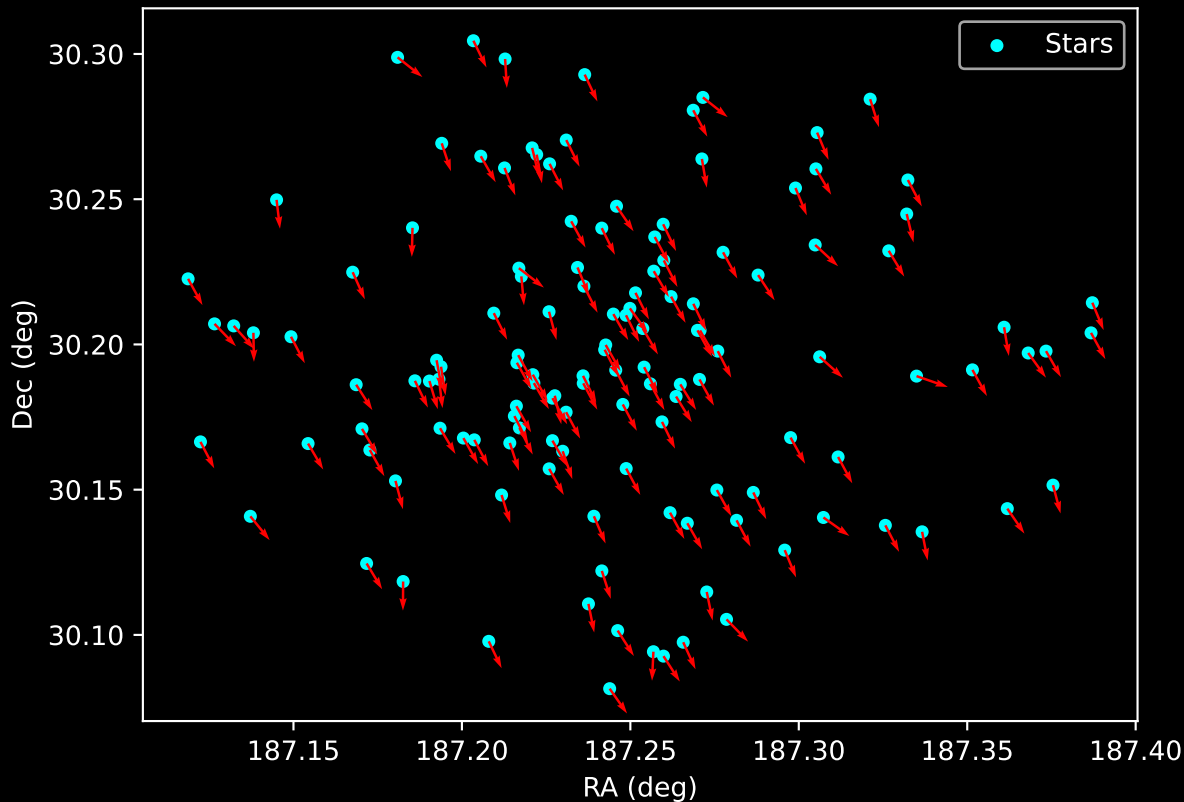
Gaia Cluster: [Basel_4] Proper Motion Vectors for Gaia Star Field (n= 132)
