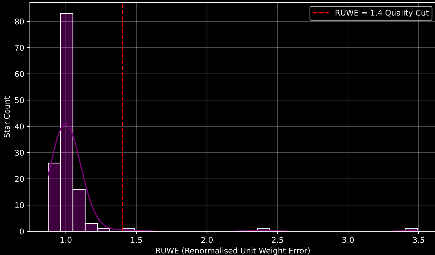
Gaia Cluster: [Basel_4] RUWE Distribution (n= 132)
