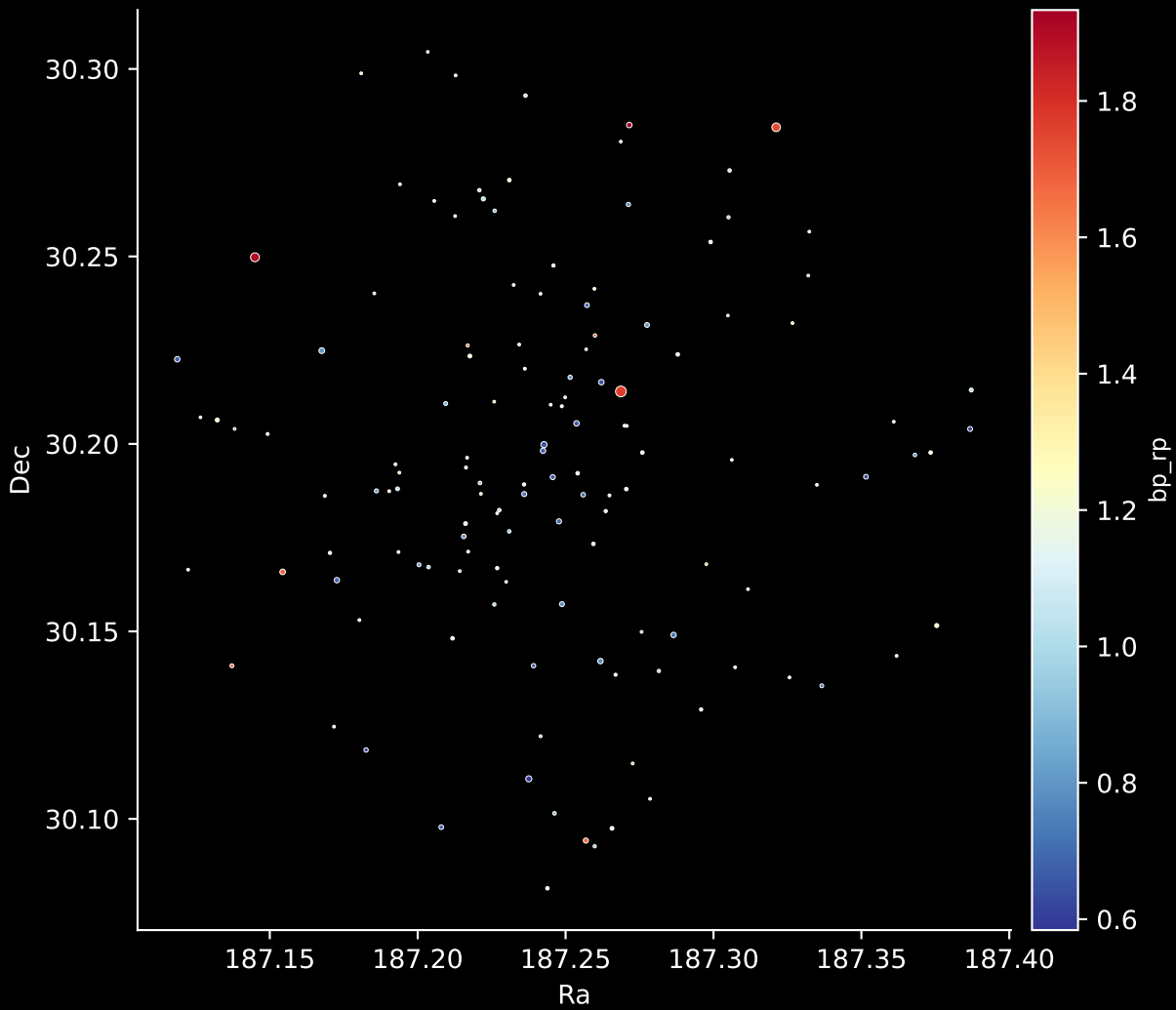
Gaia Cluster: [Basel_4] Stars: 132
