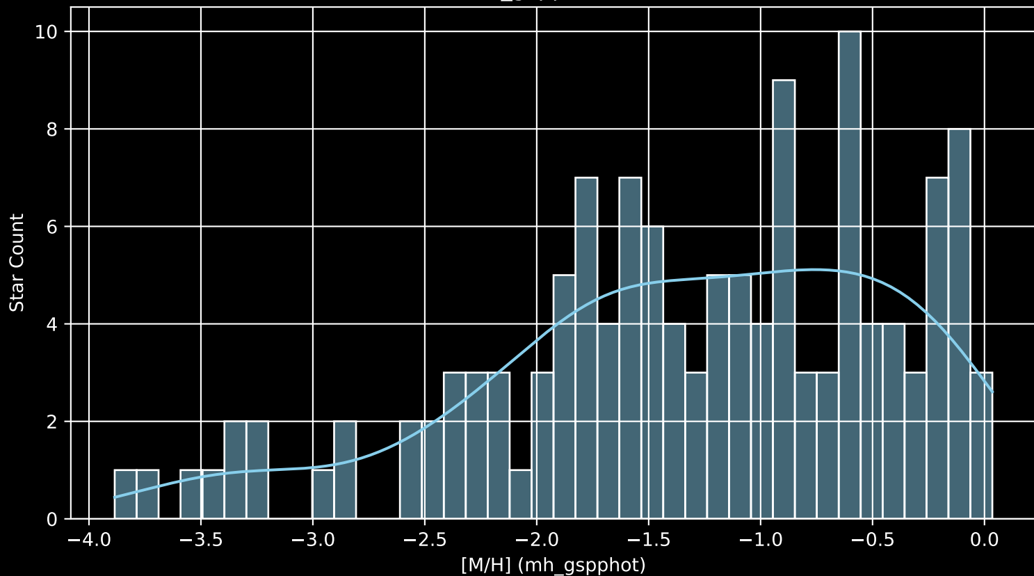
Gaia Cluster: [Basel_4 [M/H] (mh_gspphot) (n= 132)
