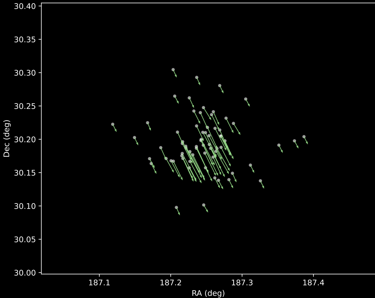
Gaia DR3 Cluster 5 Proper Motion Vectors (n=68)
