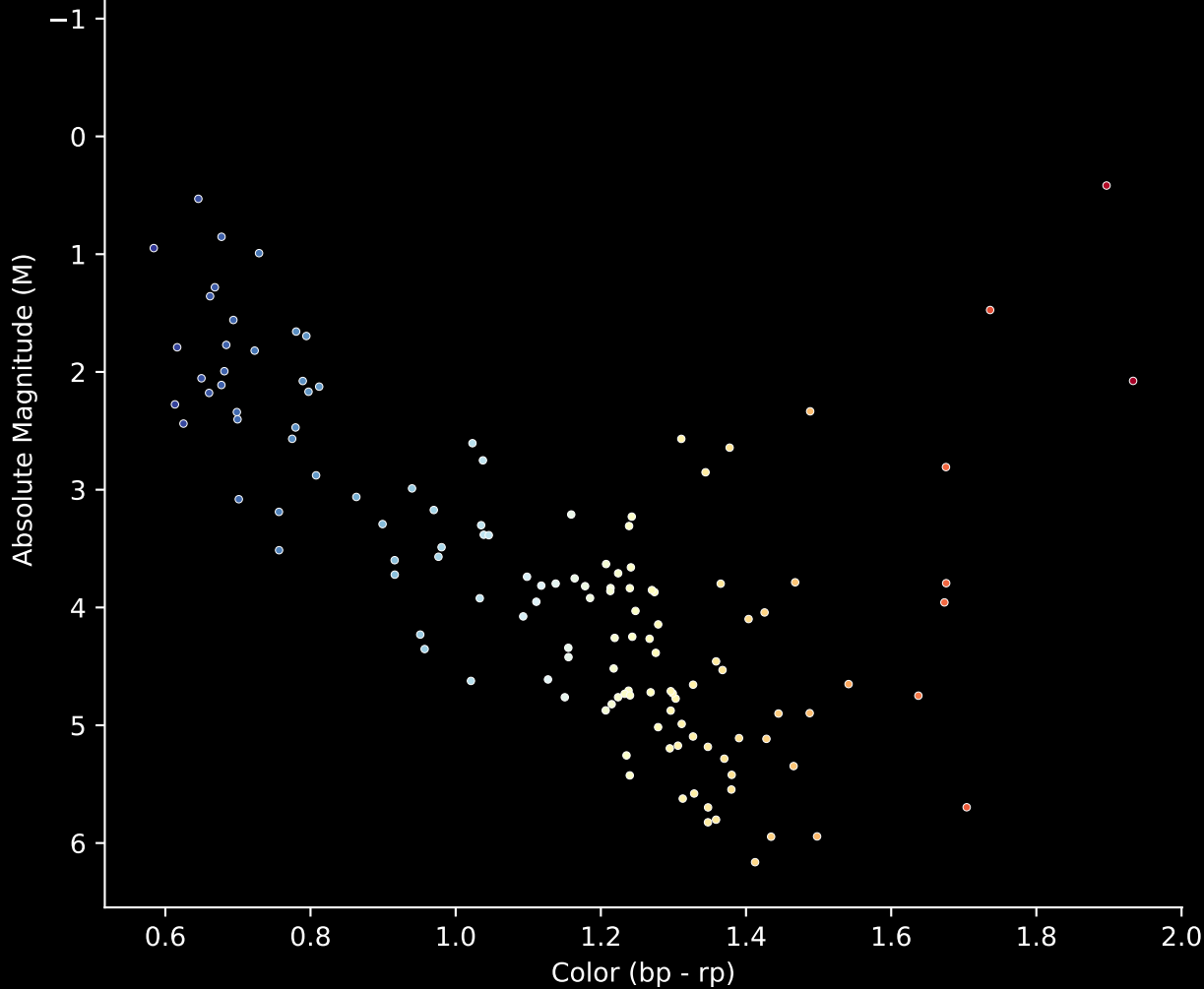
Gaia Cluster: [Basel_4] Stars (n= 132) Hertzprung-Russel Diagram
