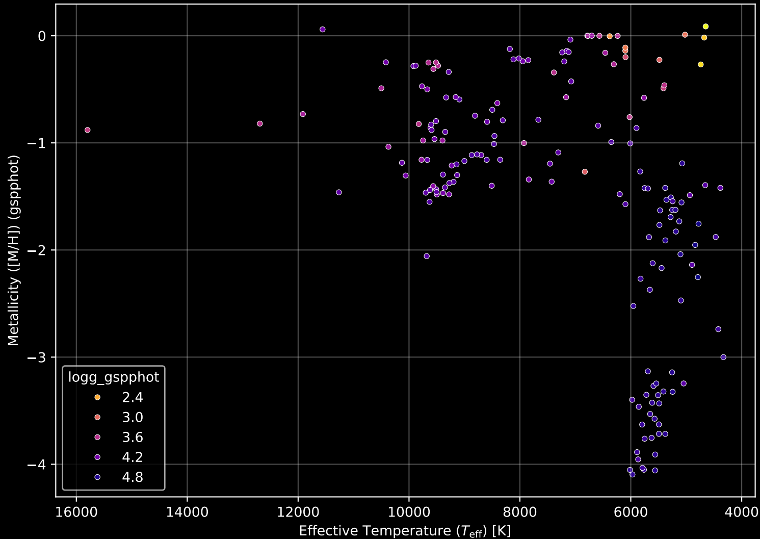
Gaia Cluster: [Berkeley_1] Stellar Population Parameters (n= 175)
