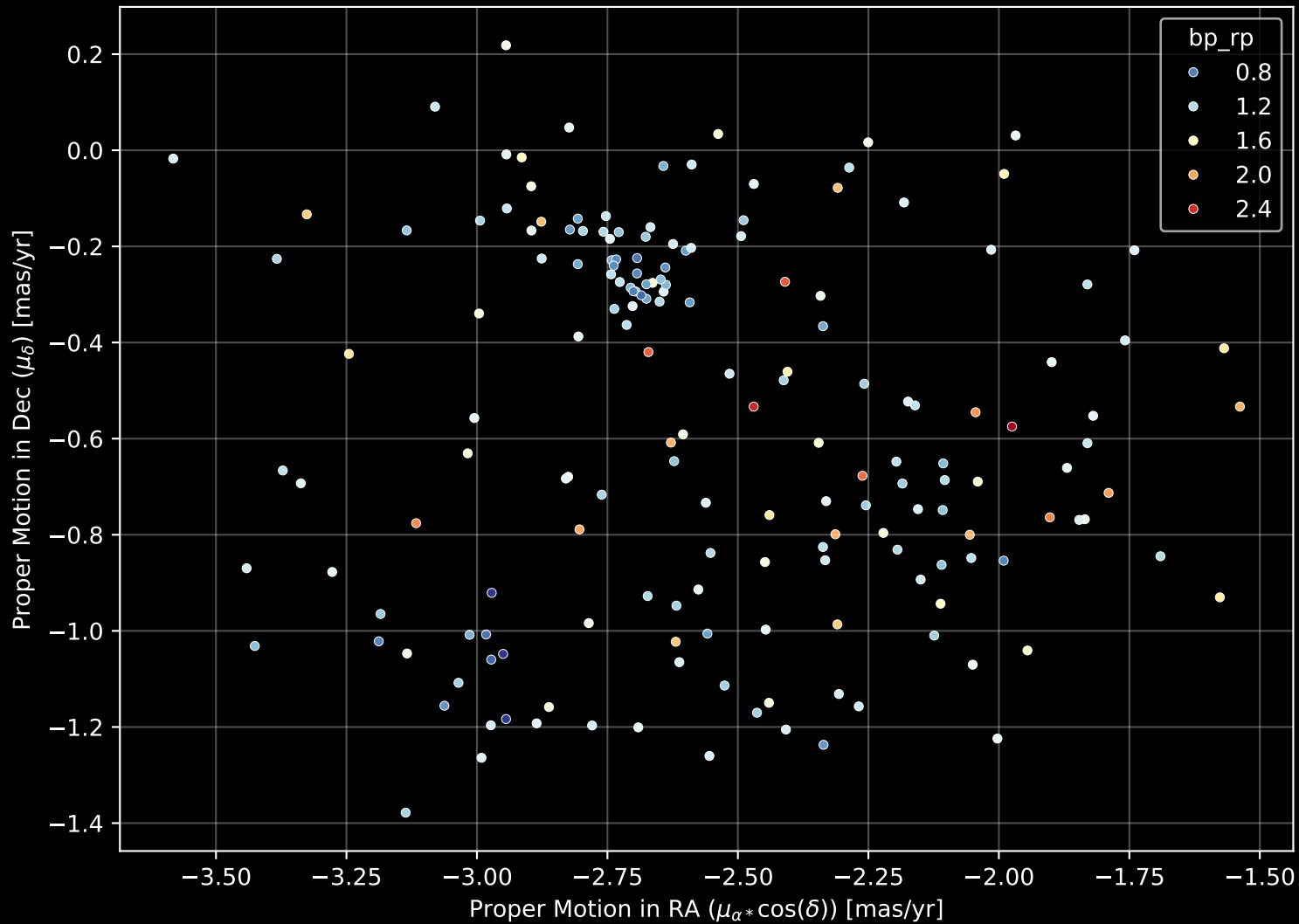
Gaia Cluster: [Berkeley_1] Proper Motion Diagram (n= 175)
