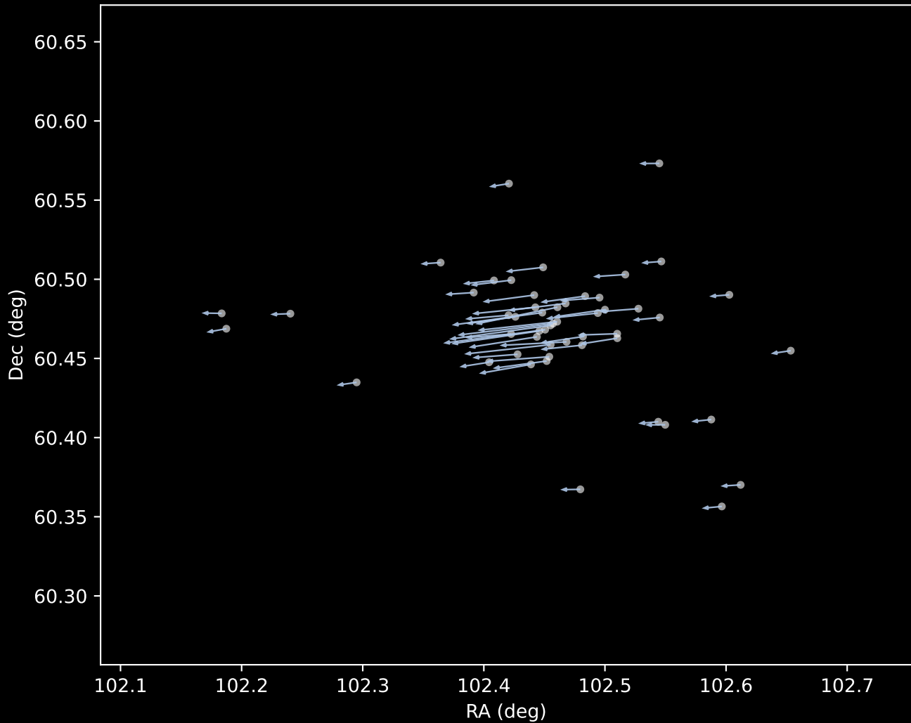
Gaia DR3 Cluster 1 Proper Motion Vectors (n=52)
