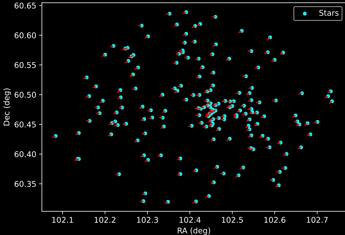
Gaia Cluster: [Berkeley_1] Proper Motion Vectors for Gaia Star Field (n= 175)
