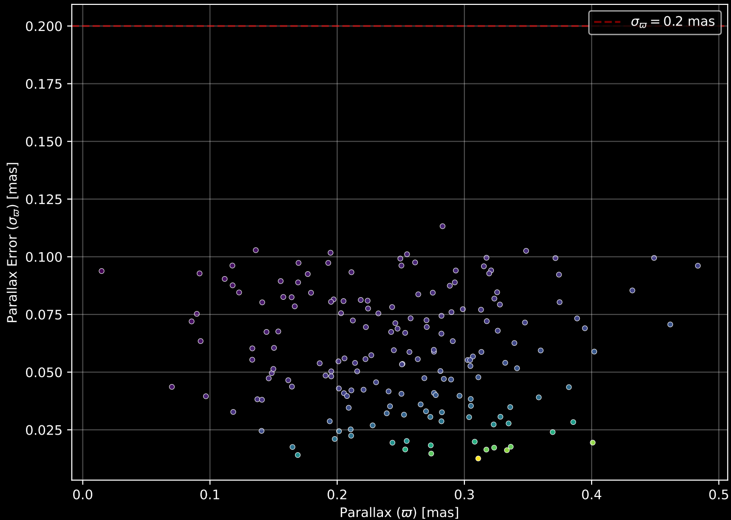
Gaia Cluster: [Berkeley_1] Parallax Quality (n= 175)
