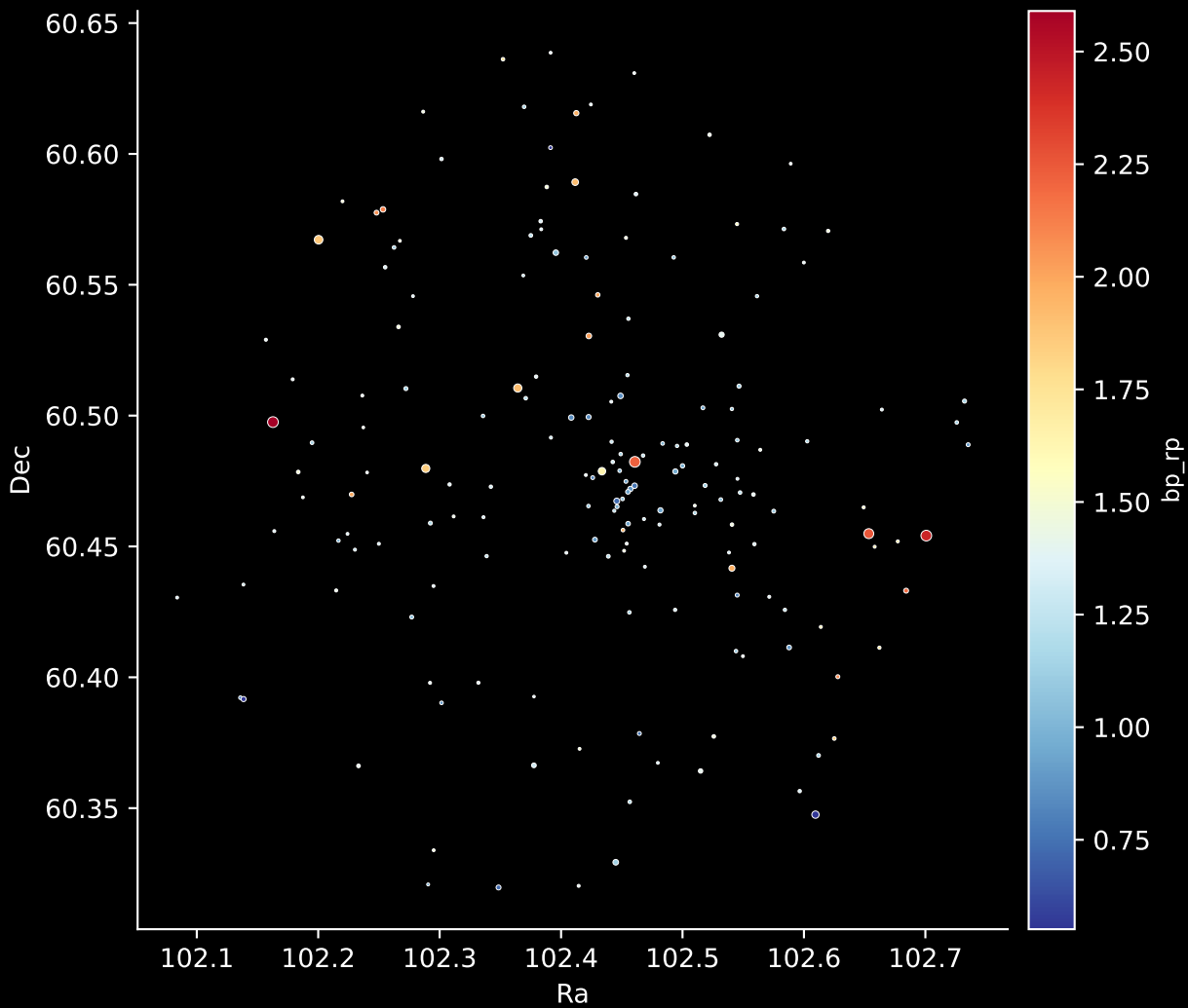
Gaia Cluster: [Berkeley_1] Stars: 175
