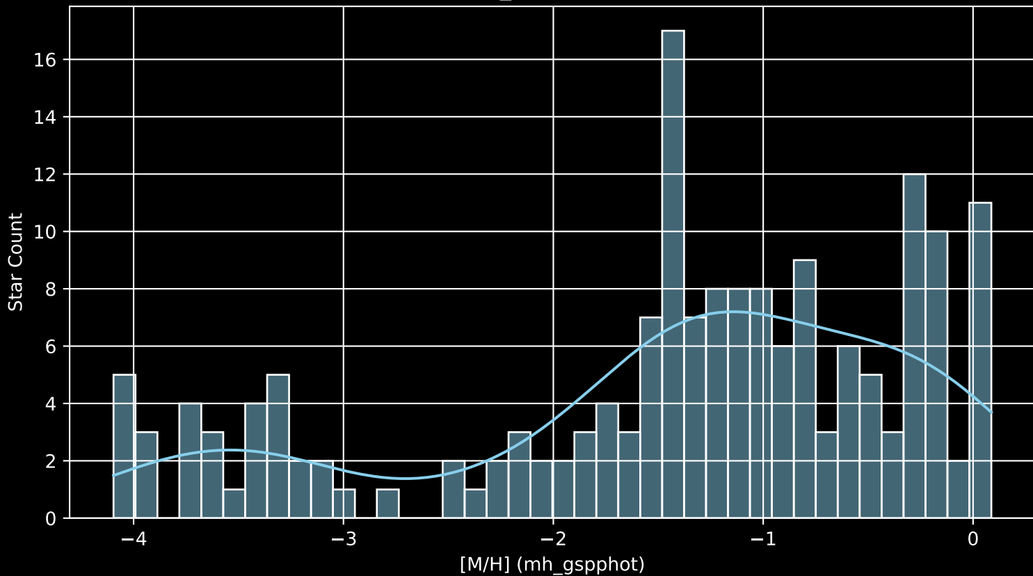
Gaia Cluster: [Berkeley_1 [M/H] (mh_gspphot) (n= 175)
