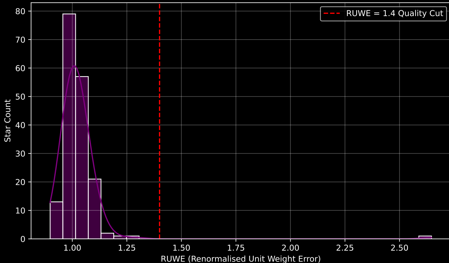
Gaia Cluster: [Berkeley_1] RUWE Distribution (n= 175)
