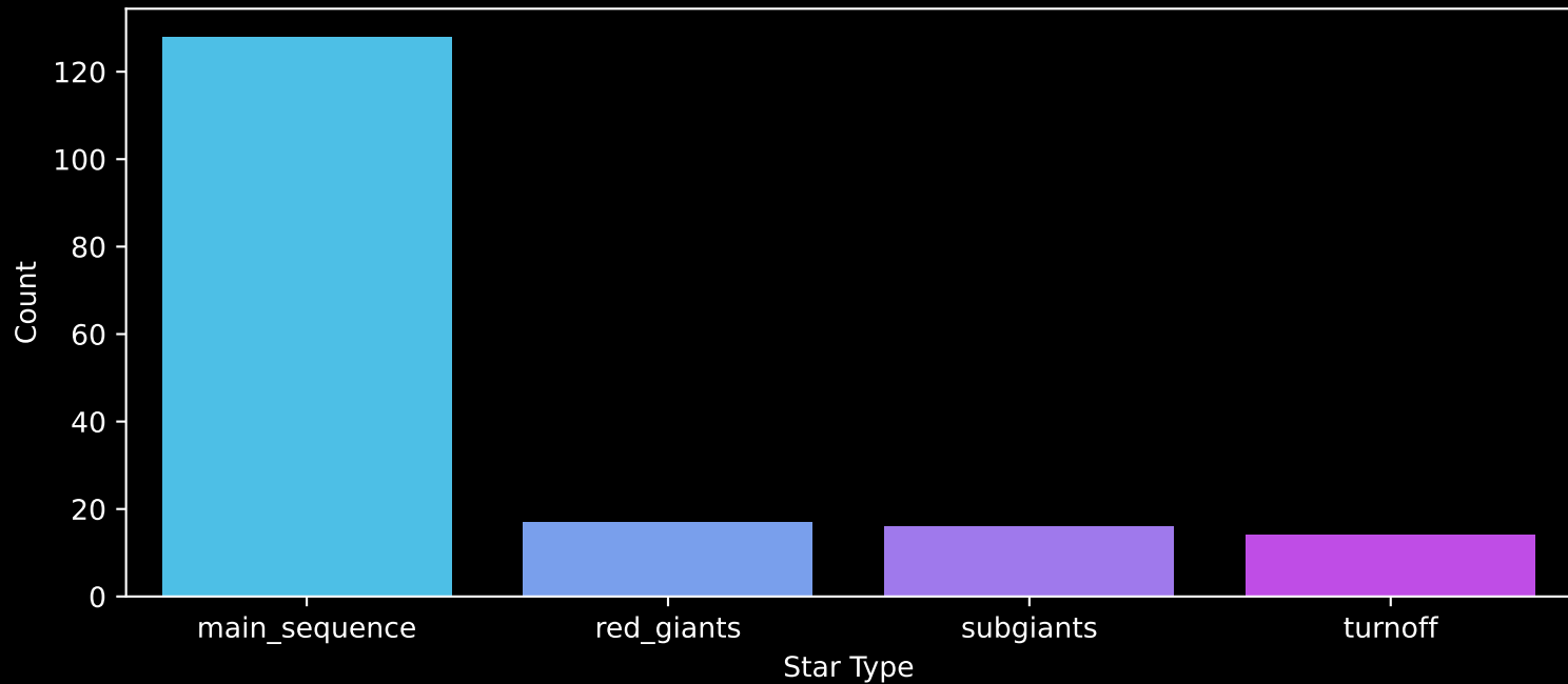
Gaia Cluster: [Berkeley_1] Count plot of Star Type
