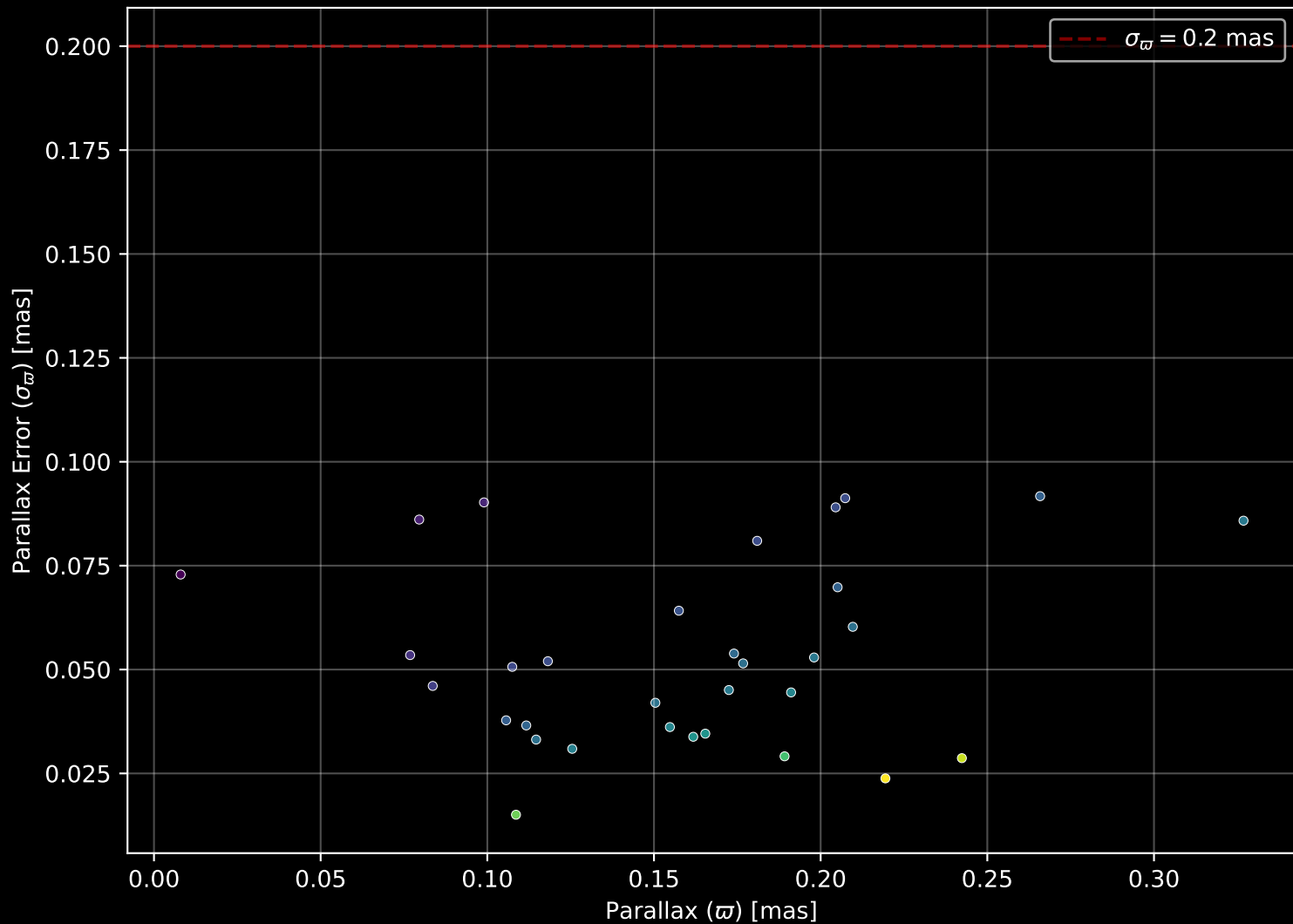
Gaia Cluster: [Berkeley_103] Parallax Quality (n= 32)
