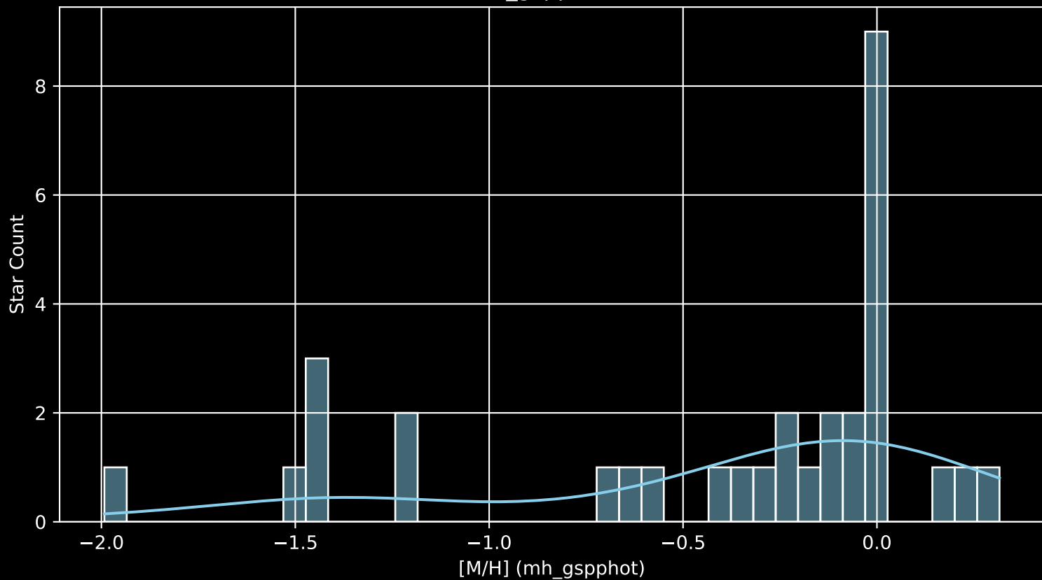
Gaia Cluster: [Berkeley_103 [M/H] (mh_gspphot) (n= 32)
