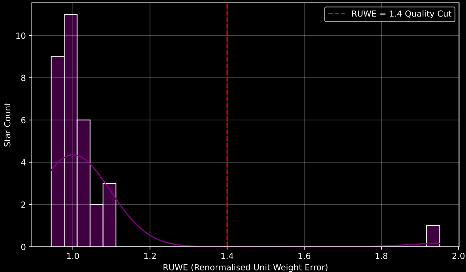
Gaia Cluster: [Berkeley_103] RUWE Distribution (n= 32)
