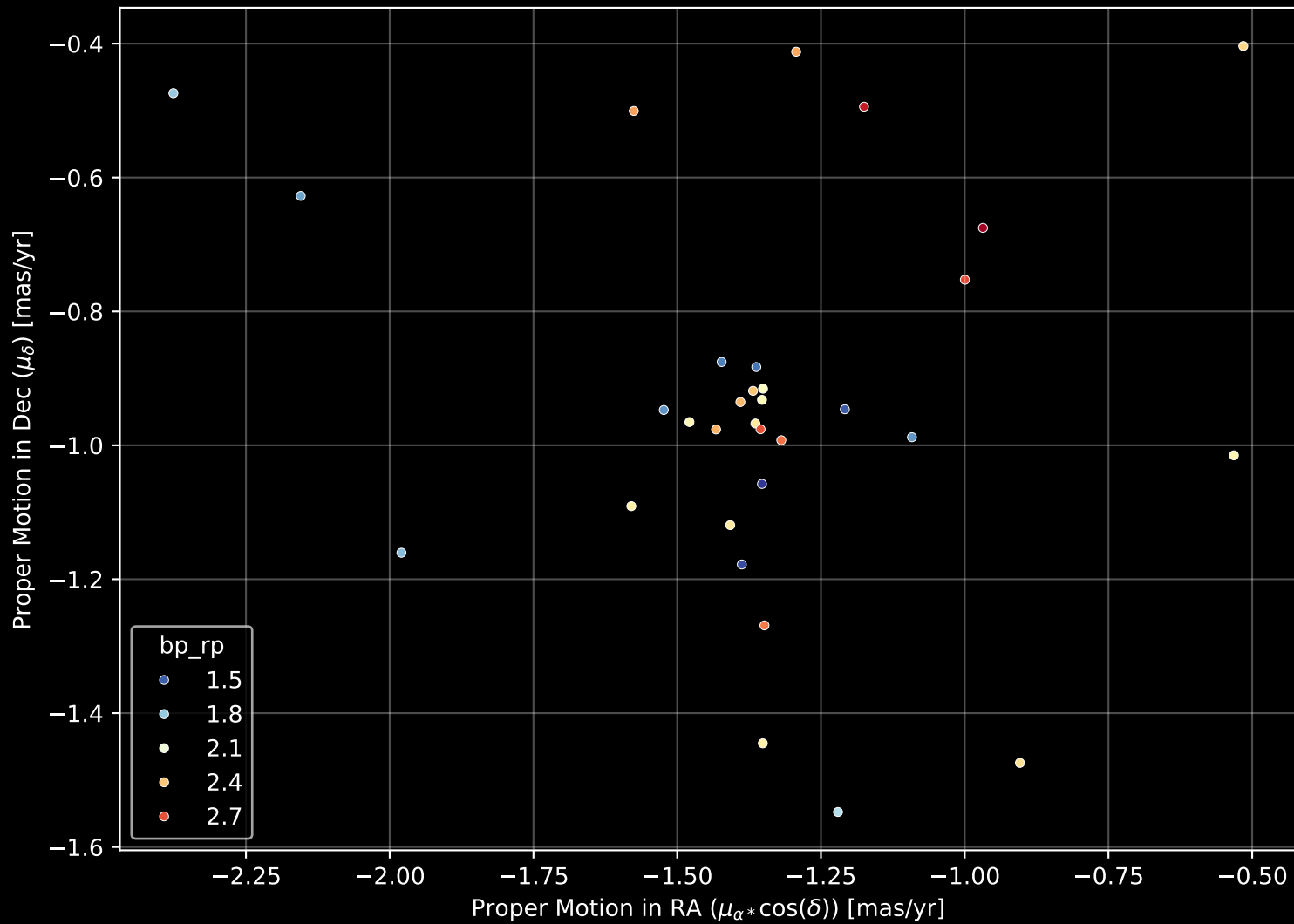
Gaia Cluster: [Berkeley_103] Proper Motion Diagram (n= 32)
