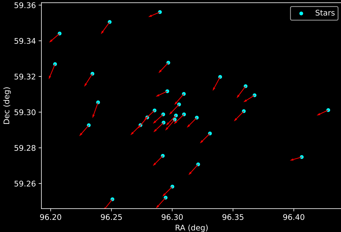
Gaia Cluster: [Berkeley_103] Proper Motion Vectors for Gaia Star Field (n= 32)
