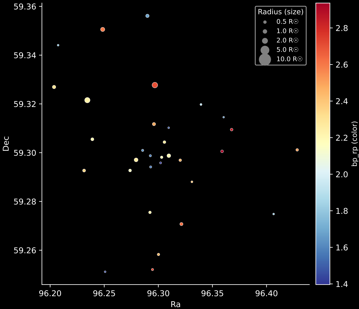
Gaia Cluster: [Berkeley_103] Stars: 32
