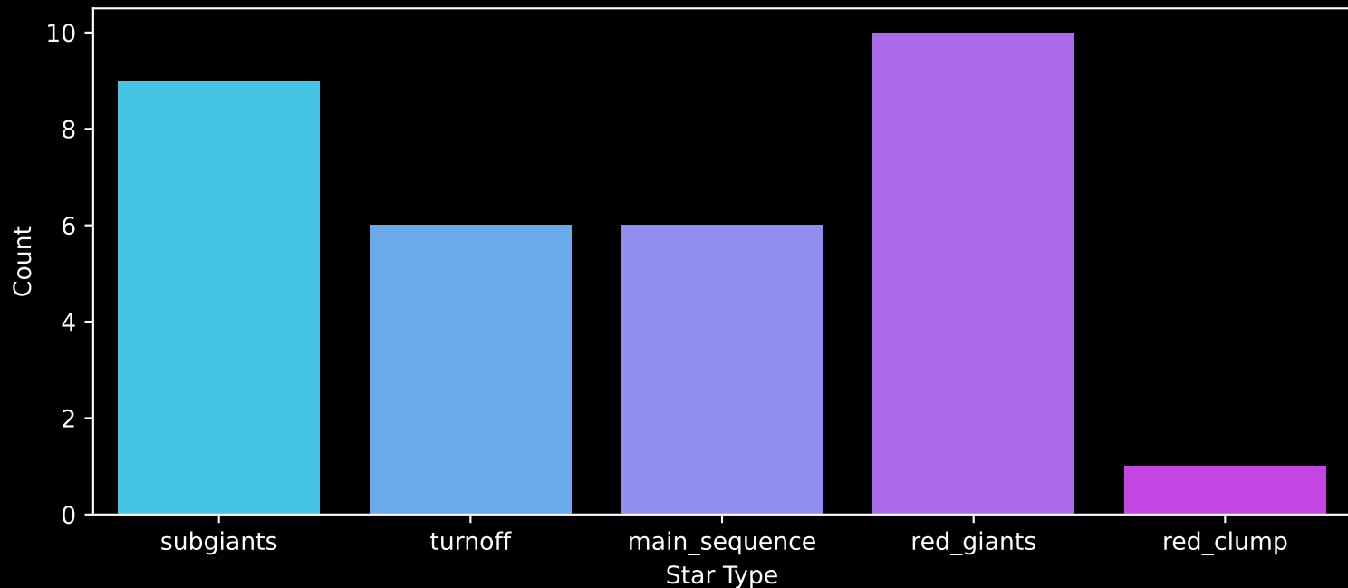
Gaia Cluster: [Berkeley_103] Count plot of Star Type
