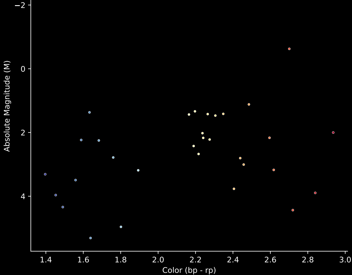
Gaia Cluster: [Berkeley_103] Stars (n= 32) Hertzprung-Russel Diagram
