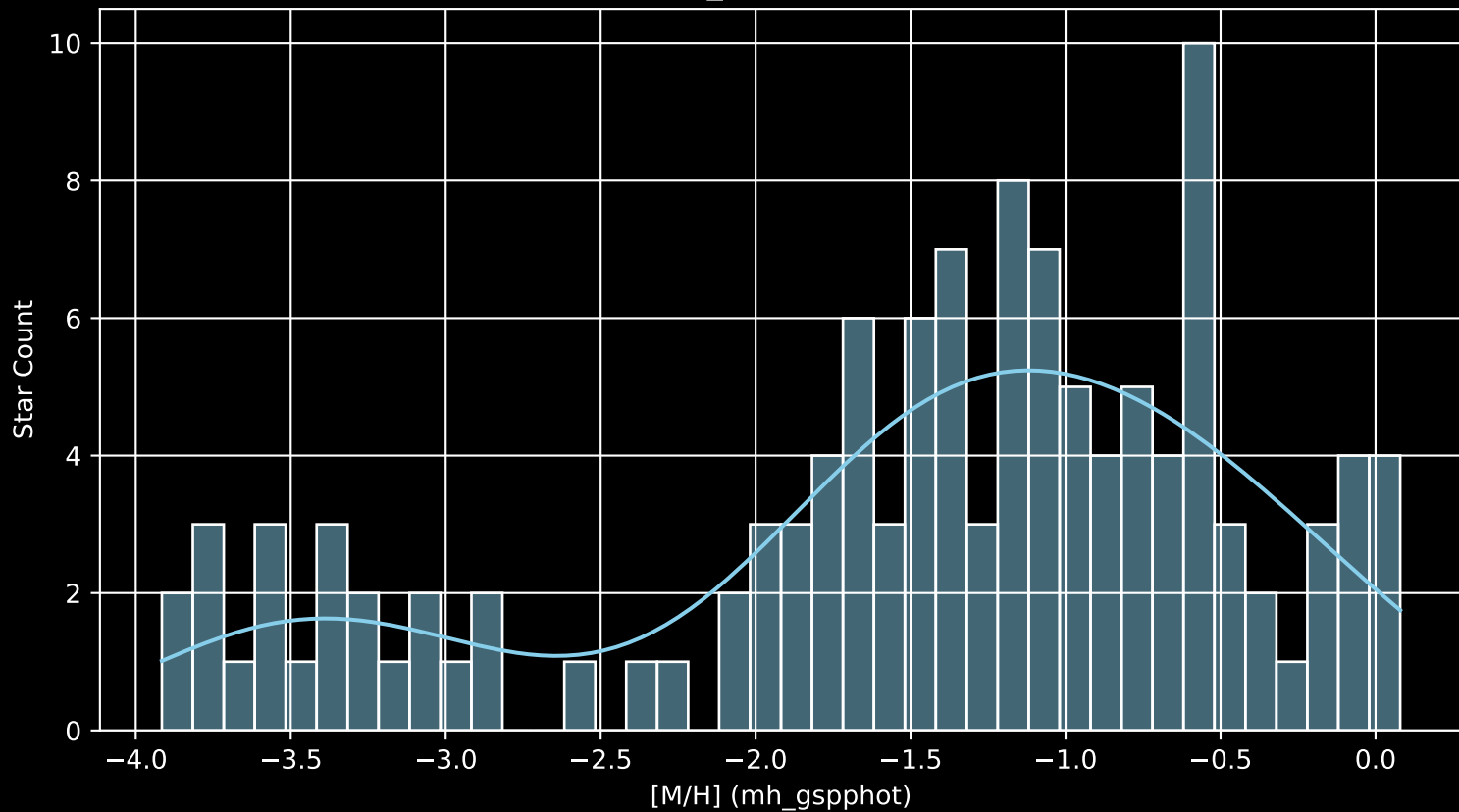
Gaia Cluster: [Berkeley_11 [M/H] (mh_gspphot) (n= 121)
