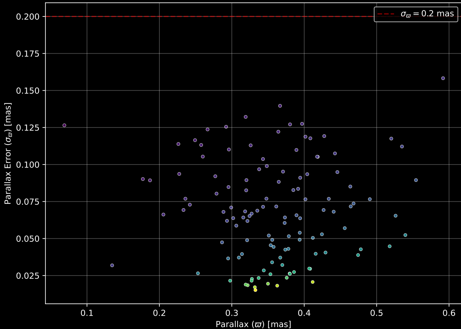
Gaia Cluster: [Berkeley_11] Parallax Quality (n= 121)
