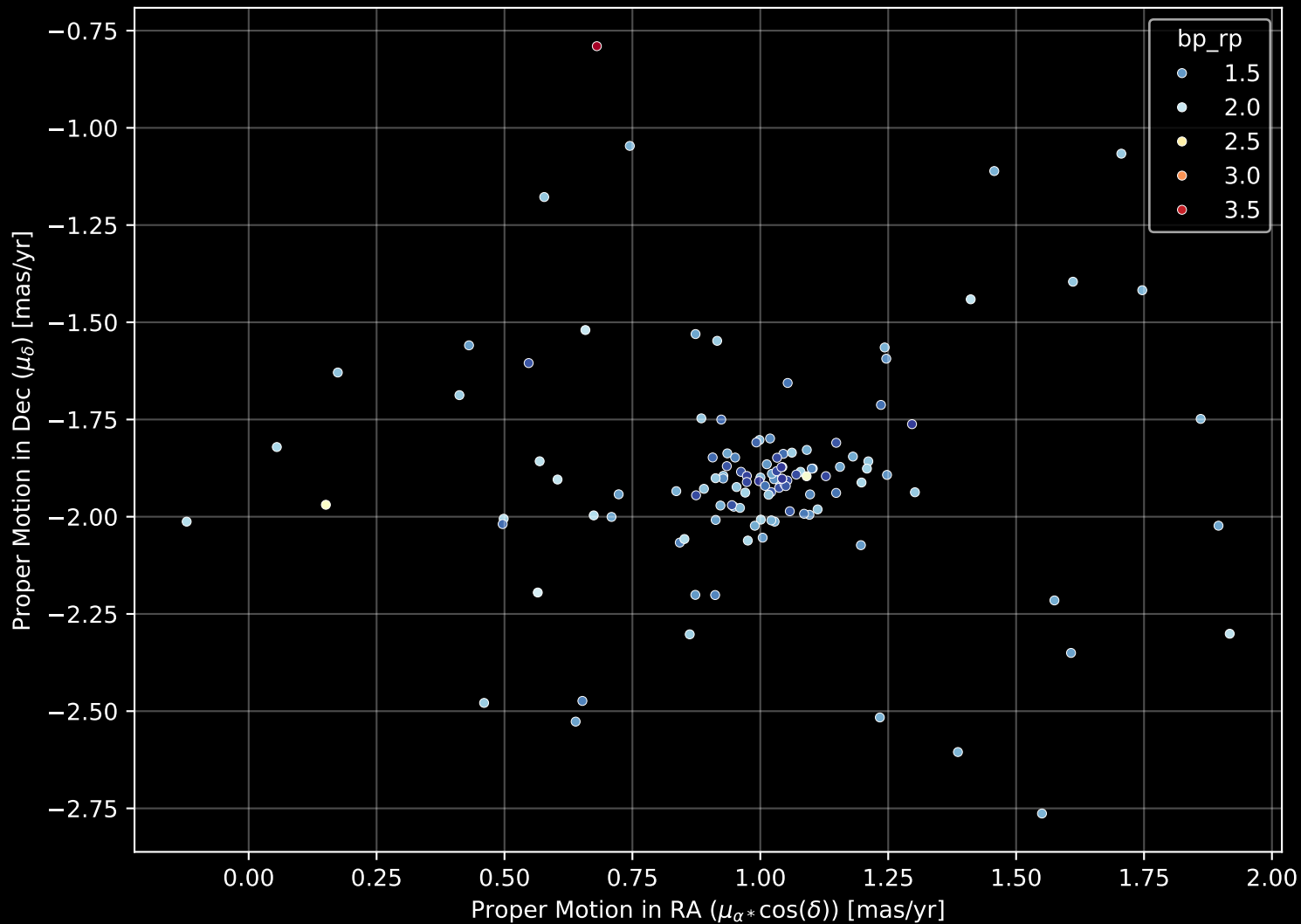
Gaia Cluster: [Berkeley_11] Proper Motion Diagram (n= 121)
