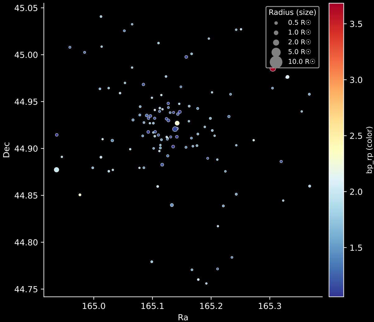
Gaia Cluster: [Berkeley_11] Stars: 121
