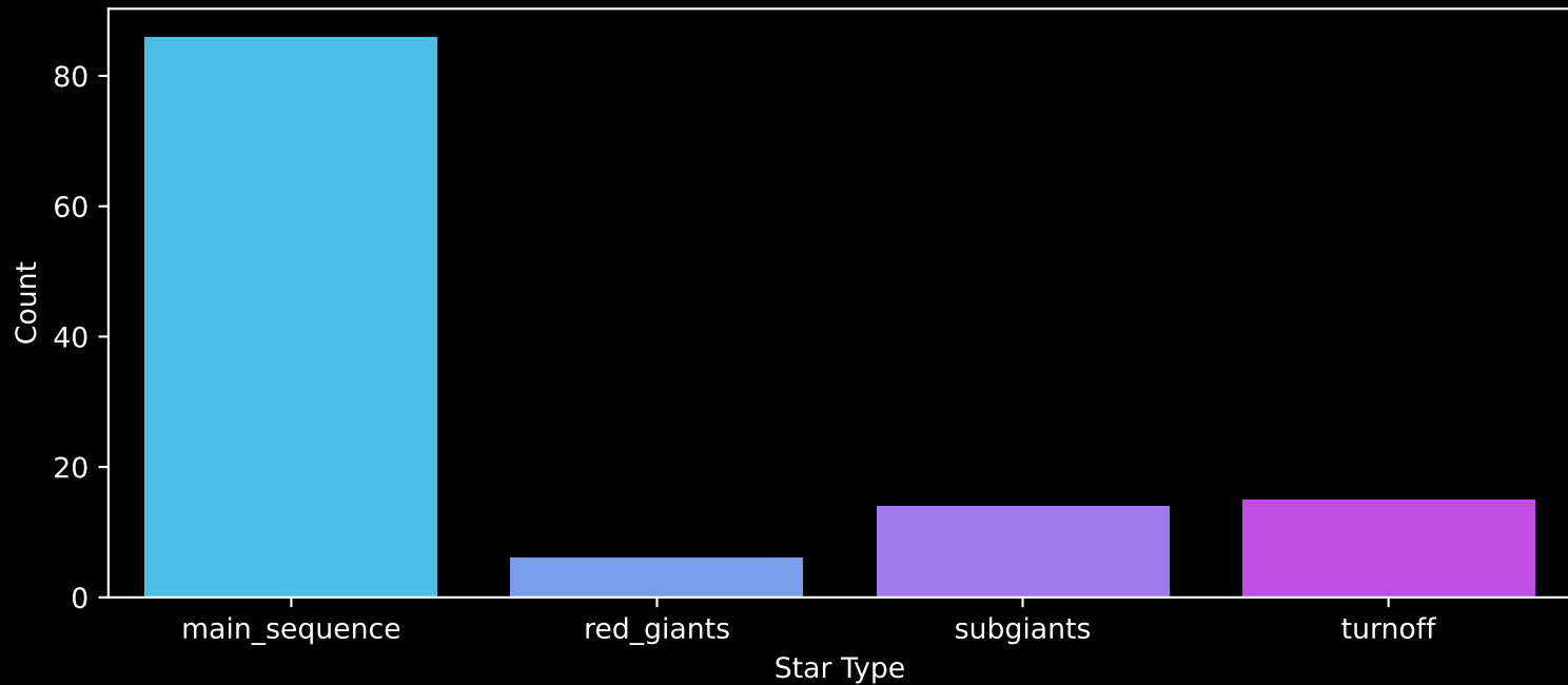
Gaia Cluster: [Berkeley_11] Count plot of Star Type
