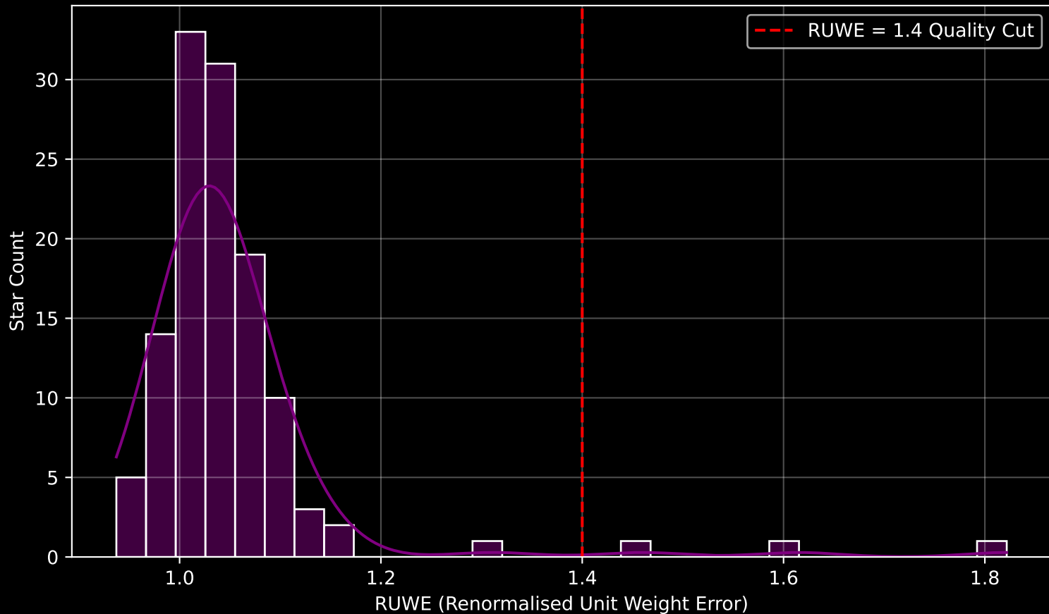
Gaia Cluster: [Berkeley_11] RUWE Distribution (n= 121)
