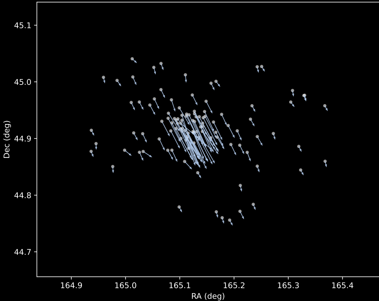
Gaia DR3 Cluster 1 Proper Motion Vectors (n=109)
