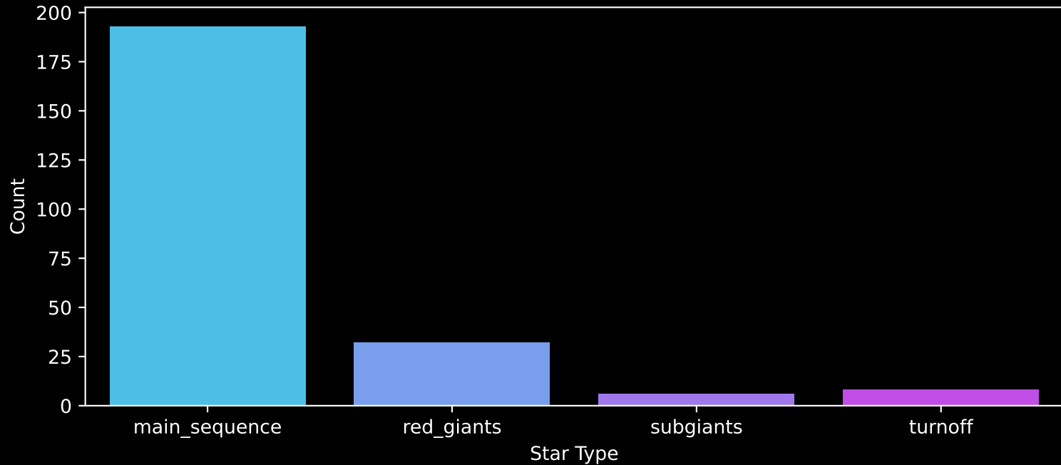
Gaia Cluster: [Berkeley_14] Count plot of Star Type
