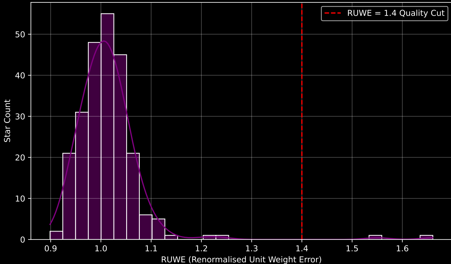
Gaia Cluster: [Berkeley_14] RUWE Distribution (n= 239)
