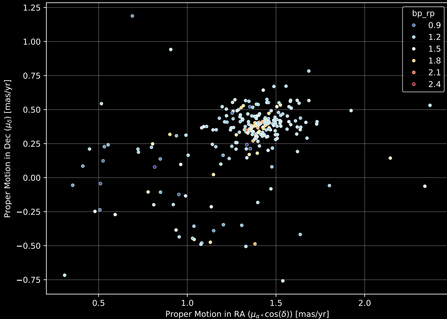
Gaia Cluster: [Berkeley_14] Proper Motion Diagram (n= 239)
