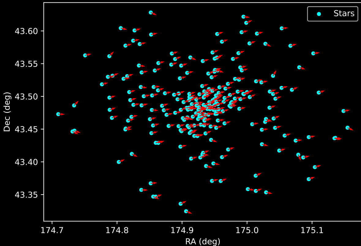
Gaia Cluster: [Berkeley_14] Proper Motion Vectors for Gaia Star Field (n= 239)
