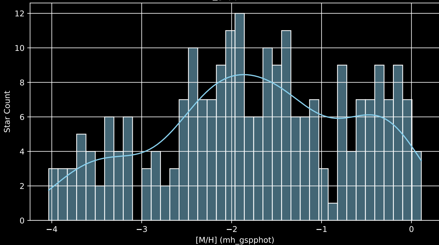
Gaia Cluster: [Berkeley_14 [M/H] (mh_gspphot) (n= 239)
