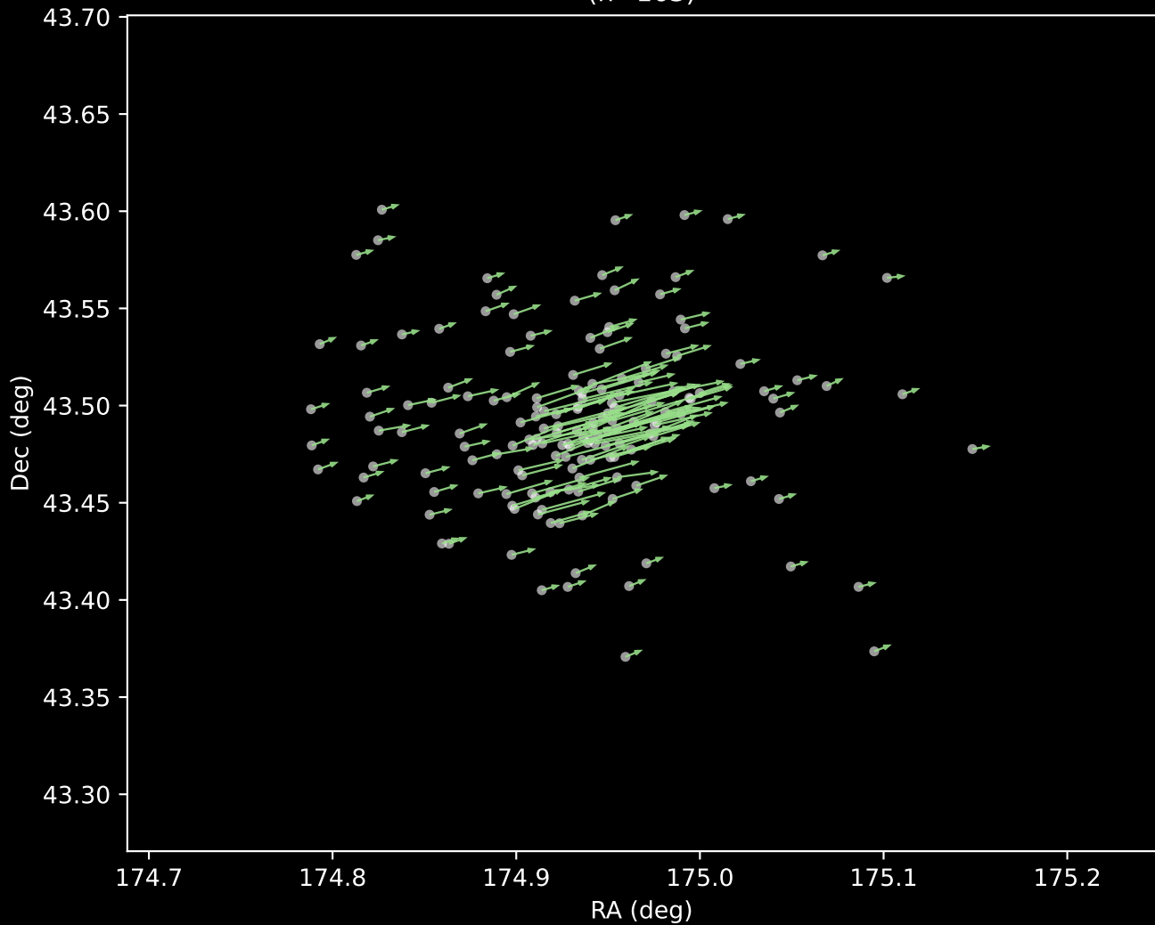
Gaia DR3 Cluster 5 Proper Motion Vectors (n=163)
