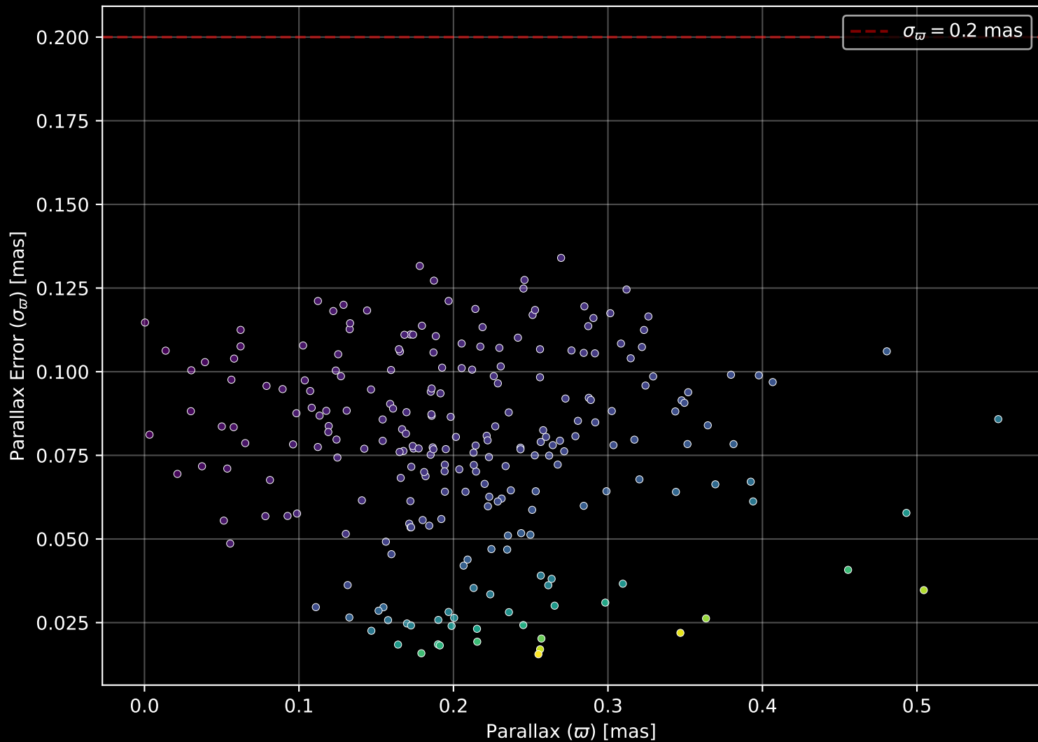
Gaia Cluster: [Berkeley_14] Parallax Quality (n= 239)
