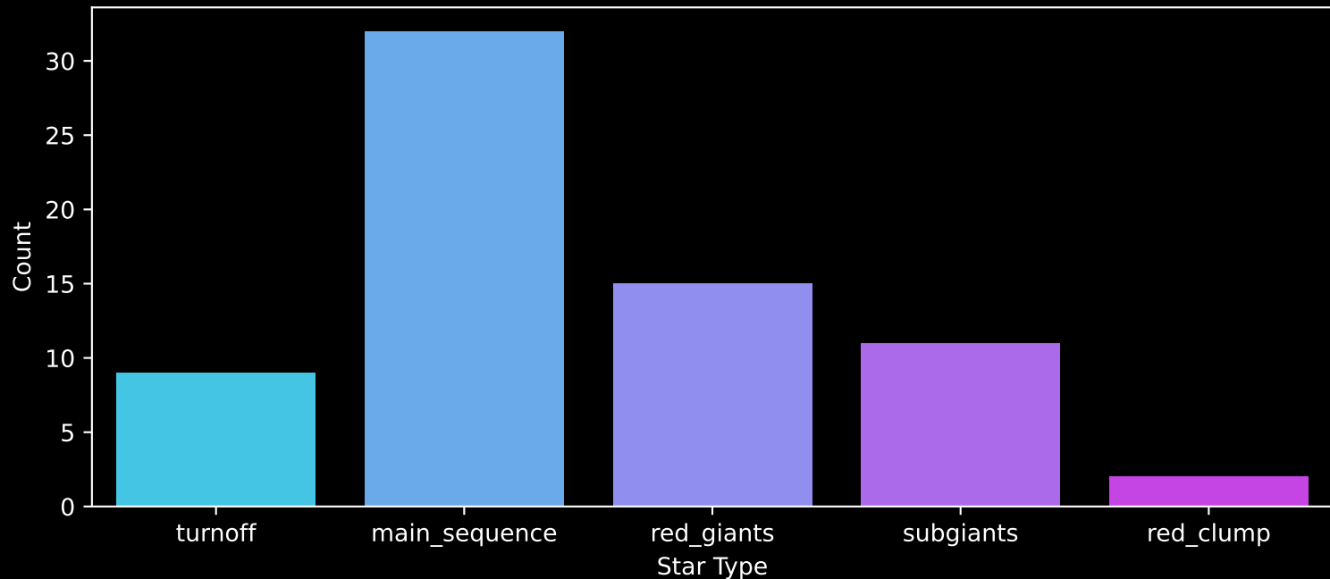
Gaia Cluster: [Berkeley_2] Count plot of Star Type
