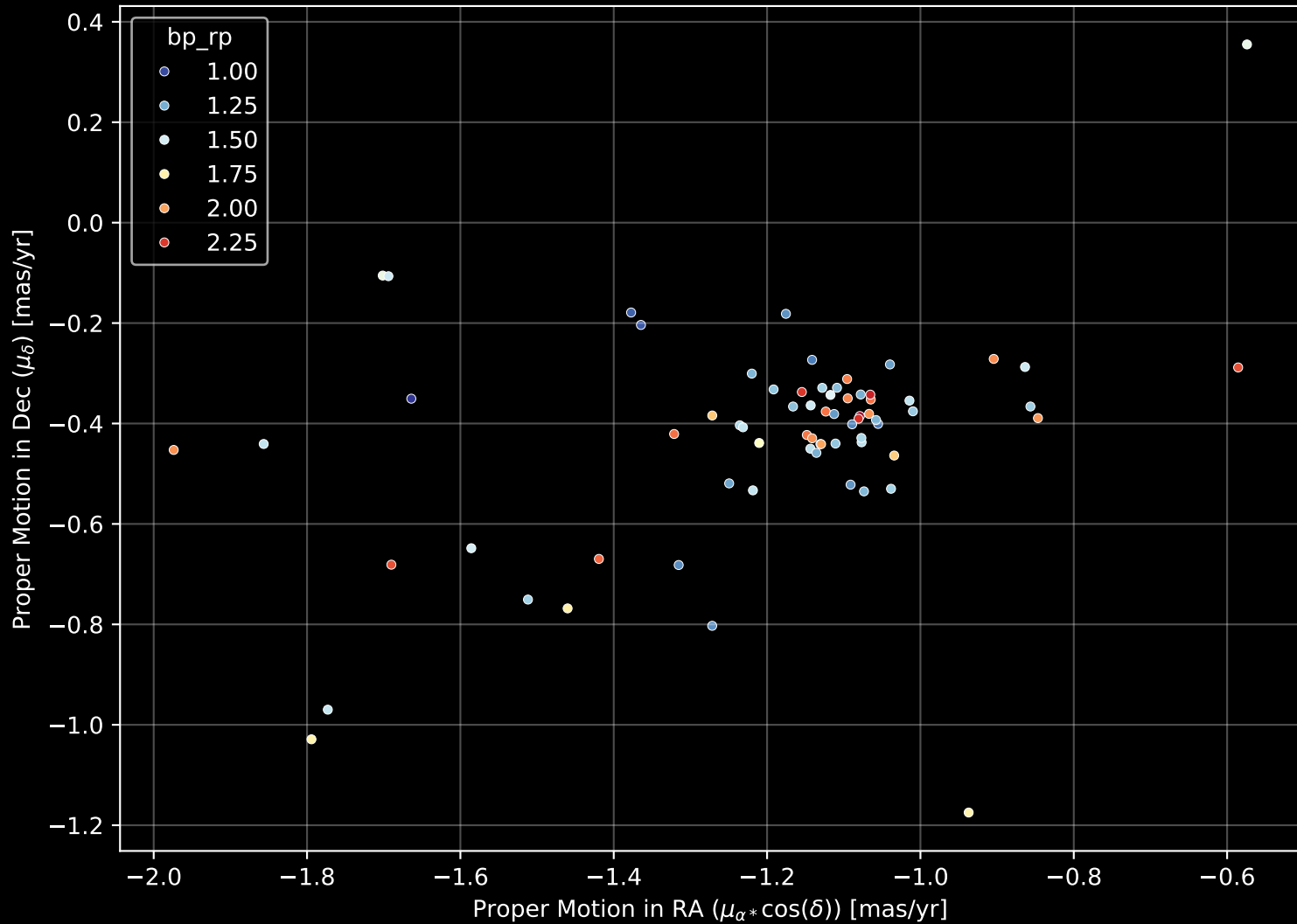
Gaia Cluster: [Berkeley_2] Proper Motion Diagram (n= 69)
