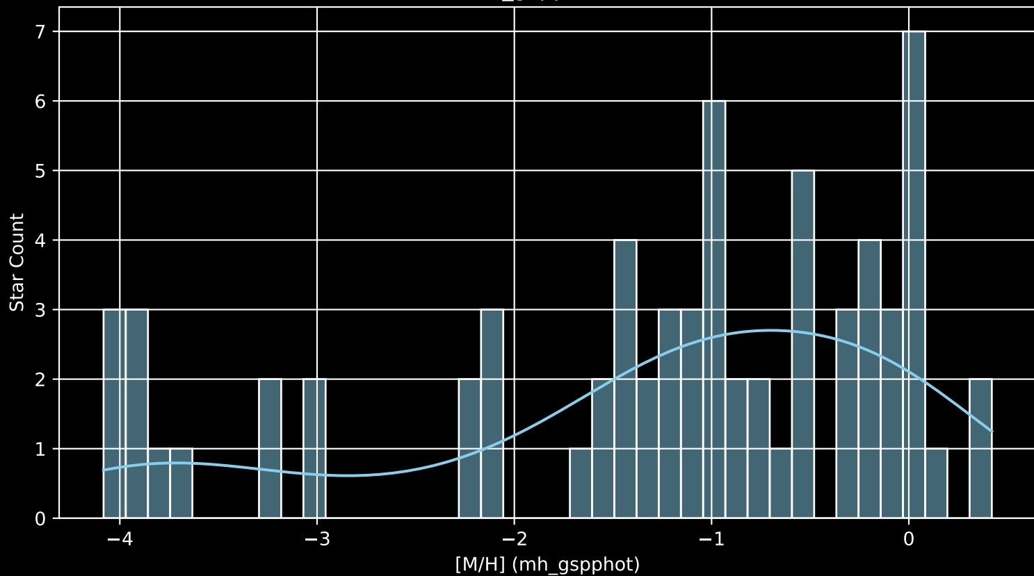
Gaia Cluster: [Berkeley_2 [M/H] (mh_gspphot) (n= 68)
