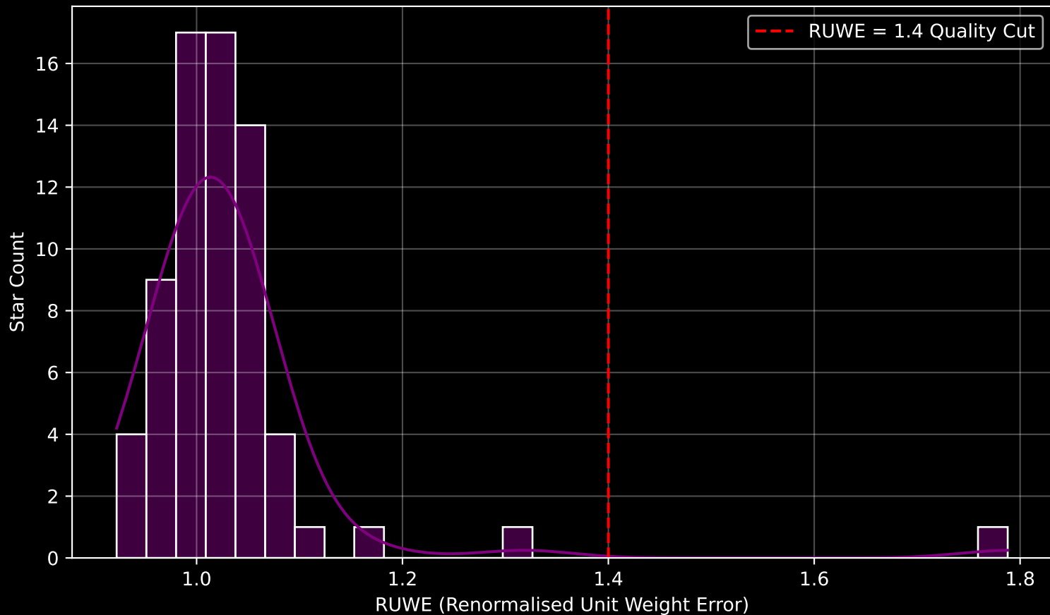
Gaia Cluster: [Berkeley_2] RUWE Distribution (n= 69)
