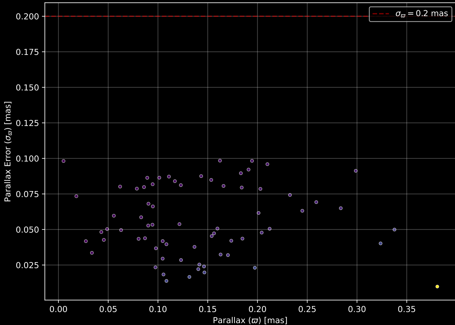
Gaia Cluster: [Berkeley_2] Parallax Quality (n= 69)
