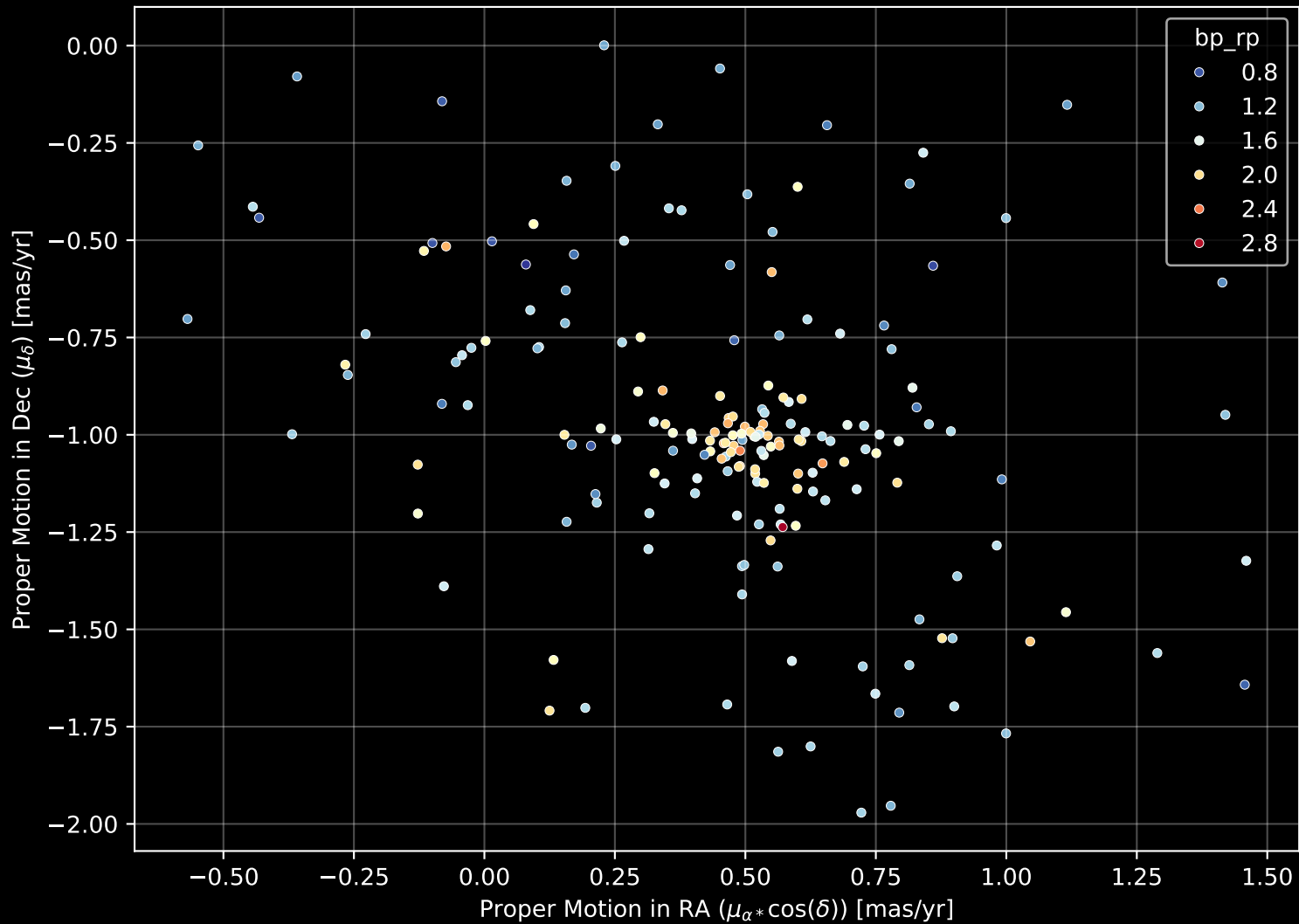
Gaia Cluster: [Berkeley_21] Proper Motion Diagram (n= 188)
