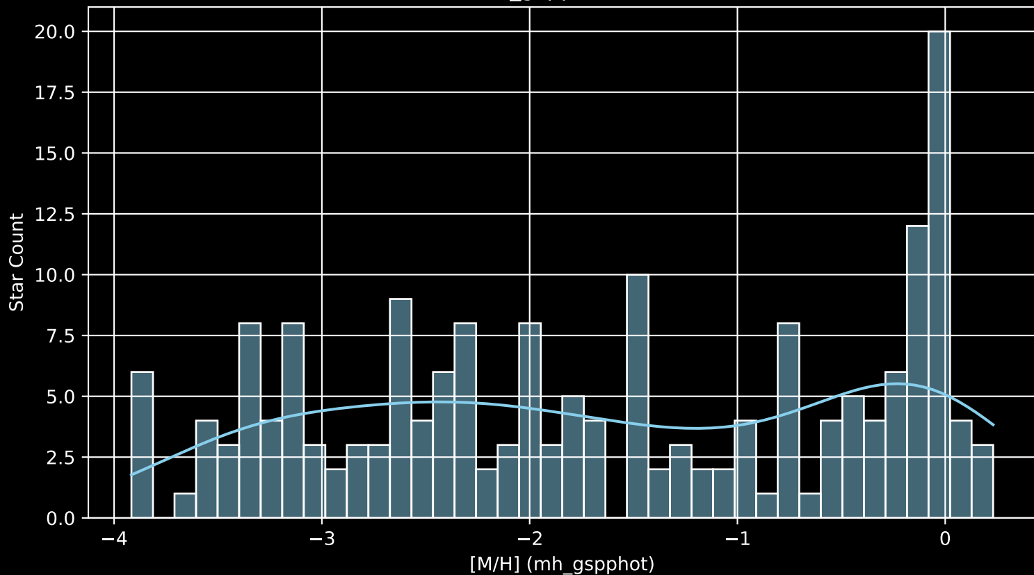
Gaia Cluster: [Berkeley_21 [M/H] (mh_gspphot) (n= 188)
