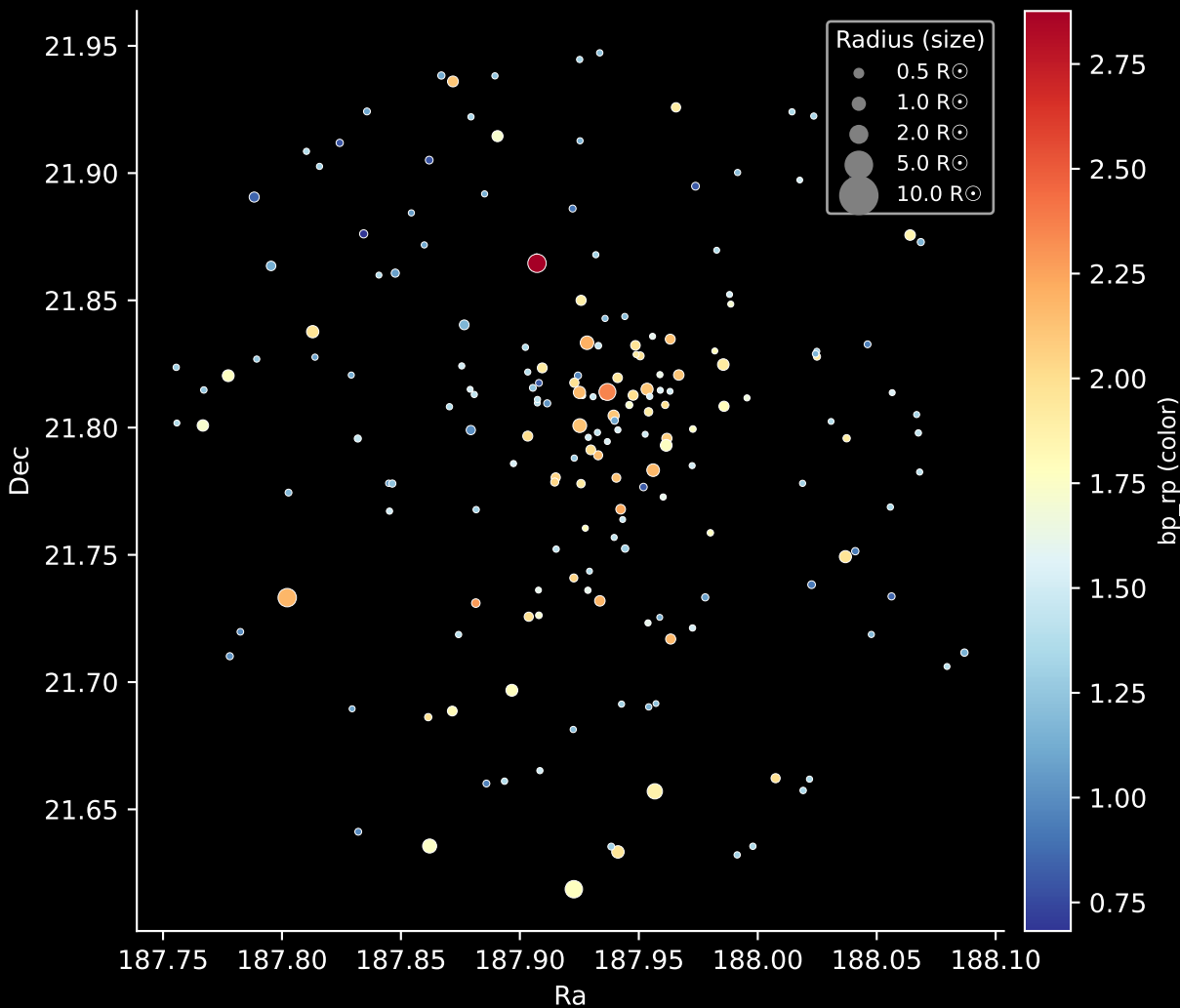
Gaia Cluster: [Berkeley_21] Stars: 188
