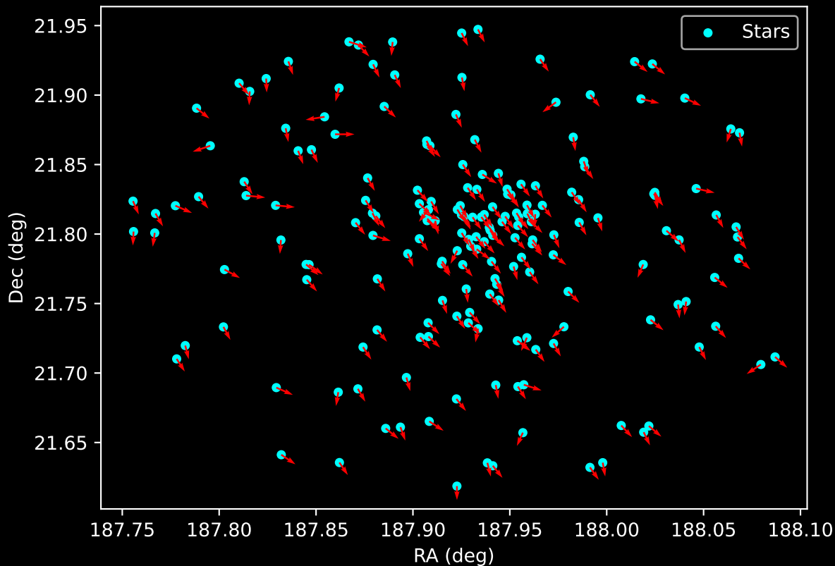
Gaia Cluster: [Berkeley_21] Proper Motion Vectors for Gaia Star Field (n= 188)
