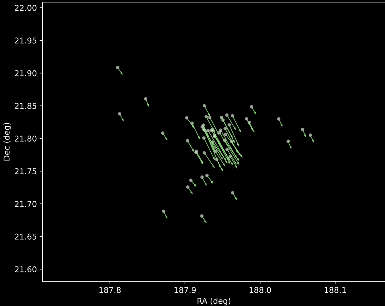
Gaia DR3 Cluster 5 Proper Motion Vectors (n=53)
