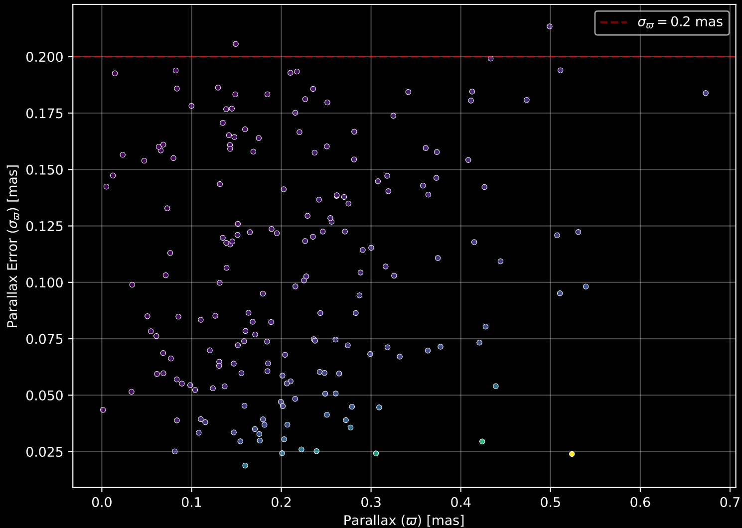
Gaia Cluster: [Berkeley_21] Parallax Quality (n= 188)
