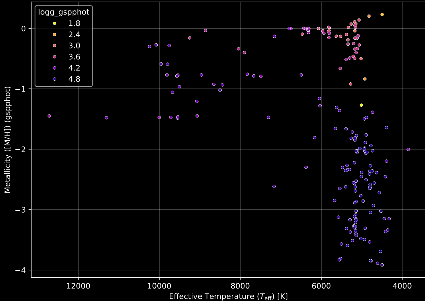
Gaia Cluster: [Berkeley_21] Stellar Population Parameters (n= 188)
