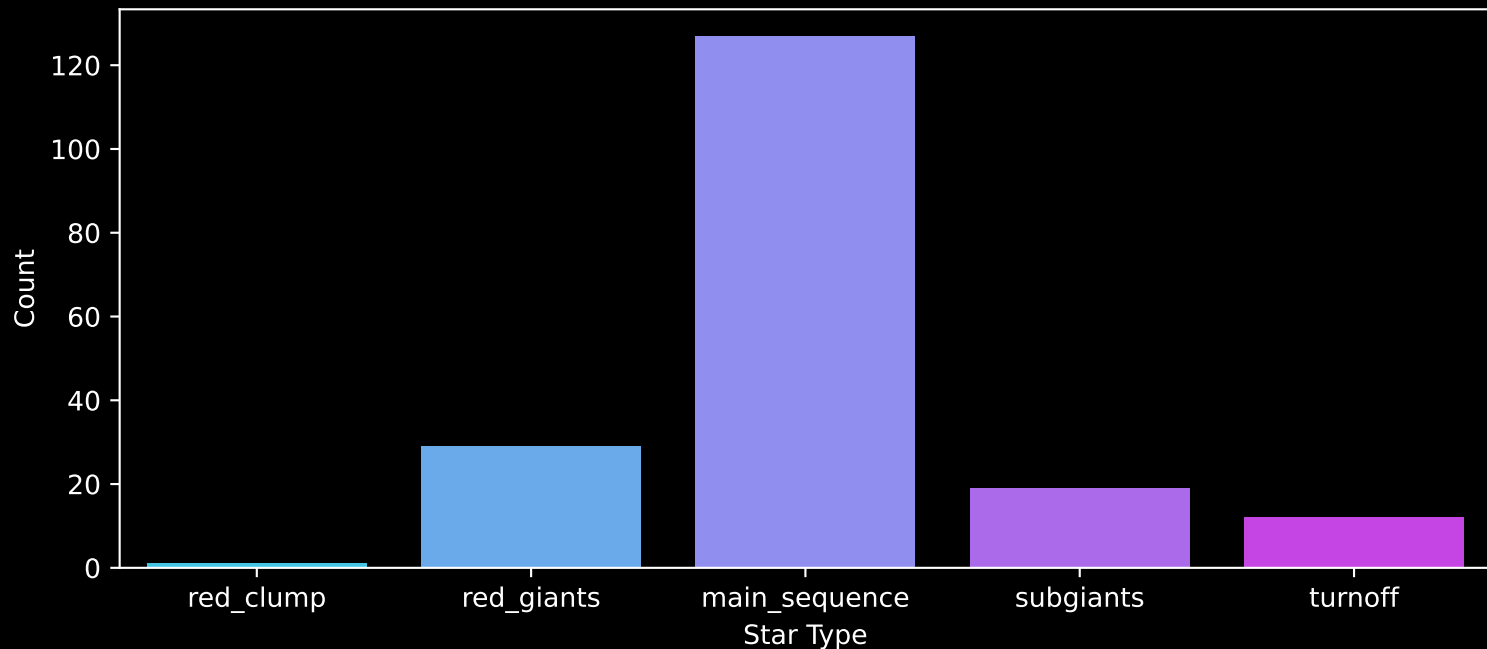
Gaia Cluster: [Berkeley_21] Count plot of Star Type
