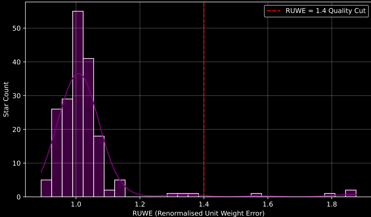
Gaia Cluster: [Berkeley_21] RUWE Distribution (n= 188)
