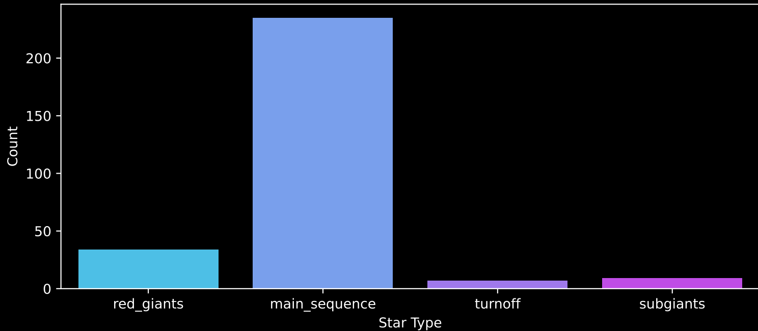
Gaia Cluster: [Berkeley_24] Count plot of Star Type
