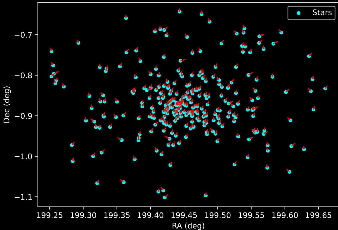
Gaia Cluster: [Berkeley_24] Proper Motion Vectors for Gaia Star Field (n= 285)
