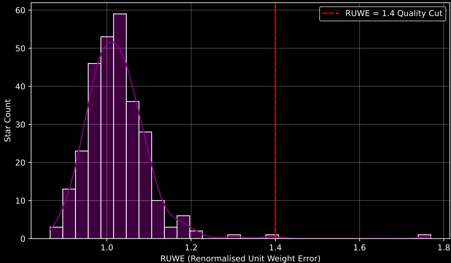
Gaia Cluster: [Berkeley_24] RUWE Distribution (n= 285)
