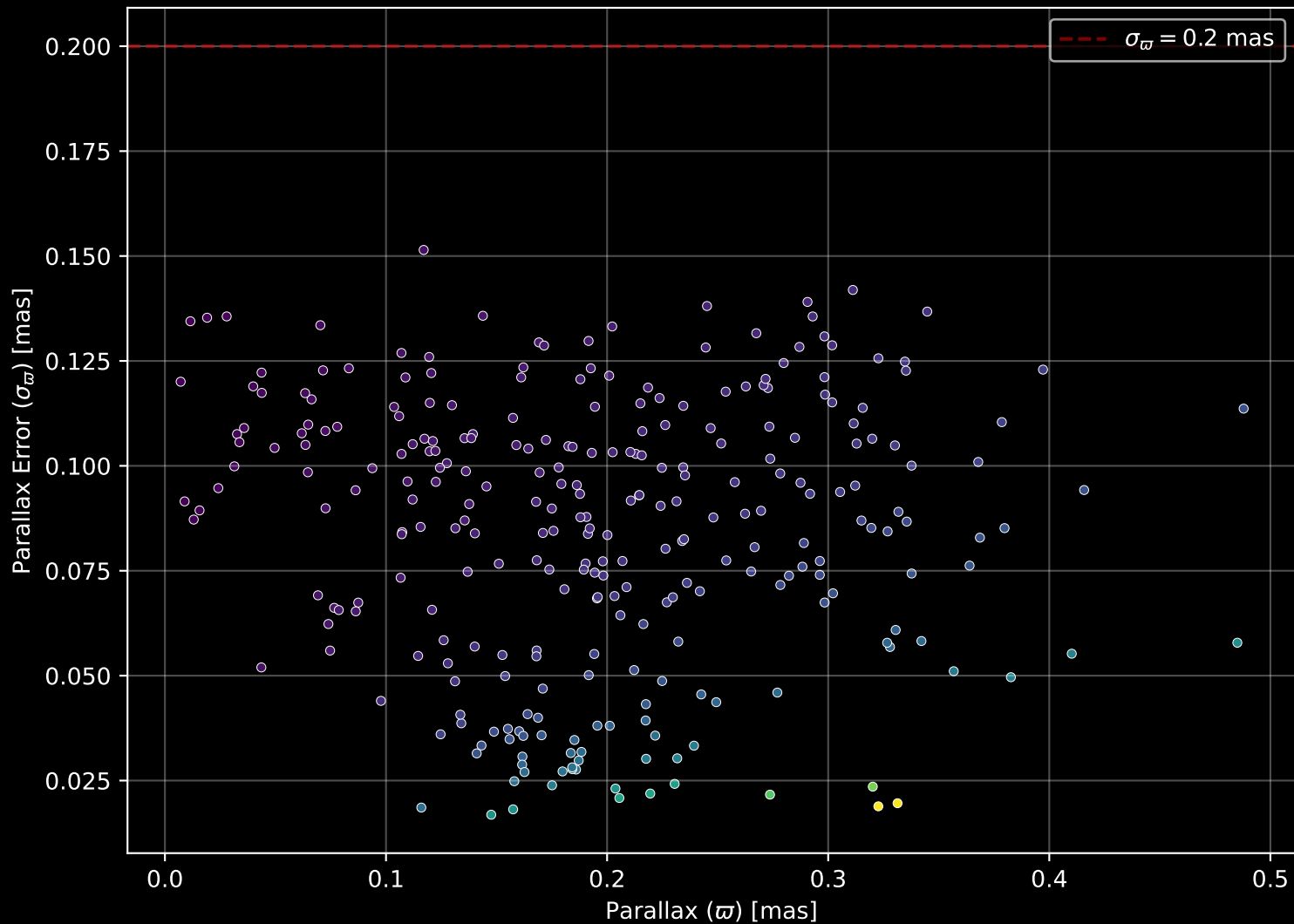
Gaia Cluster: [Berkeley_24] Parallax Quality (n= 285)
