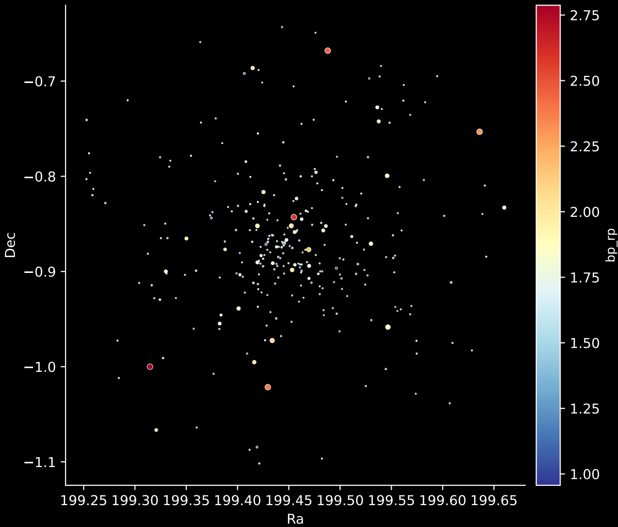
Gaia Cluster: [Berkeley_24] Stars: 285
