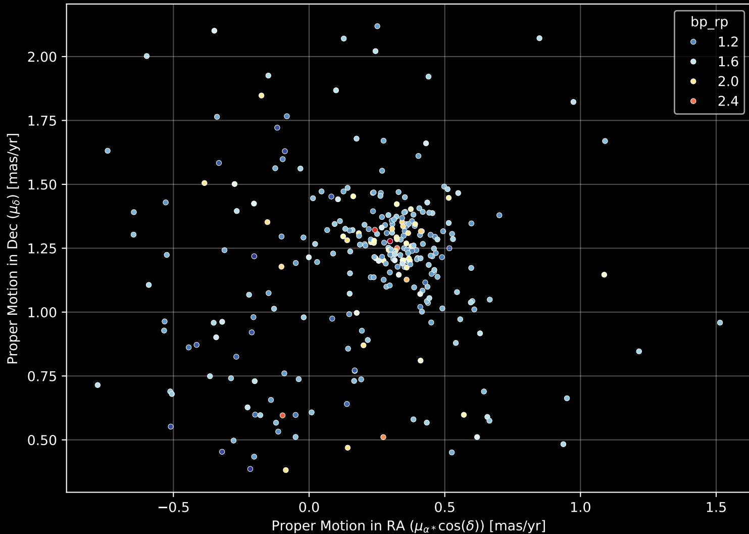
Gaia Cluster: [Berkeley_24] Proper Motion Diagram (n= 285)
