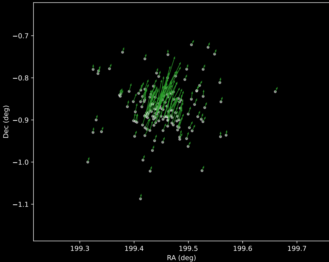
Gaia DR3 Cluster 4 Proper Motion Vectors (n=153)
