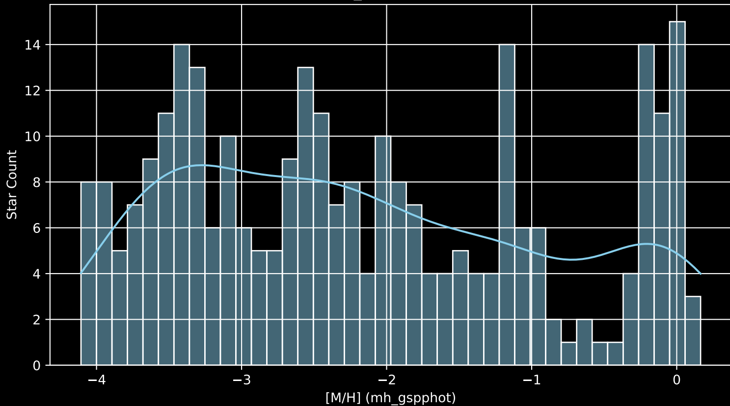
Gaia Cluster: [Berkeley_24 [M/H] (mh_gspphot) (n= 285)
