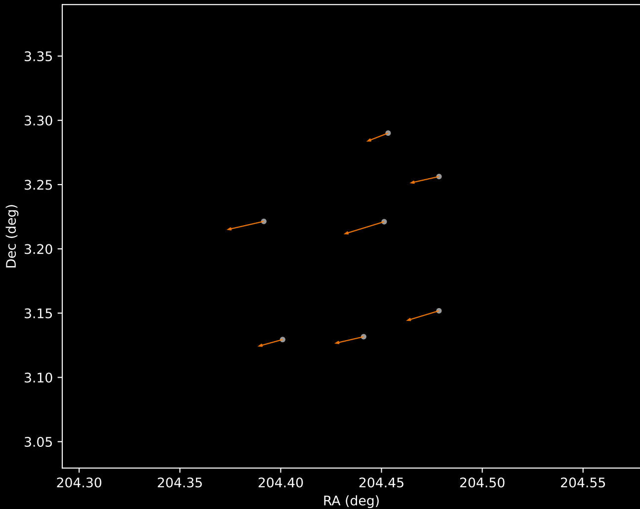
Gaia DR3 Cluster 2 Proper Motion Vectors (n=7)
