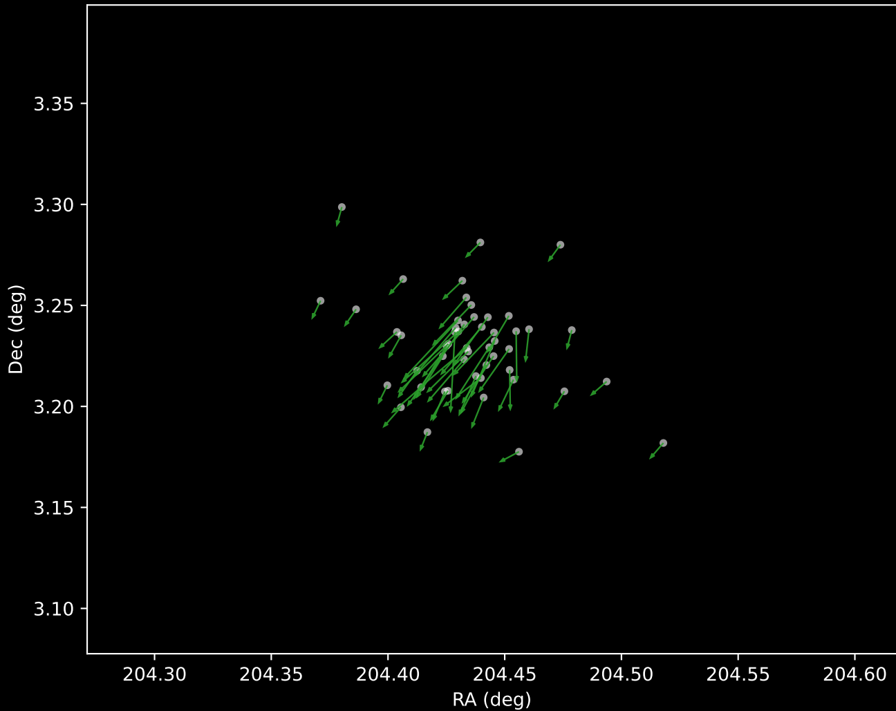
Gaia DR3 Cluster 4 Proper Motion Vectors (n=51)
