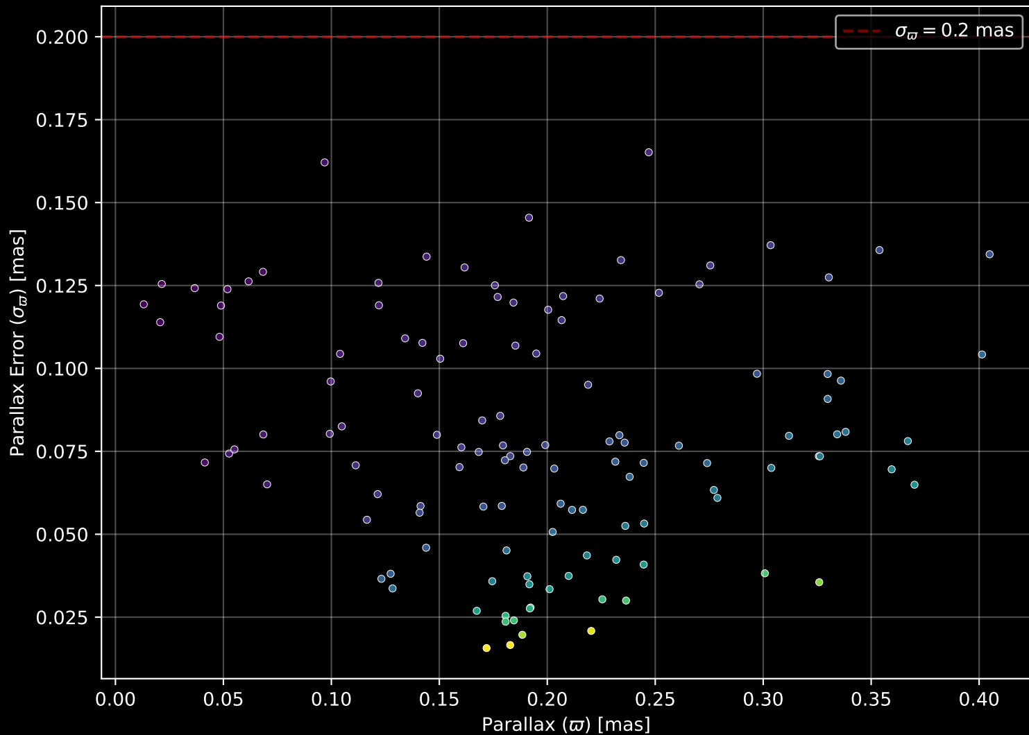
Gaia Cluster: [Berkeley_30] Parallax Quality (n= 125)
