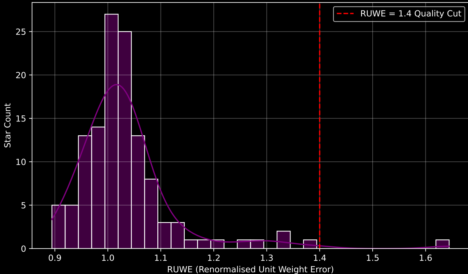
Gaia Cluster: [Berkeley_30] RUWE Distribution (n= 125)
