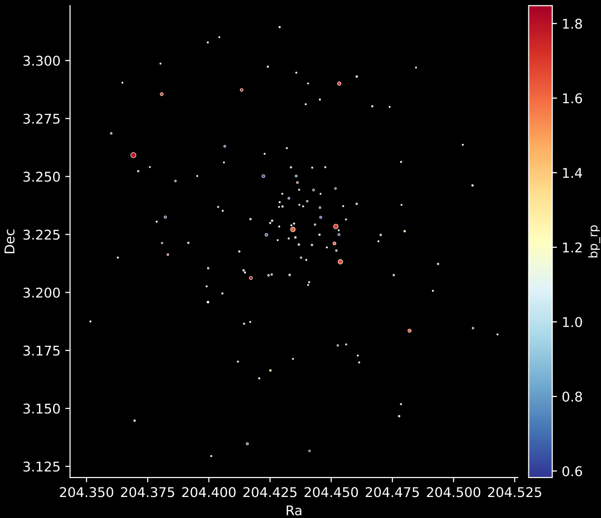
Gaia Cluster: [Berkeley_30] Stars: 125
