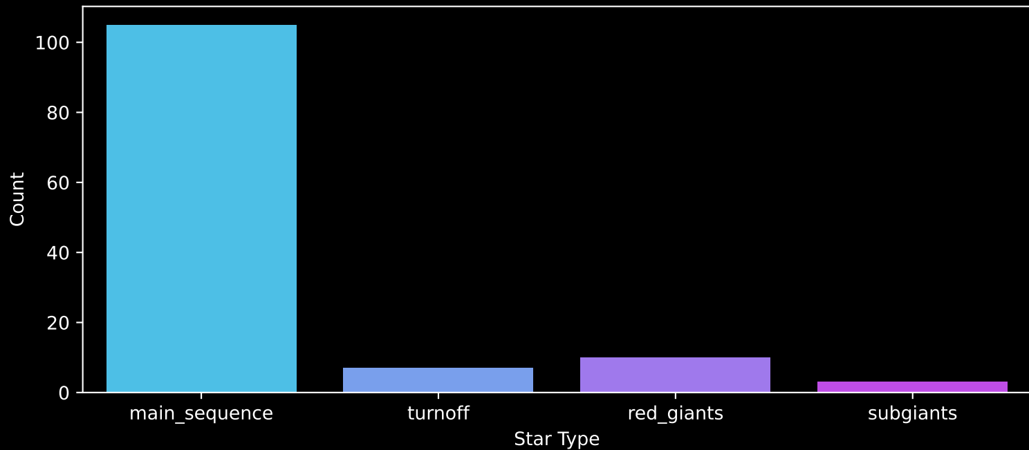
Gaia Cluster: [Berkeley_30] Count plot of Star Type
