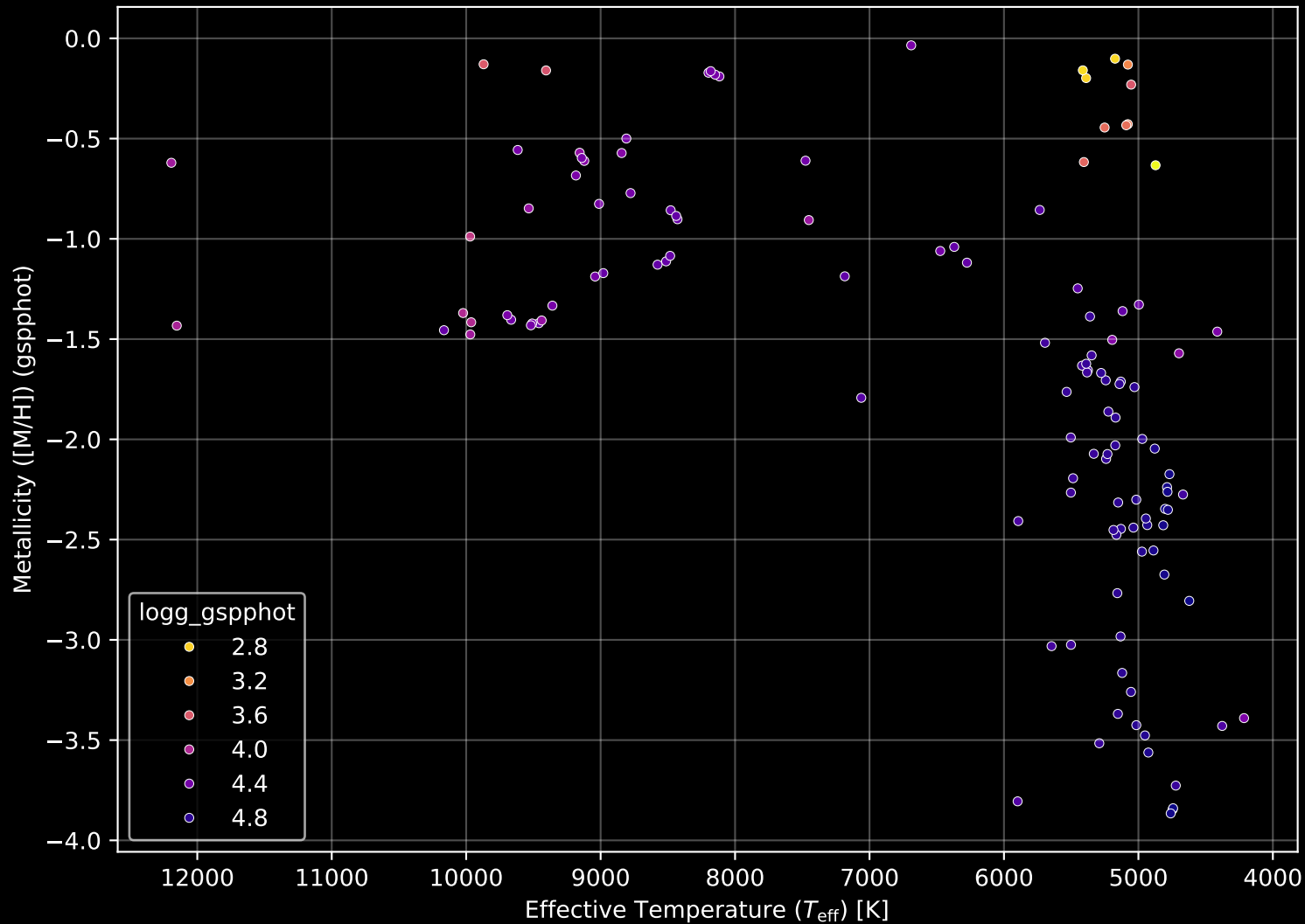
Gaia Cluster: [Berkeley_30] Stellar Population Parameters (n= 125)
