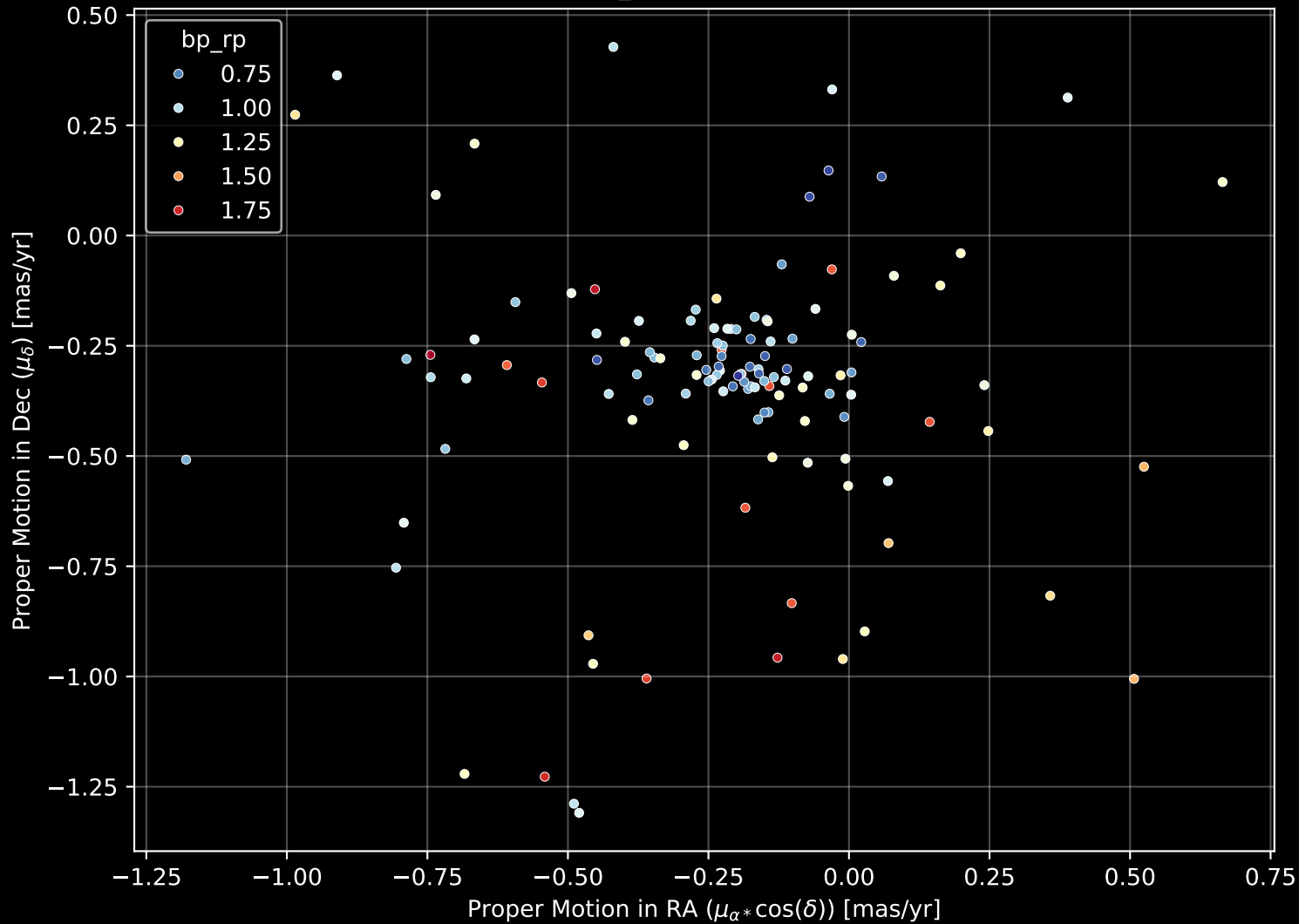
Gaia Cluster: [Berkeley_30] Proper Motion Diagram (n= 125)
