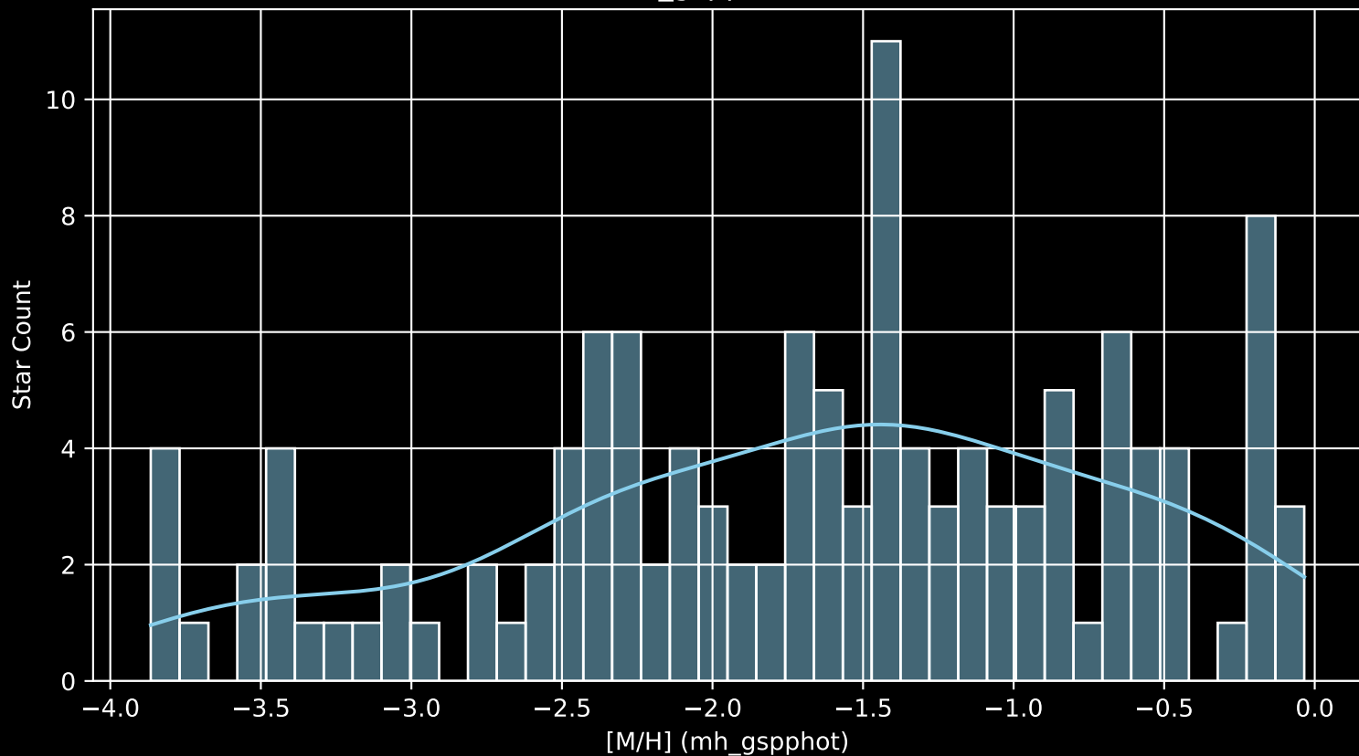
Gaia Cluster: [Berkeley_30 [M/H] (mh_gspphot) (n= 125)
