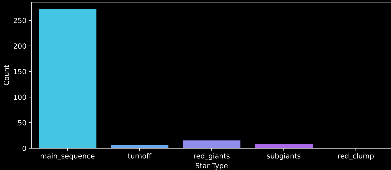
Gaia Cluster: [Berkeley_31] Count plot of Star Type
