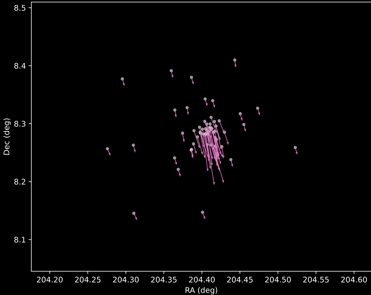
Gaia DR3 Cluster 12 Proper Motion Vectors (n=58)
