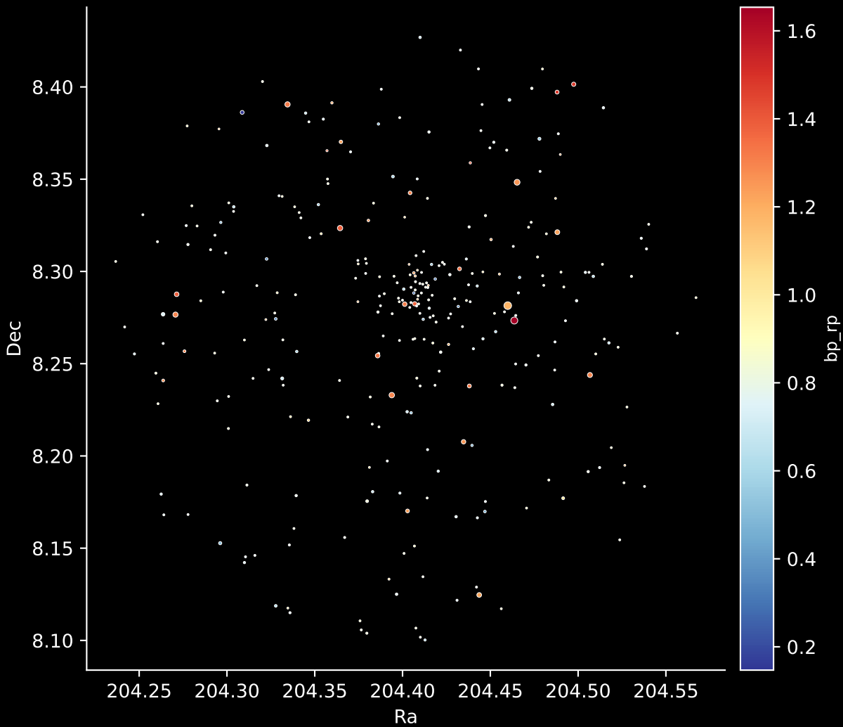
Gaia Cluster: [Berkeley_31] Stars: 303
