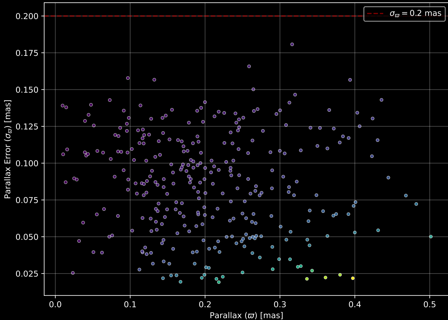
Gaia Cluster: [Berkeley_31] Parallax Quality (n= 303)
