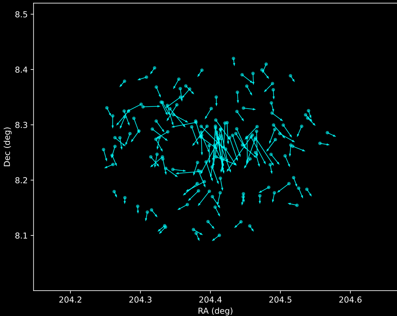
Gaia DR3 Noise Stream Proper Motion Vectors (n=152)
