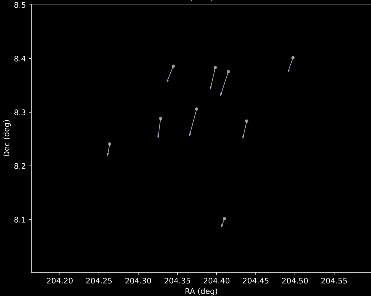
Gaia DR3 Cluster 9 Proper Motion Vectors (n=9)
