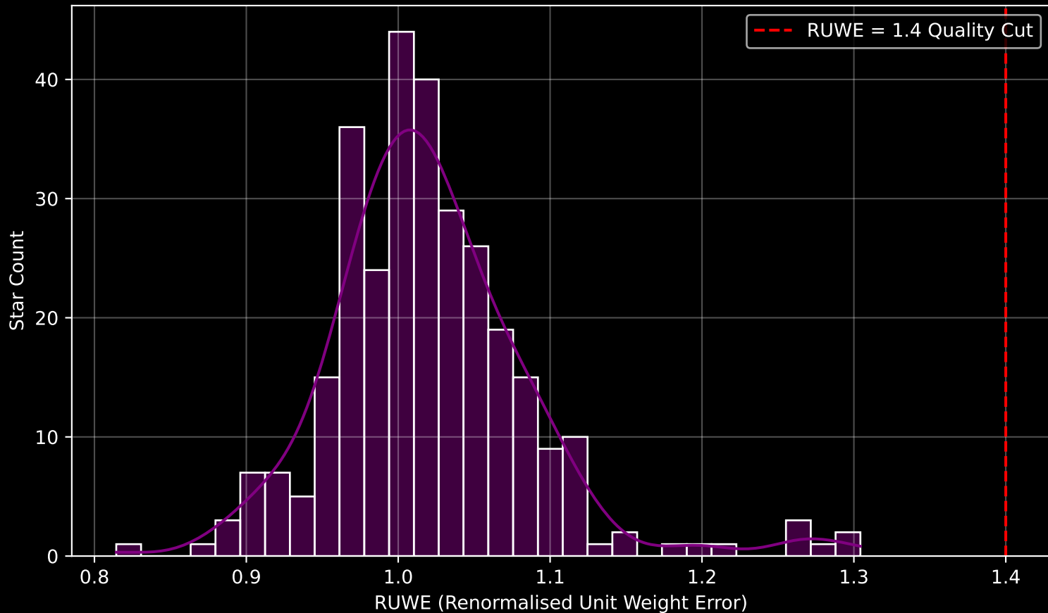
Gaia Cluster: [Berkeley_31] RUWE Distribution (n= 303)
