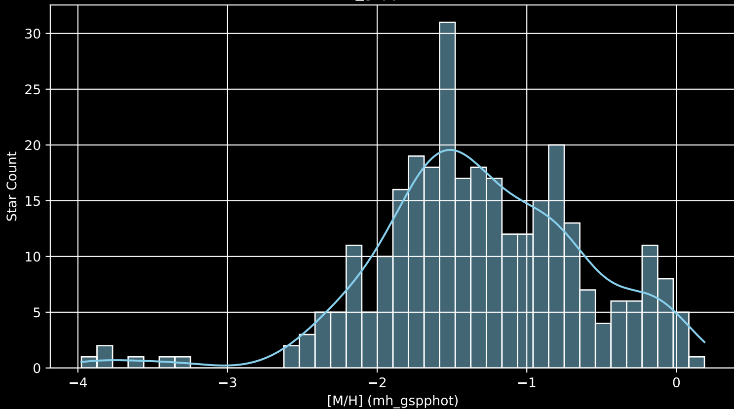
Gaia Cluster: [Berkeley_31 [M/H] (mh_gspphot) (n= 303)
