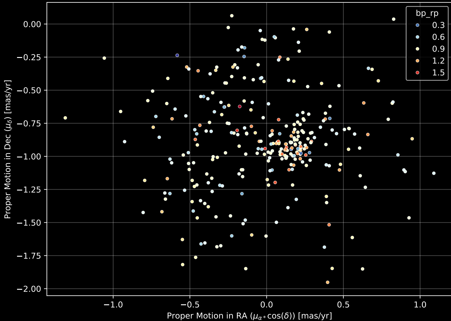
Gaia Cluster: [Berkeley_31] Proper Motion Diagram (n= 303)
