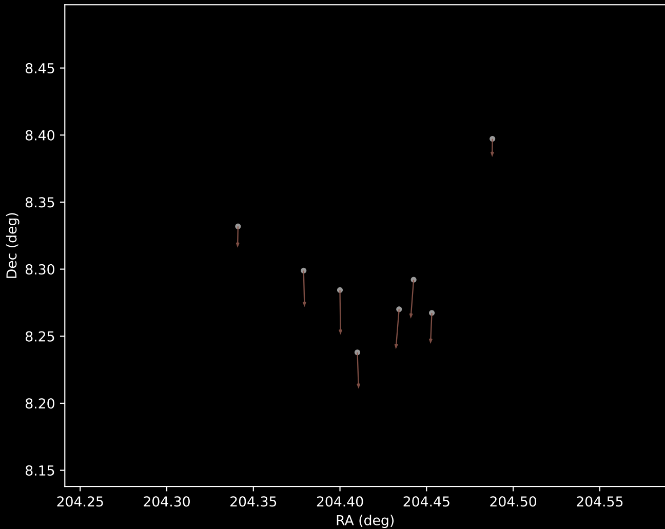
Gaia DR3 Cluster 10 Proper Motion Vectors (n=8)
