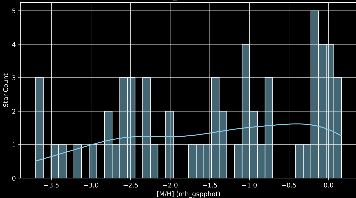
Gaia Cluster: [Berkeley_34 [M/H] (mh_gspphot) (n= 59)
