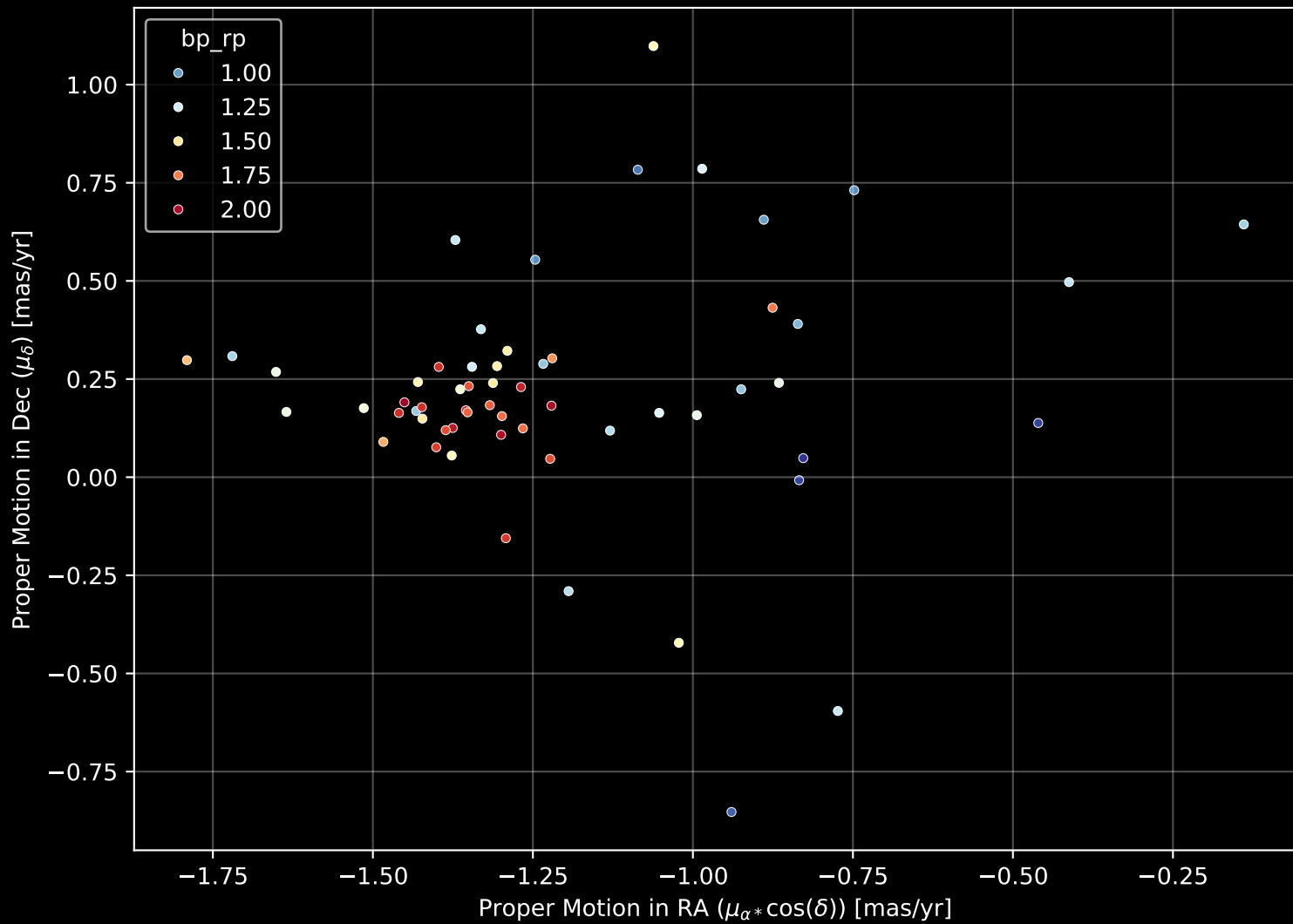
Gaia Cluster: [Berkeley_34] Proper Motion Diagram (n= 59)
