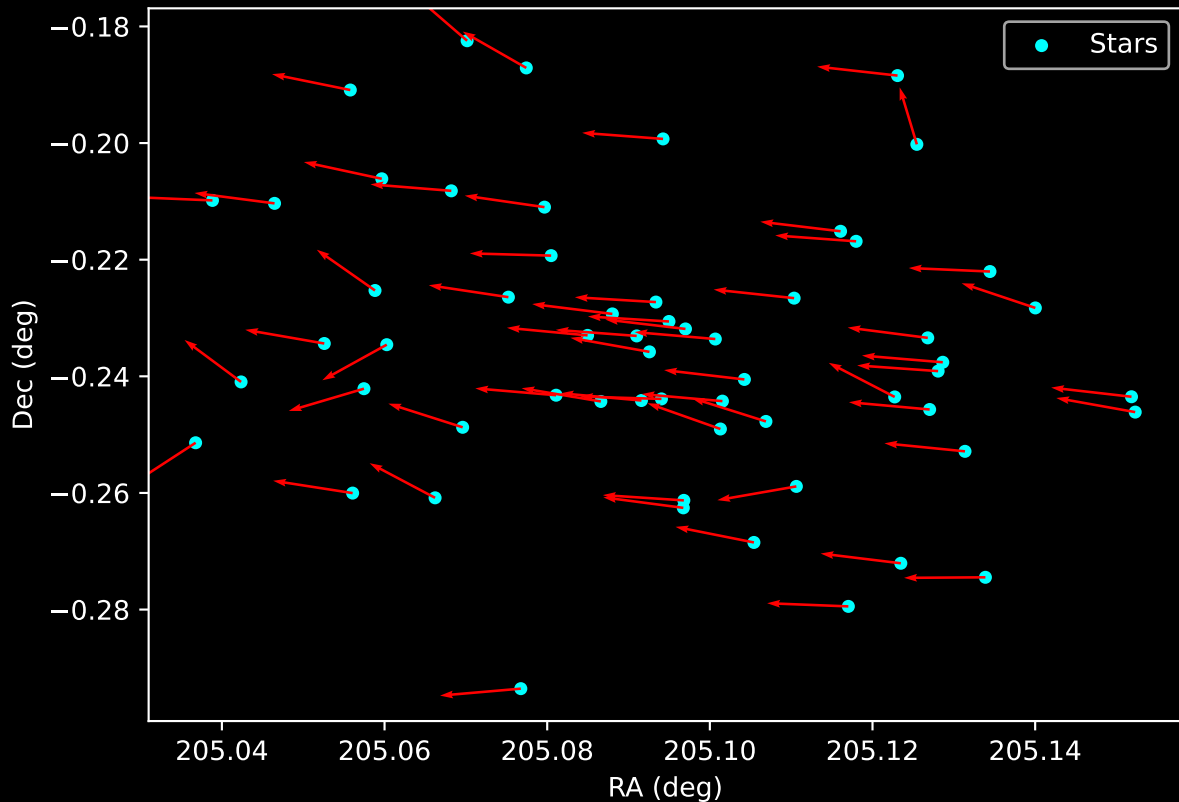
Gaia Cluster: [Berkeley_34] Proper Motion Vectors for Gaia Star Field (n= 59)
