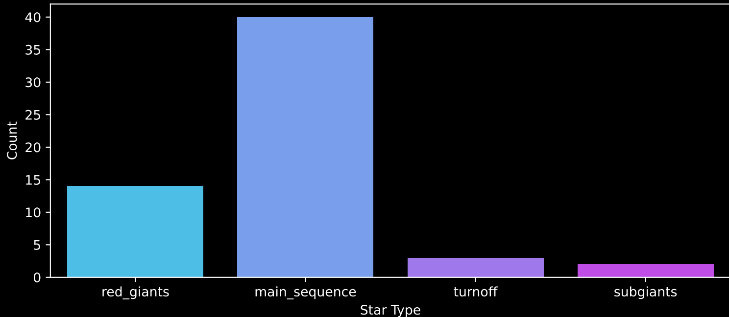
Gaia Cluster: [Berkeley_34] Count plot of Star Type
