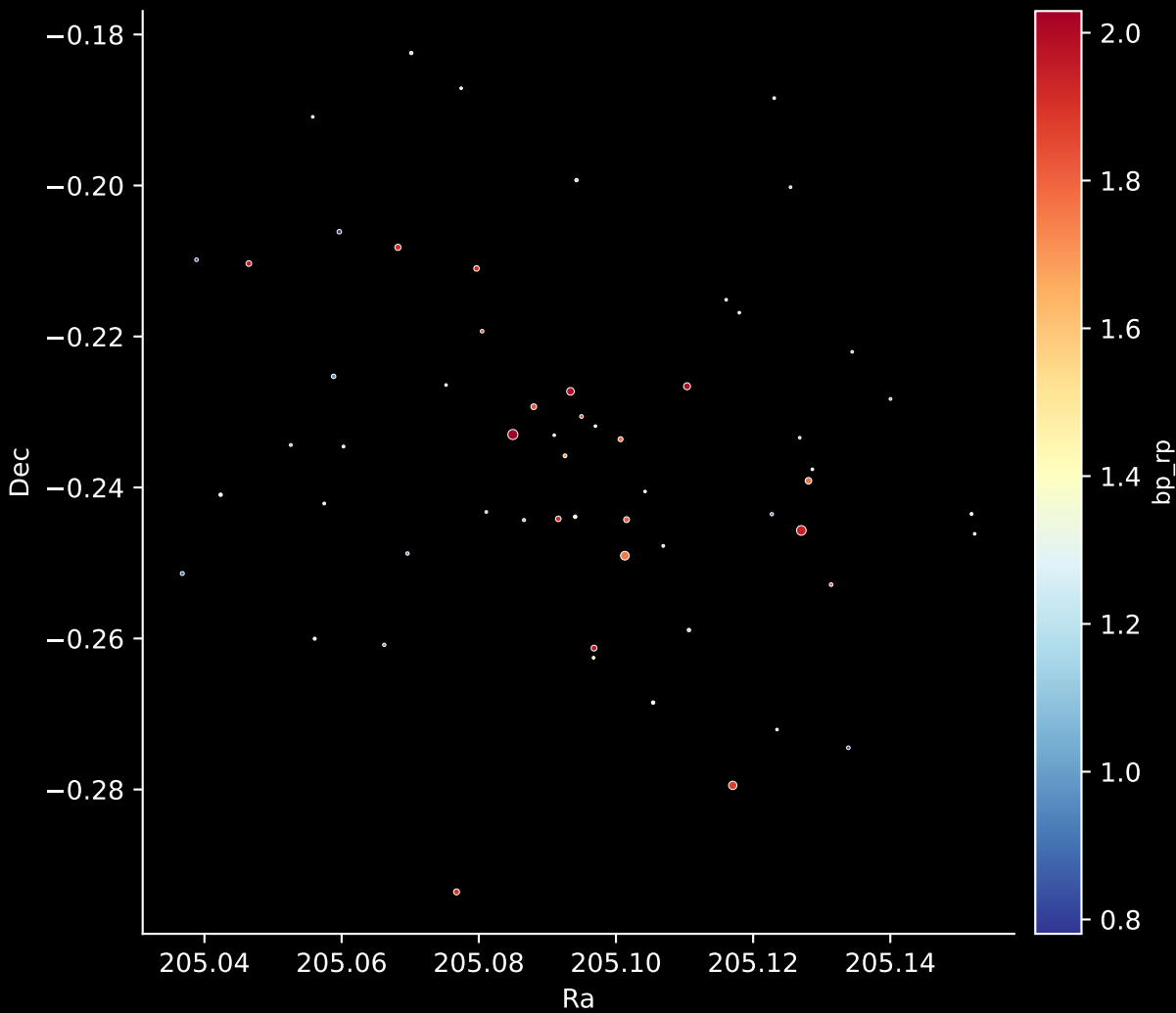
Gaia Cluster: [Berkeley_34] Stars: 59
