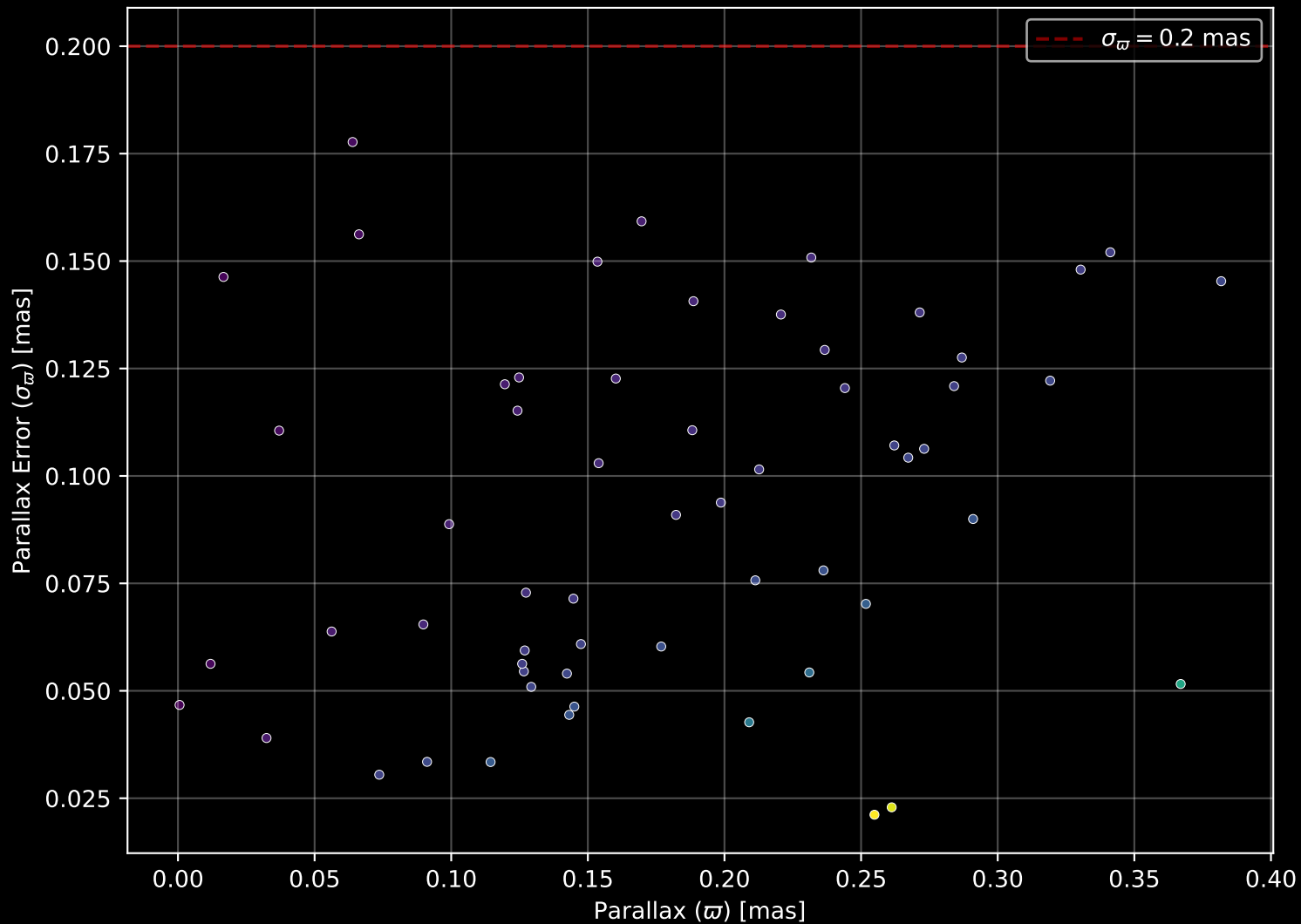
Gaia Cluster: [Berkeley_34] Parallax Quality (n= 59)
